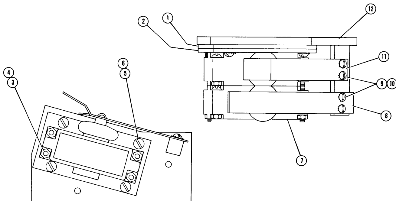
FIG. 8104B TICKER SWITCH
