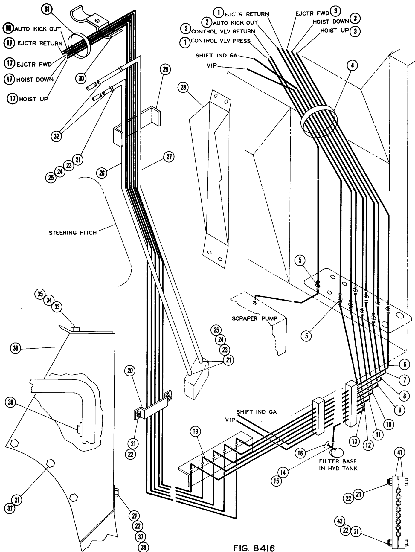
SCRAPER CONTROL PIPING
