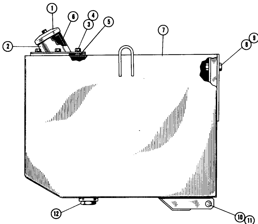
FIG. 7359 B FUEL TANK
