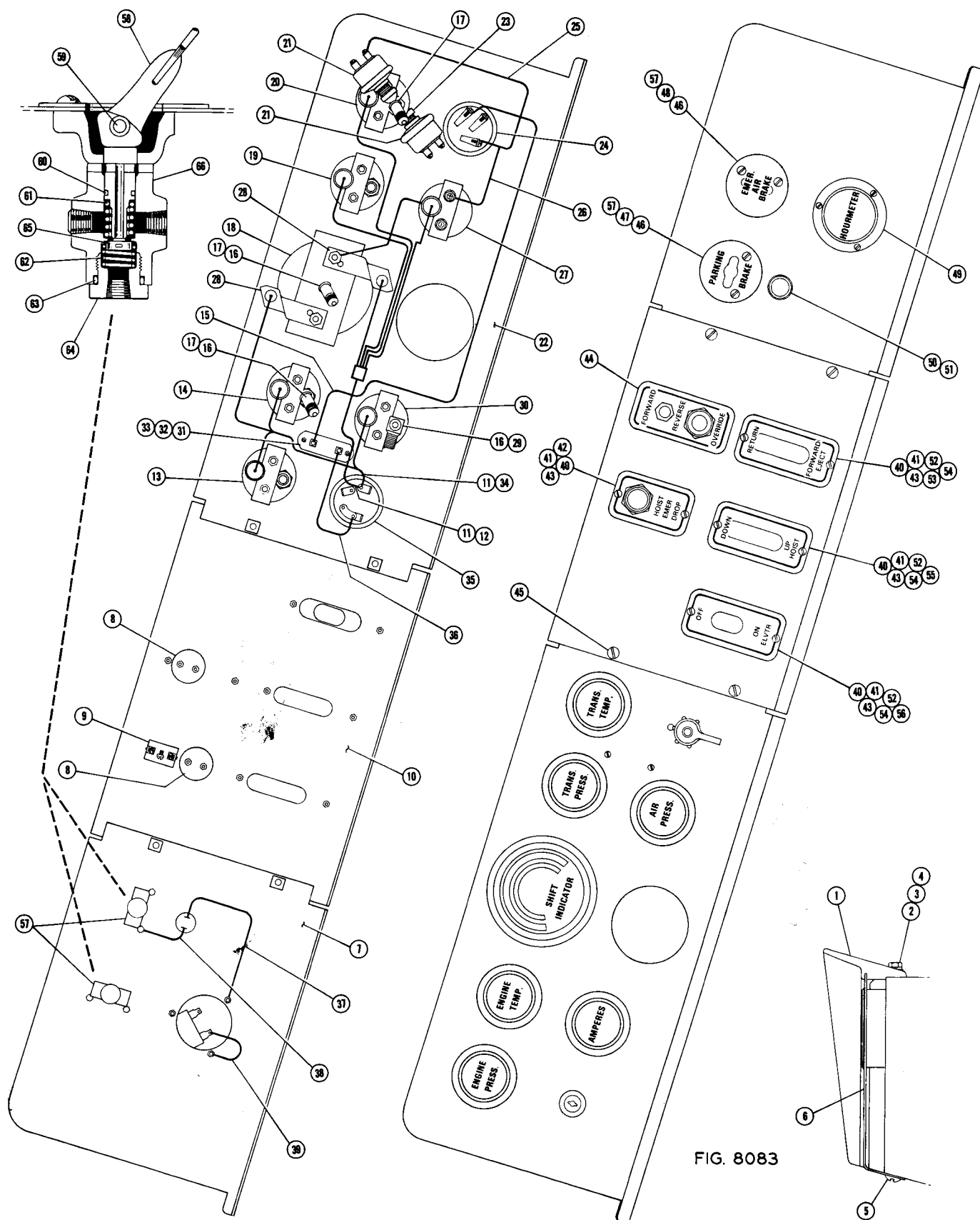
INSTRUMENT PANEL
