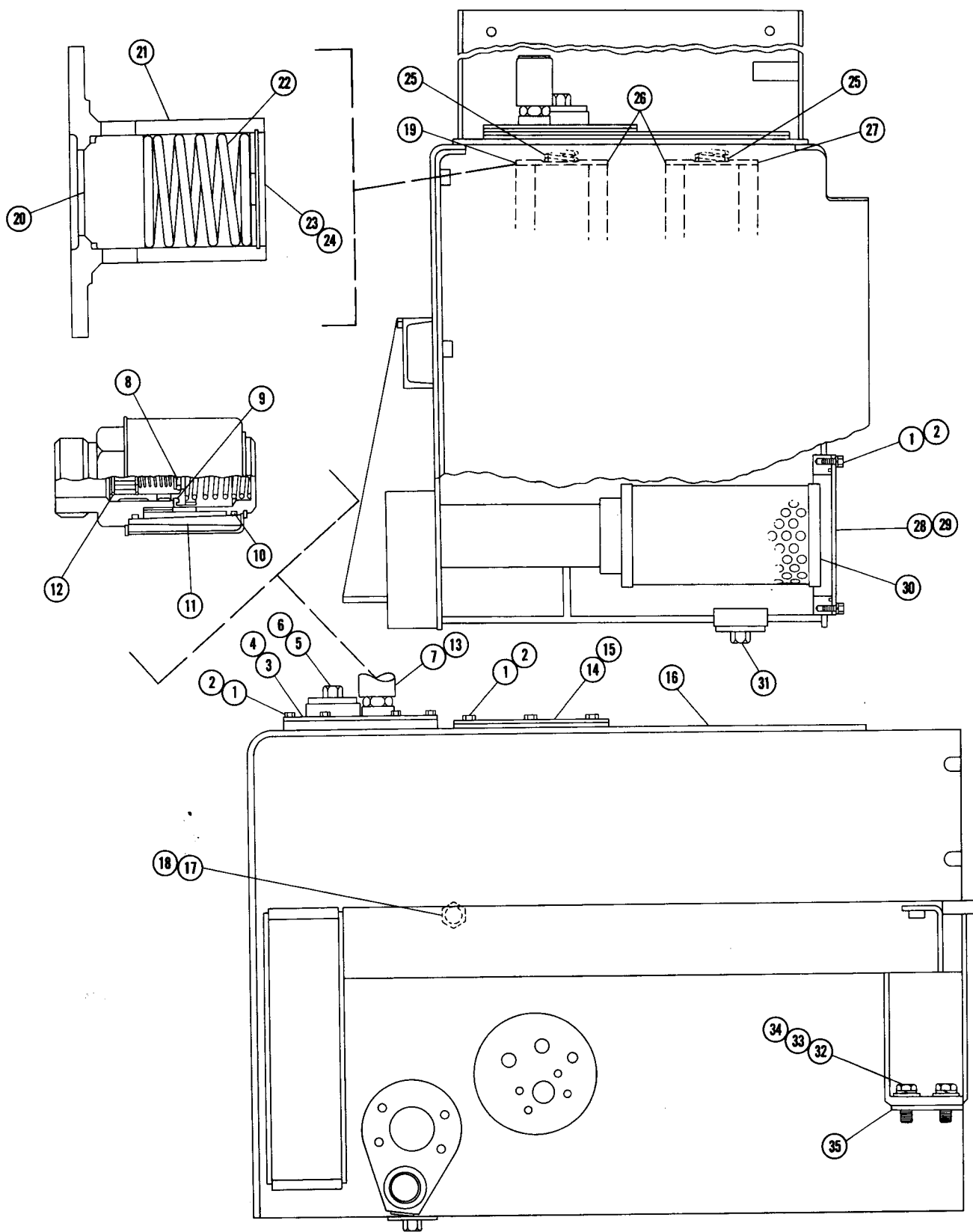
FIG. 5938 HYDRAULIC TANK
