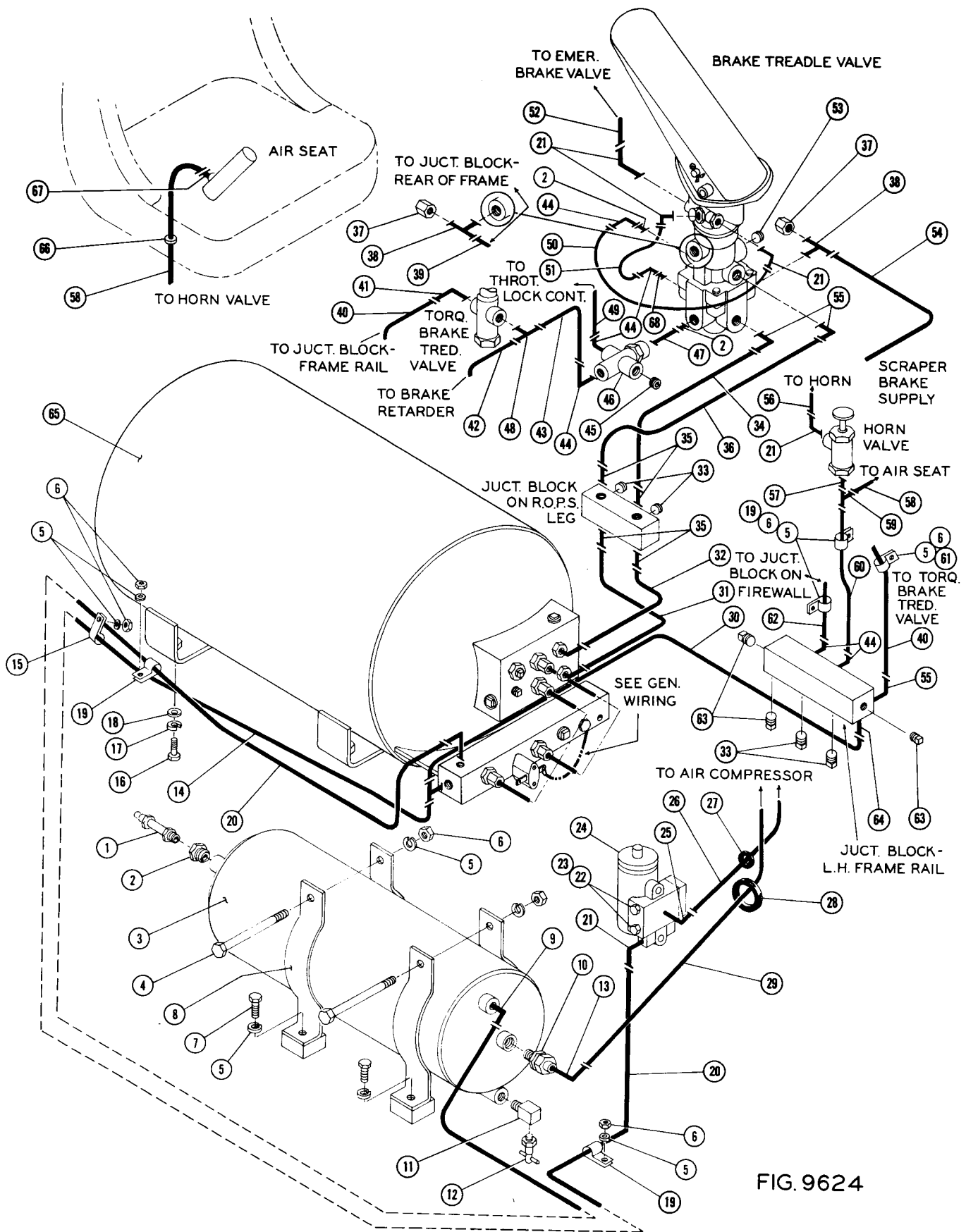
AIR SYSTEM PIPING
