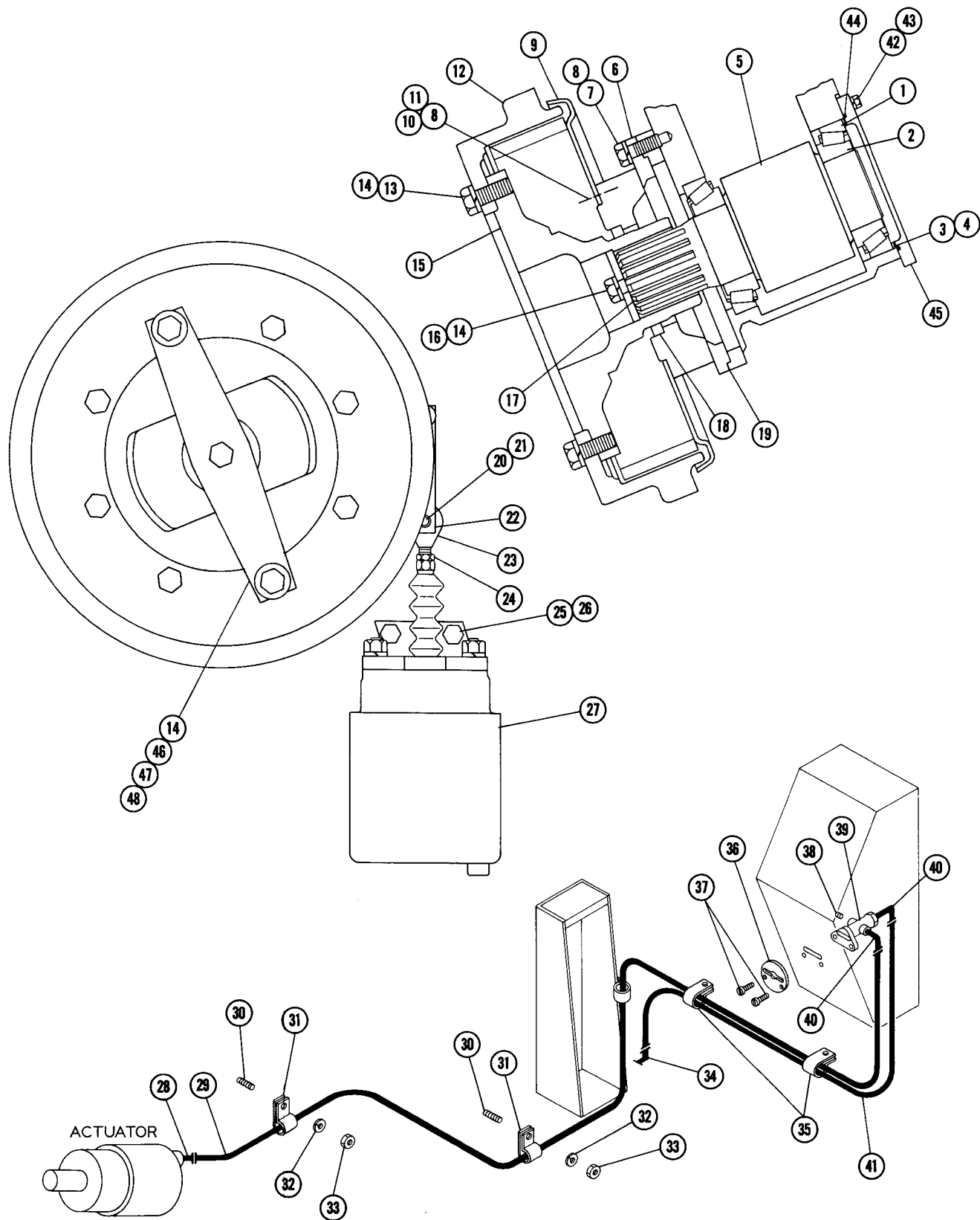
FIG. 8062 PARKING BRAKE
