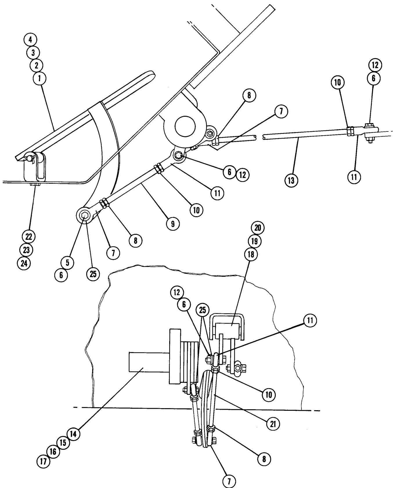
FIG. 8362 THROTTLE LINKAGE
