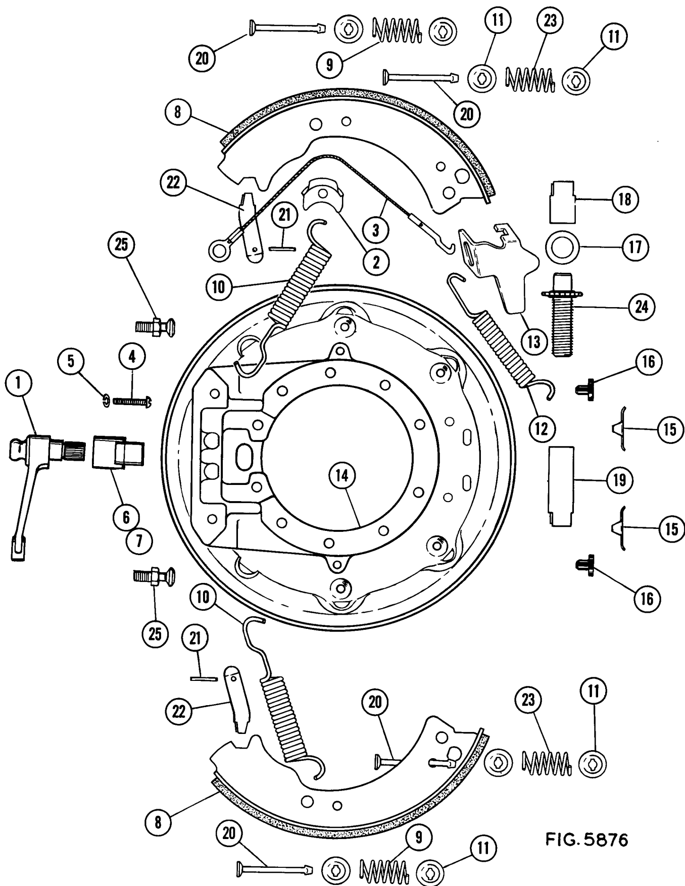
PARKING BRAKE
