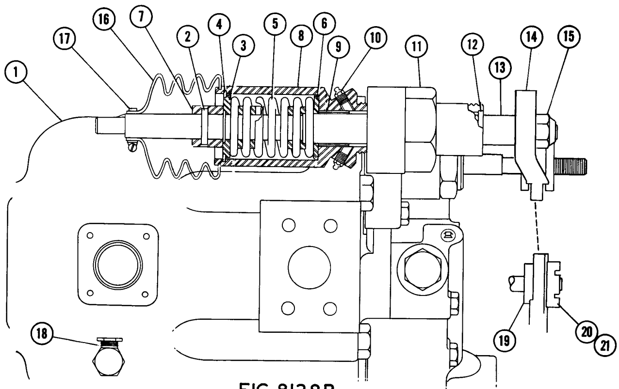
STEERING PUMP ASSY.
