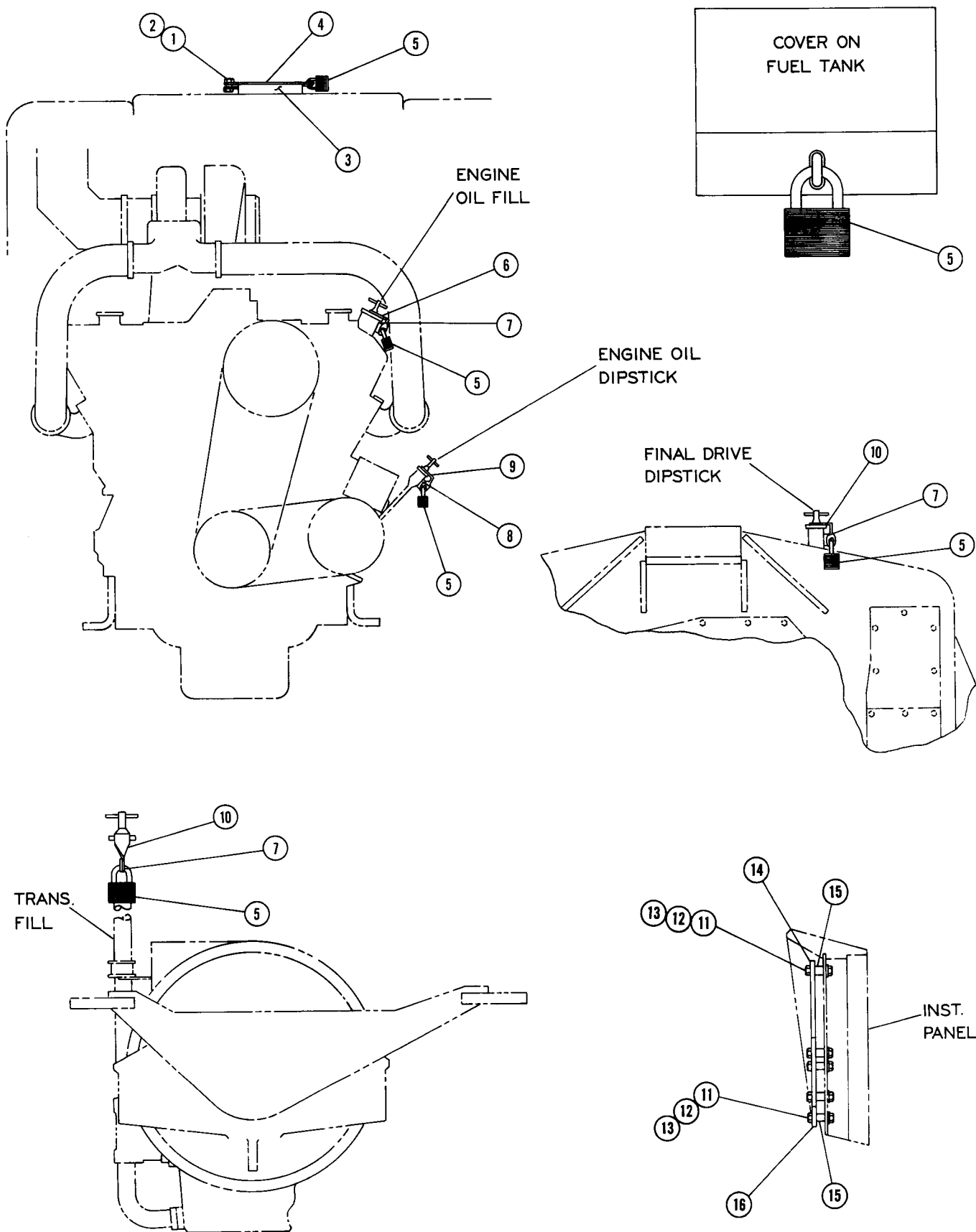
FIG. 8581 VANDALISM PROTECTION
