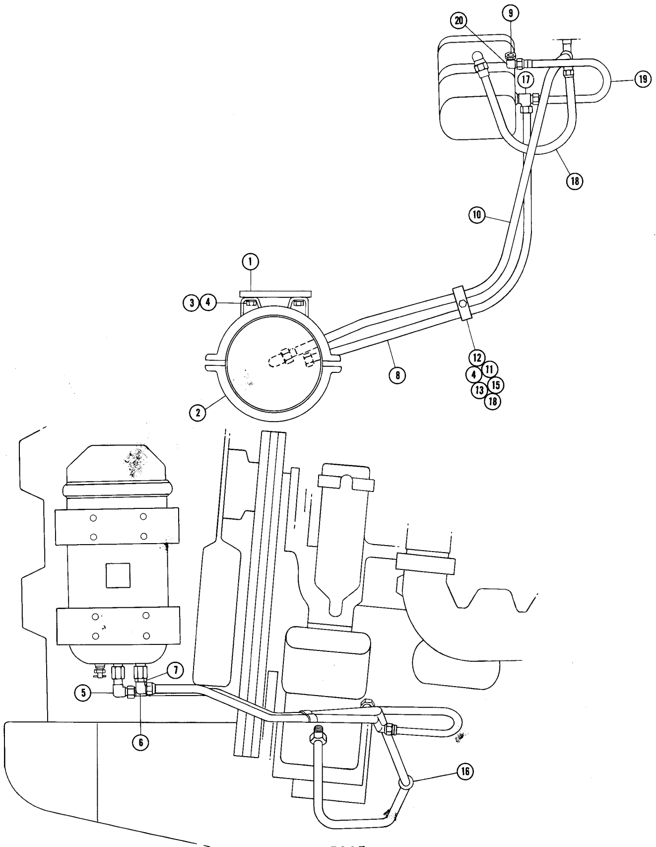
FIG. 5985 LUBE FILTER, BY-PASS
