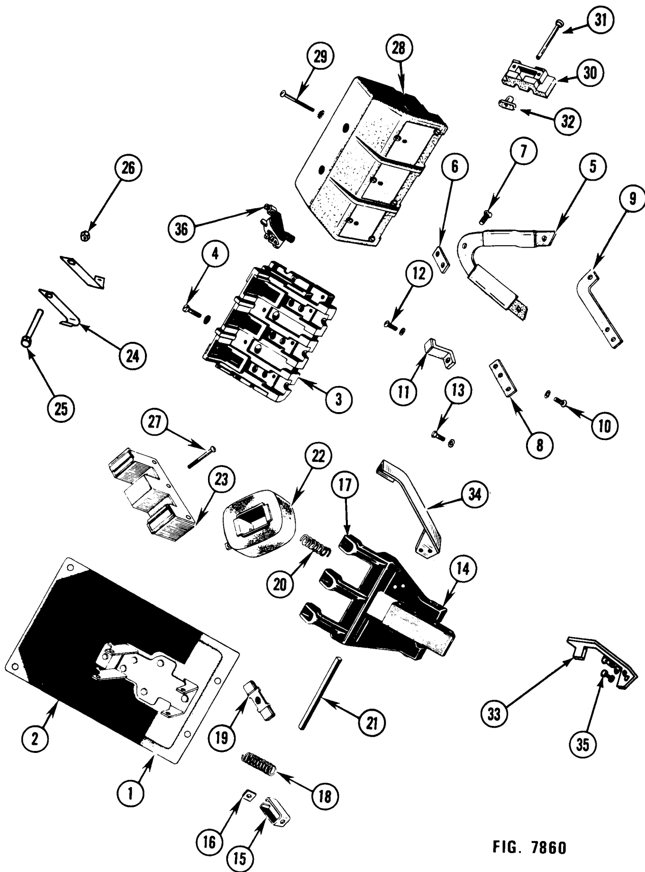
CONTACTOR SWITCH
