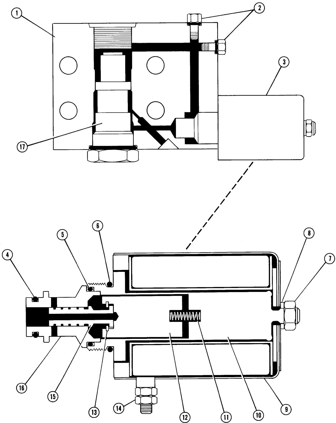
FIG. 8133 MANIFOLD ASSEMBLY
