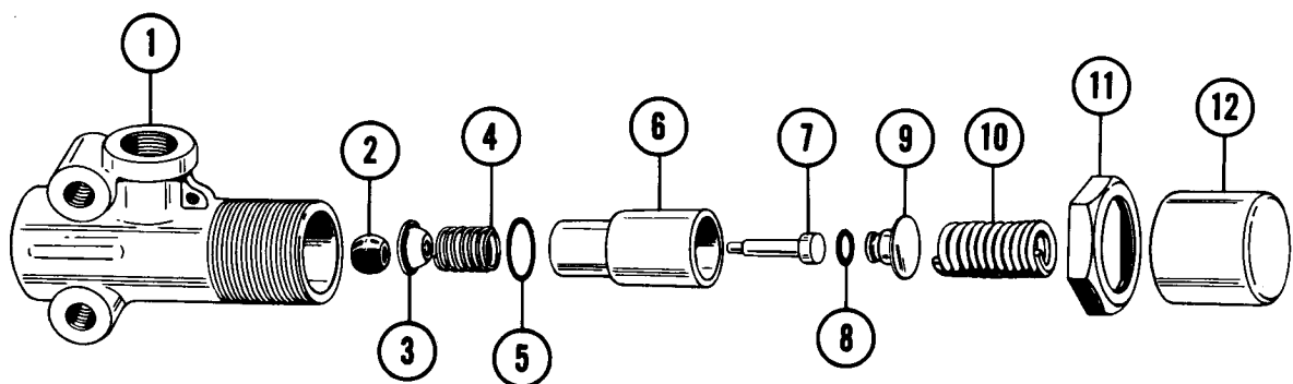
FIG. 740I C PRESSURE PROTECTION VALVE
