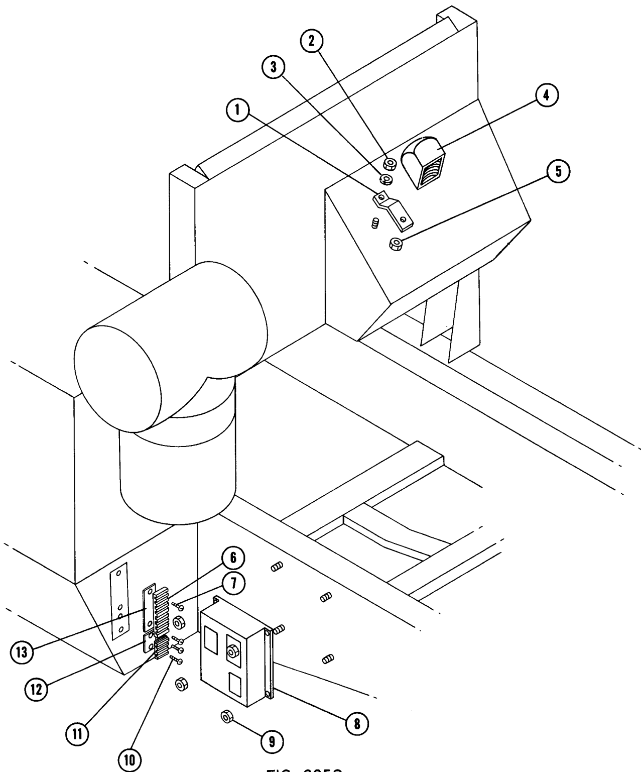
FIG. 6052 COMPONENTS - ELECTRICAL
