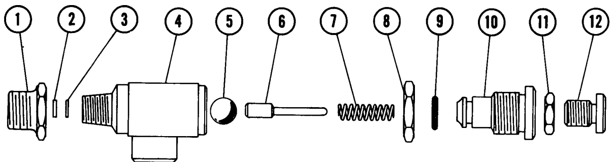
FIG. 740I B COMPRESSOR UNLOADER VALVE
