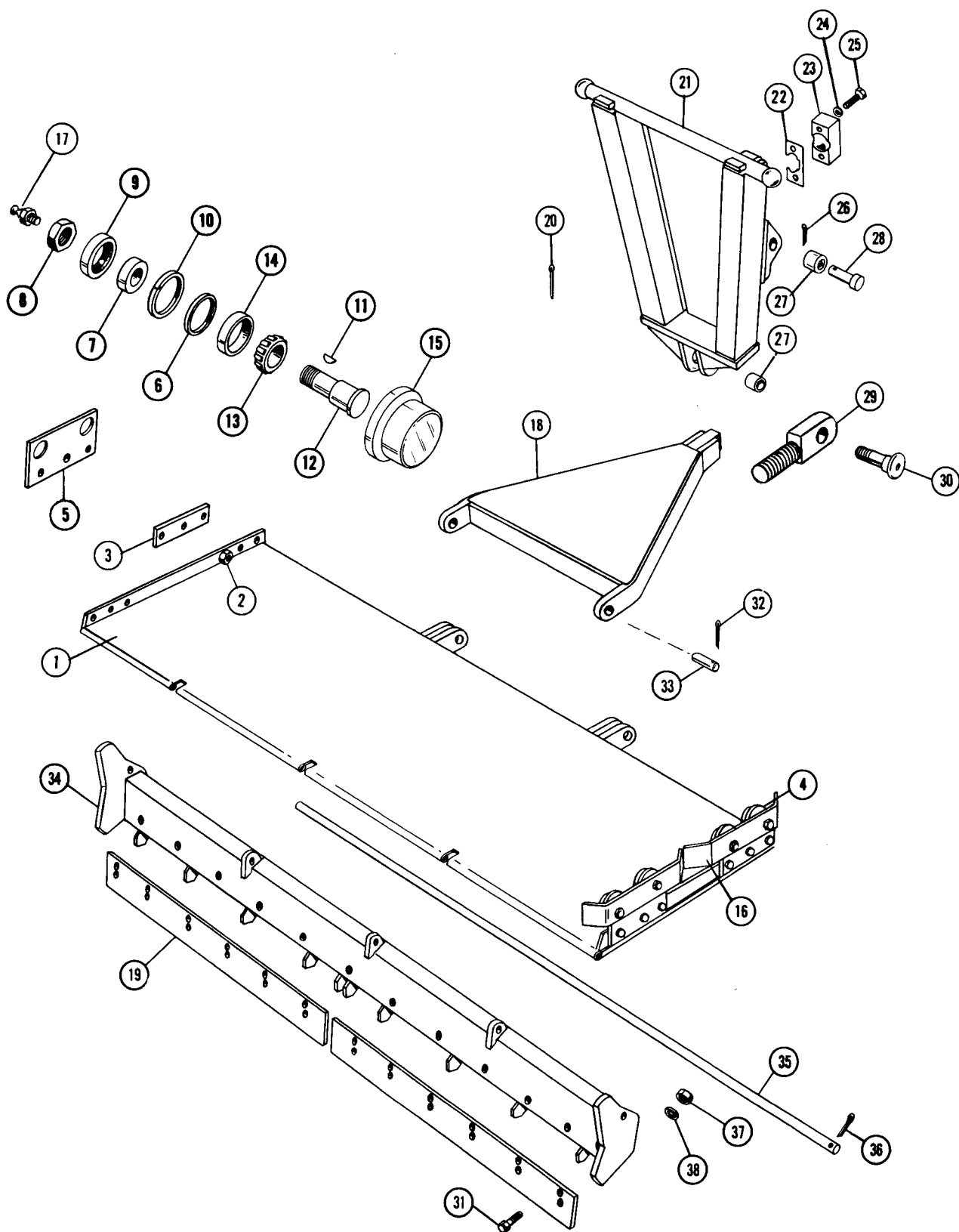
FIG. 6081 BOTTOM-ROLLING
