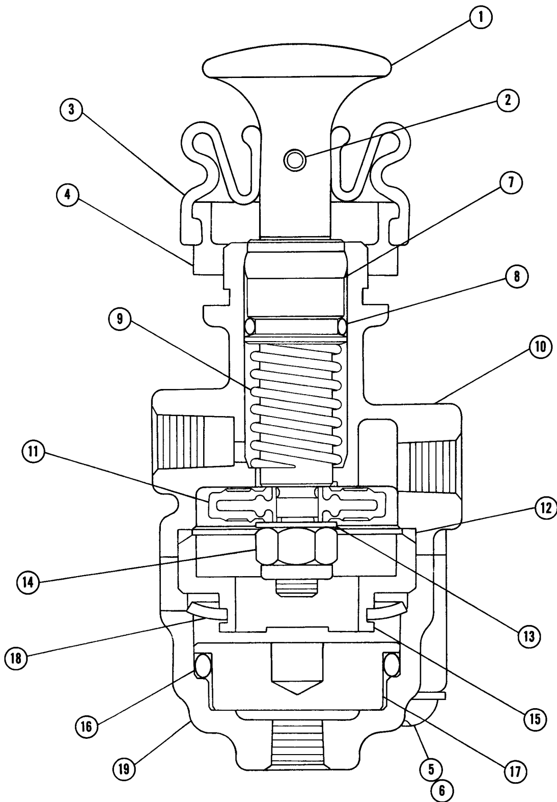
FIG. 6075 VALVE-CONTROL
