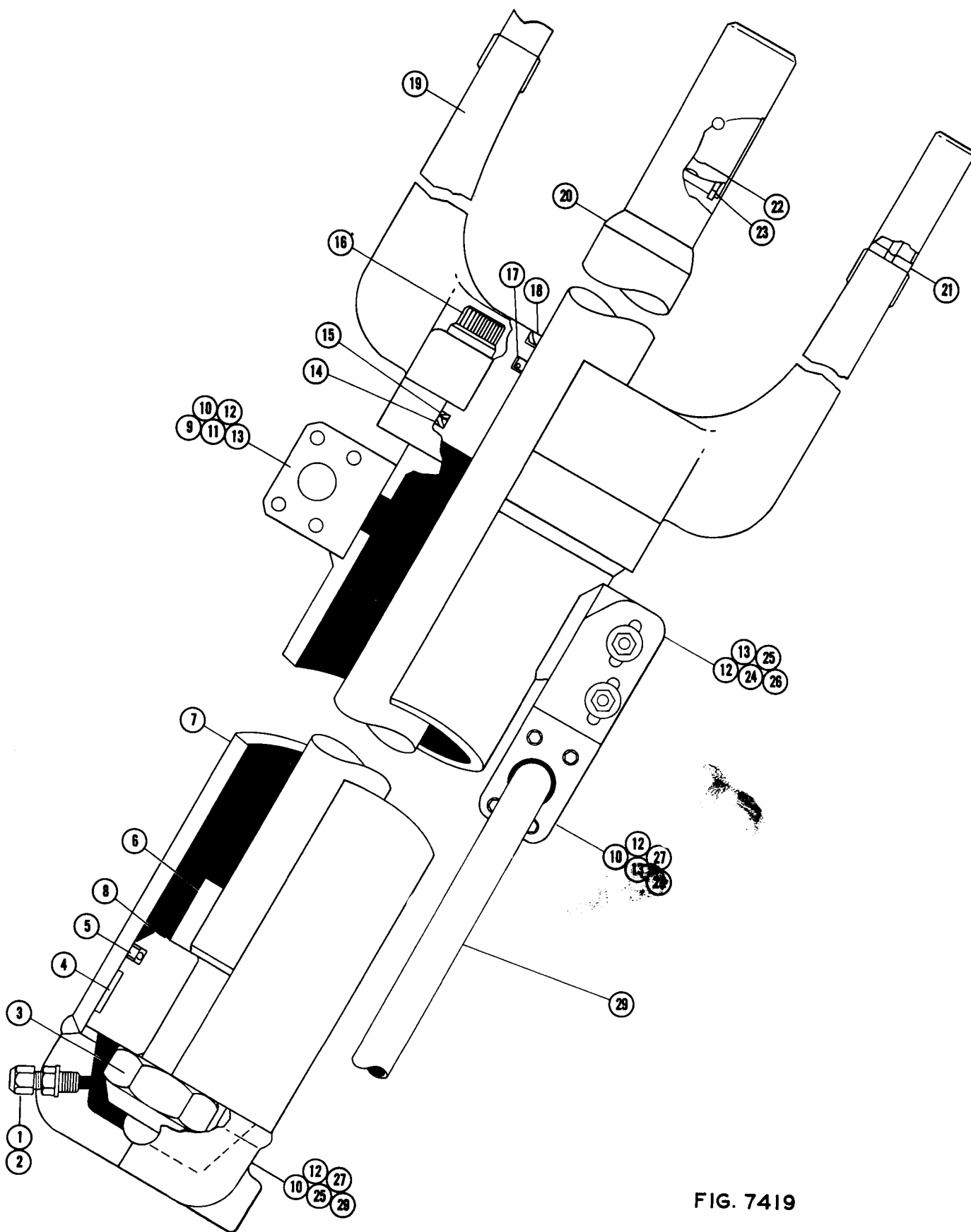
STEERING CYLINDER
