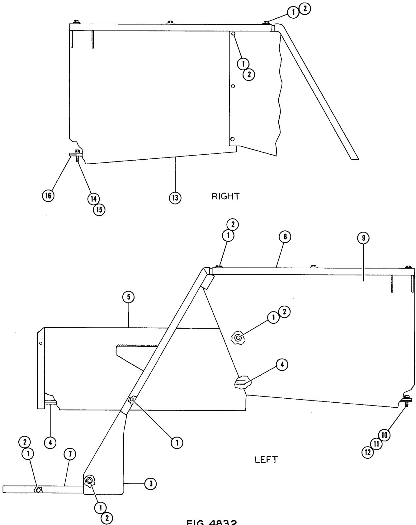
FIG. 4832 FENDERS
