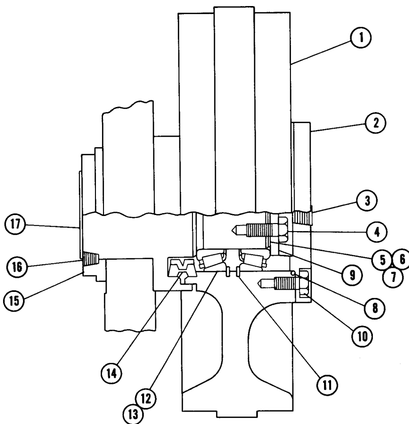
FIG. 6090B ROLLER-TAIL
