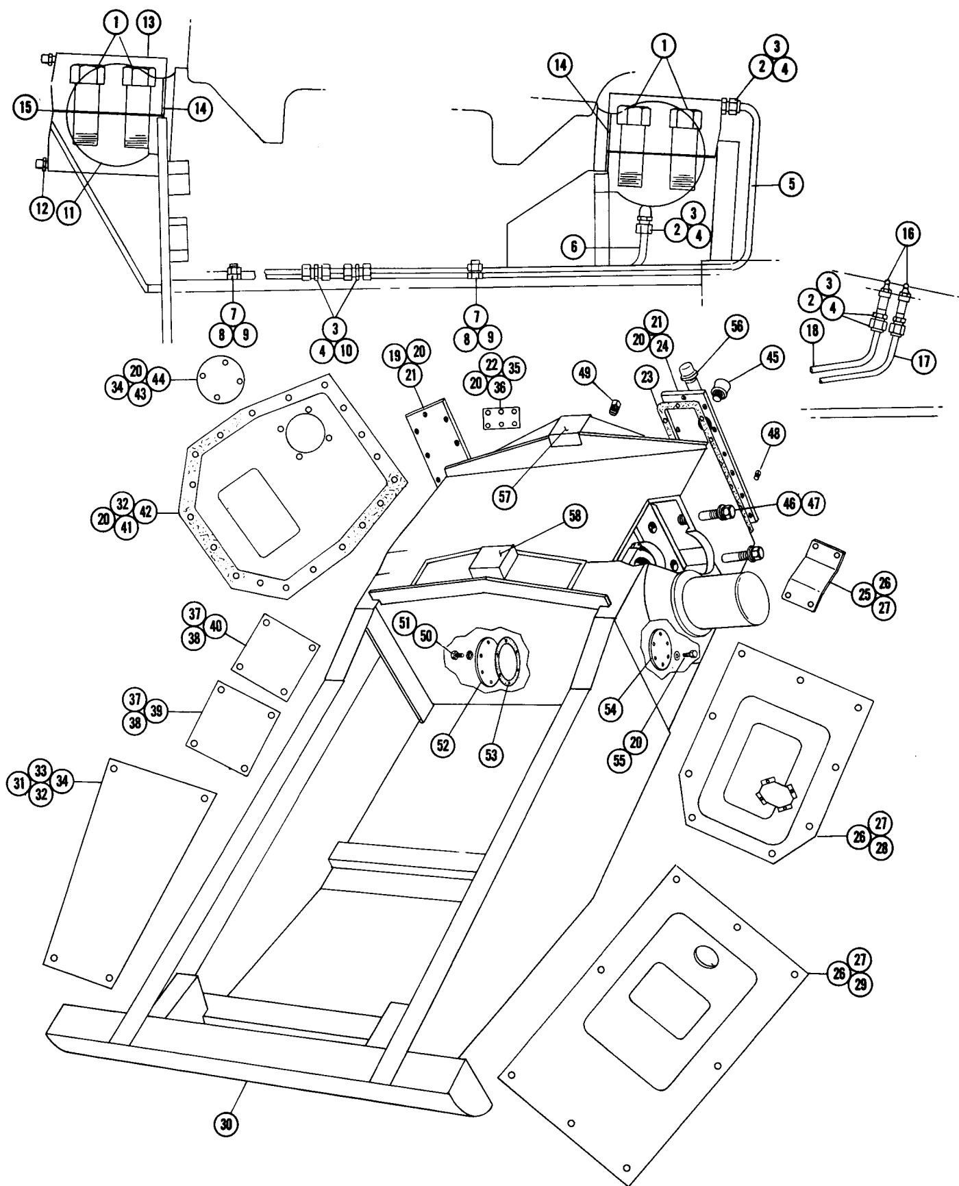
FIG. 7854 MAIN CASE
