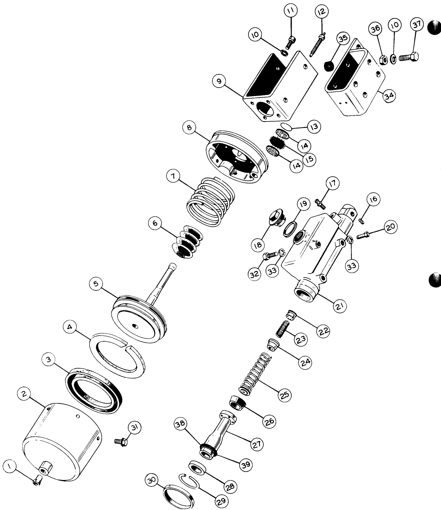
FIG.2644 POWER CLUSTER-BRAKE
