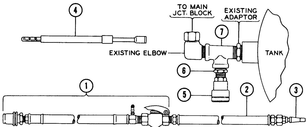
FIG. 740I A TIRE INFLATION KIT
