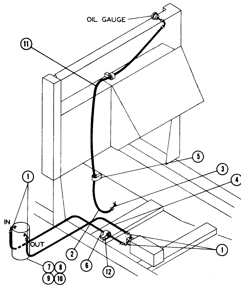
FIG. 8098A ENGINE OIL PIPING
