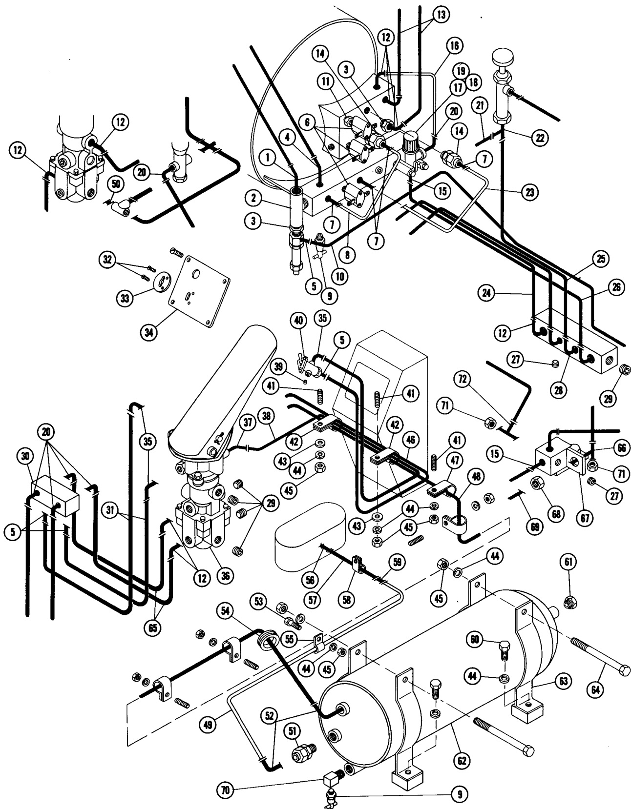
FIG. 7386 EMERGENCY BRAKE
