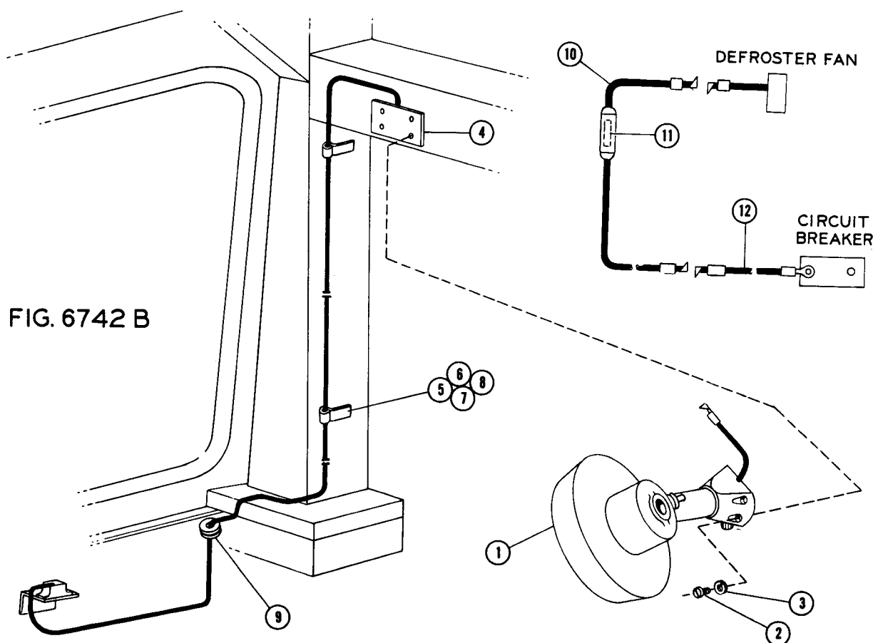
DEFROSTER
