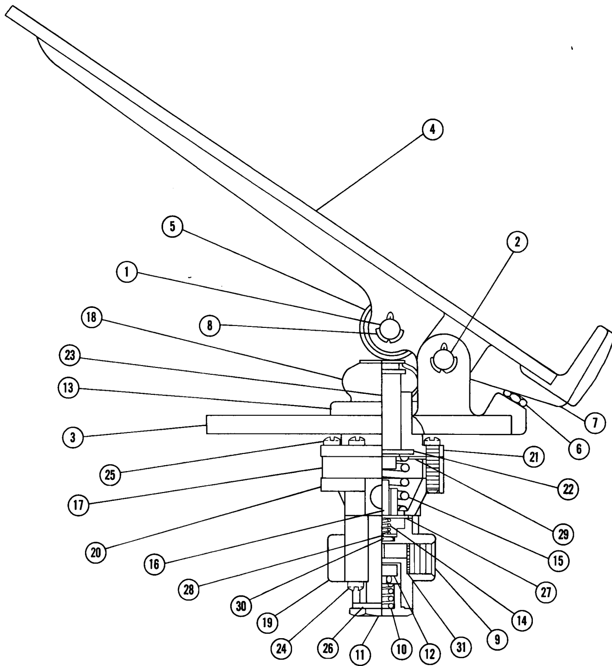
FIG. 6005 TREADLE VALVE
