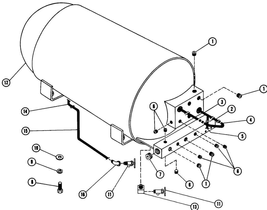
FIG. 7359 A AIR TANK
