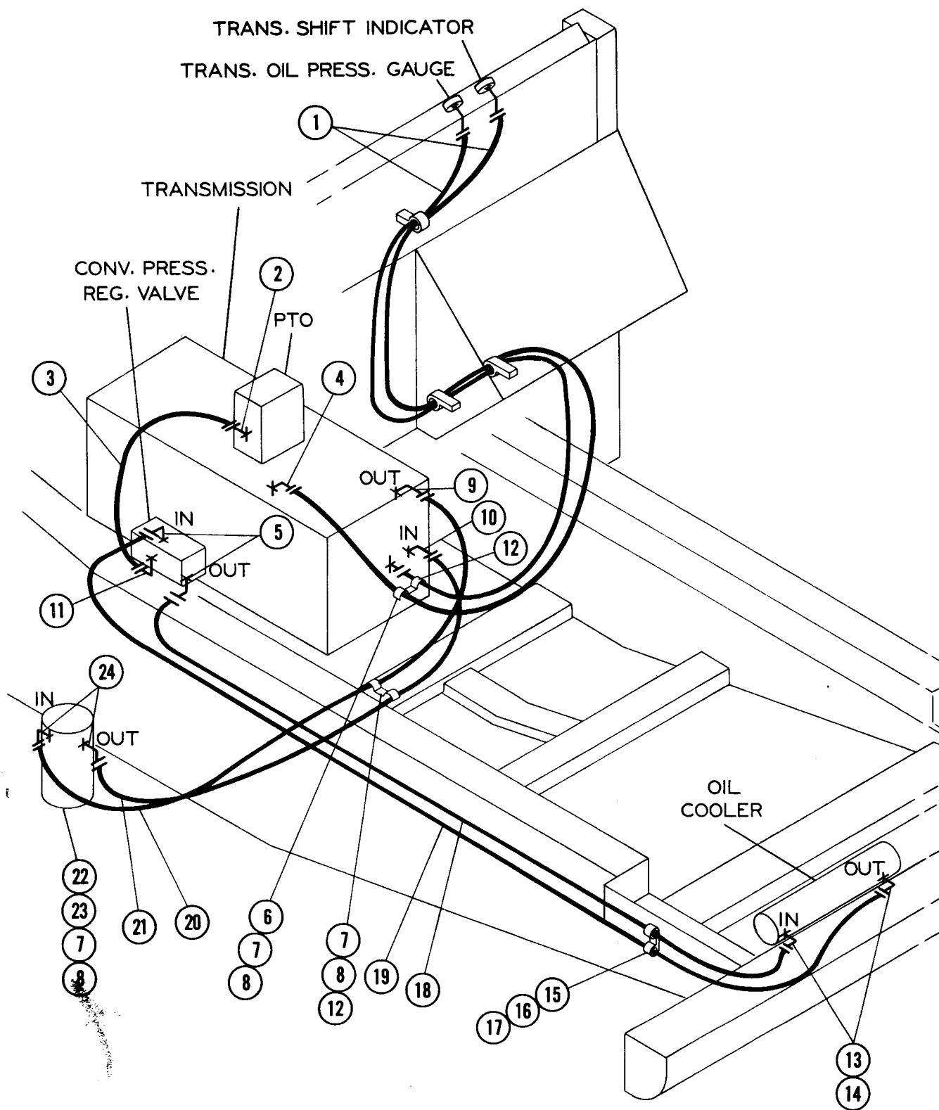
FIG. 5947 PIPING - TRANSMISSION
