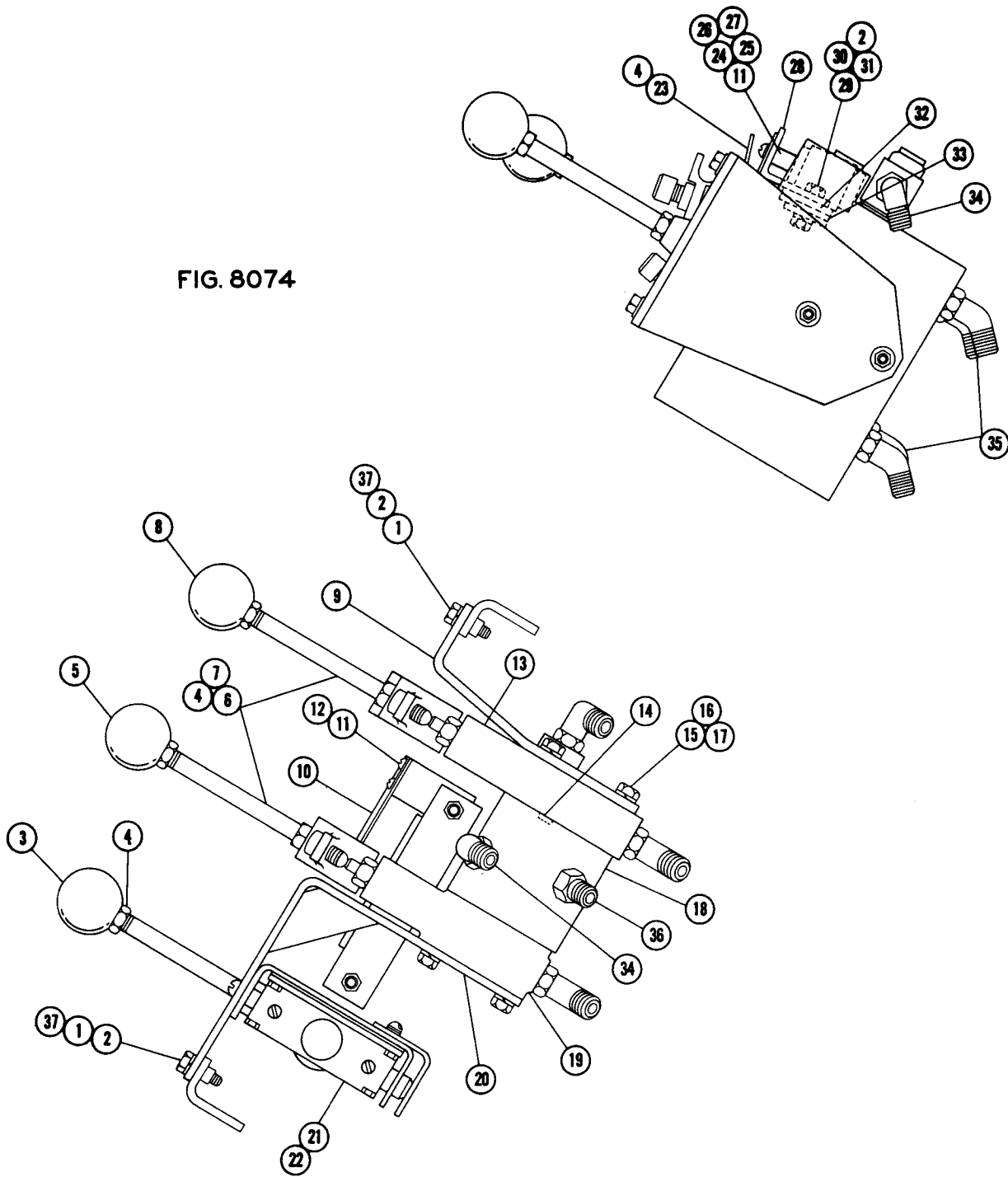
SCRAPER CONTROL PANEL
