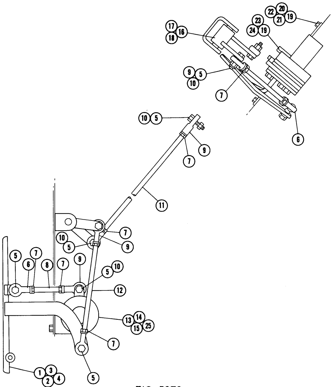
FIG. 5979 LINKAGE-THROTTLE
