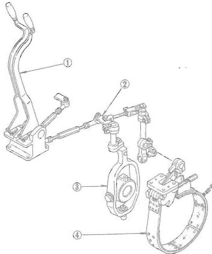
1-Steering clutch lever 3-Shifter yoke 2-Link lever 4-Brake band
