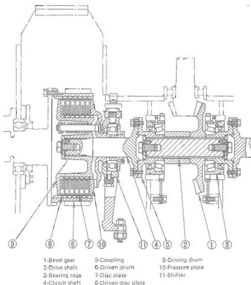
Steering clutch-and-brake — Cross section
