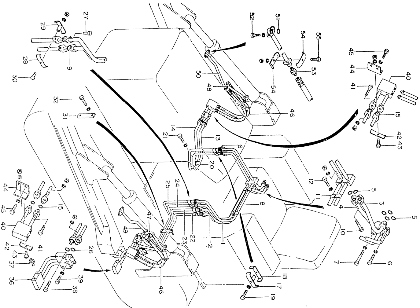
FIG. No. 7-17-2 (リヤ) (Rear)
