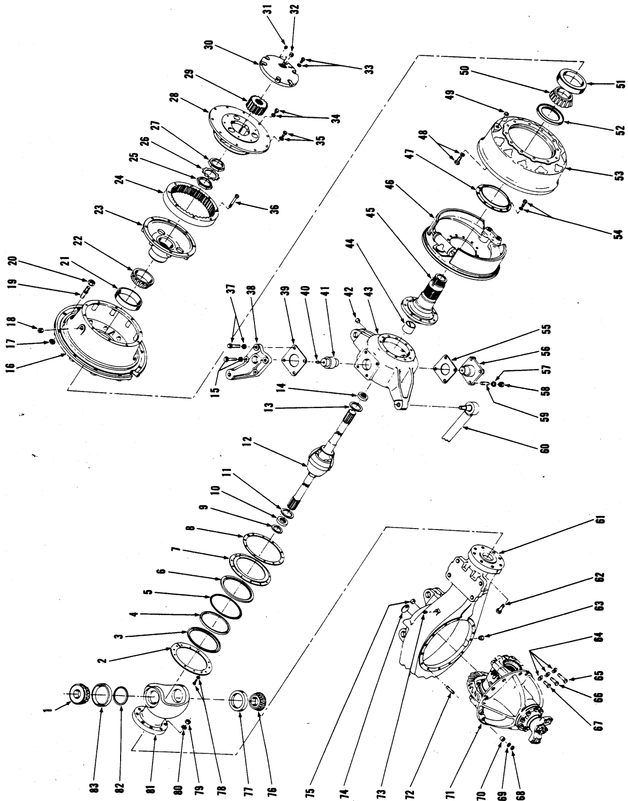
AXLE ASSEMBLY — REAR DRIVE STEER
