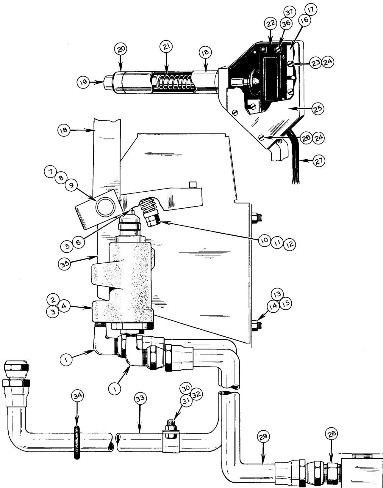
FIG. 1360 SCRAPER HOIST CONTROL
