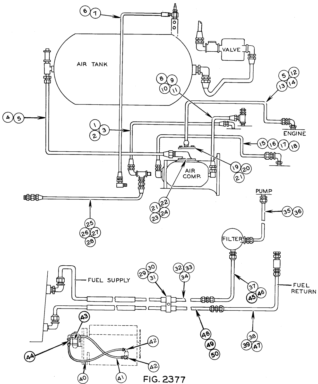
ENGINE PIPING
