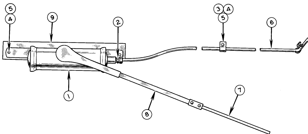
FIG. 2404 B WINDSHIELD WIPER-REAR
