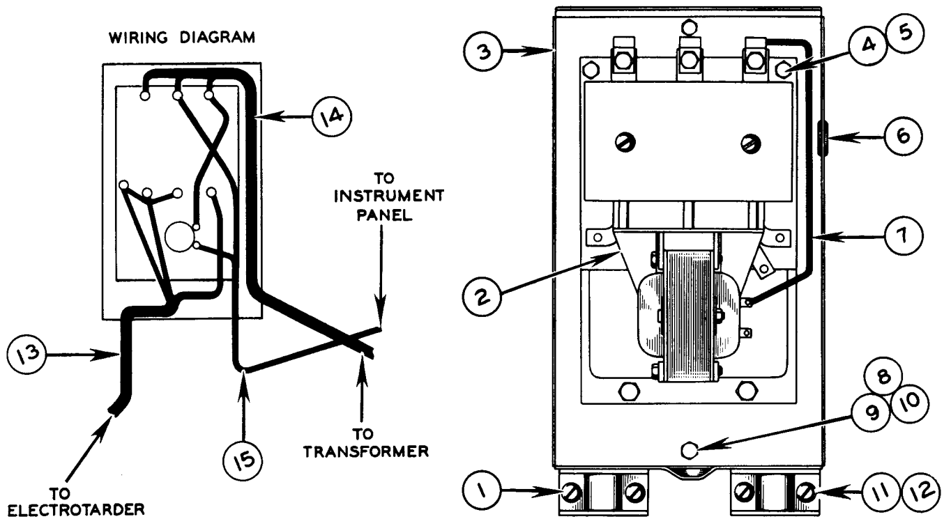
FIG. 1632 B ELECTROTARDER SWITCH BOX
