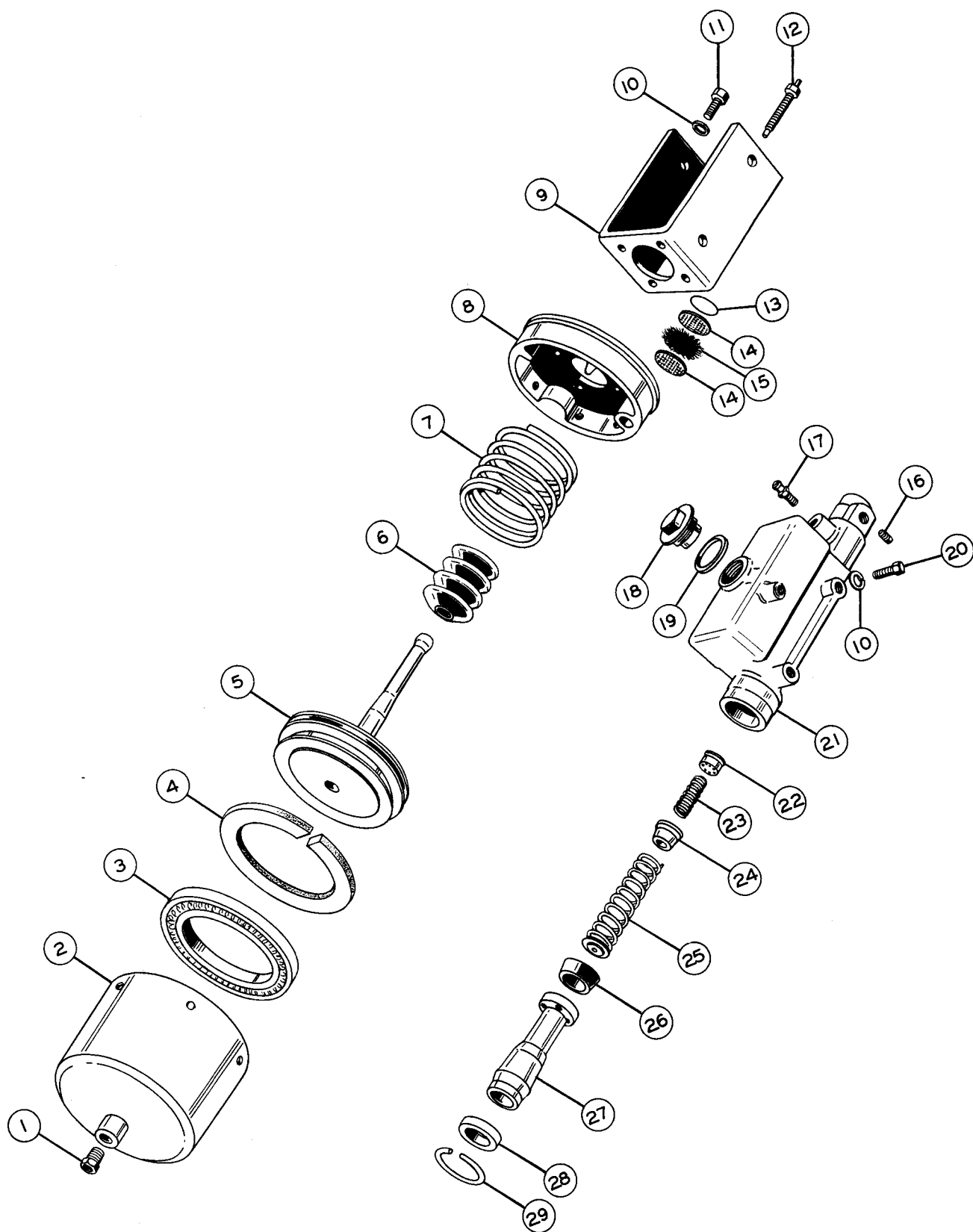
FIG. 2518 BRAKE CYLINDER
