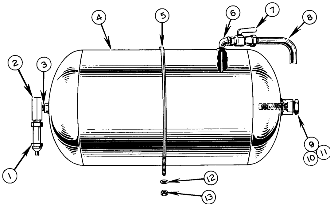
FIG. 1400 B AIR TANK
