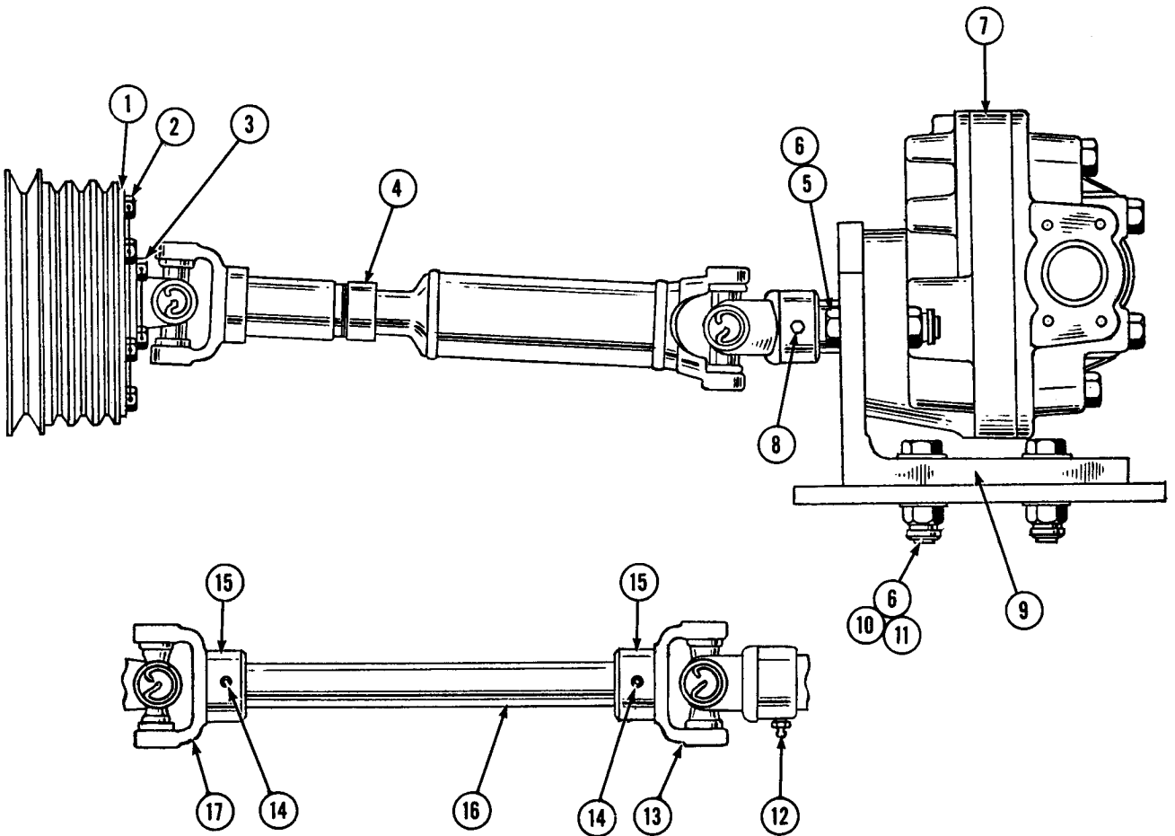
FIG. 3225 B PUMP DRIVE
