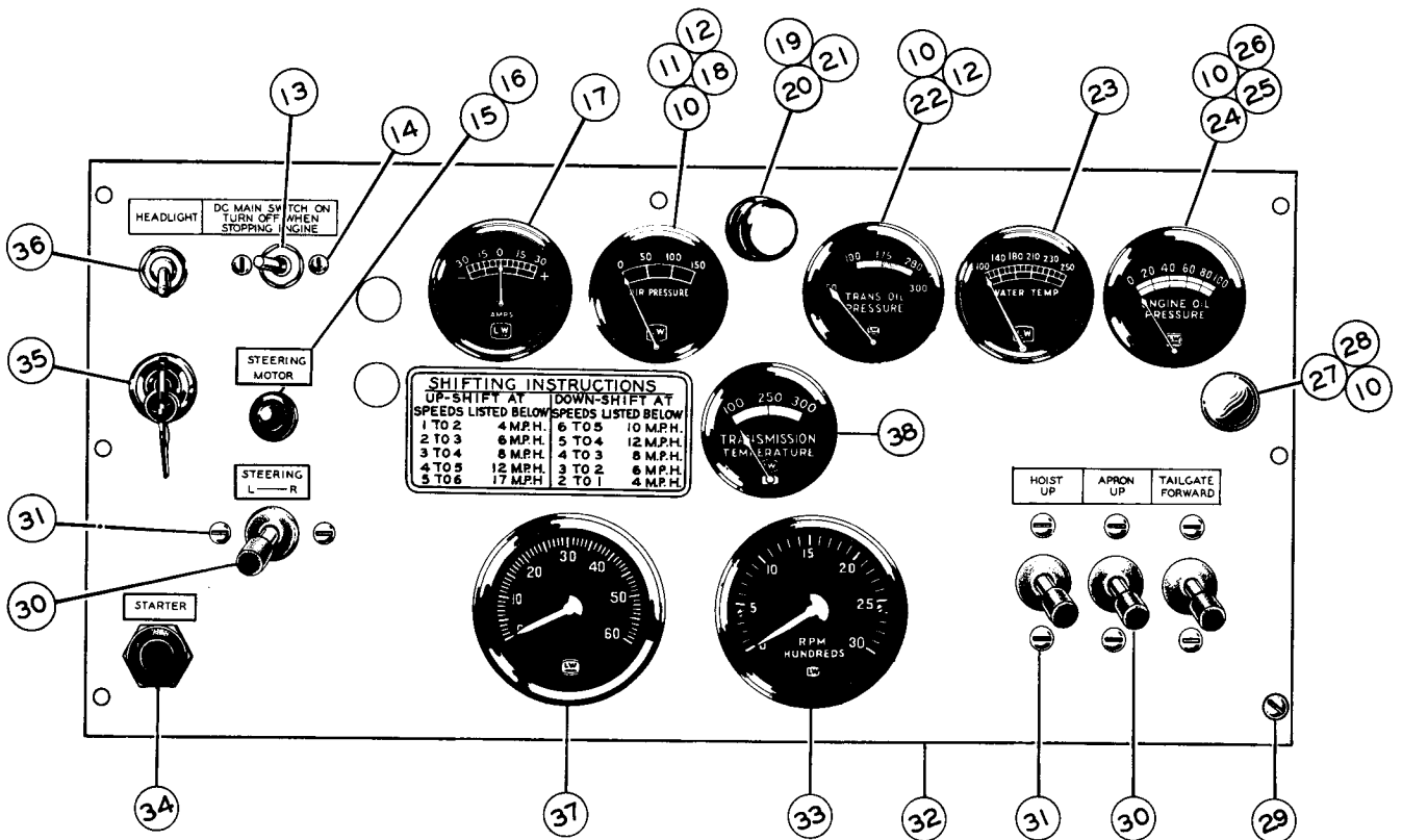
FIG. 2578 INSTRUMENT PANEL
