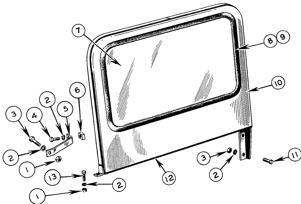
FIG. 2396 A WINDSHIELD
