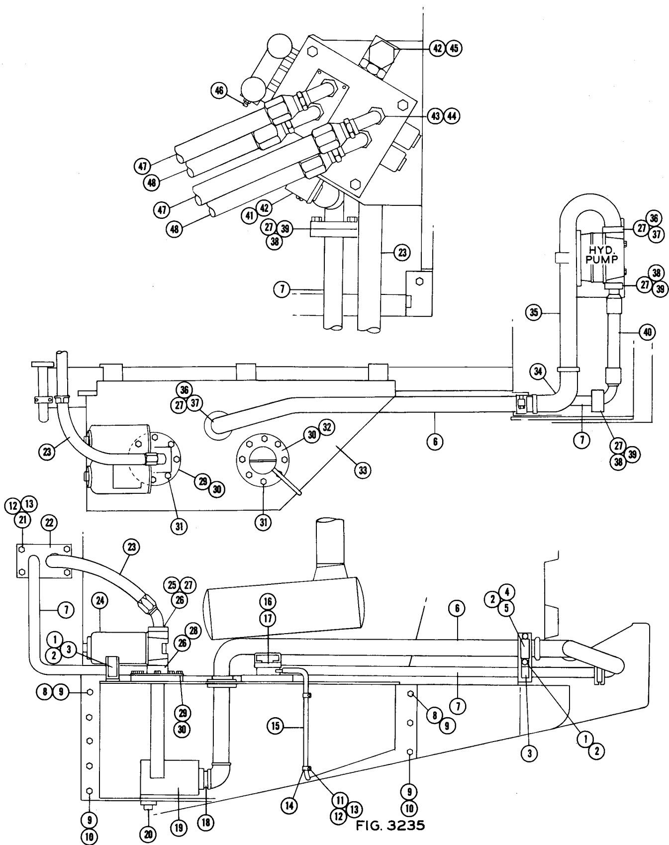
PIPING-SCRAPER CONTROL
