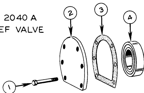
FIG. 2040 B TRANSMISSION PUMP ADAPTOR
