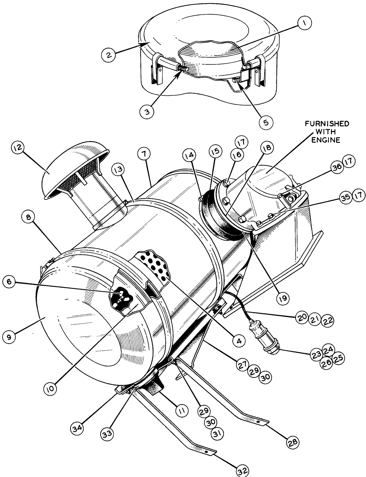
FIG. 2387 AIR CLEANER
