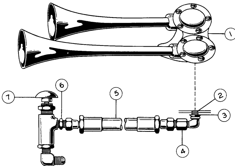
FIG. 2400 C AIR HORN
