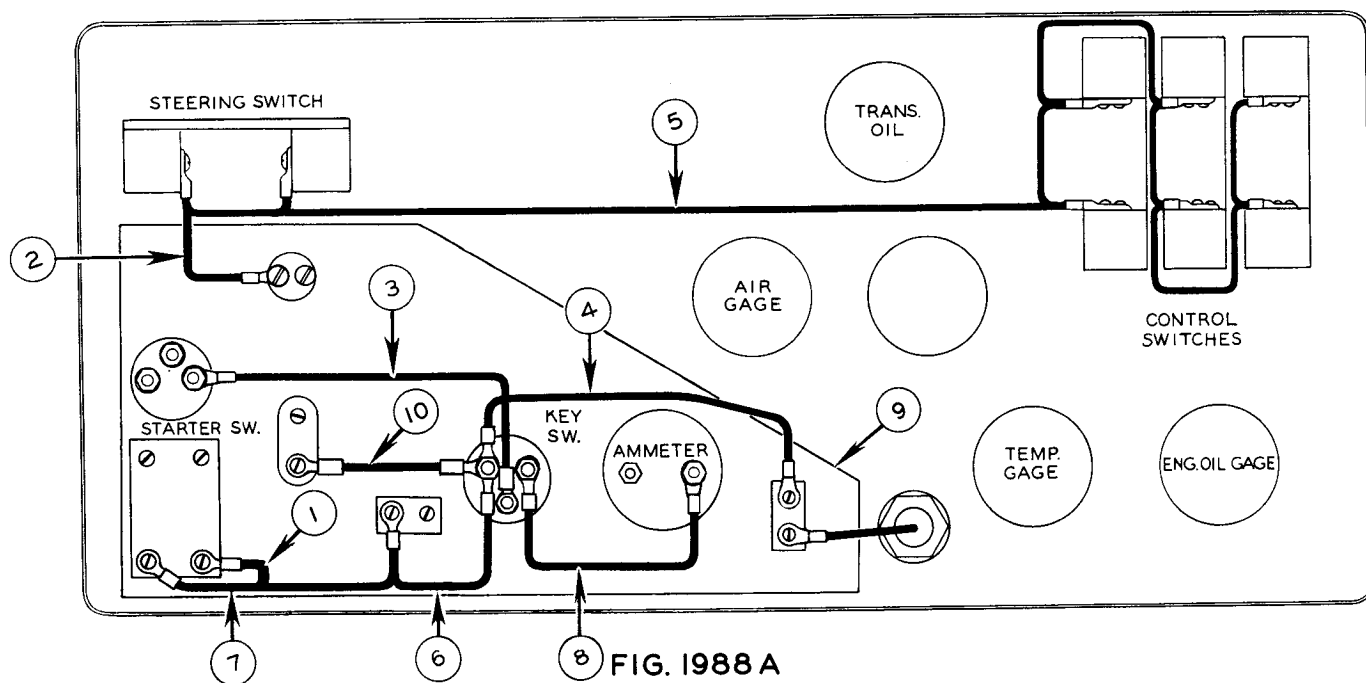
WIRING-INSTRUMENT PANEL
