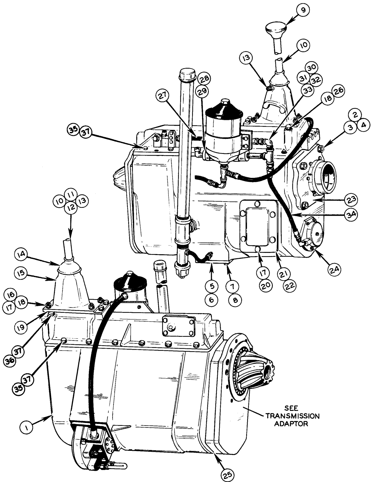
FIG. 1628 TRANSMISSION MISCELLANEOUS
