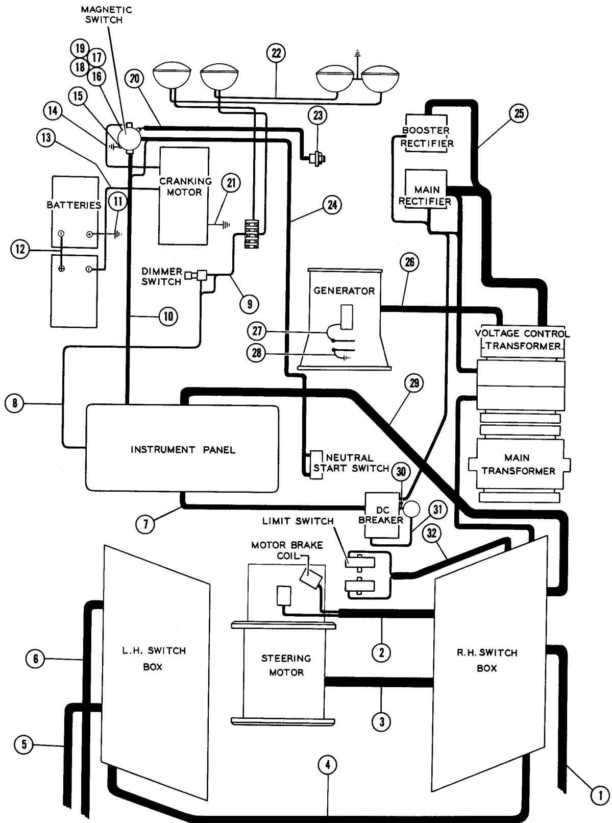
FIG.3223 WIRING- GENERAL
