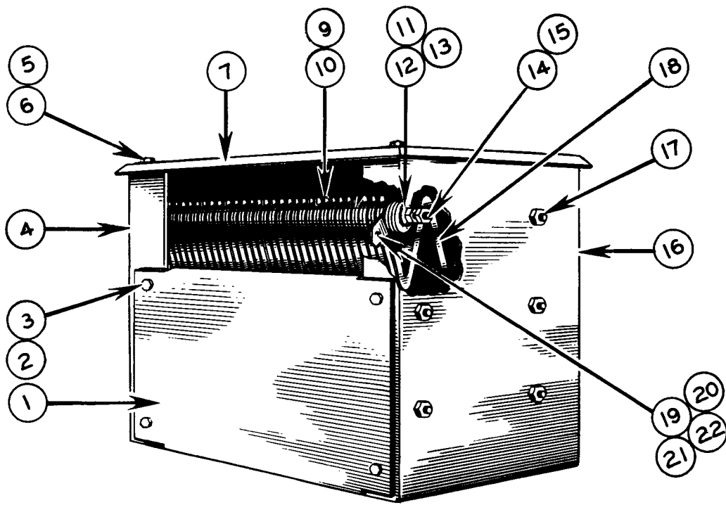
FIG. 1632 A ELECTROTARDER
