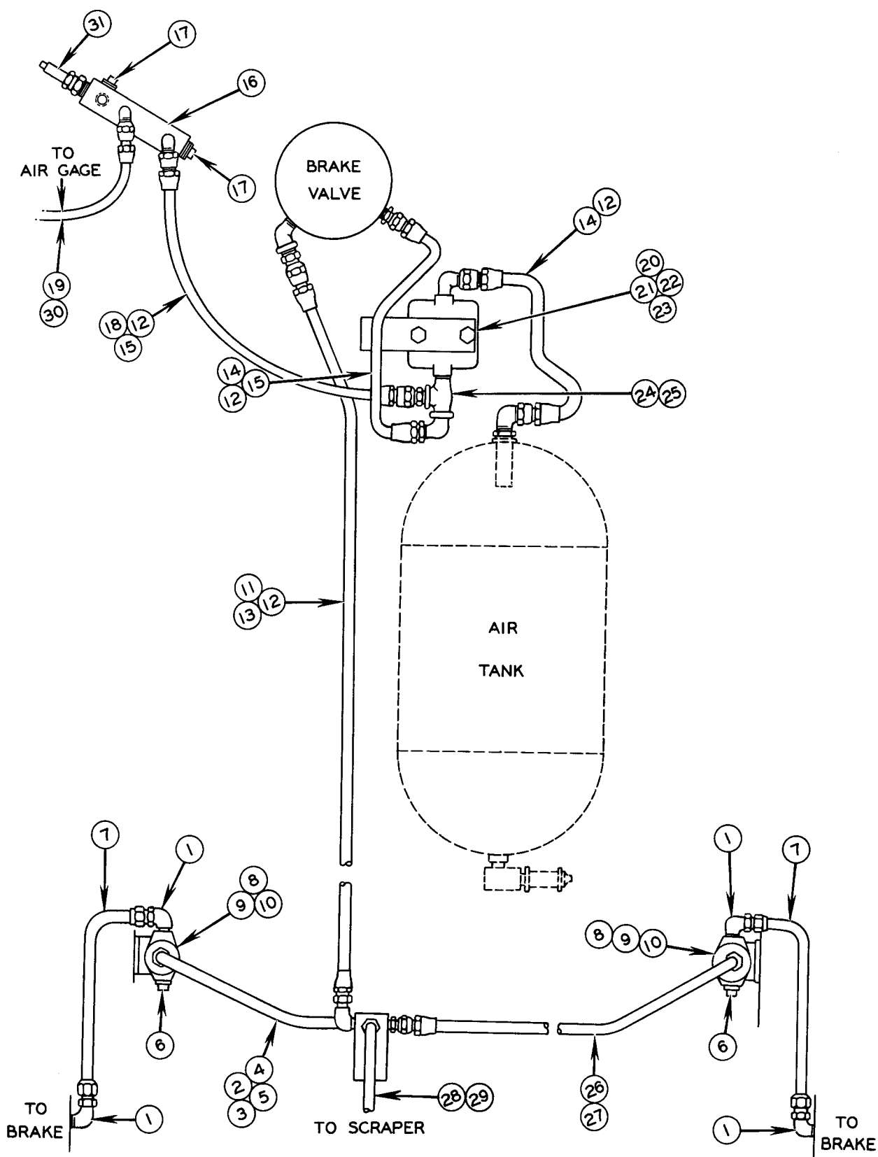
FIG. 1629 BRAKE SYSTEM PIPING
