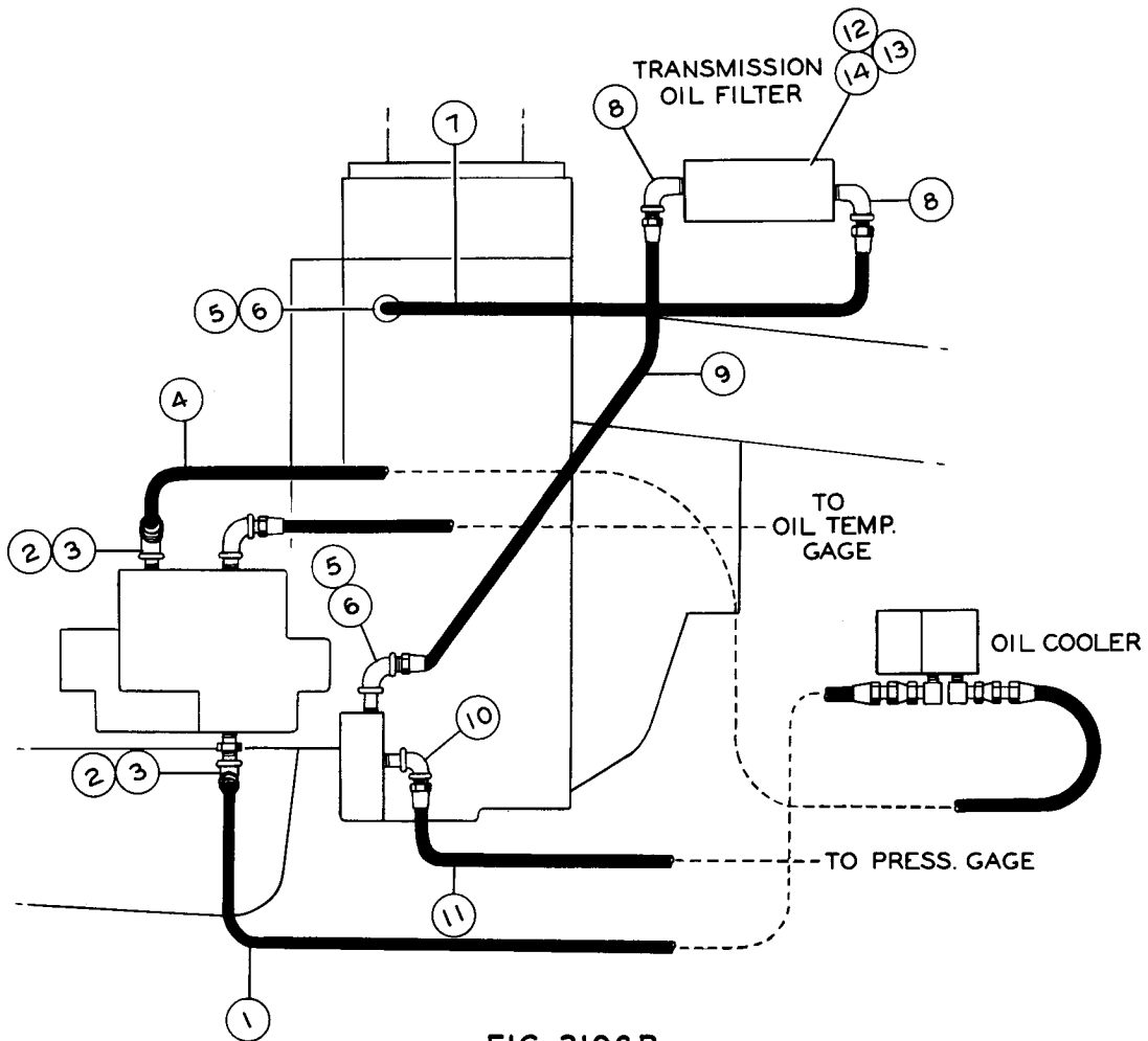
PIPING-ALLISON TRANSMISSION
