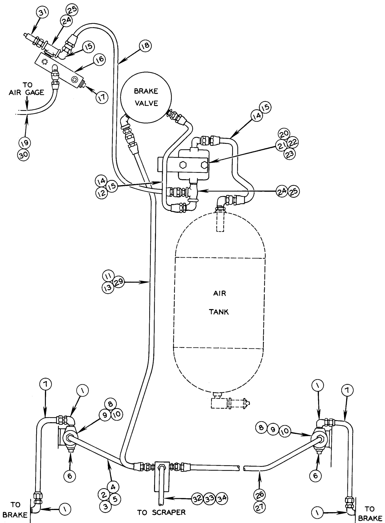
FIG. 1997 BRAKE SYSTEM PIPING
