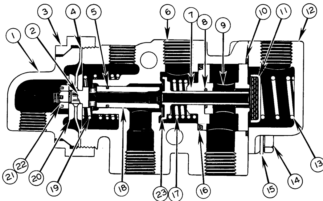
FIG. 1690 B TRACTOR PROTECTION VALVE
