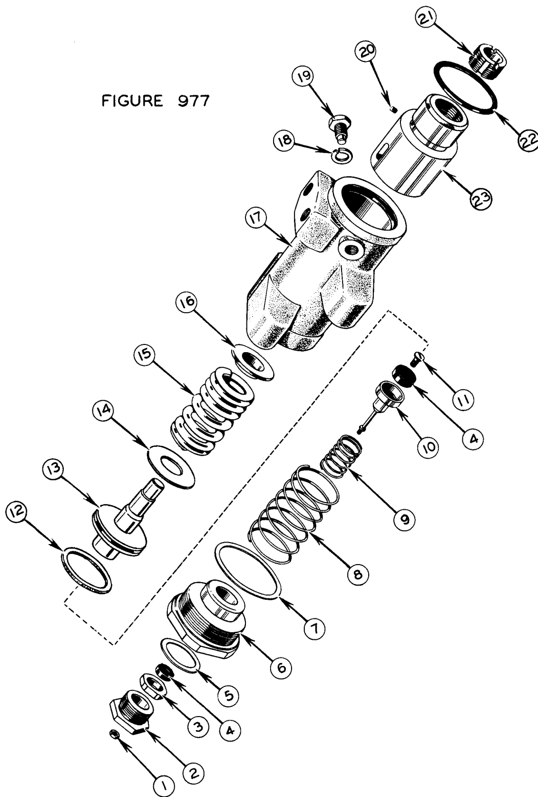
AIR VALVE
