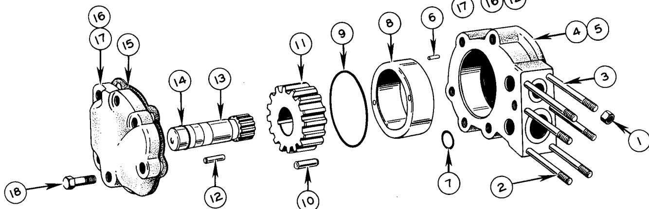
FIG. 2040 C TRANSMISSION PUMP
