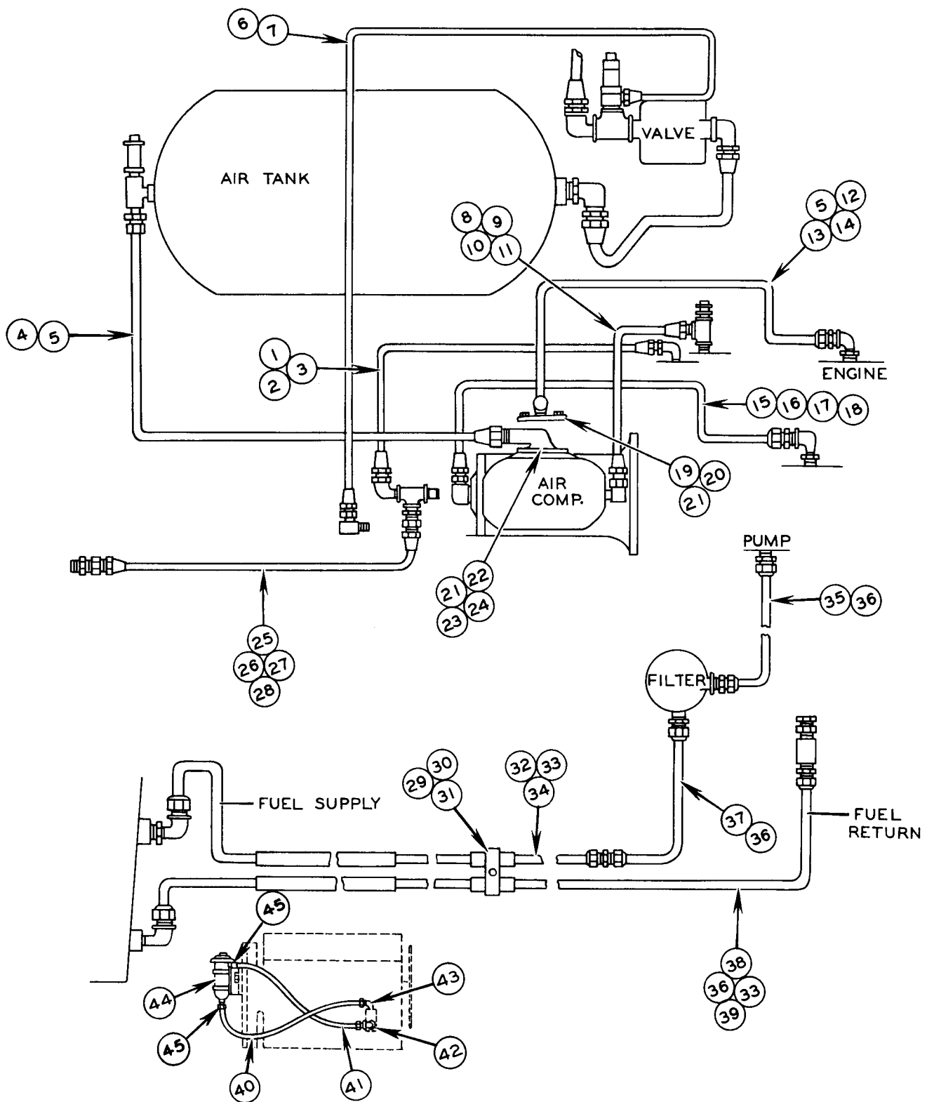
FIG. 1686 ENGINE PIPING
