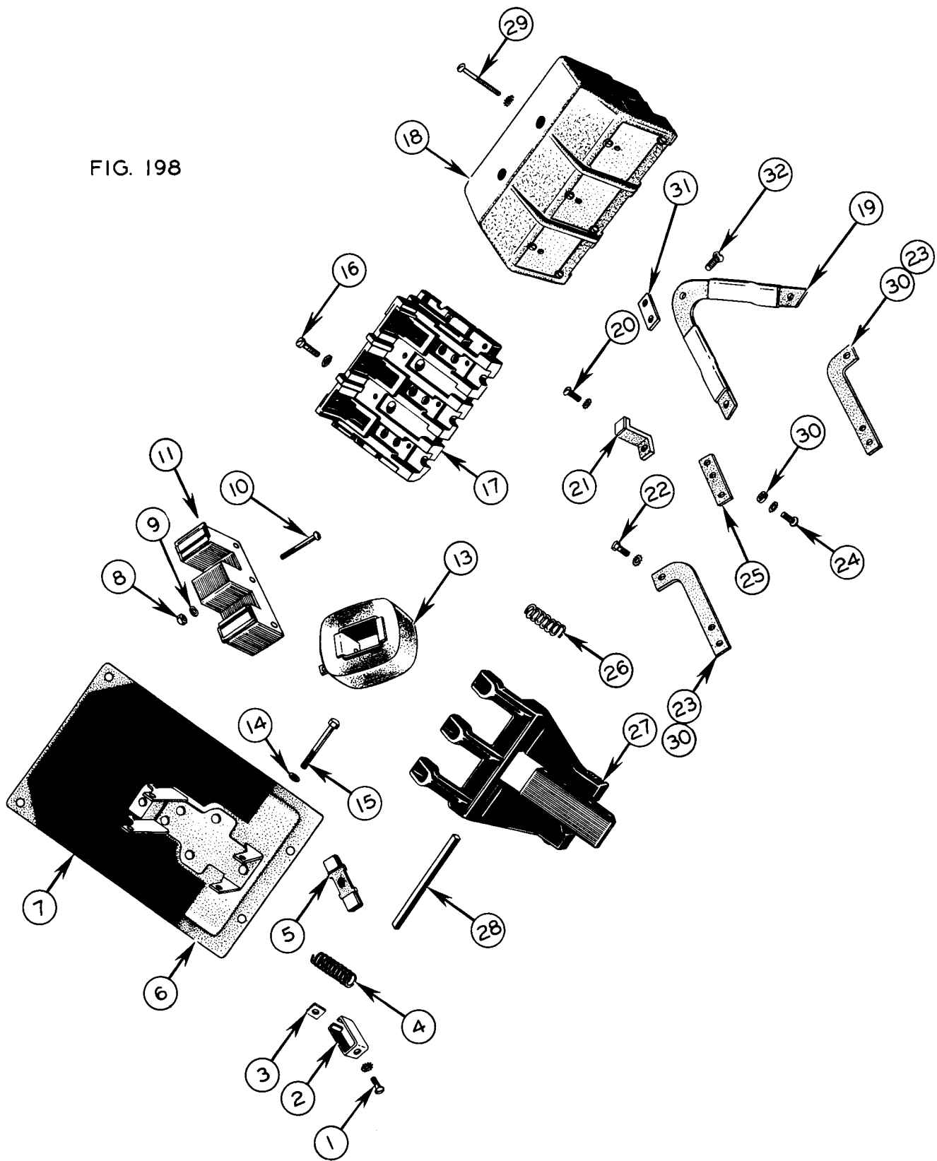
CONTACTOR
