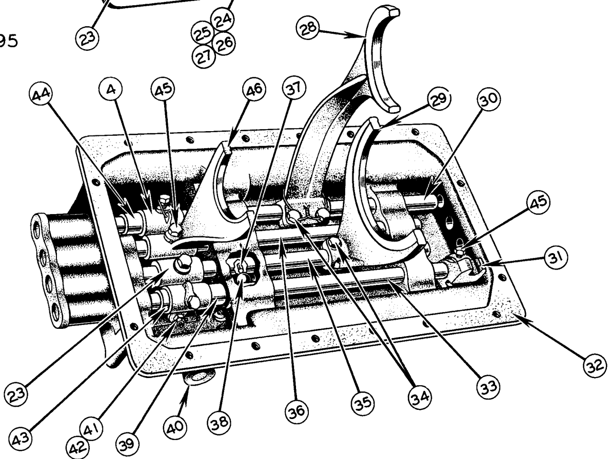
SHIFT BAR HOUSING
