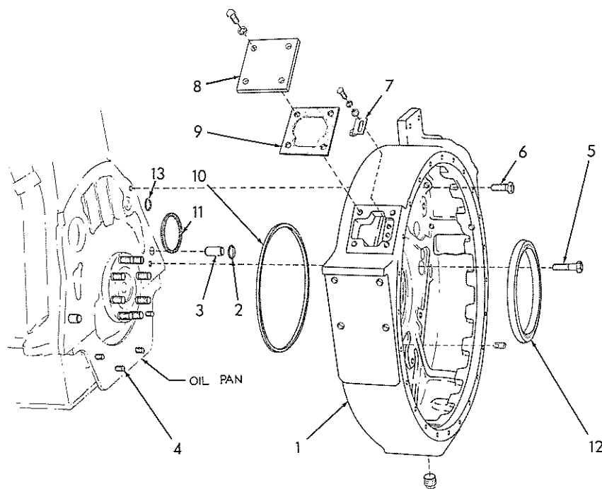
FLYWHEEL HOUSING
