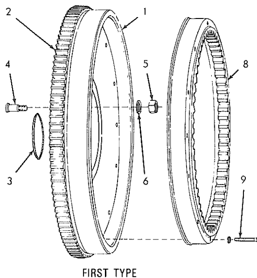
FLYWHEEL
