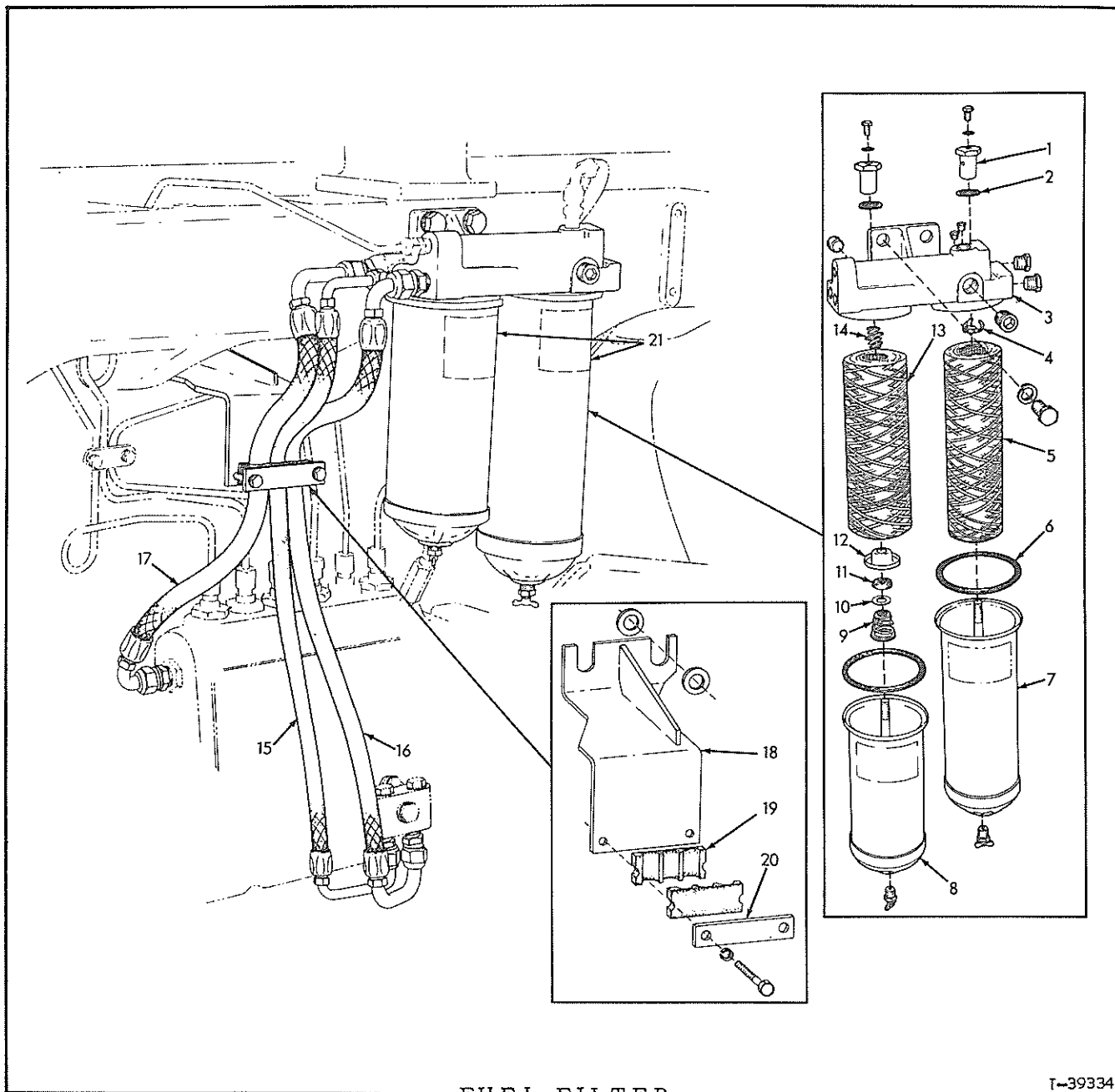
FUEL FILTER
