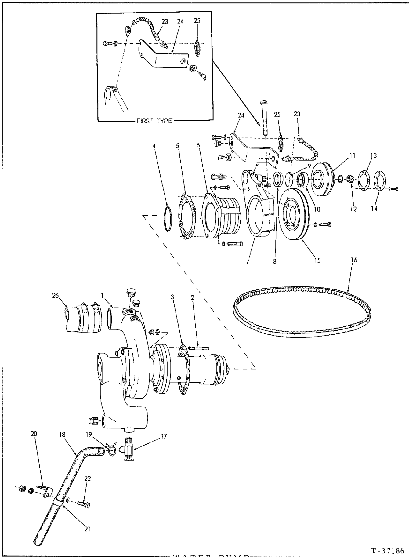
WATER PUMP
