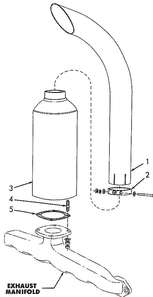
EXHAUST PIPE
