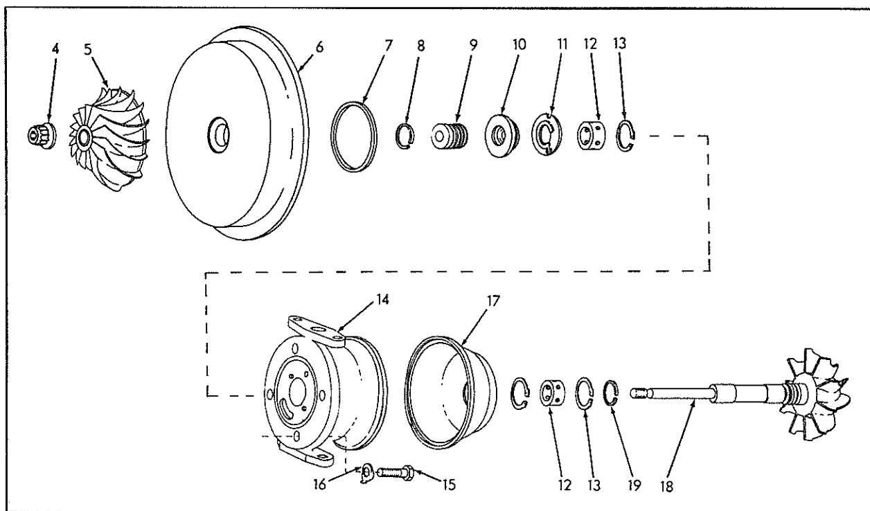
TURBOCHARGER ASSEMBLY
