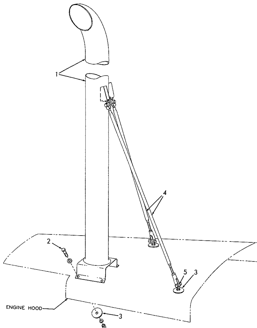
EXHAUST EXTENSION
