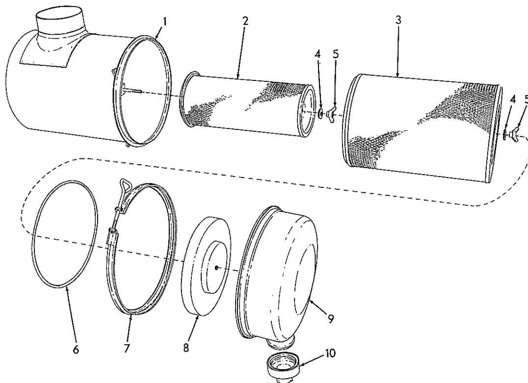
AIR CLEANER
