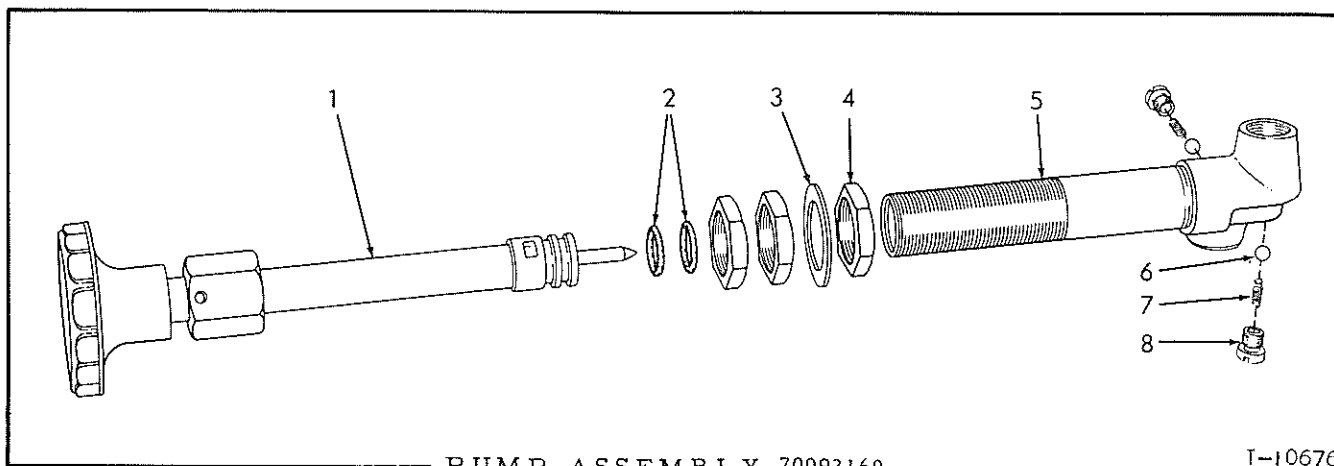
PUMP ASSEMBLY 70092160
