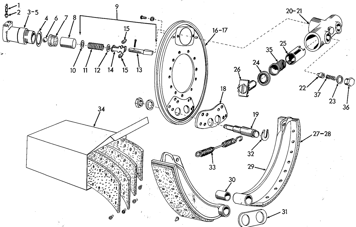
BRAKE ASSEMBLY (Rear Axle)
