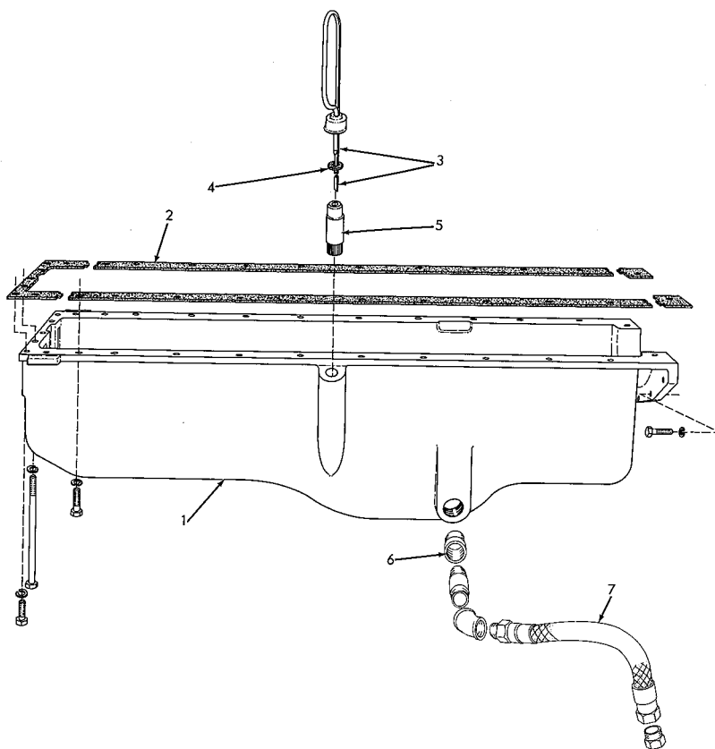
OIL PAN
