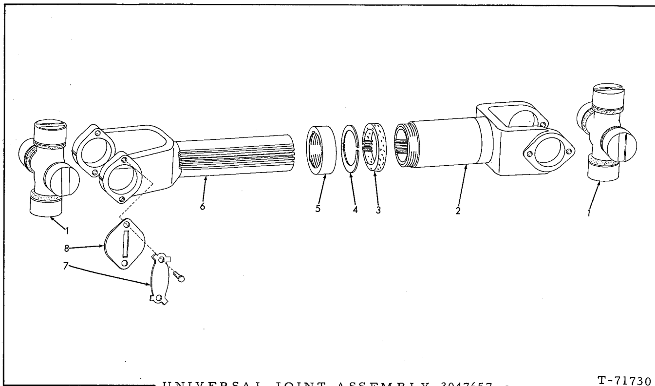
UNIVERSAL JOINT ASSEMBLY 3047657
