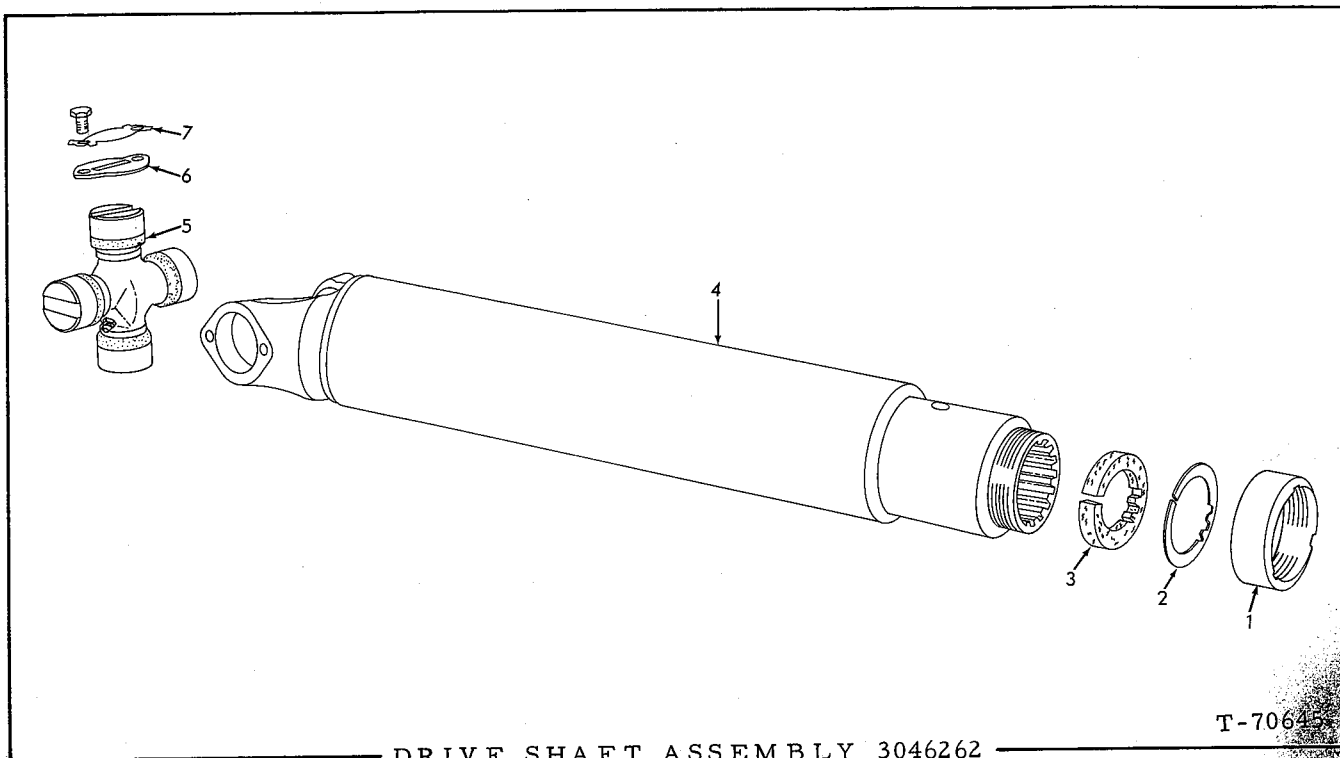
DRIVE SHAFT ASSEMBLY 3046262
