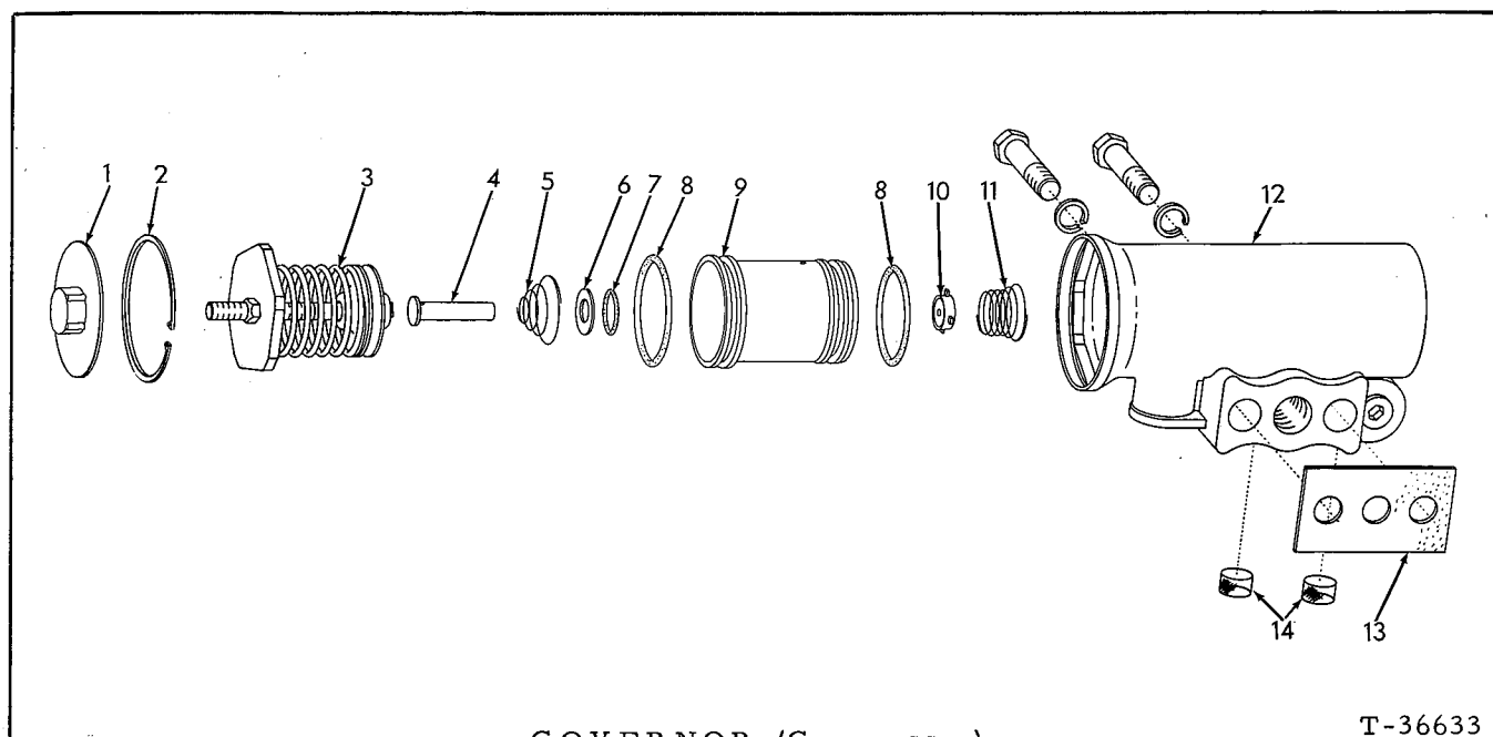
GOVERNOR (Compressor)
