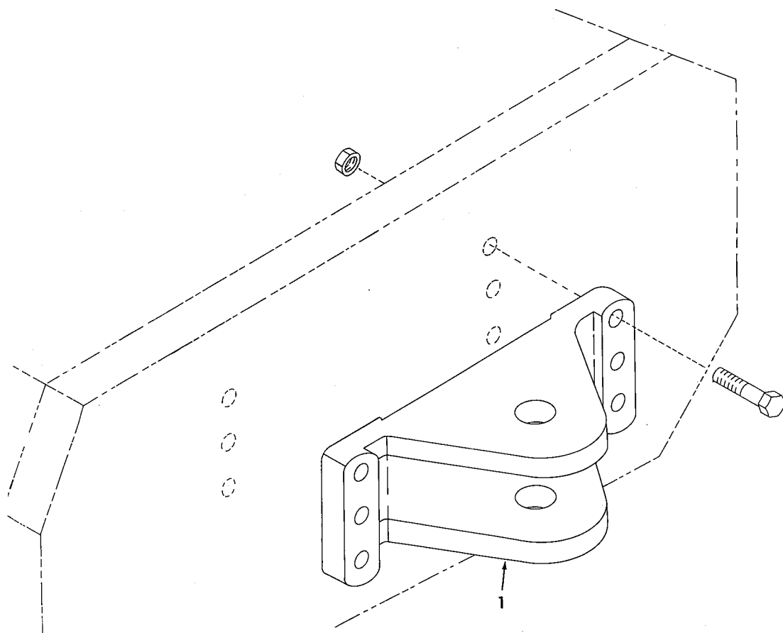
DRAWBAR
