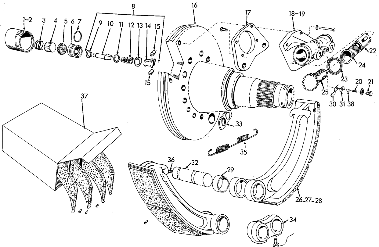
BRAKE ASSEMBLY (Front Axle) 130
