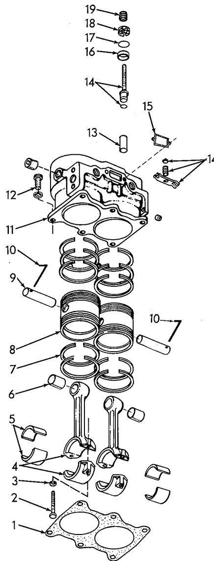
COMPRESSOR CYLINDER BLOCK
