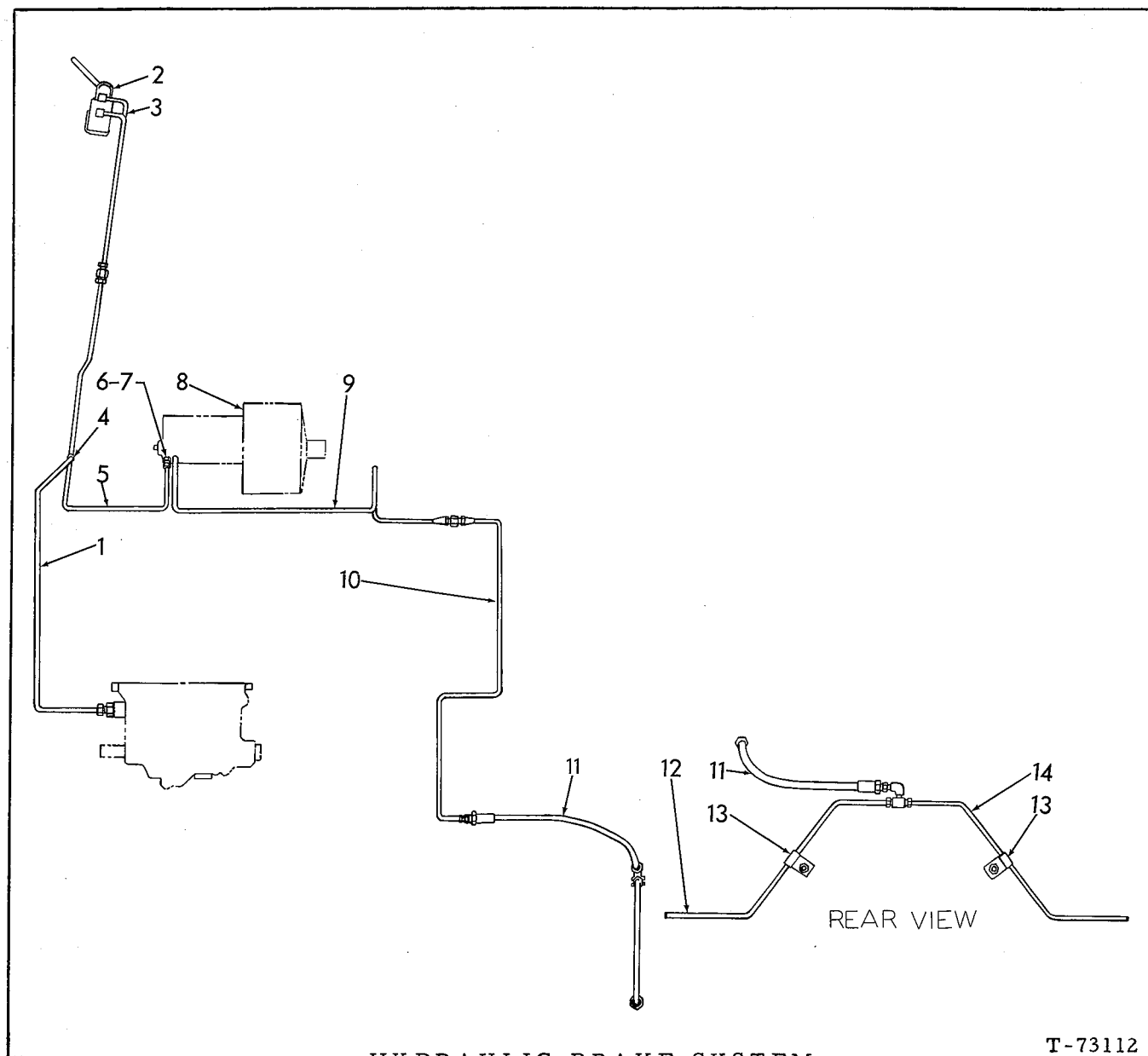
HYDRAULIC BRAKE SYSTEM (Rear Axle)
