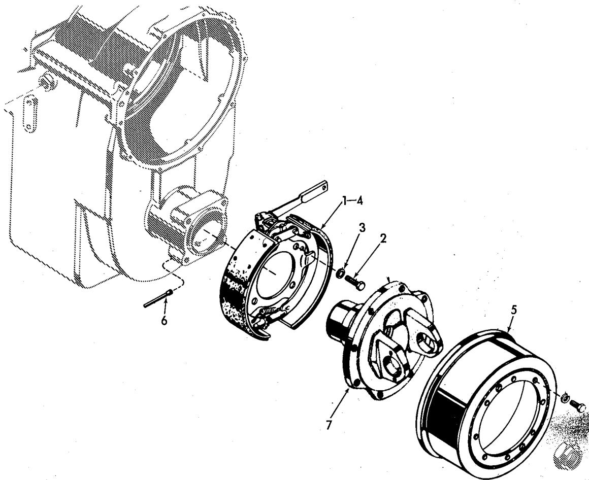
PARKING BRAKE ASSEMBLY
