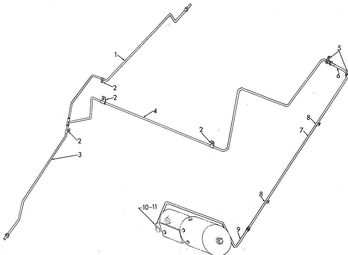
HYDRAULIC BRAKE LINES (Front Section)
