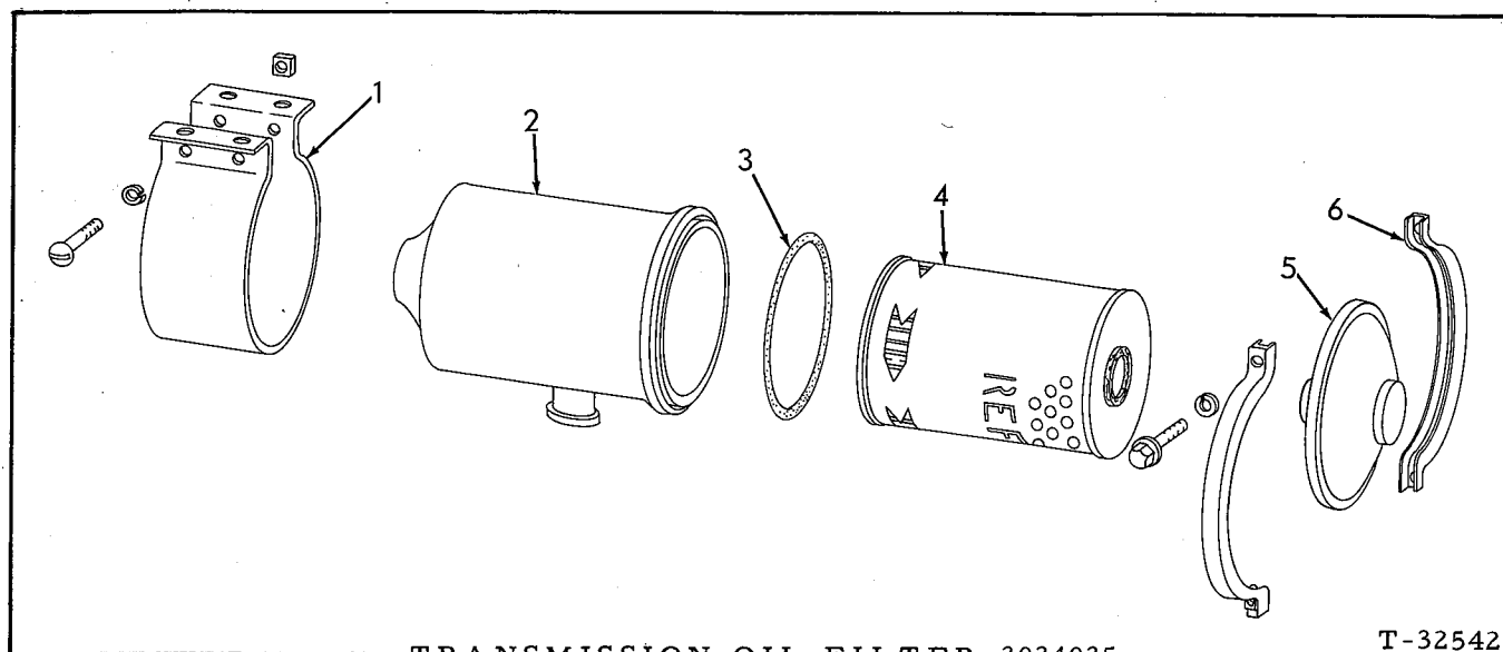
TRANSMISSION OIL FILTER 3034035
