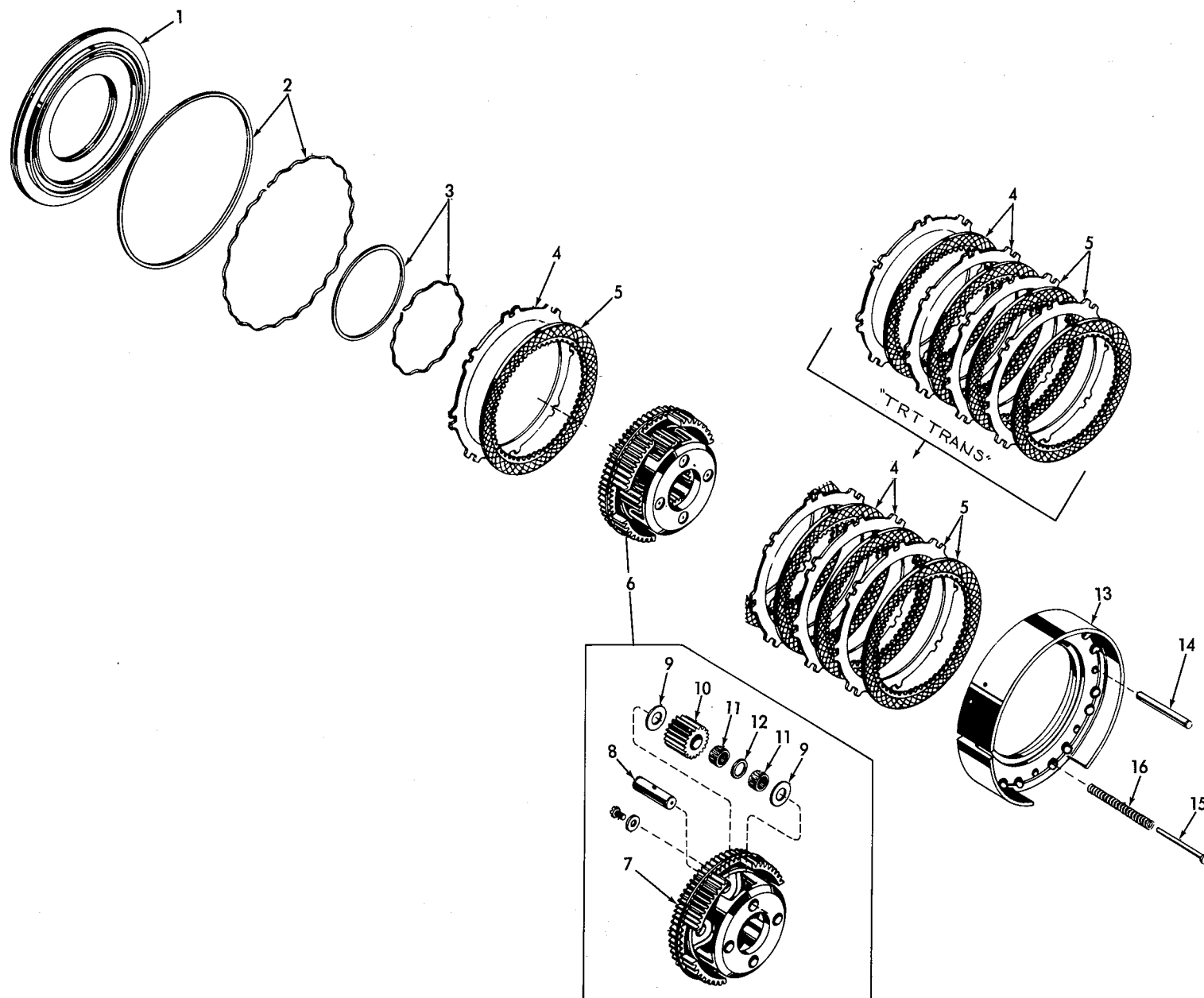
REVERSE CLUTCH AND PLANETARY
