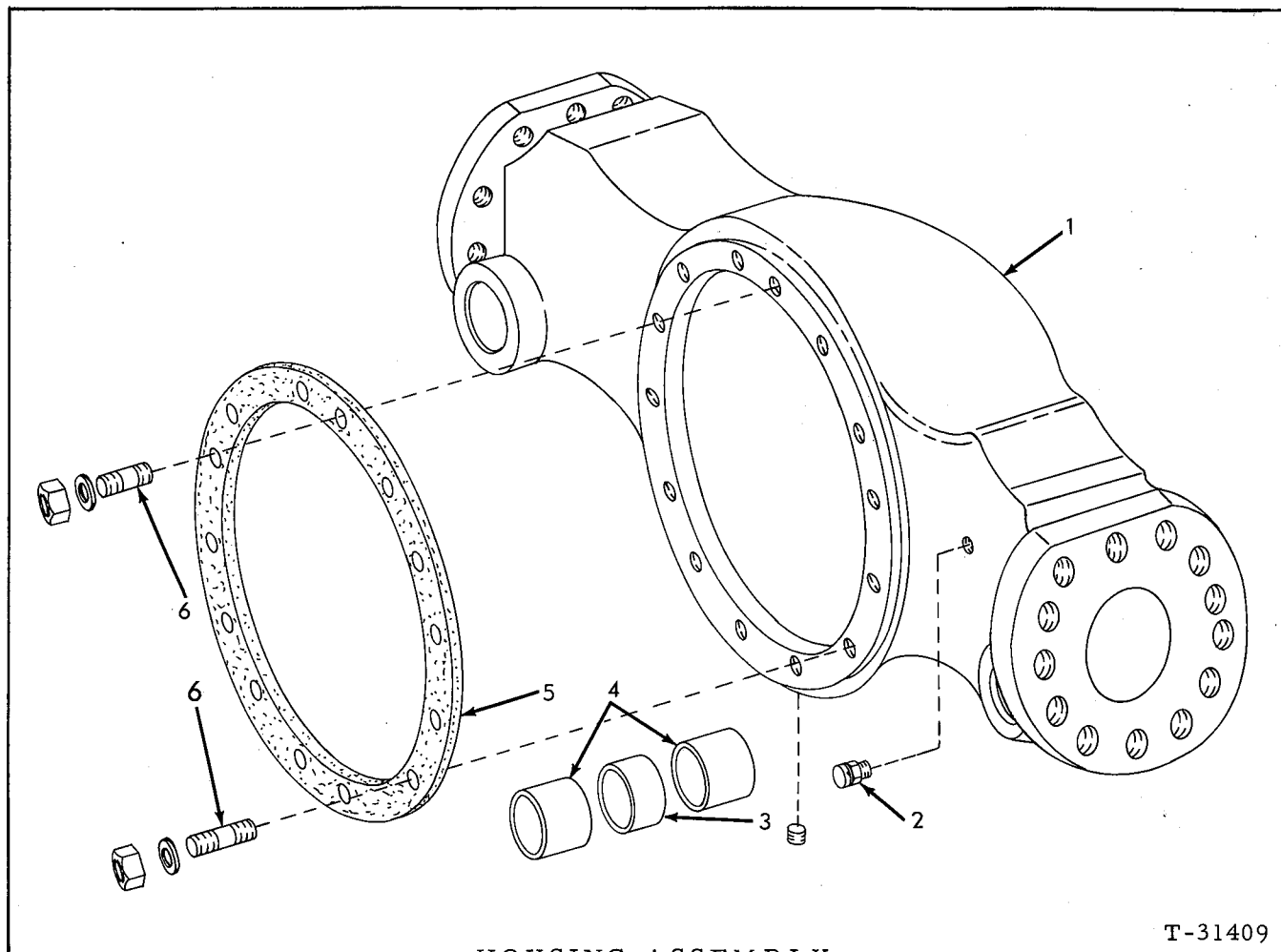
HOUSING ASSEMBLY (Rear Axle)
