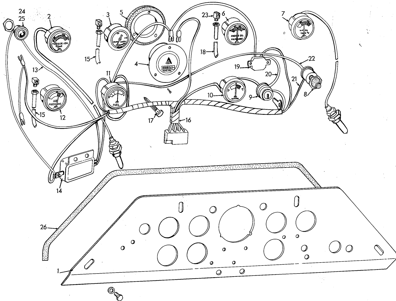
INSTRUMENT PANEL AND GAUGES
