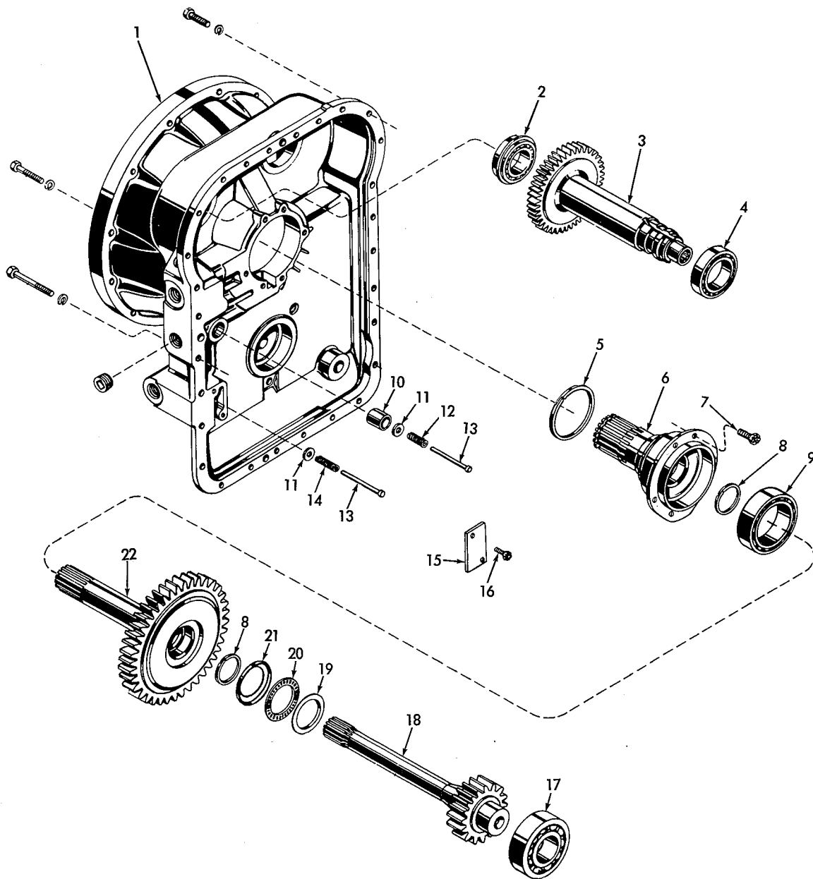
TORQUE CONVERTER HOUSING
