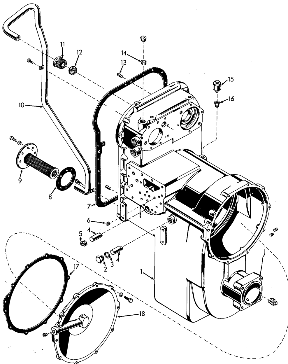
TRANSMISSION HOUSING AND COVER
