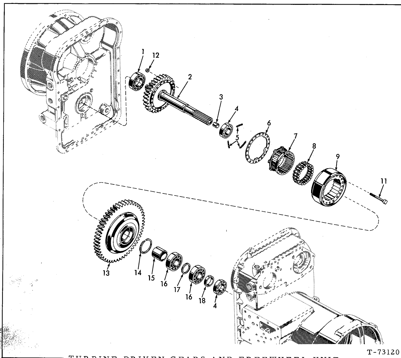
TURBINE DRIVEN GEARS AND FREEWHEEL UNIT
