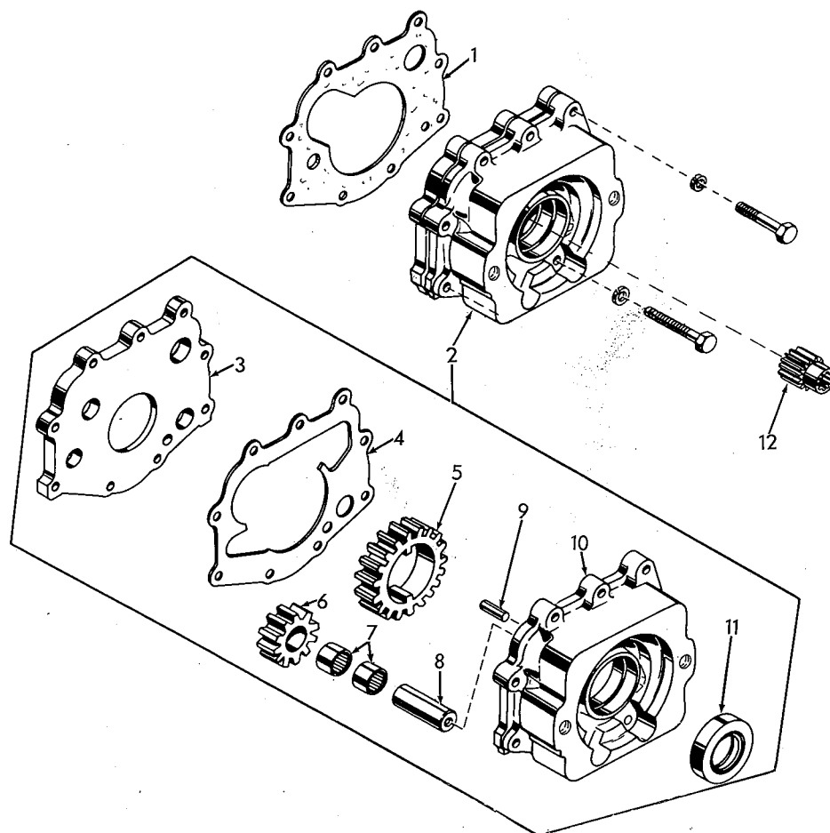
CHARGING OIL PUMP
