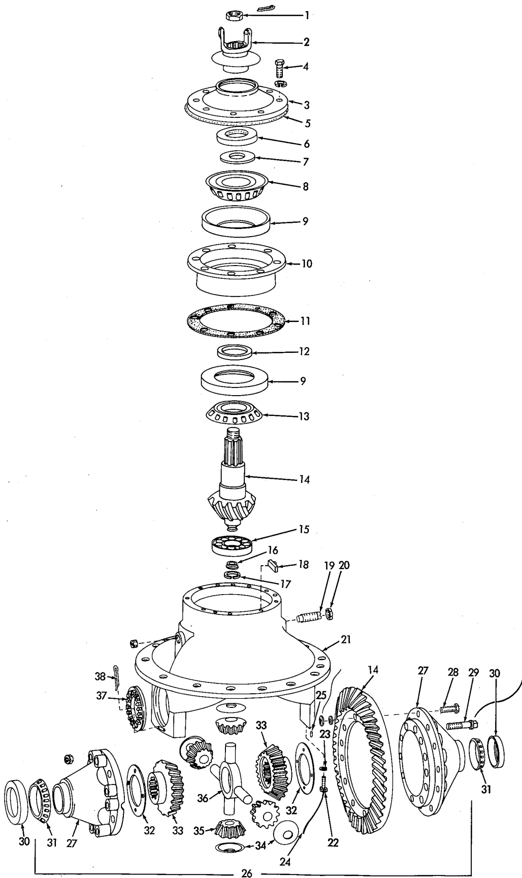
DIFFERENTIAL CARRIER ASSEMBLY 3047867 (Front Axle)
