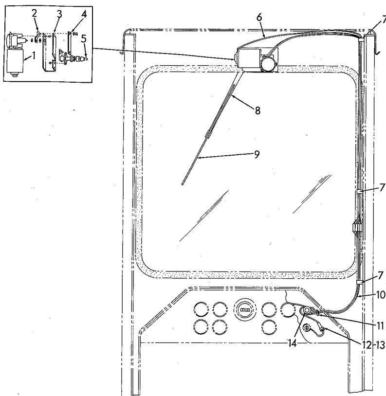
WIPER GROUP
