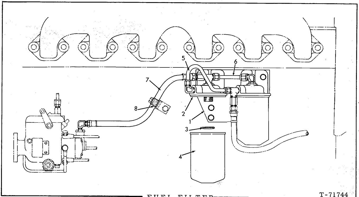
FUEL FILTER
