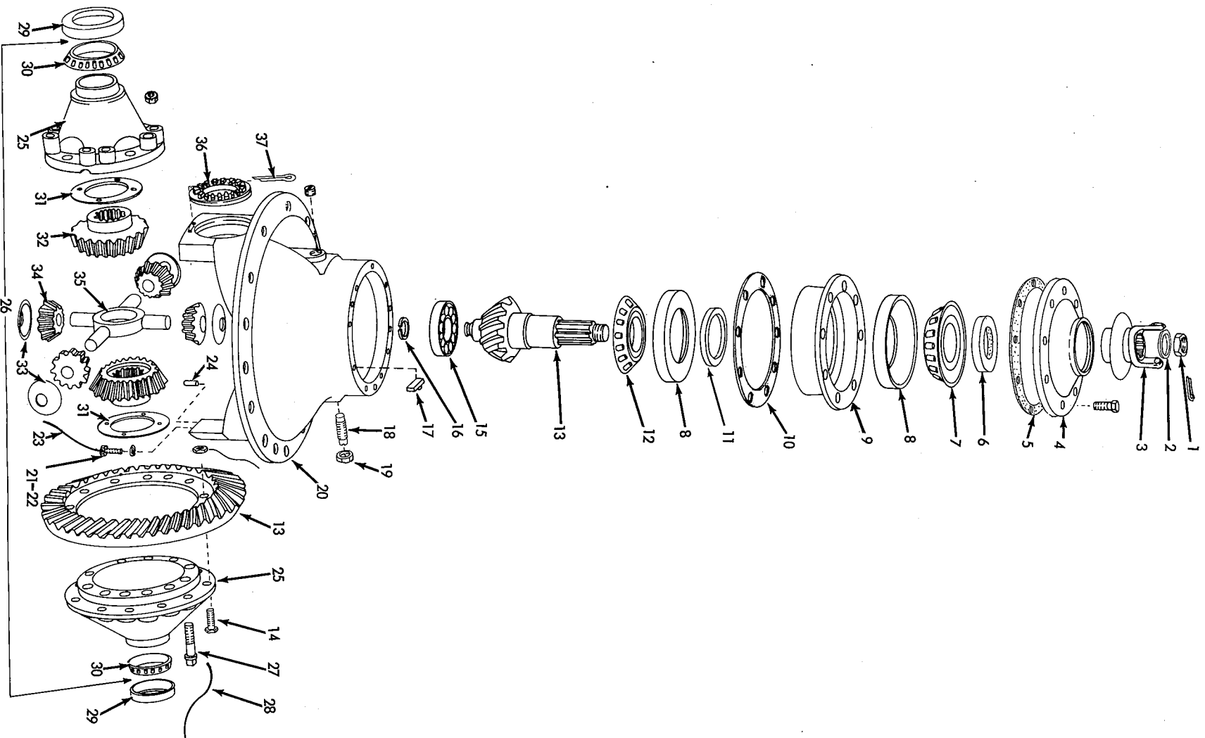
DIFFERENTIAL CARRIER ASSEMBLY 3048428
