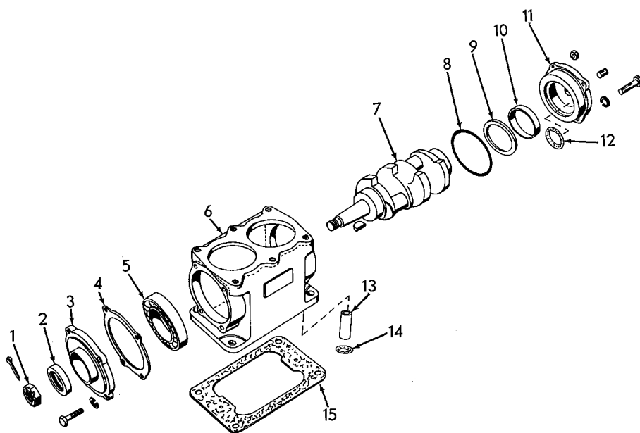
COMPRESSOR CRANKCASE
