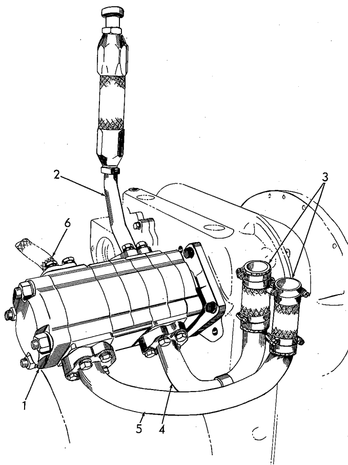
HYDRAULIC PUMP AND PIPING
