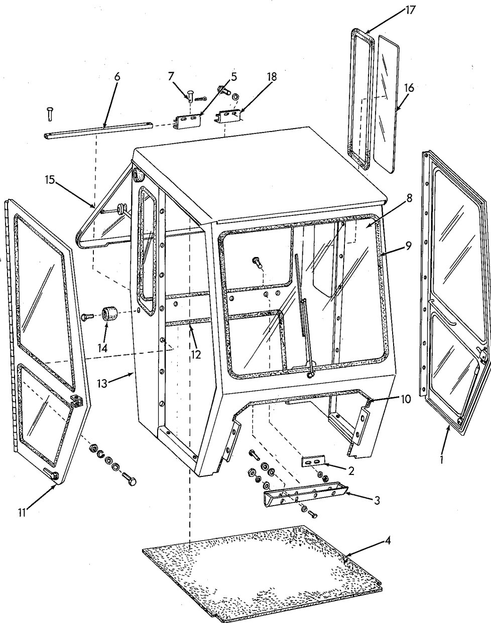
CAB
