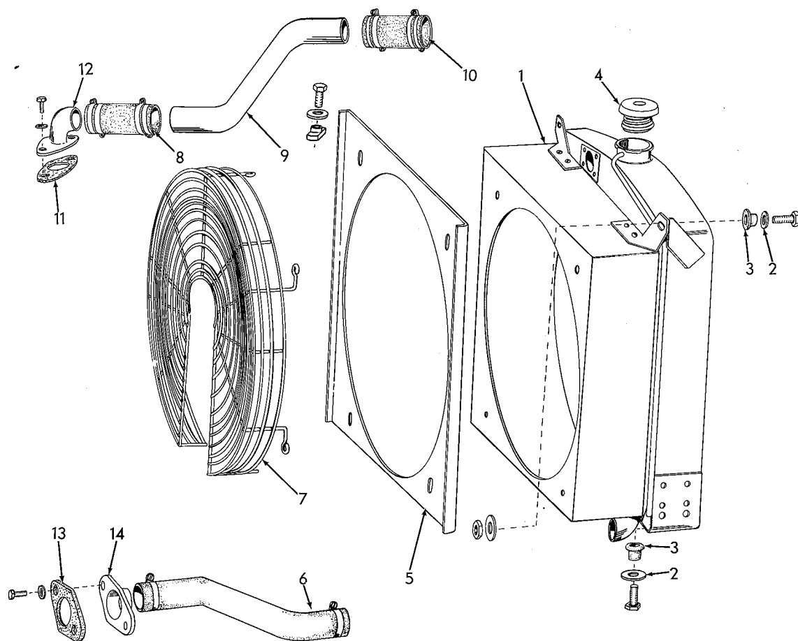
RADIATOR
