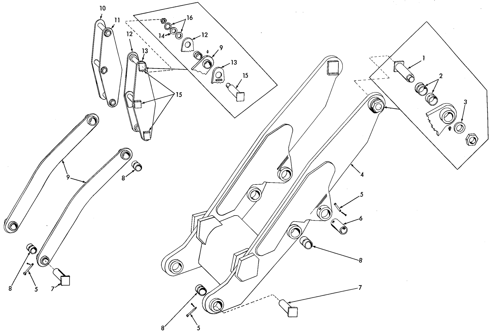
LINKAGE GROUP
