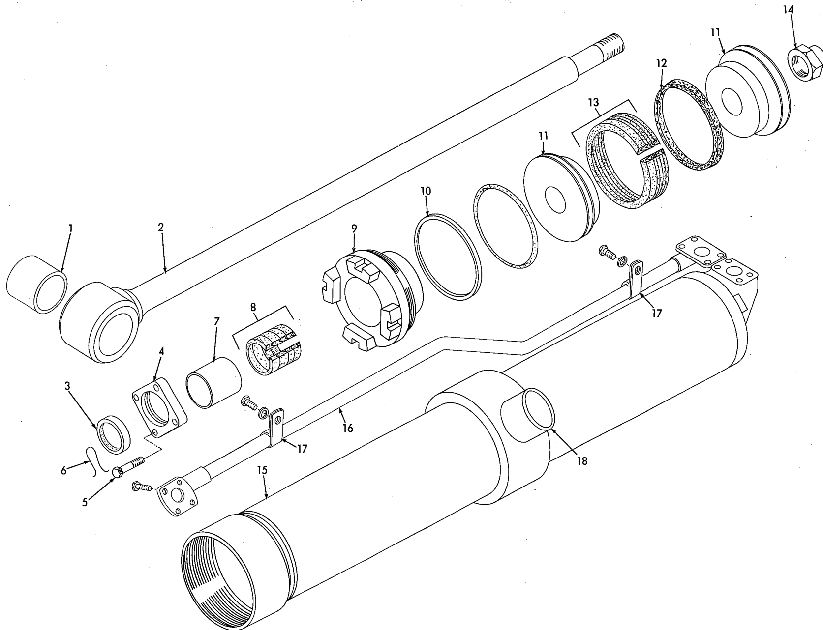
LIFT CYLINDER ASSEMBLY PARTS
