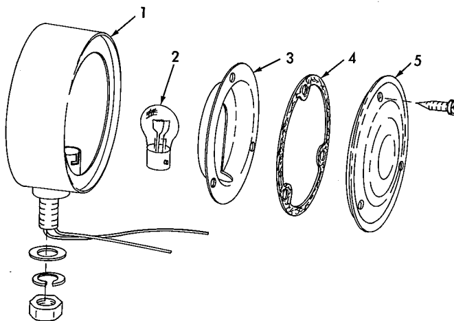
TAIL LIGHT ASSEMBLY 3044008
