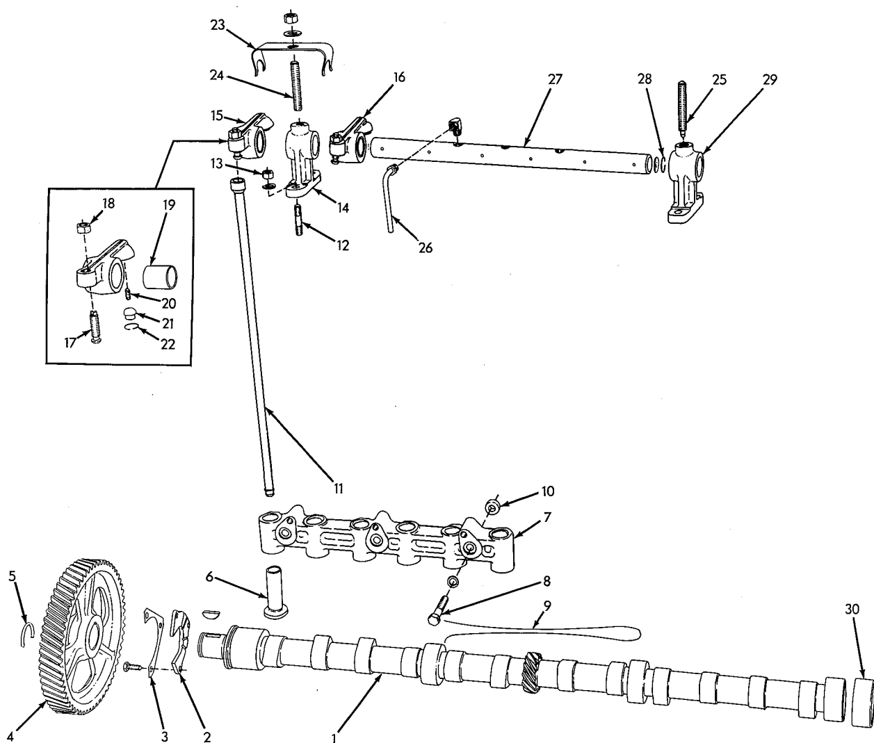
VALVE OPERATING MECHANISM
