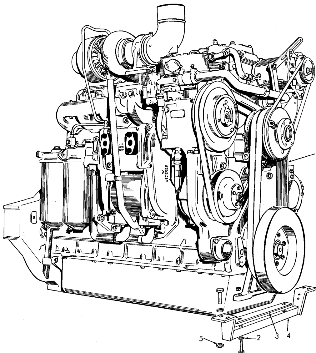
ENGINE AND MOUNTING
