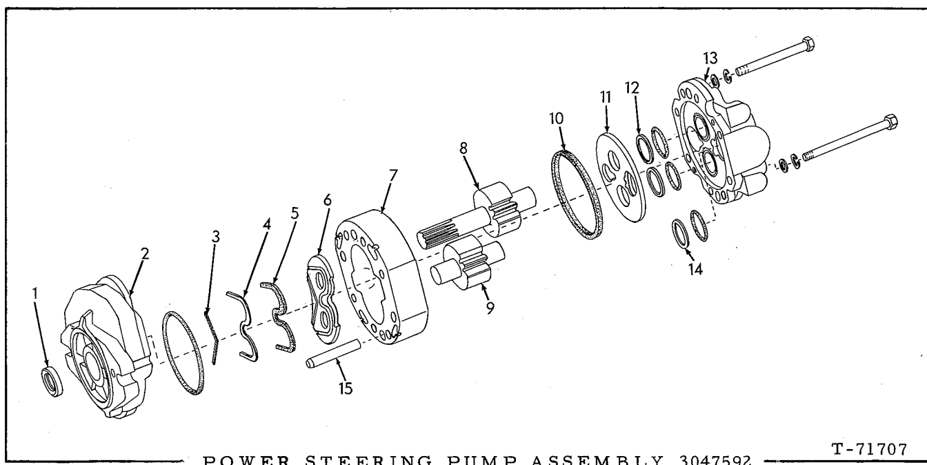
POWER STEERING PUMP ASSEMBLY 3047592
