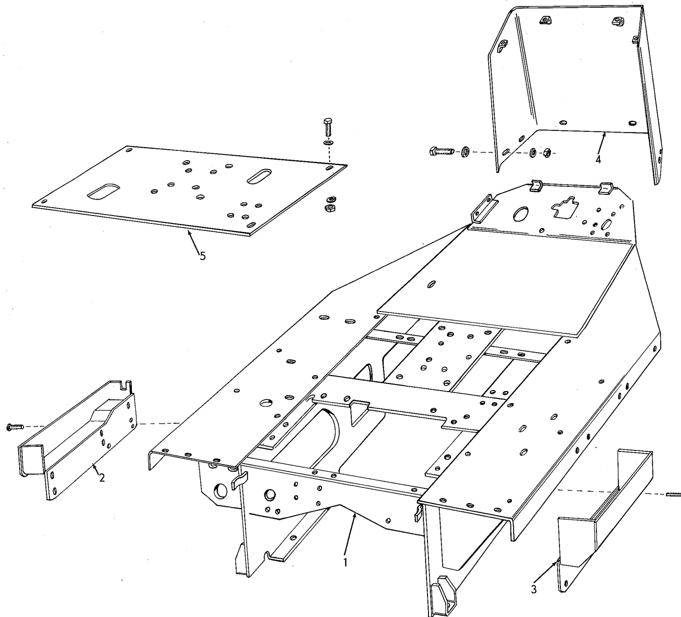
COWL, FLOOR PLATE AND PLATFORM
