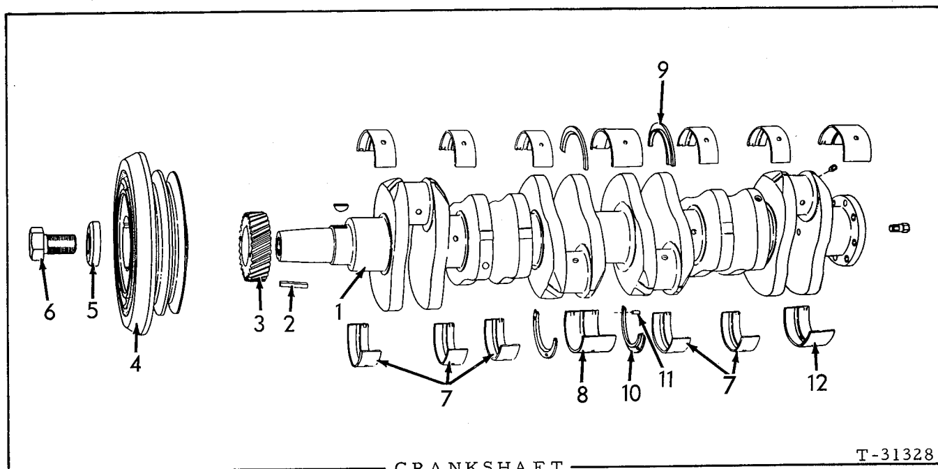
CRANKSHAFT
