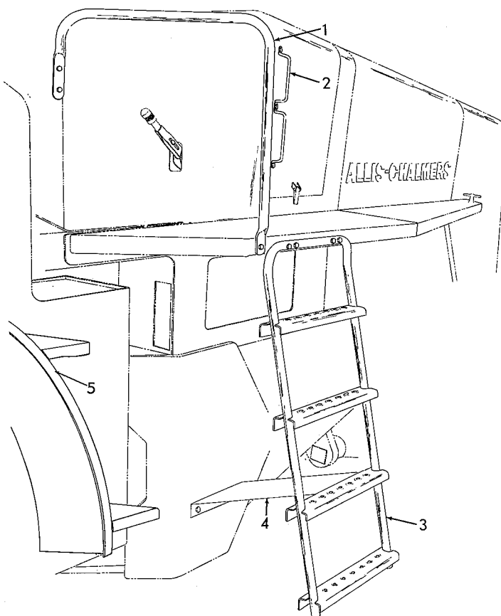
LADDER, HAND RAIL AND FENDERS
