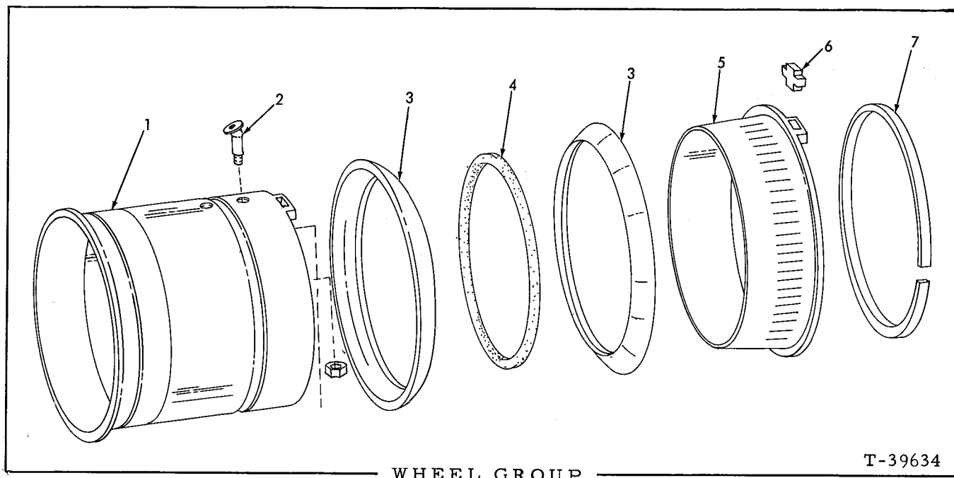
WHEEL GROUP
