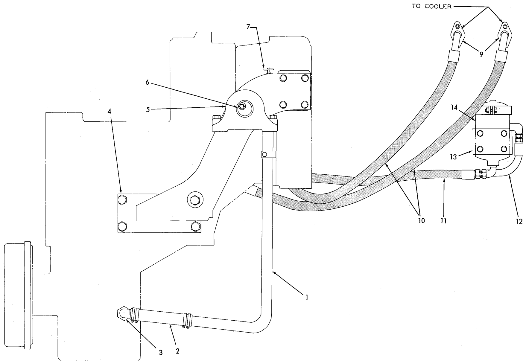
TRANSMISSION COOLING LINES, FILTER AND MOUNTING
