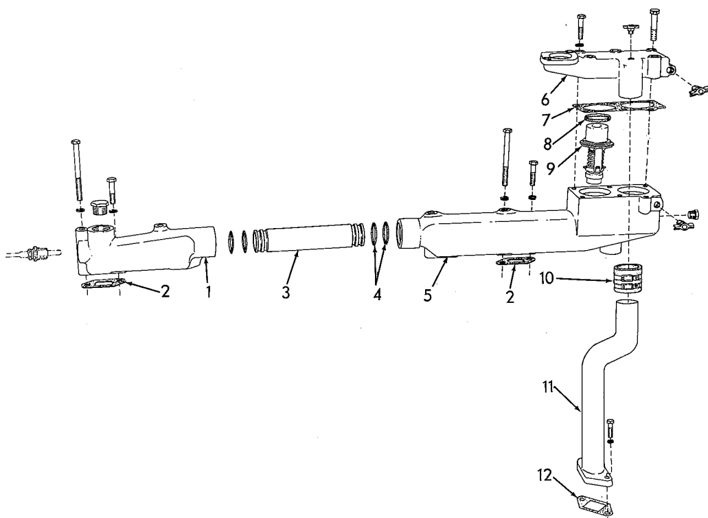
WATER OUTLET MANIFOLD
