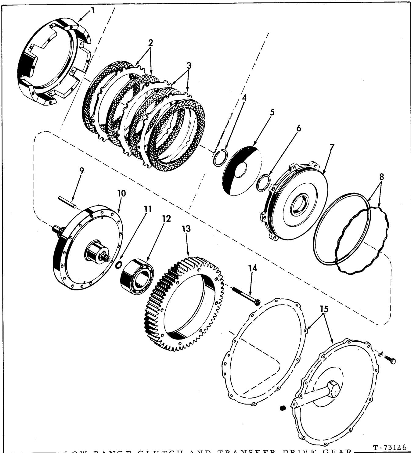
LOW RANGE CLUTCH AND TRANSFER DRIVE GEAR
