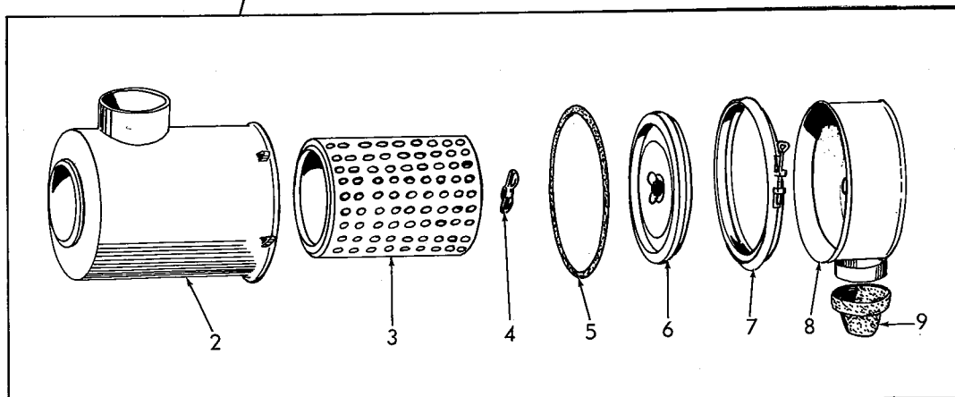
AIR CLEANER
