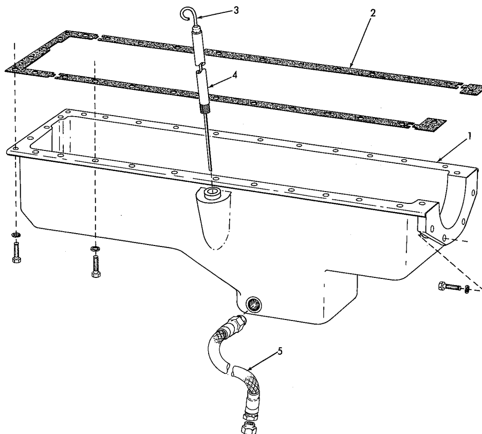
OIL PAN
