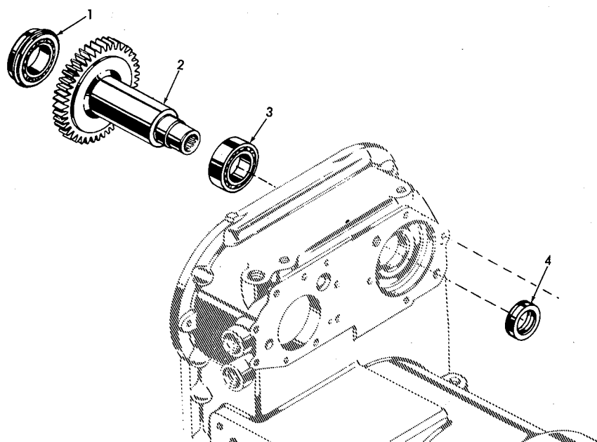
ACCESSORY DRIVE
