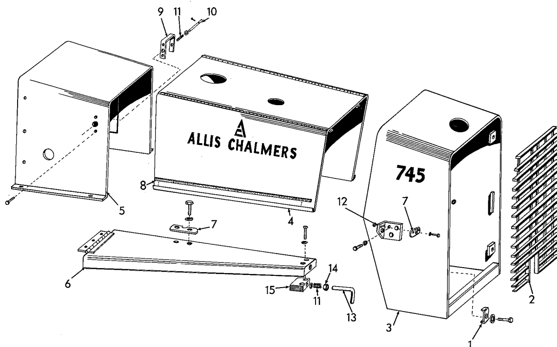
RADIATOR SUPPORT HOOD AND FENDERS
