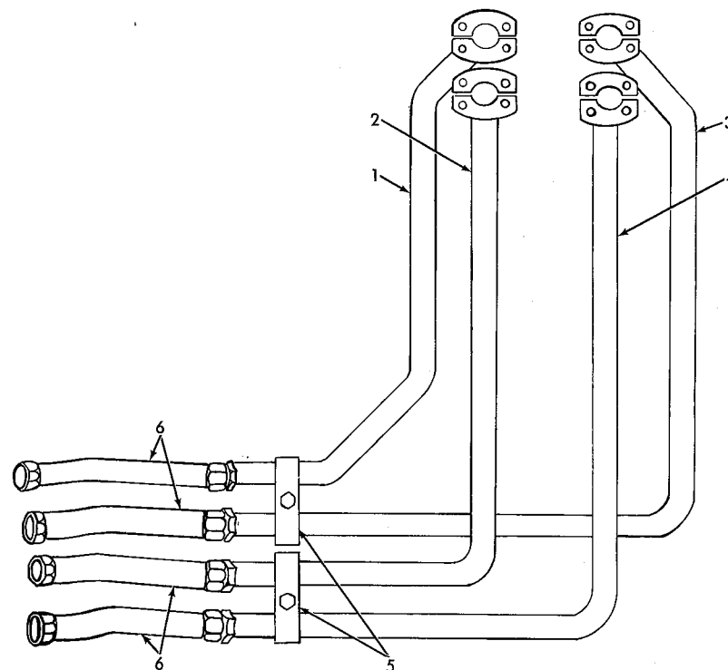
HYDRAULIC PIPING GROUP (Rear Section)
