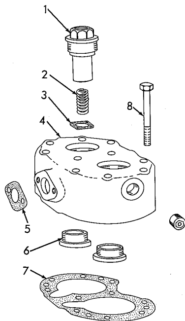
COMPRESSOR CYLINDER HEAD
