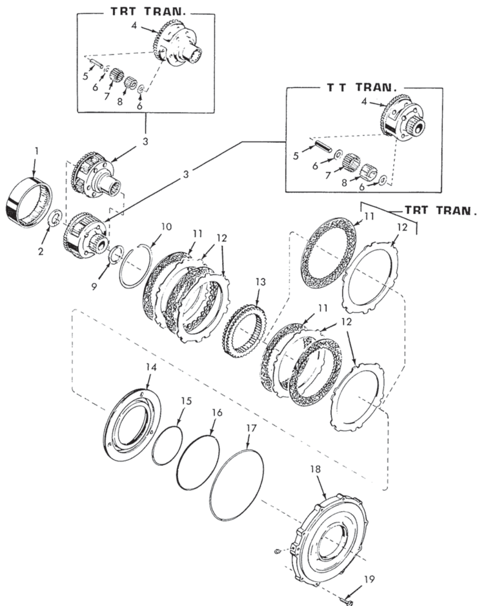
FORWARD CLUTCH AND PLANETARY
