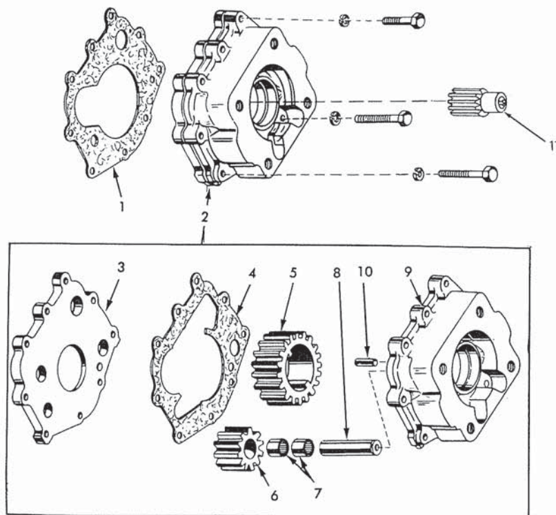
TRANSMISSION CHARGING OIL PUMP
