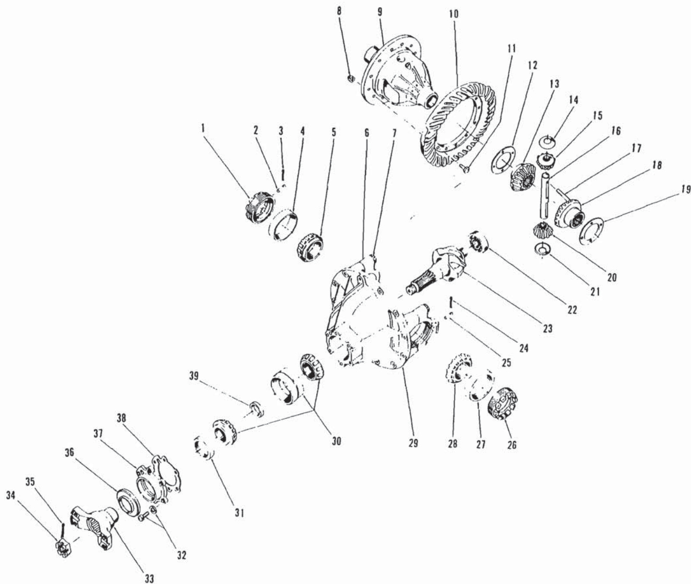
DIFFERENTIAL AND CARRIER ASSEMBLY — REAR DRIVE STEER
