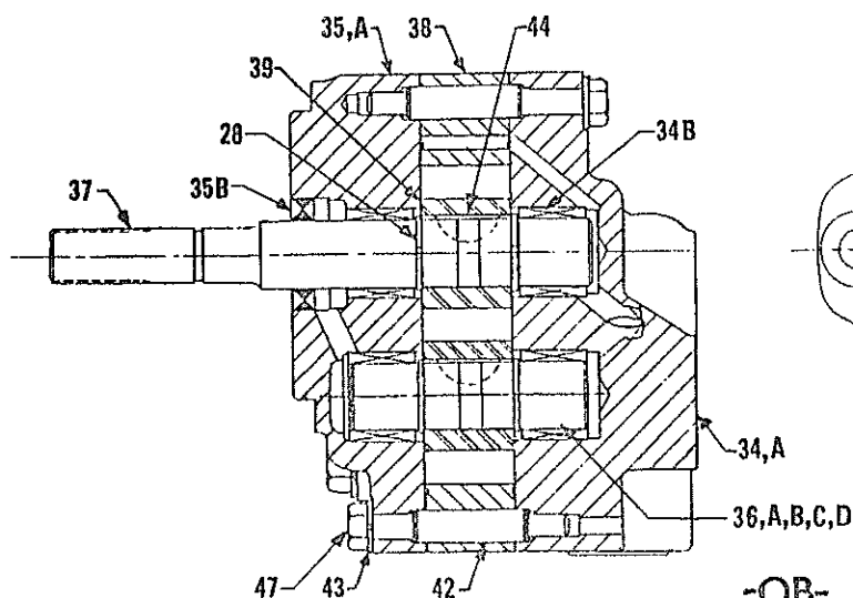
HYDRAULIC DUAL PUMP AND PULLEY (WEBSTER) (On Pacer 446, 447 - Super 466, 467)
