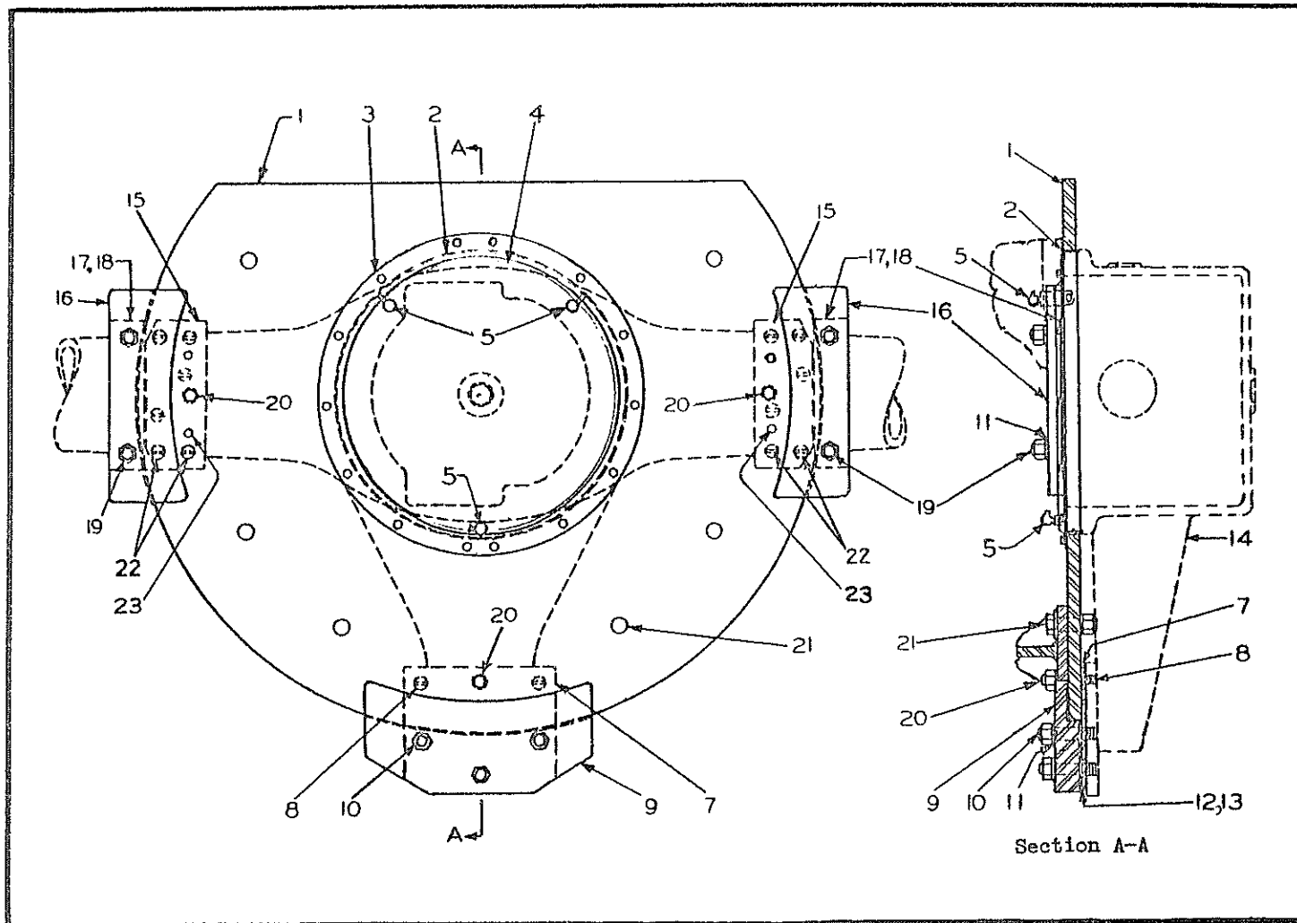
REAR AXLE CIRCLE ON SUPER 400 AND SUPER 500
