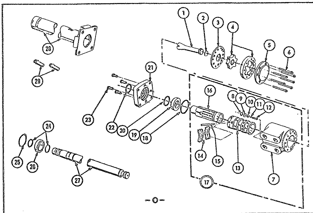
STEERING UNIT - ORBITROL
