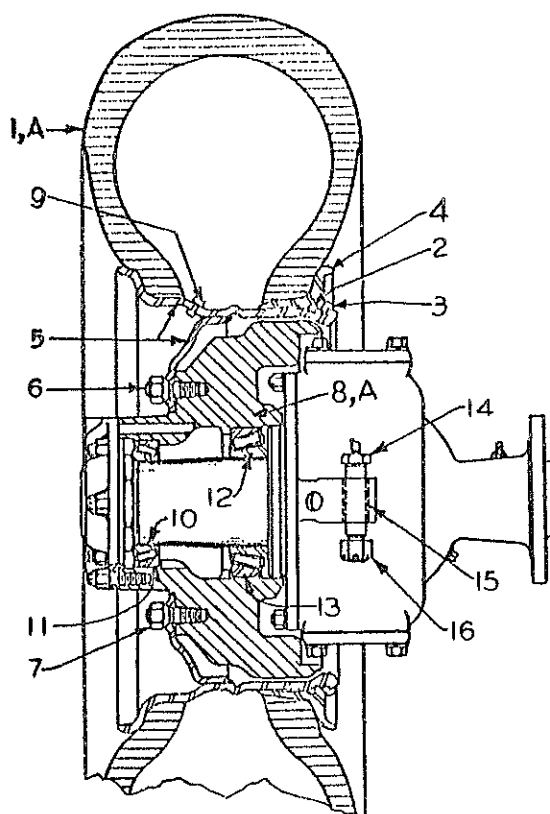
REAR AXLE STEERING KNUCKLE, WHEEL AND TIRE (On Pacer 400)
