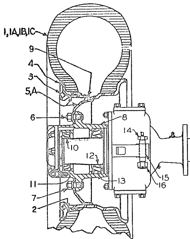
FRONT AXLE STEERING KNUCKLE, WHEEL AND TIRE (ON SUPER 400 AND SUPER 500)
