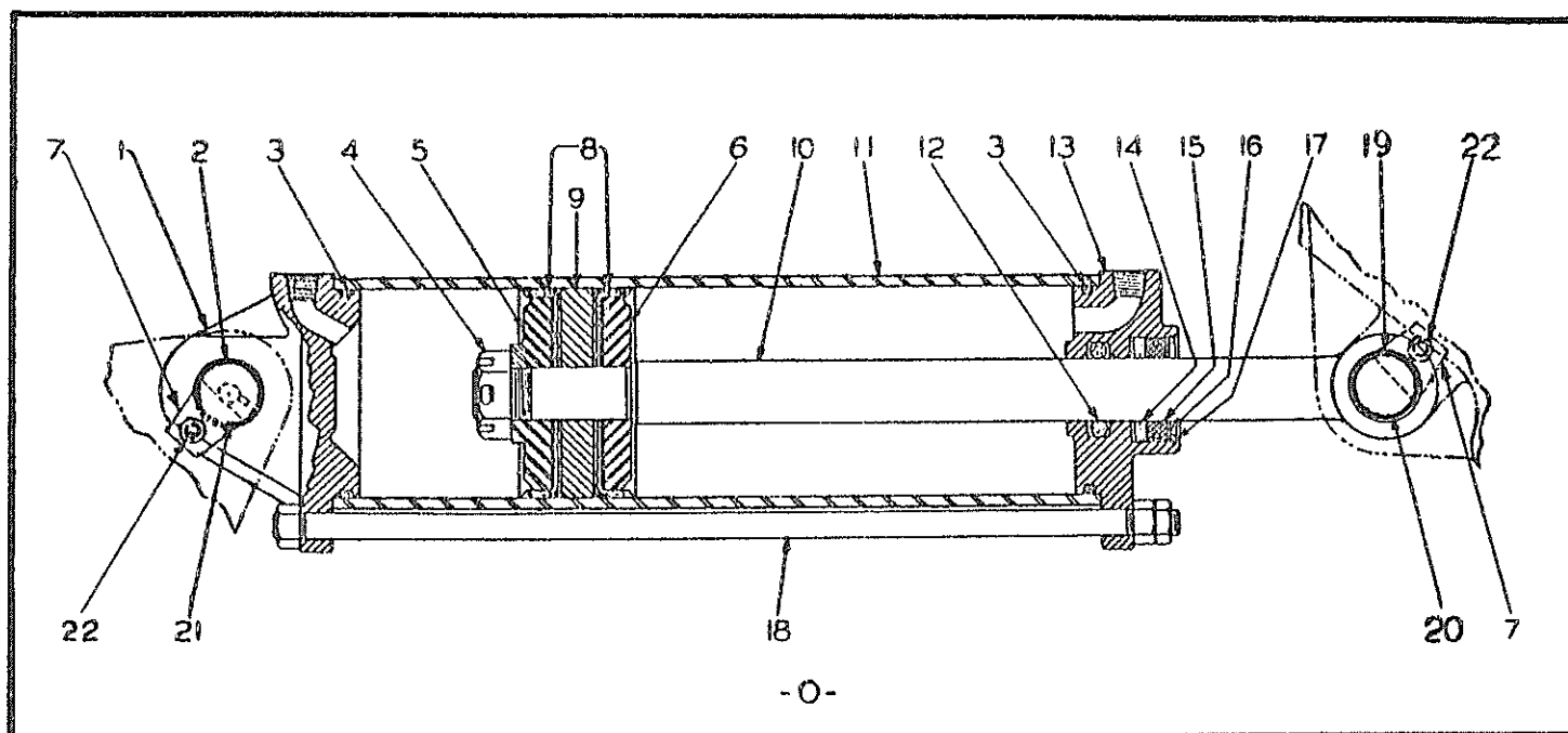
REAR AXLE STEERING RAM (On Super 400 & Super 500)
