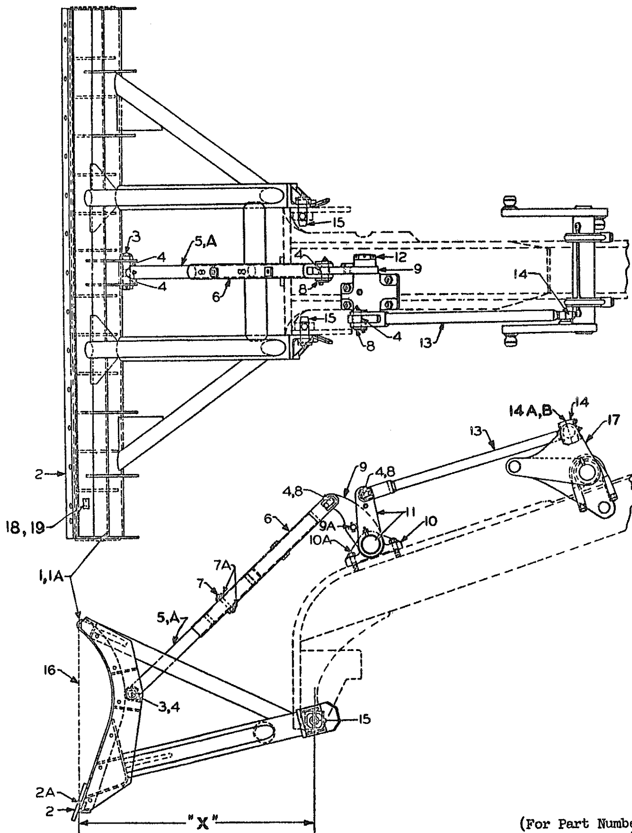
BULLDOZER (For Pacer 400 - Super 400 - Super 500)
