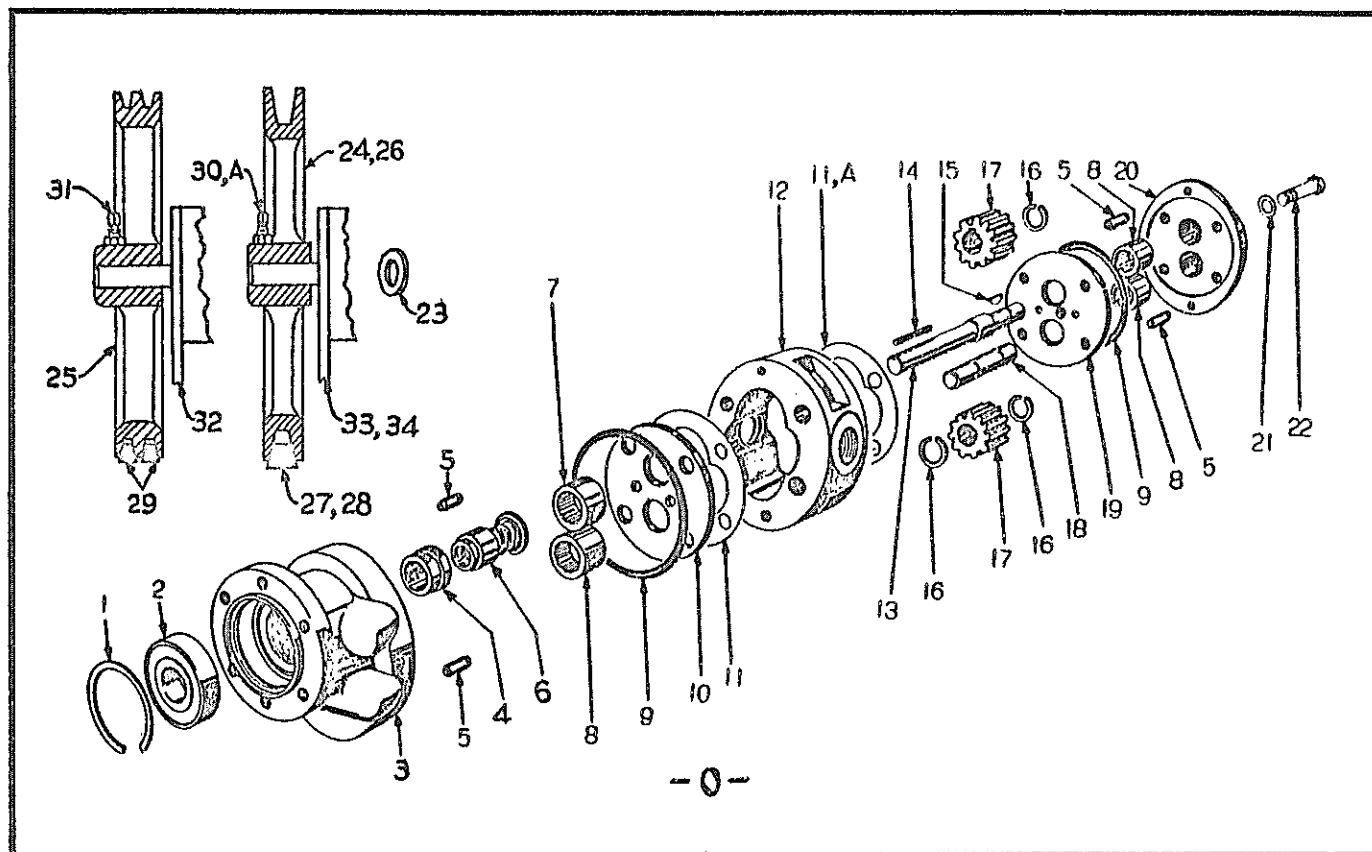
HYDRAULIC SINGLE PUMP AND PULLEY (HYDRECO) (On Pacer 445 - Super 465 - Super 565, 566)
