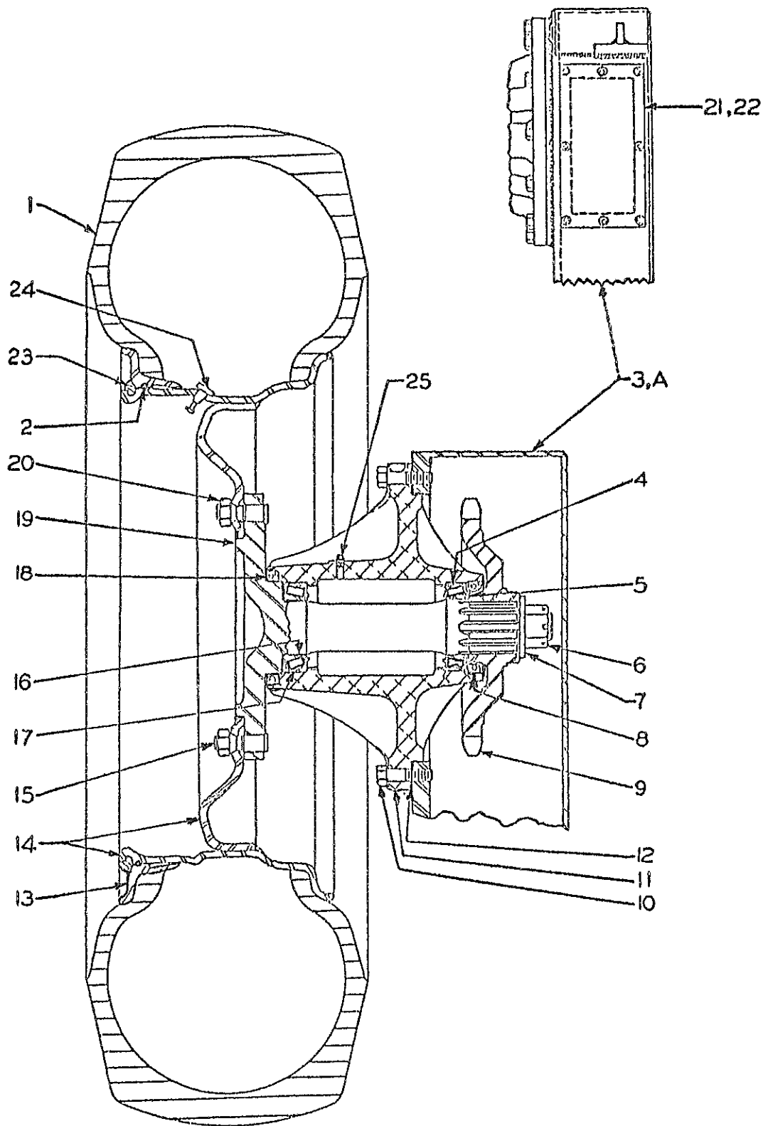
REAR WHEEL AND AXLE ASSEMBLY (On Super 400 and Super 500) (2" Pitch Chain)
