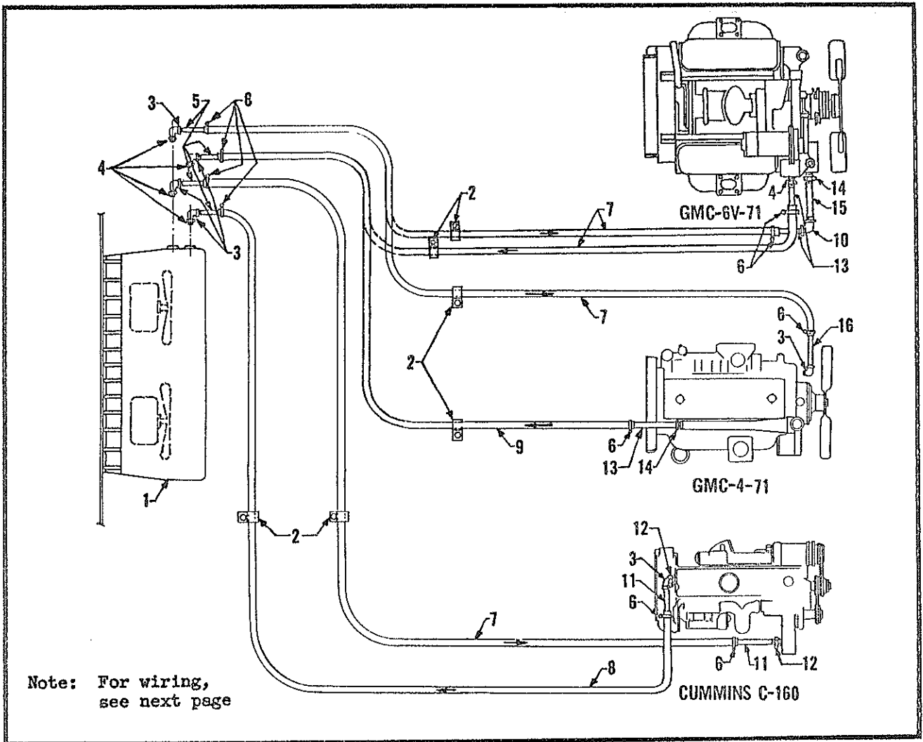
HEATER PIPING (For GMC-471, Cummins C-160, and GMC-6V-71 Engines)
