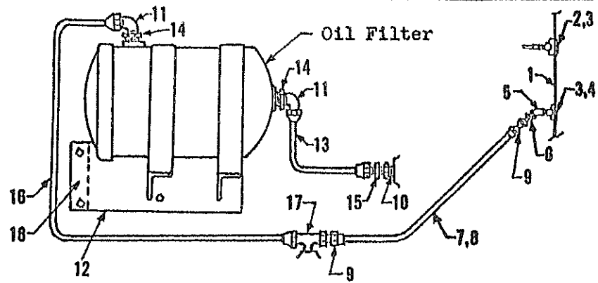
Oil Pressure Lines
