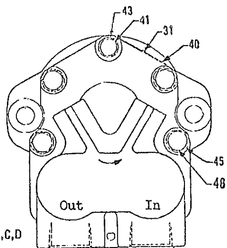
HYDRAULIC DUAL PUMP AND PULLEY (WEBSTER) (On Pacer 446, 447 - Super 466, 467)
