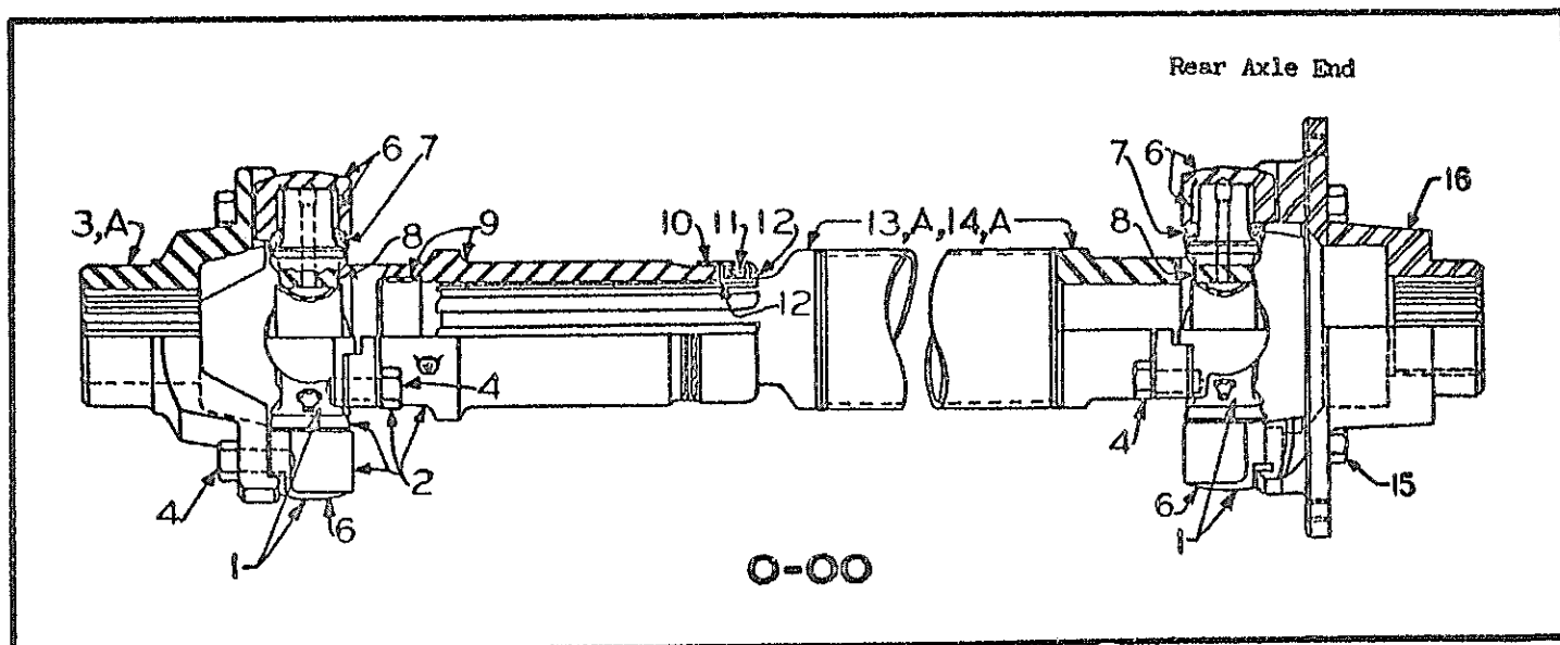
REAR PROPELLER SHAFT (From Transfer Case to Auxiliary Brake on Rear Axle Gear Carrier) (For Pacer 400 - Super 400 - Super 500)
