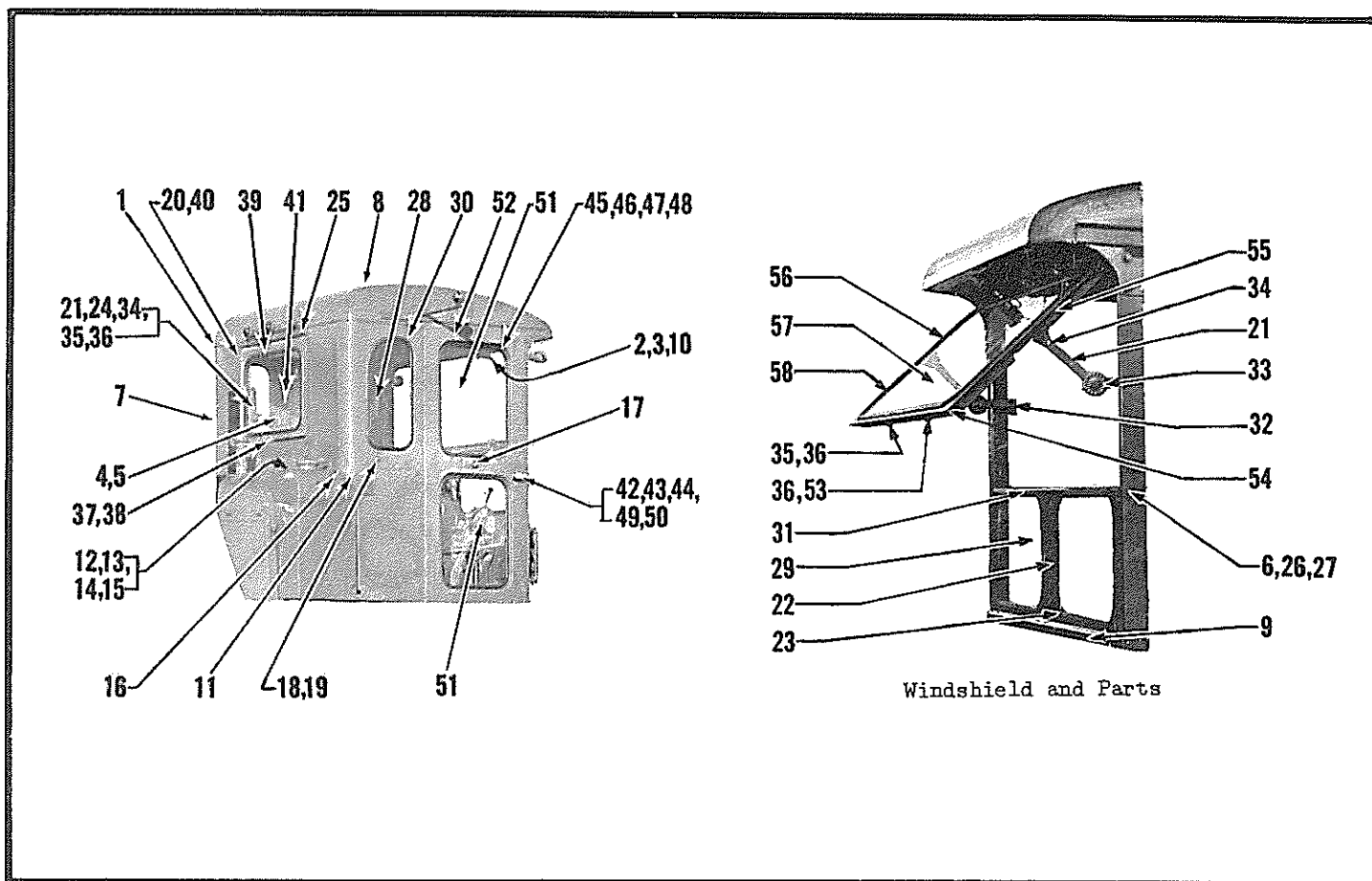
CAB - OPEN AND CLOSED TYPES (For Pacer 400 - Super 400 - Super 500)
