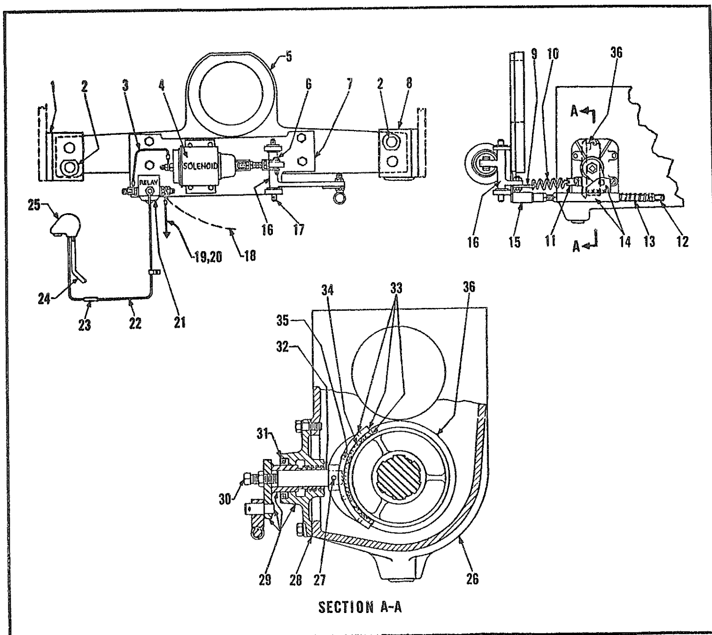
TRANSMISSION BRAKE FOR 4-SPEED MANUAL SHIFT TRANSMISSION (On Pacer 447 and Super 467)
