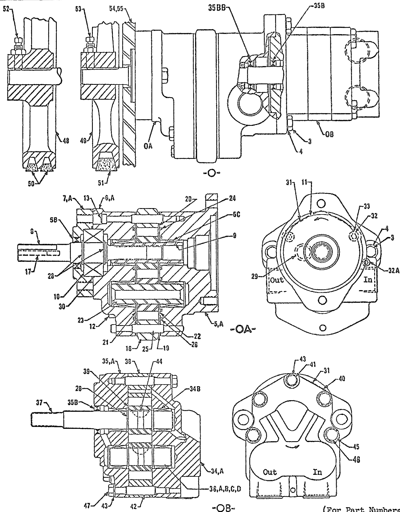
HYDRAULIC DUAL PUMP AND PULLEY (WEBSTER) (On Pacer 446, 447 - Super 466, 467)
