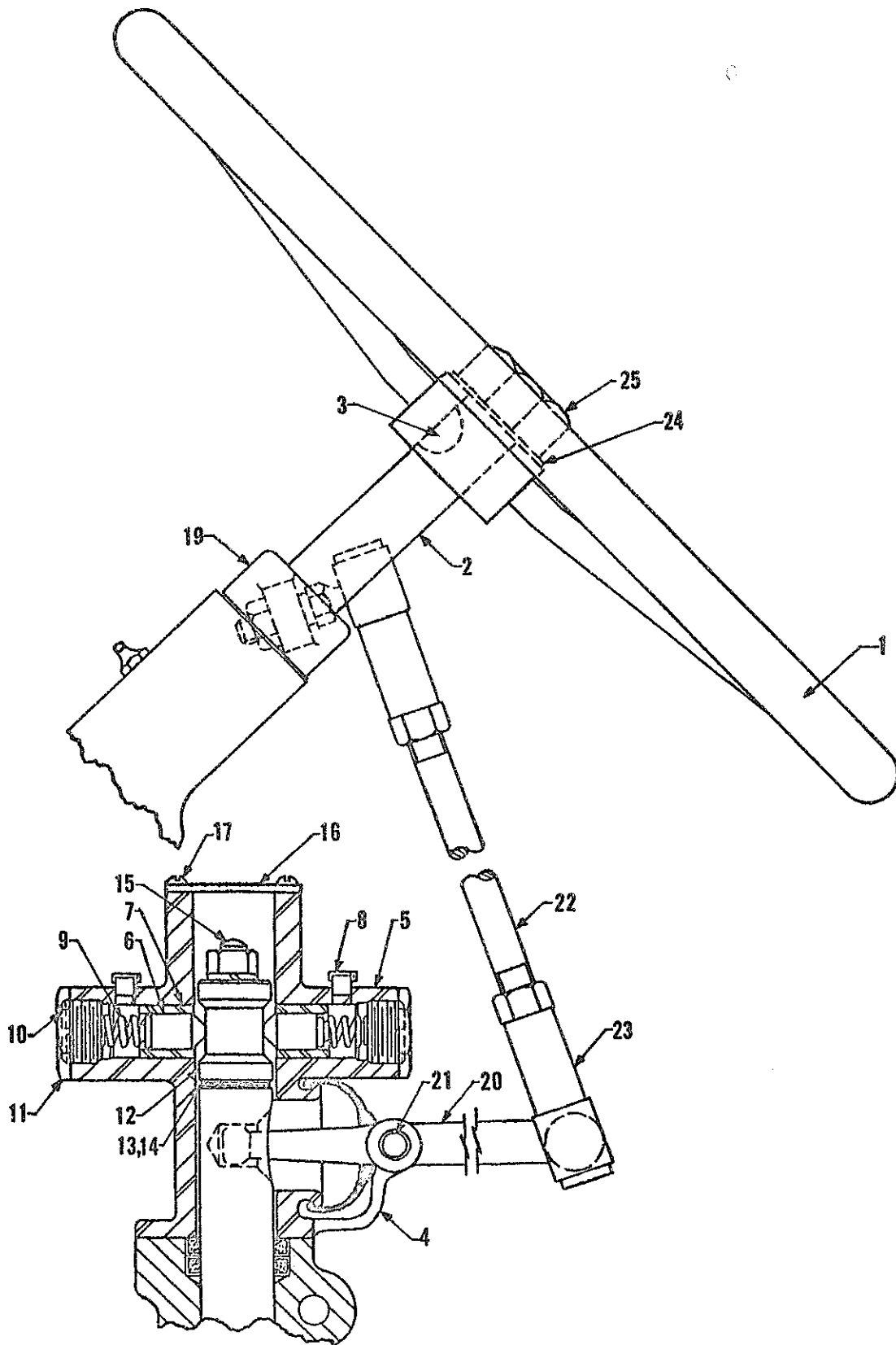
DUOMATIC FRONT STEER MECHANISM (For Pacer 400 - Super 400 - Super 500)
