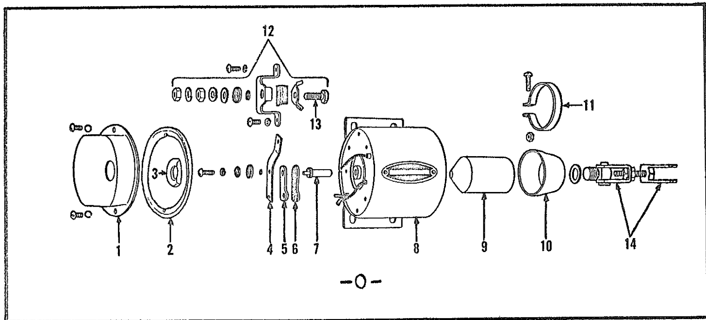
SOLENOID SWITCH FOR CIRCLE LATCH OR TRANSMISSION BRAKE* (On Pacer 400 - Super 400 - Super 500)
