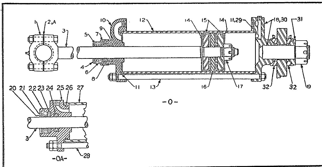
SCARIFIER RAM (Also used with Bulldozer) (For Pacer 400 - Super 400 - Super 500)
