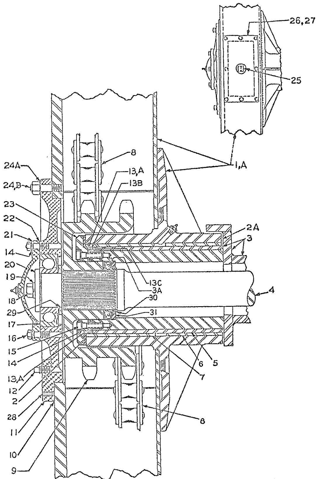
REAR AXLE PIVOT CASE AND SHAFT (On Super 400 and Super 500) (2" Pitch Chain)
