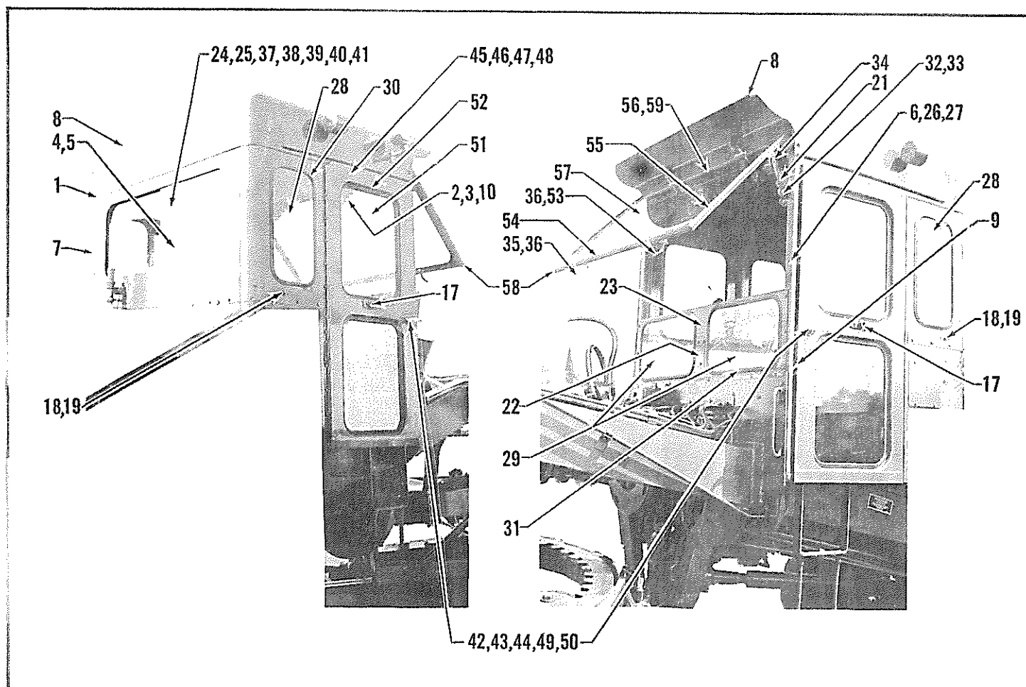
CAB - OPEN AND CLOSED TYPES
