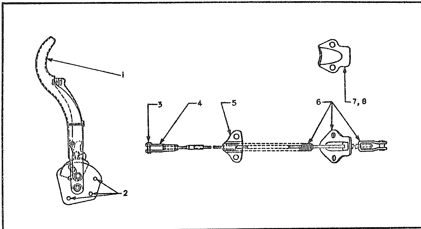
HAND BRAKE MECHANISM (PROPELLER SHAFT BRAKE) (On Pacer 400 - Super 400 - Super 500)
