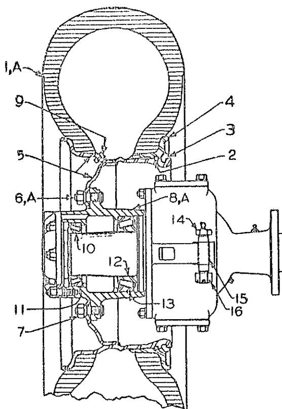
FRONT AXLE STEERING KNUCKLE, WHEEL AND TIRE (ON PACER 400)
