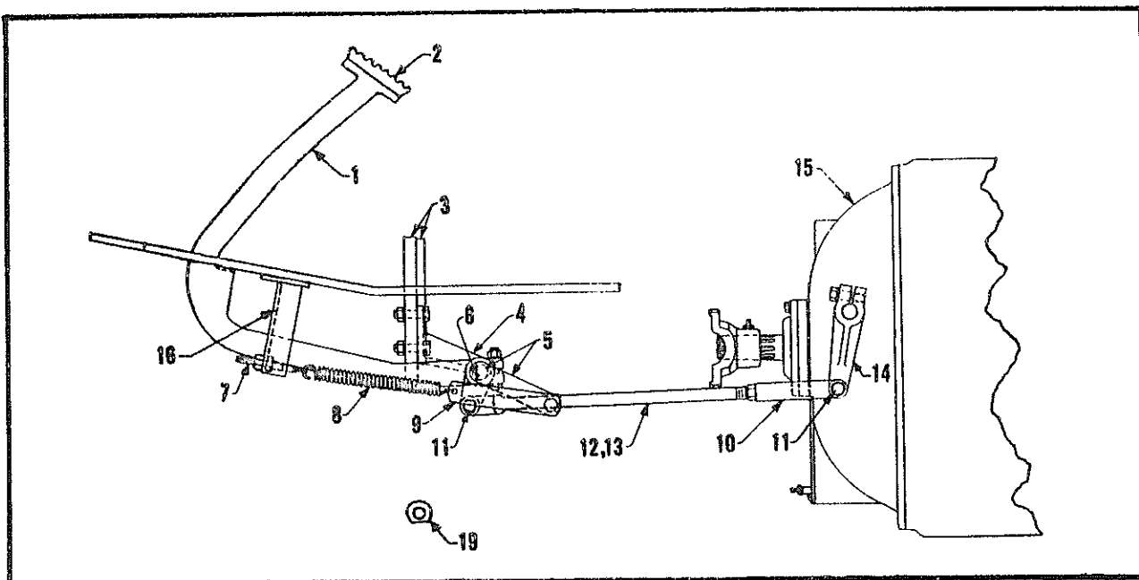
DRIVING CLUTCH OPERATING MECHANISM (On Pacer 445 & 446 - Super 465 & 466 - Super 565 & 566)
