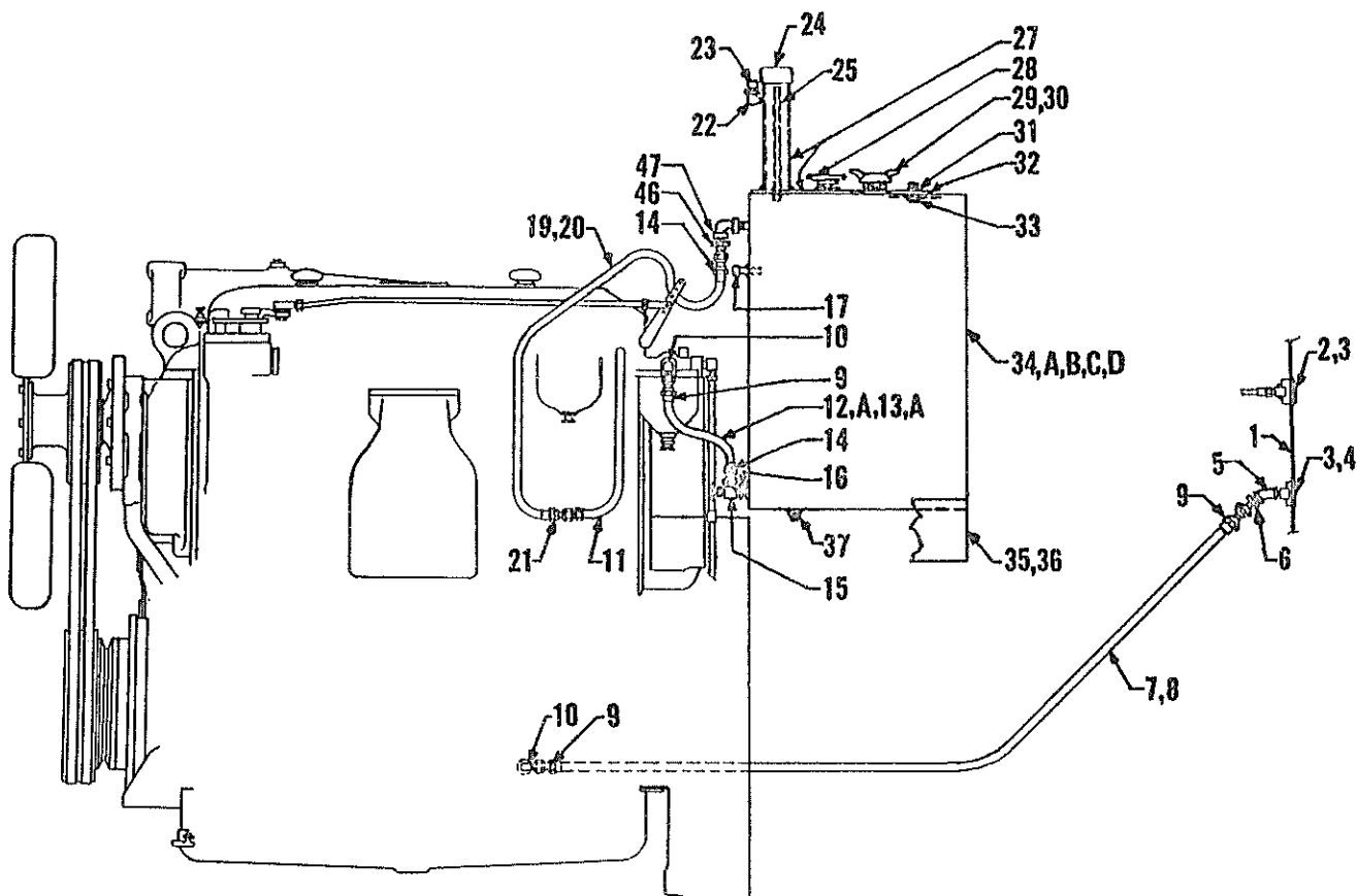
Fuel and Oil Lines
