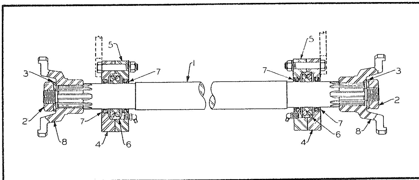
CENTER SECTION OF FRONT PROPELLER SHAFT (ON PACER 400 - SUPER 400 - SUPER 500)
