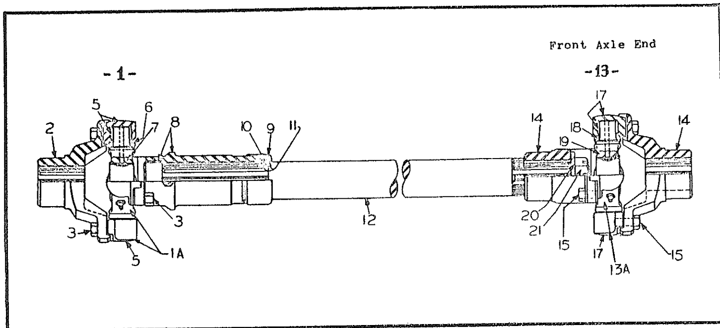
FRONT SECTION OF FRONT PROPELLER SHAFT (ON PACER 400 - SUPER 400 - SUPER 500)
