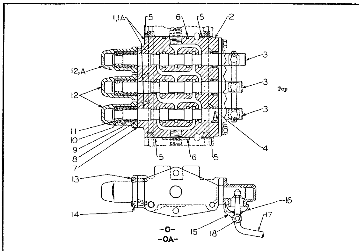
HYDRAULIC CONTROL TRIPLE VALVE (On Pacer 400 - Super 400 - Super 500)
