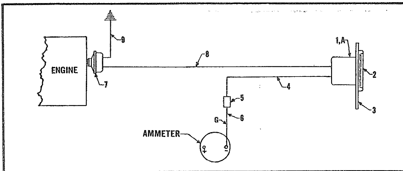
HOURLMETER FOR GMC-4-71 ENGINE
