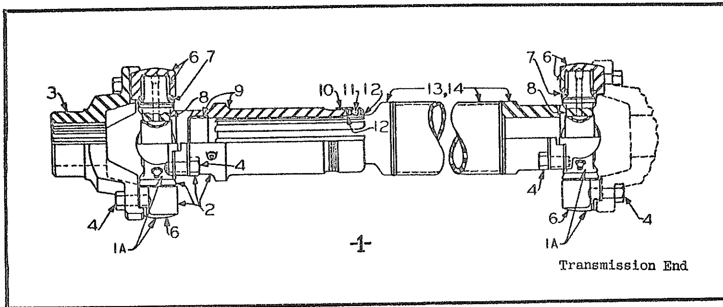
PROPELLER SHAFT (4-Speed Power Shift Transmission To Single Speed Transfer Case) (On Pacer 448 and Super 468)
