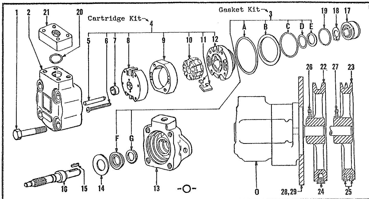
HYDRAULIC SINGLE PUMP AND PULLEY (VICKERS) (On Pacer 448 - Super 468)
