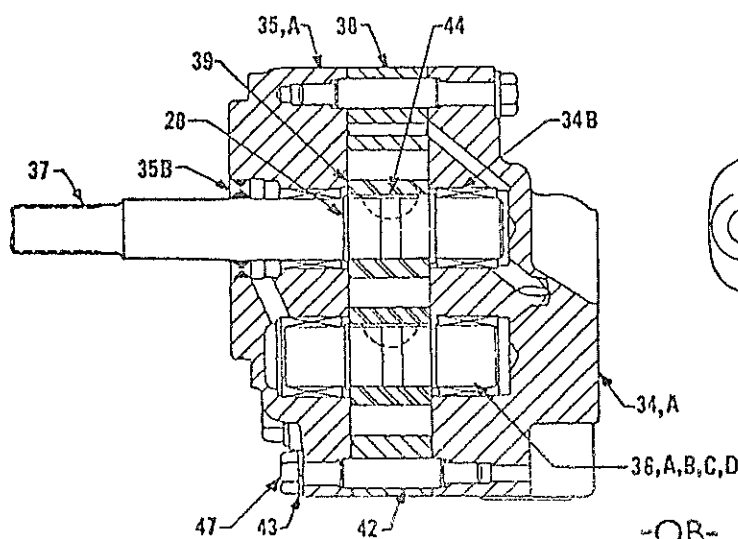
HYDRAULIC DUAL PUMP AND PULLEY (WEBSTER) (On Pacer 446, 447 - Super 466, 467)
