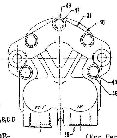
HYDRAULIC DUAL PUMP AND PULLEY (WEBSTER) (On Pacer 446, 447 - Super 466, 467)
