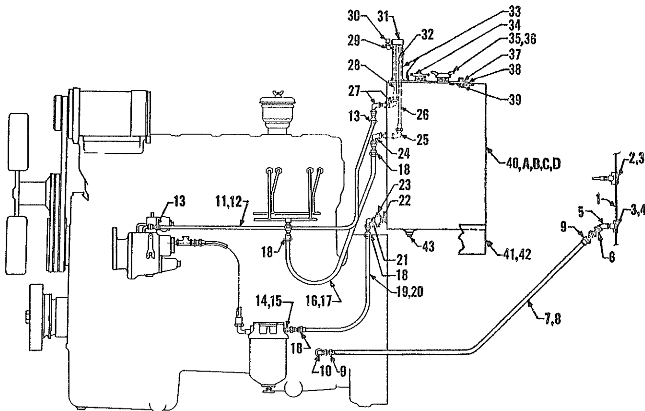
Fuel and Oil Lines
