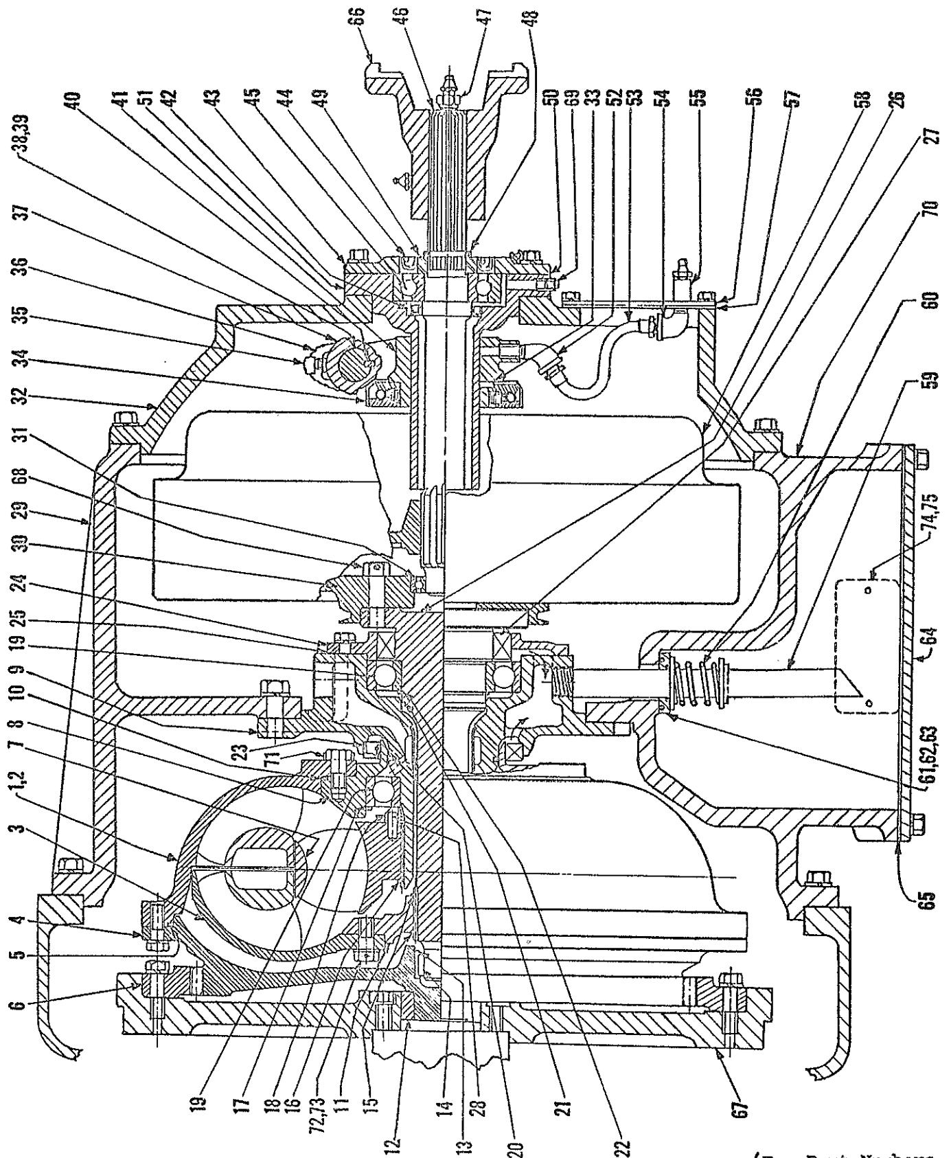
TORCON TORQUE CONVERTER (14") IN COMBINATION WITH CLUTCH DRIVE (On Pacer 446 and Super 466)
