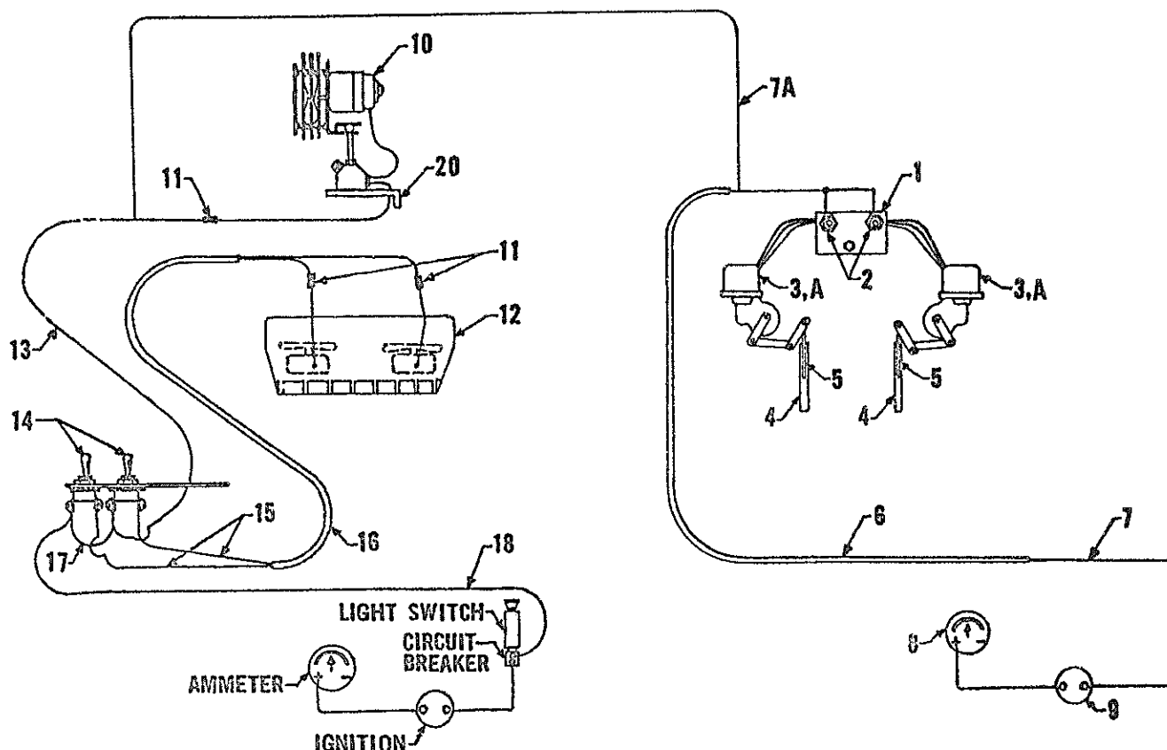
HEATER, DEFROSTER, AND WINDSHIELD WIPER WIRING (For Pacer 400 - Super 400 - Super 500)
