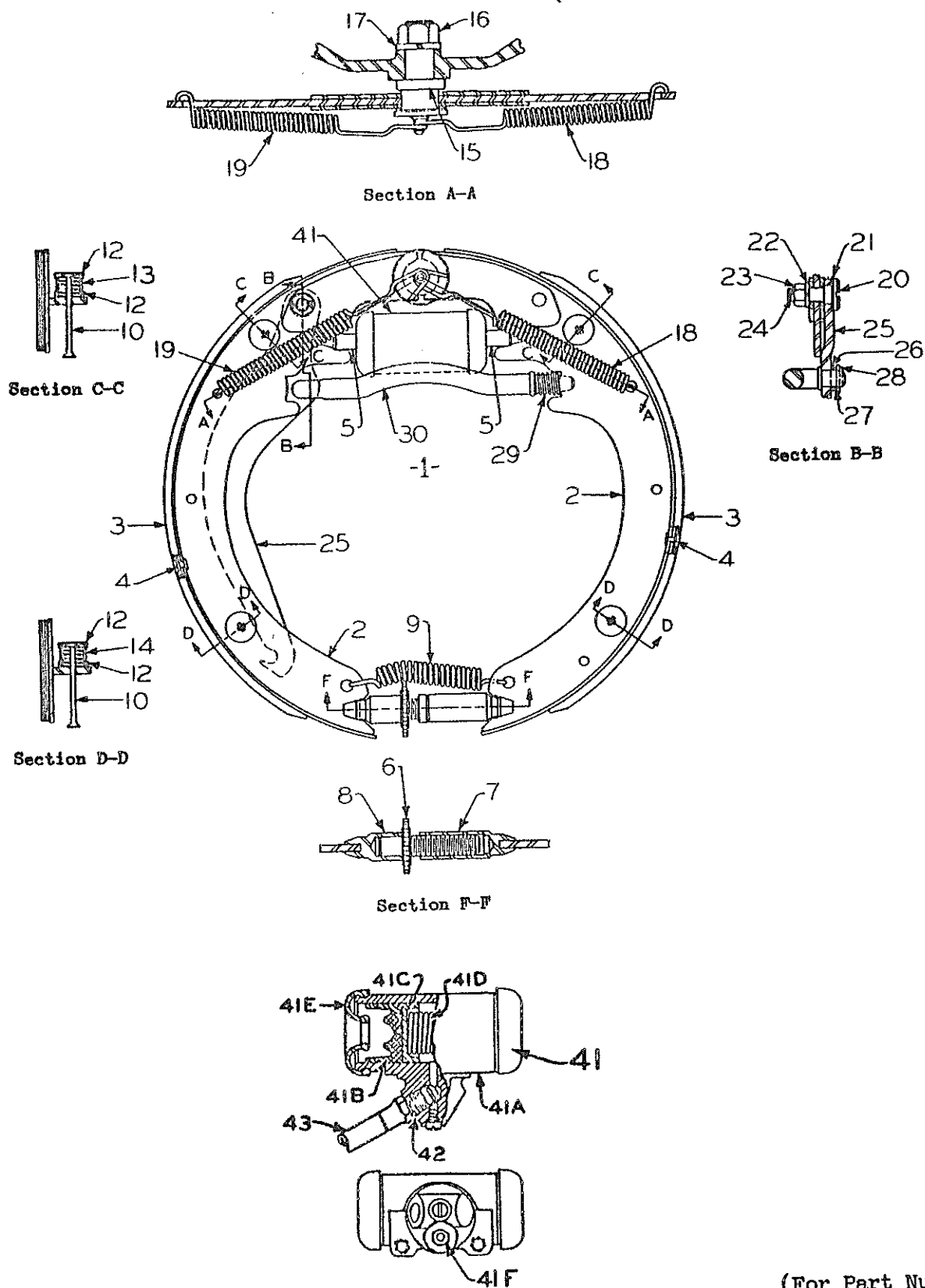
PROPELLER SHAFT BRAKE (On Pacer 400 - Super 400 - Super 500)
