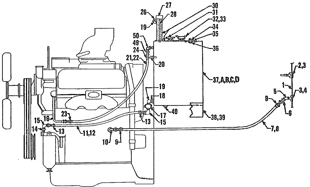
Fuel and Oil Lines
