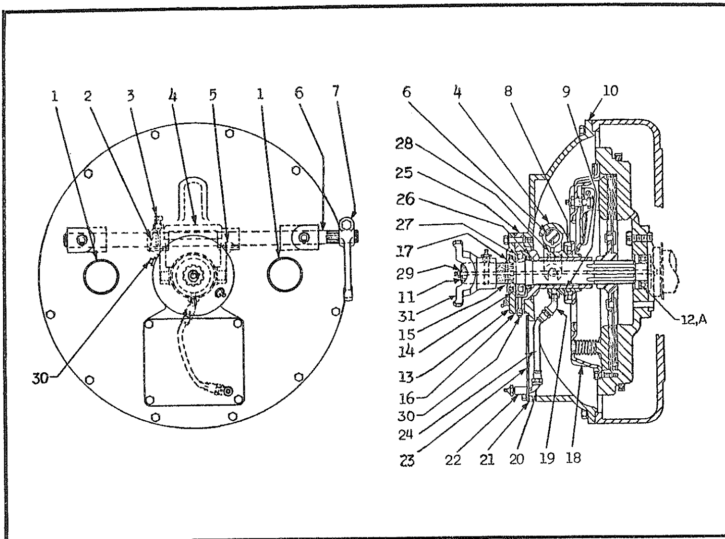
CLUTCH AND SHAFT ASSEMBLY FOR DRY CLUTCH DRIVE (ON PACER 445 - SUPER 465 - SUPER 565)
