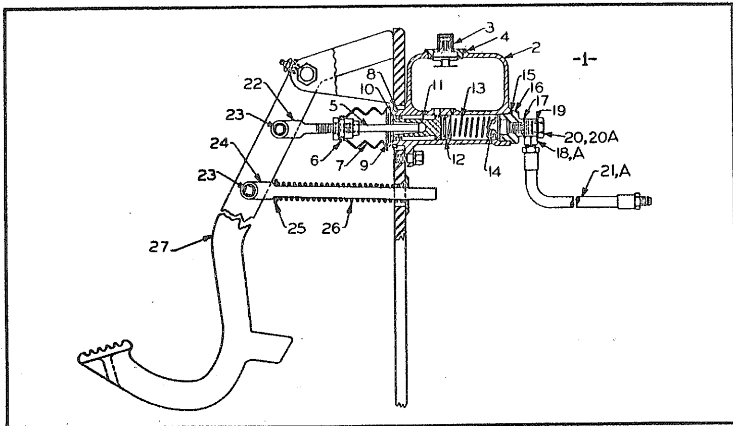
FOOT BRAKE MECHANISM (PROPELLER SHAFT BRAKE) (On Pacer 400 - Super 400 - Super 500)
