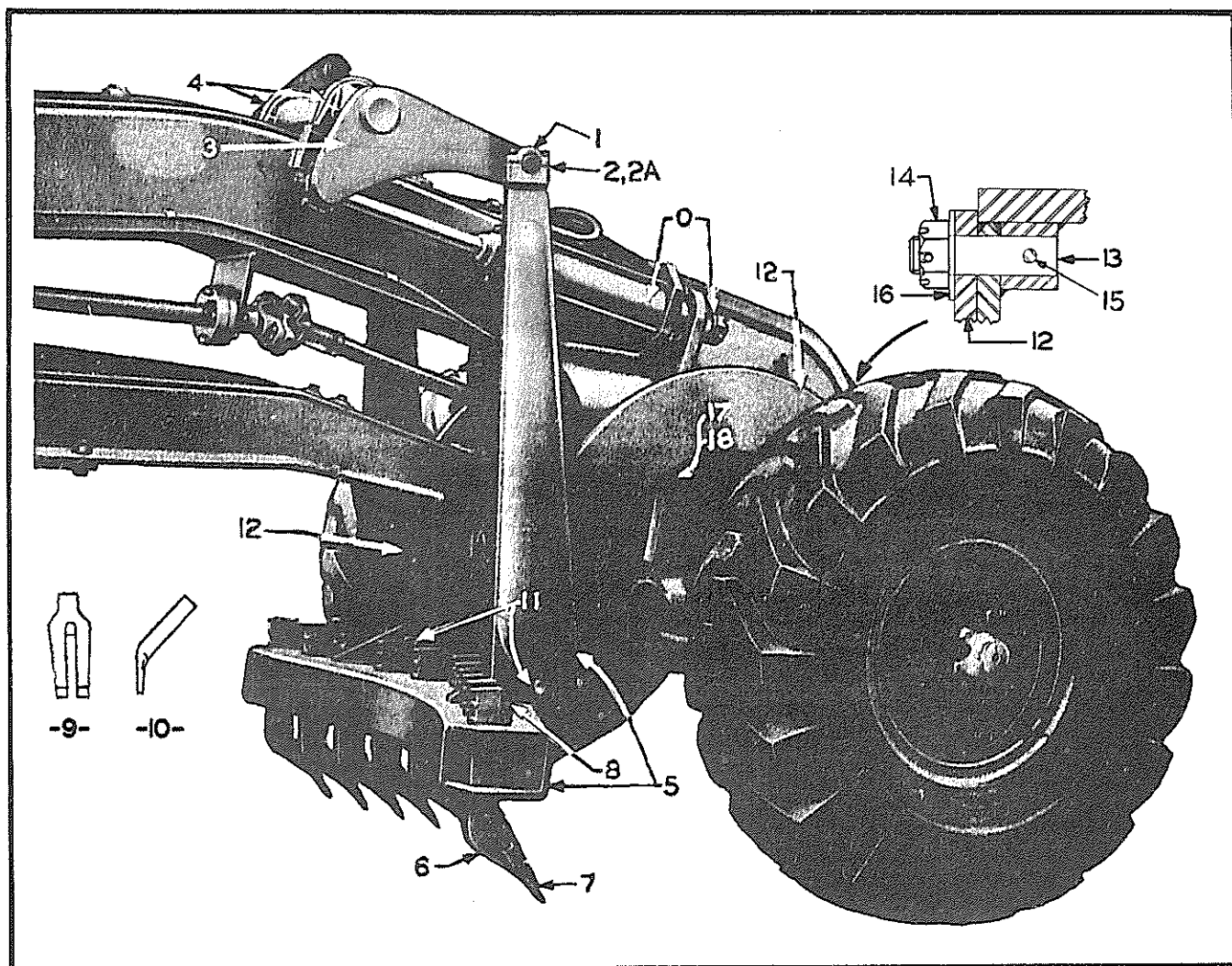
SCARIFIER (FOR PACER 400 - SUPER 400 - SUPER 500 GRADERS)
