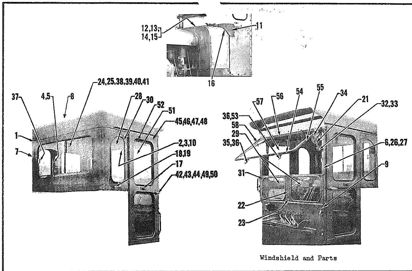
CAB - OPEN AND CLOSED TYPES (For Pacer 400 - Super 400 - Super 500)
