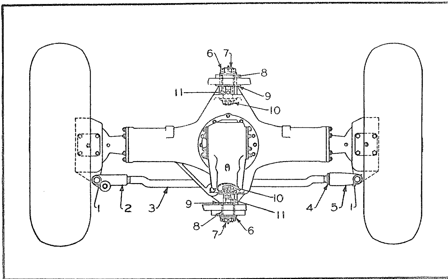
FRONT AXLE TIE ROD AND AXLE SUPPORT (ON PACER 400 - SUPER 400 - SUPER 500)
