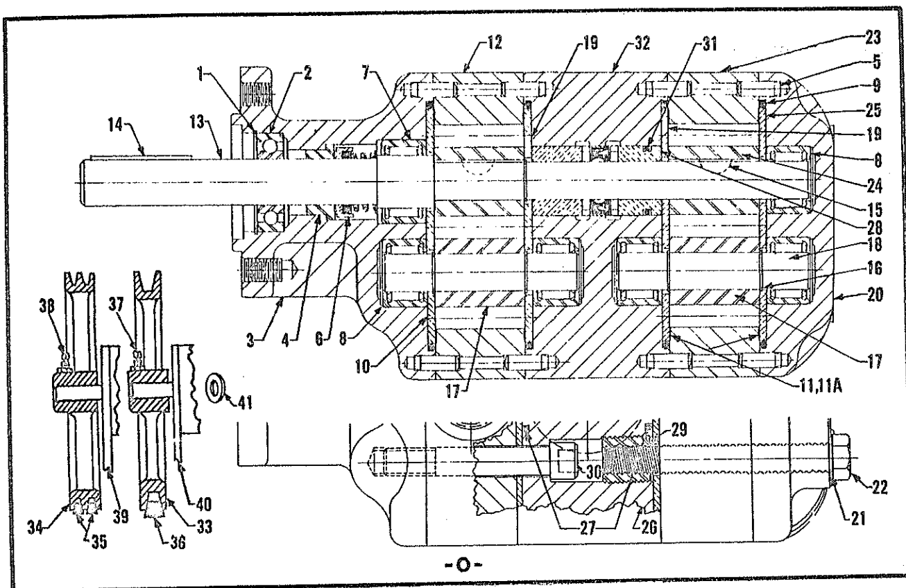
HYDRAULIC DUAL PUMP AND PULLEY (HYDRECO) (On Pacer 446, 447 - Super 466, 467)
