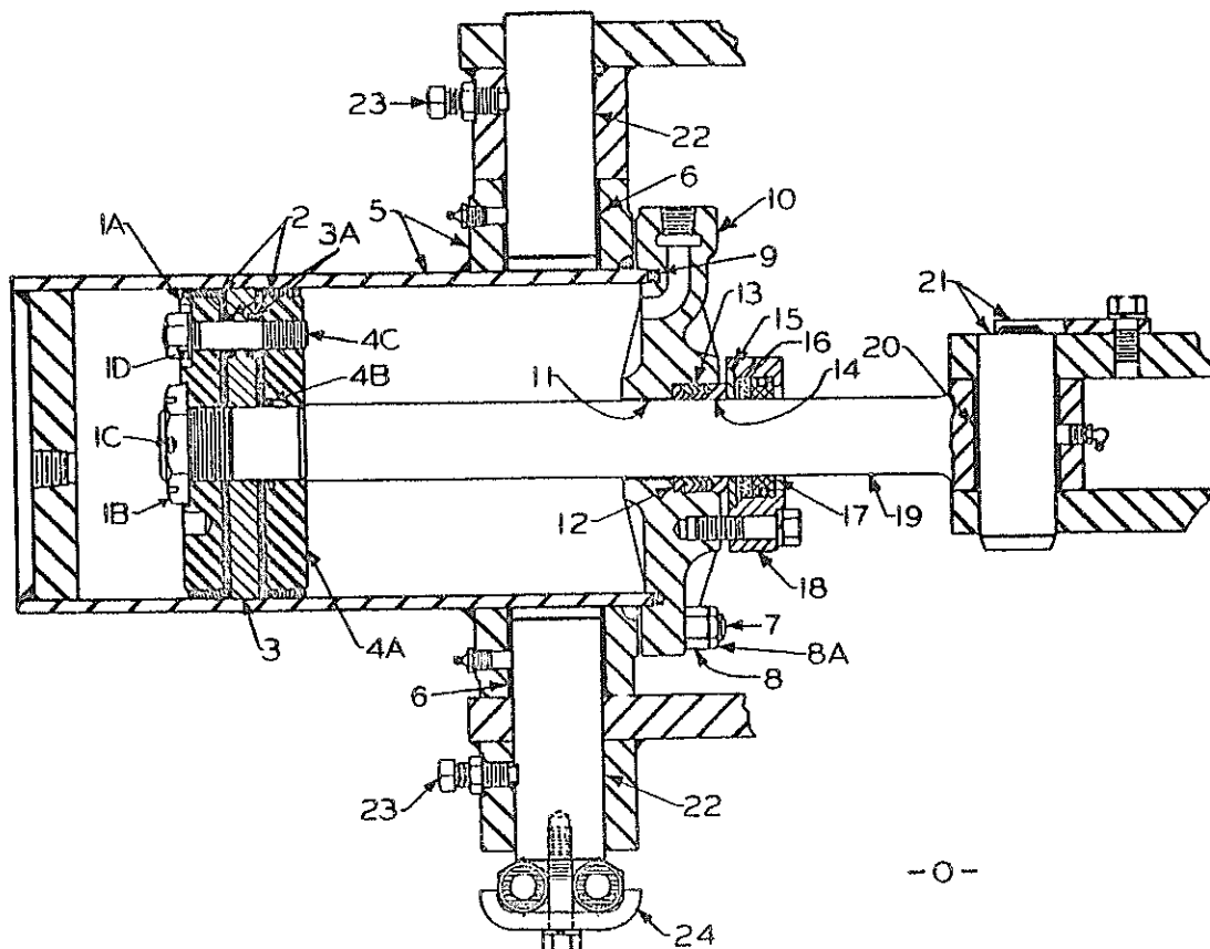
HIGH LIFT RAM (ON PACER 400 - SUPER 400 - SUPER 500)
