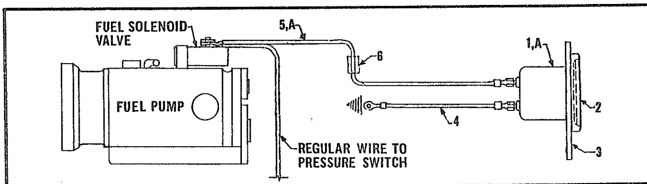
HOURLMETER FOR CUMMINS C-160 ENGINE
