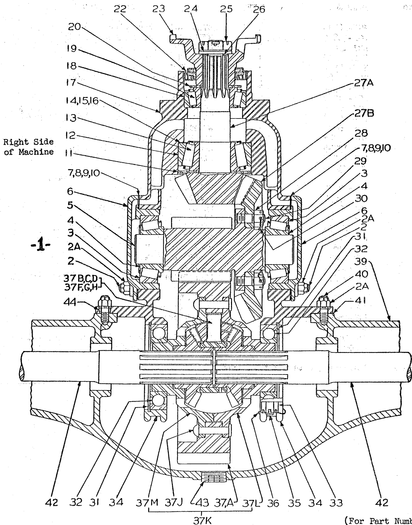
FRONT AXLE GEAR CARRIER
