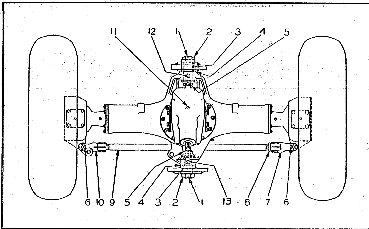
FRONT AXLE TIE ROD AND AXLE SUPPORT
