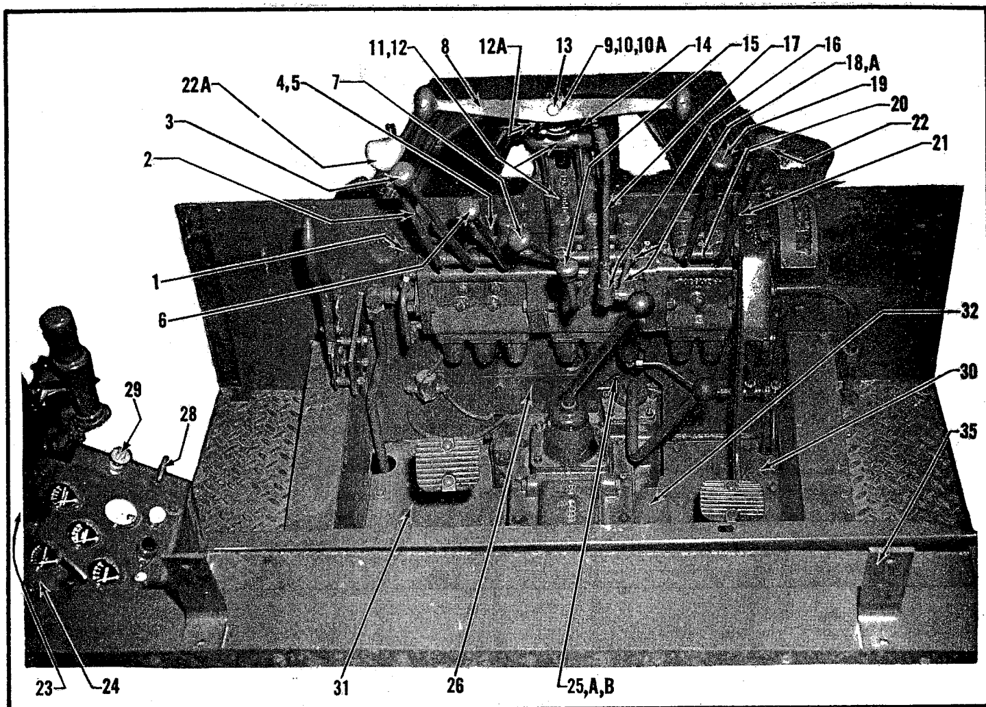
HYDRAULIC VALVE CONTROLS, SEAT, AND MISCELLANEOUS PARTS
