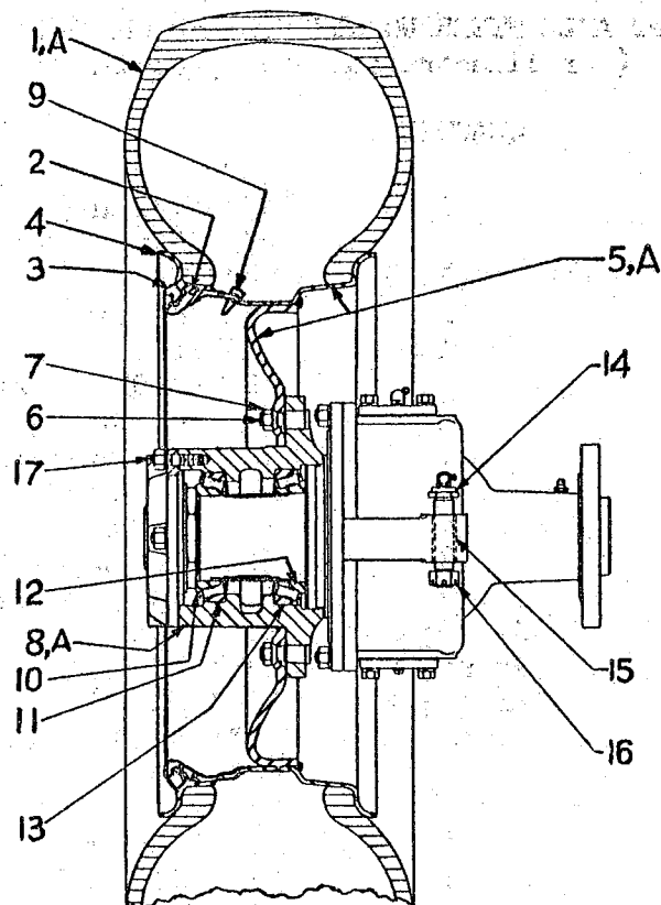
FRONT AXLE STEERING KNUCKLE, WHEEL AND TIRE (On Pacer 100 and Super 100)
