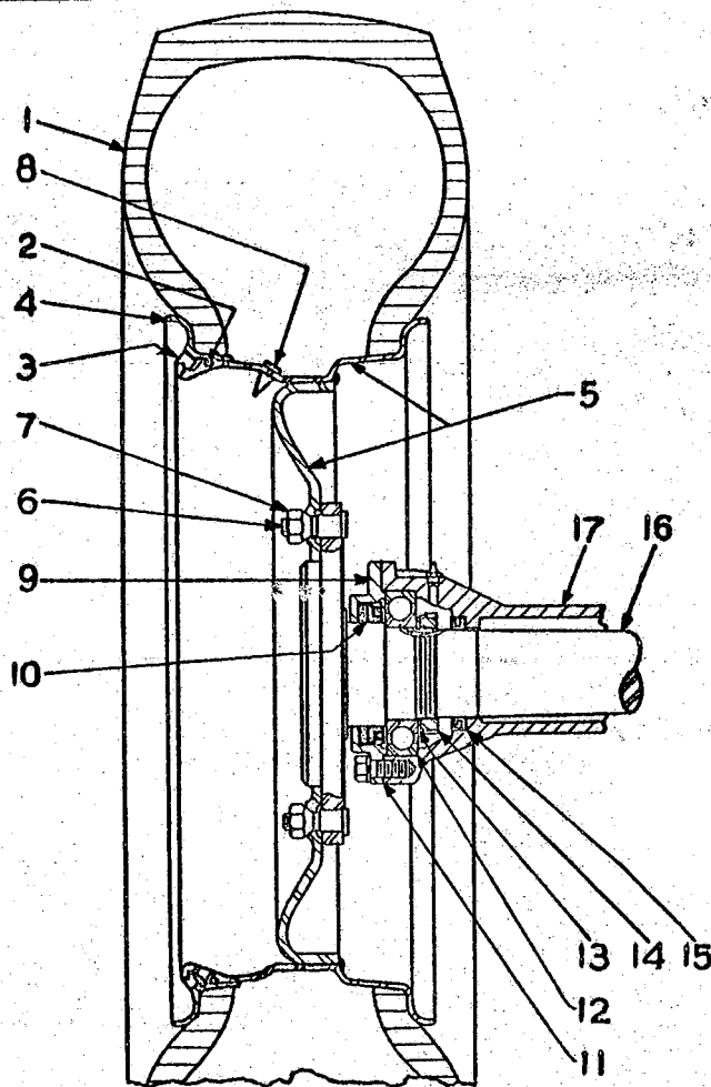
REAR AXLE HOUSING, WHEEL AND TIRE (On Pacer 100)
