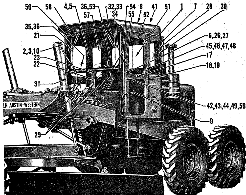
CAB - OPEN AND CLOSED TYPES
