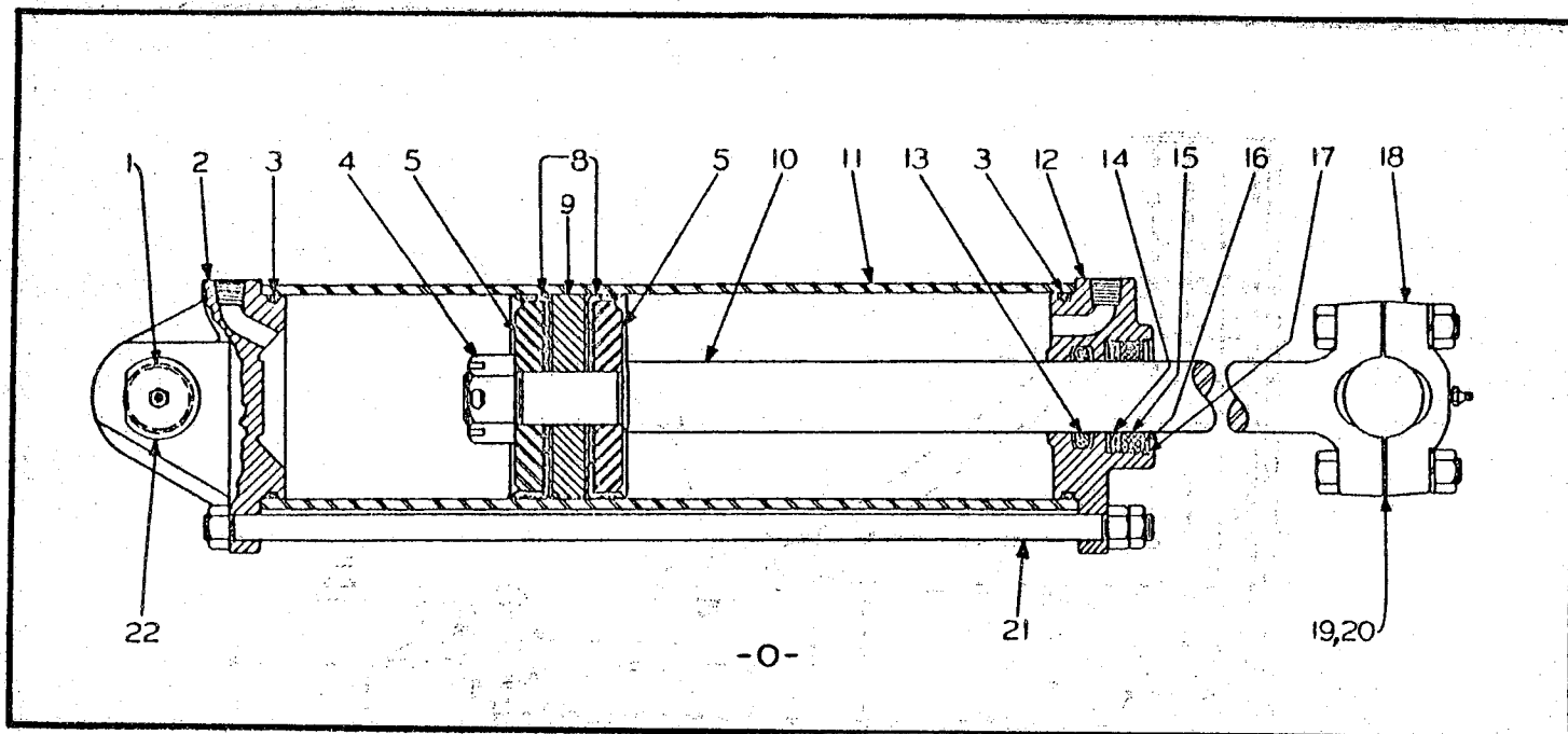
SCARIFIER RAM (Also used with Bulldozer)
