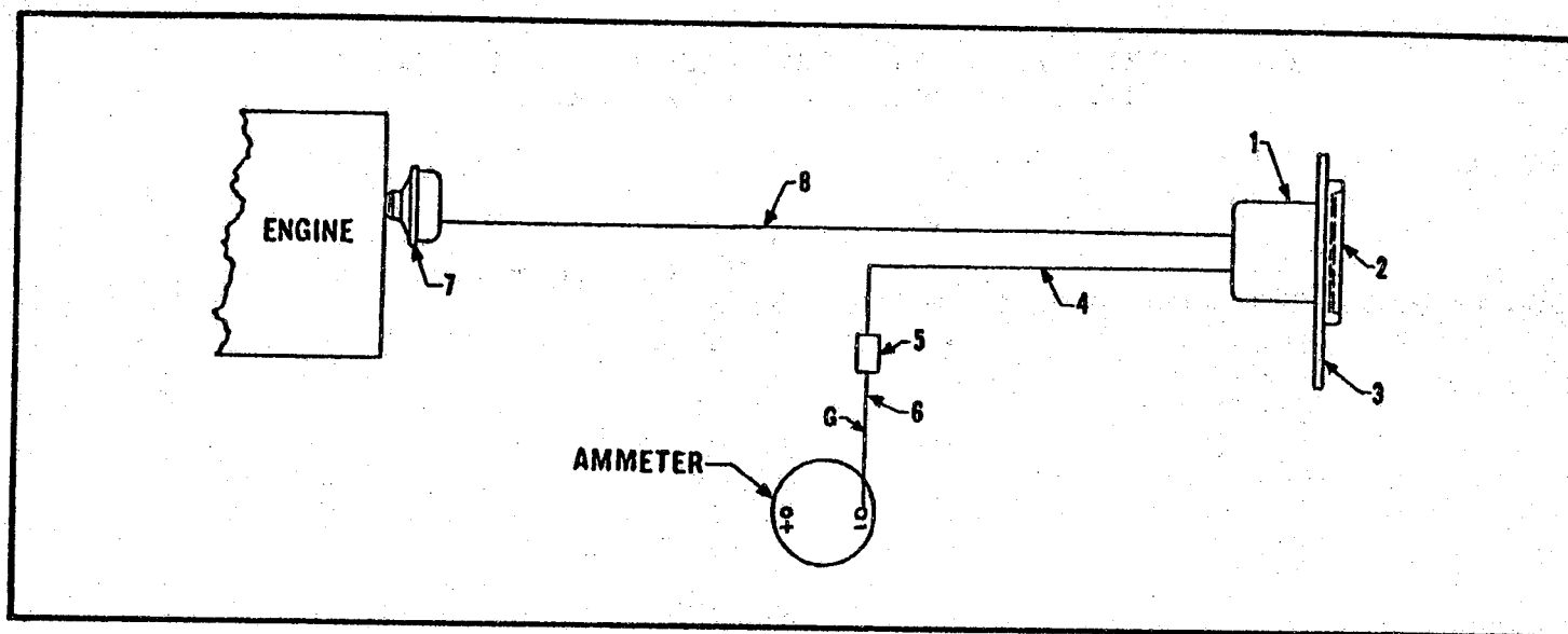
HOURLMETER FOR GMC ENGINE
