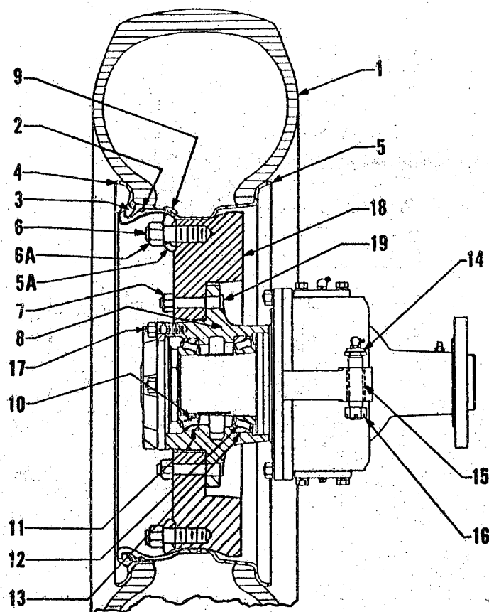
FRONT AXLE STEERING KNUCKLE, WHEEL AND TIRE (On Super 200)
