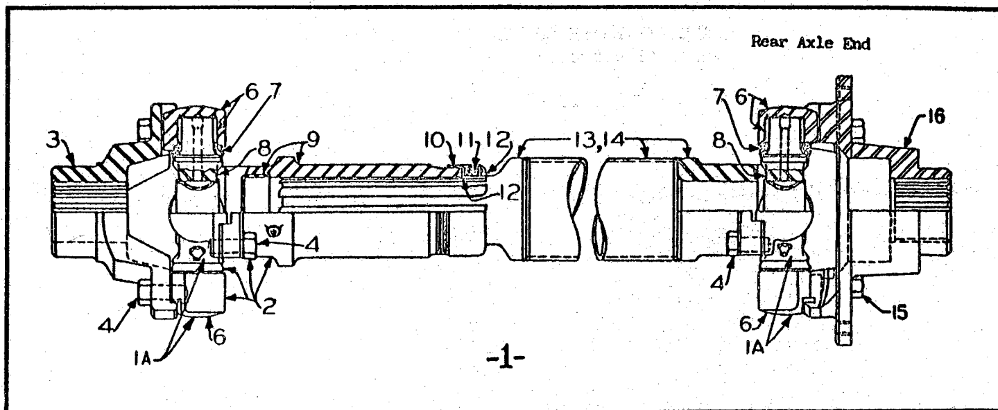
REAR PROPELLER SHAFT (From Transfer Case to Auxiliary Brake on Rear Axle Gear Carrier)
