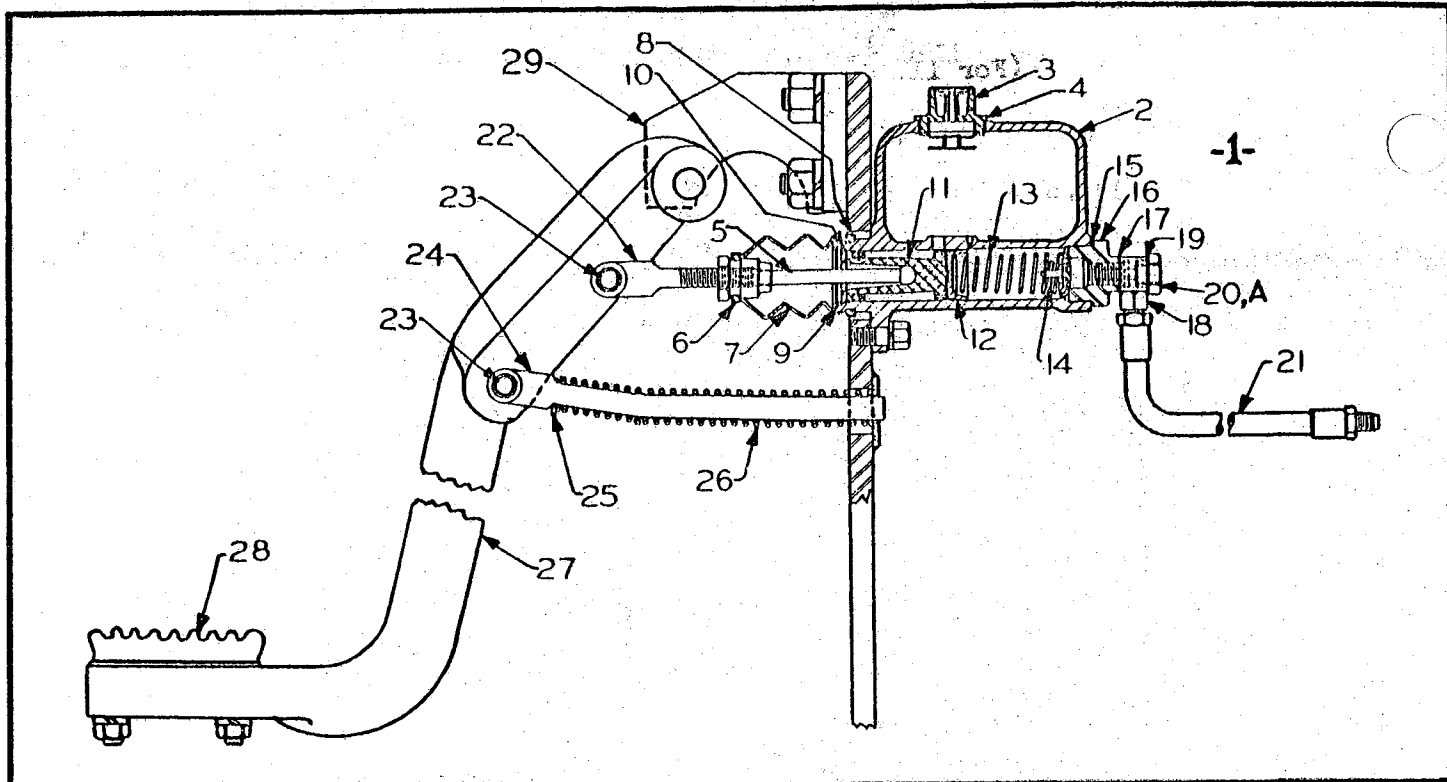
FOOT BRAKE MECHANISM (Propeller Shaft Brake)
