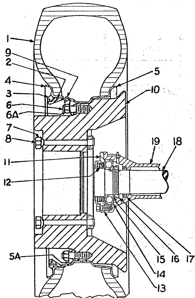
REAR AXLE HOUSING, WHEEL AND TIRE (On Pacer 200)
