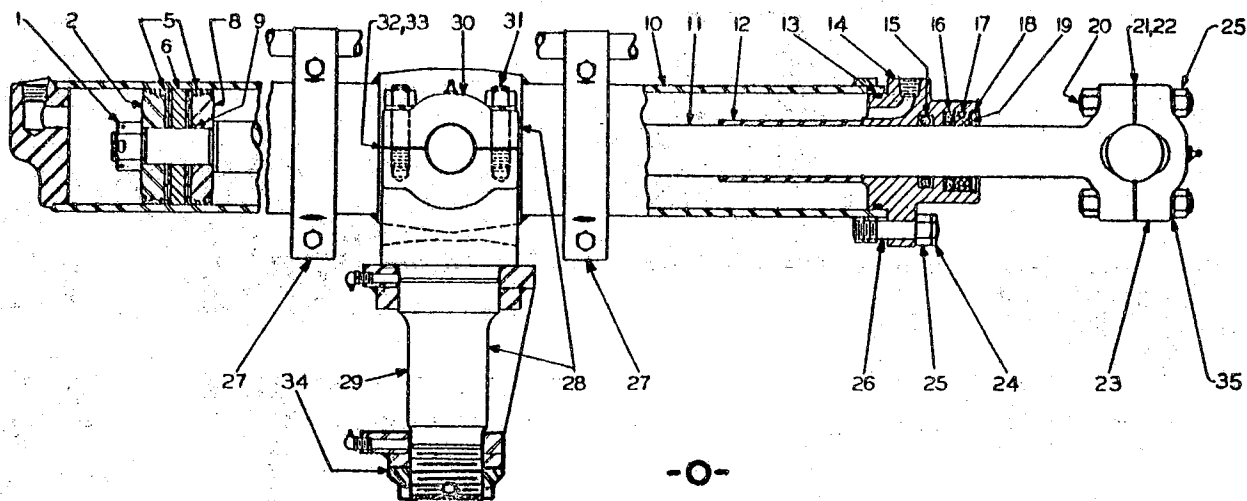
HIGH LIFT RAM
