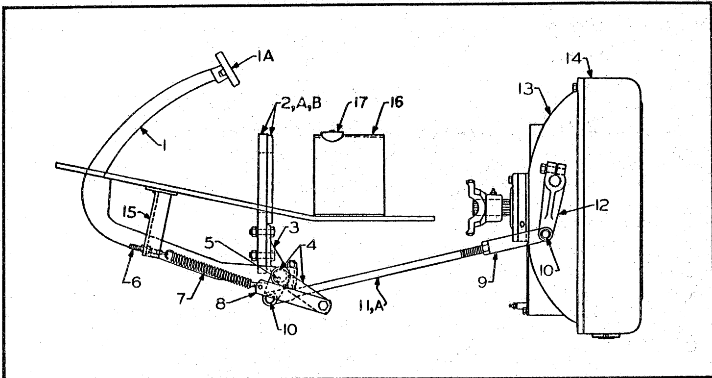
CLUTCH OPERATING MECHANISM
