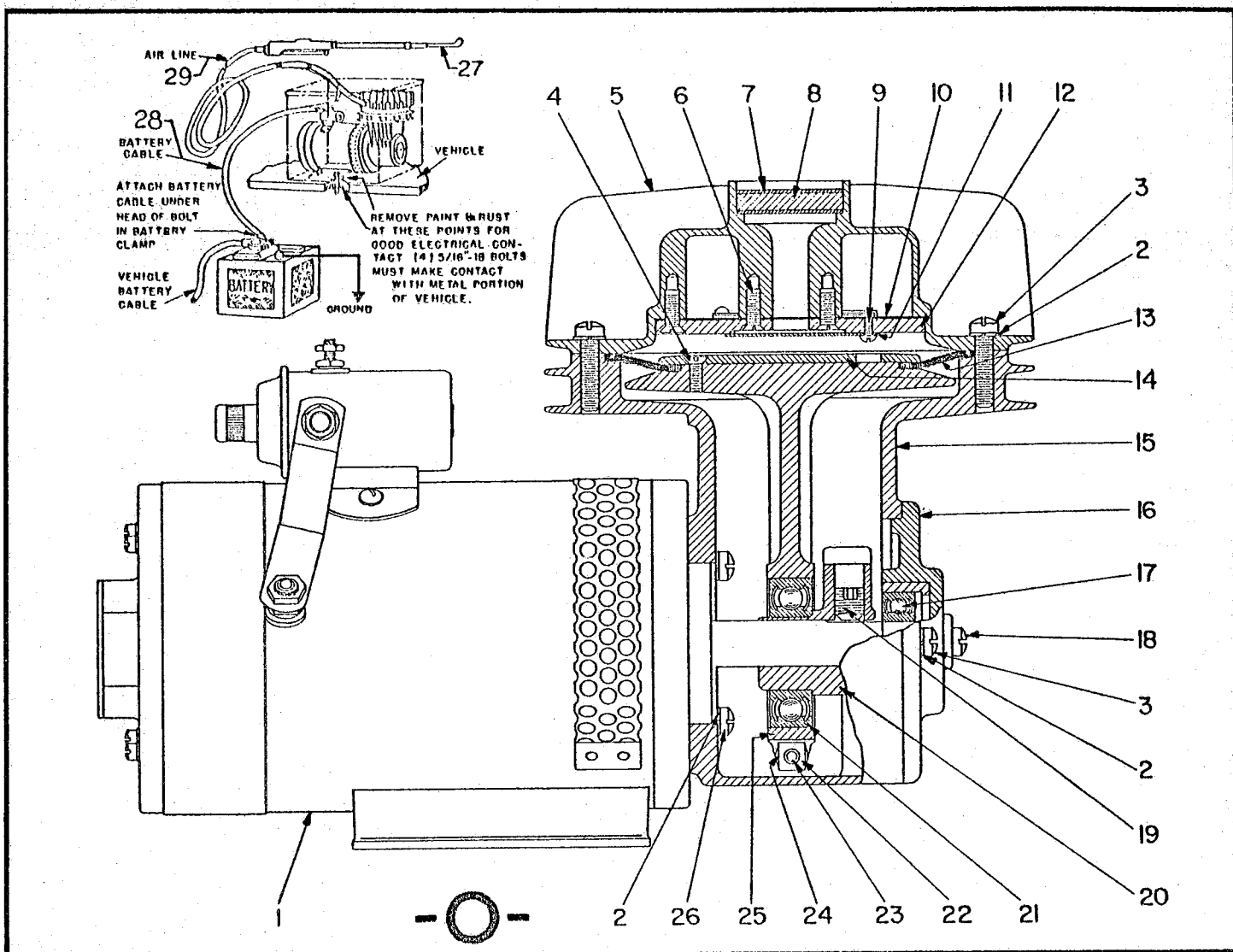
PORTABLE AIR COMPRESSOR (TIRE PUMP) - SPECIAL ORDER (12-volt Battery Operated)
