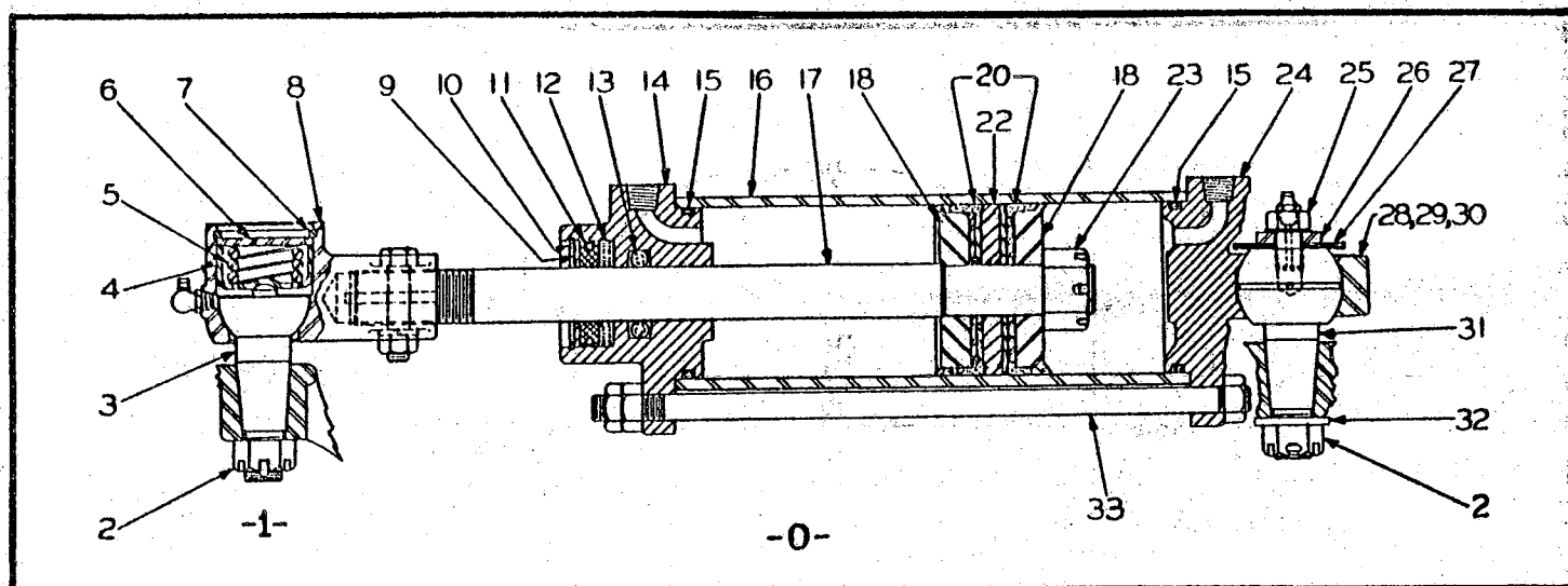
FRONT AXLE STEERING RAM
