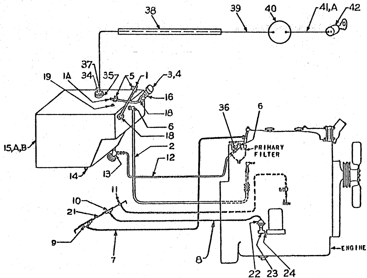
Fuel and Oil Lines
