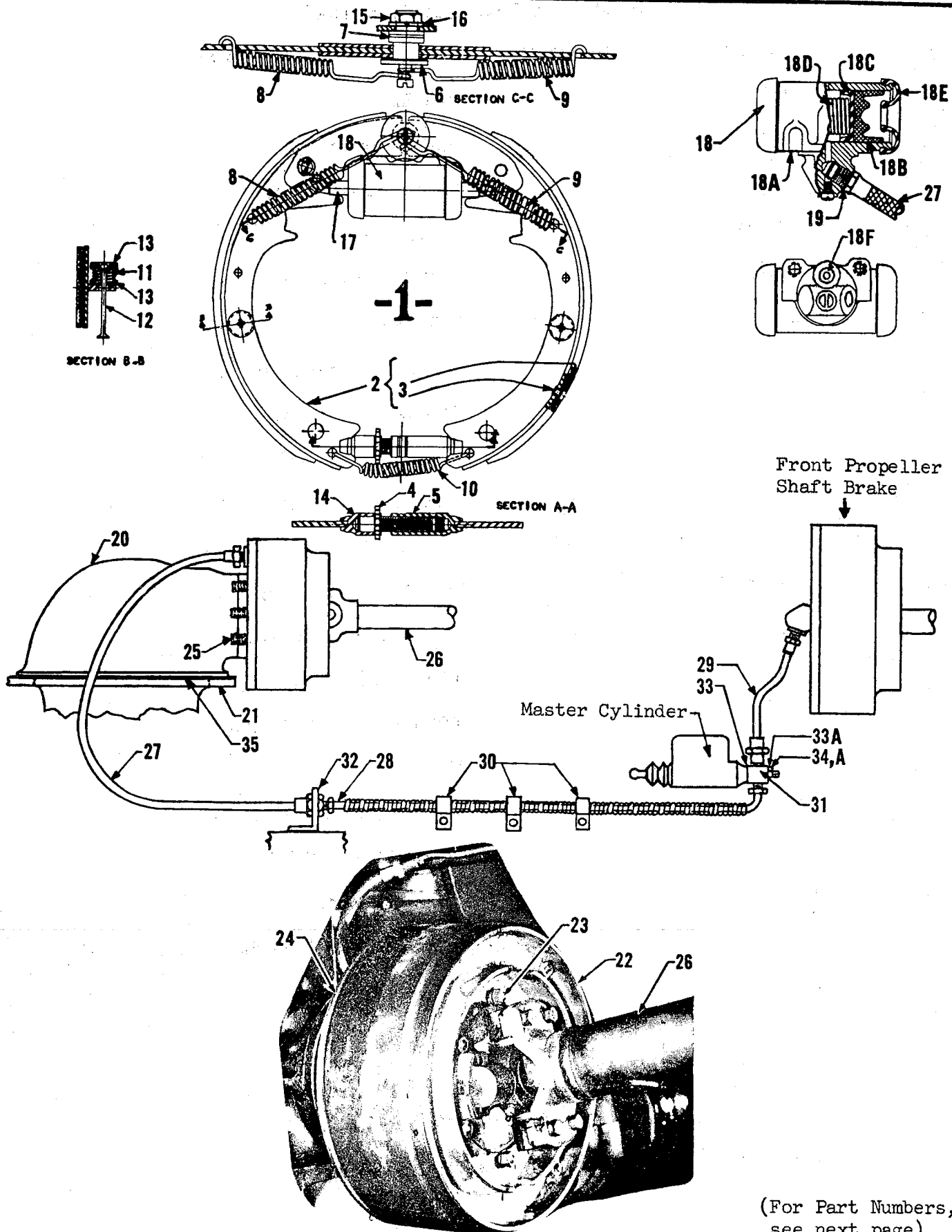
AUXILIARY BRAKE ON REAR AXLE GEAR CARRIER
