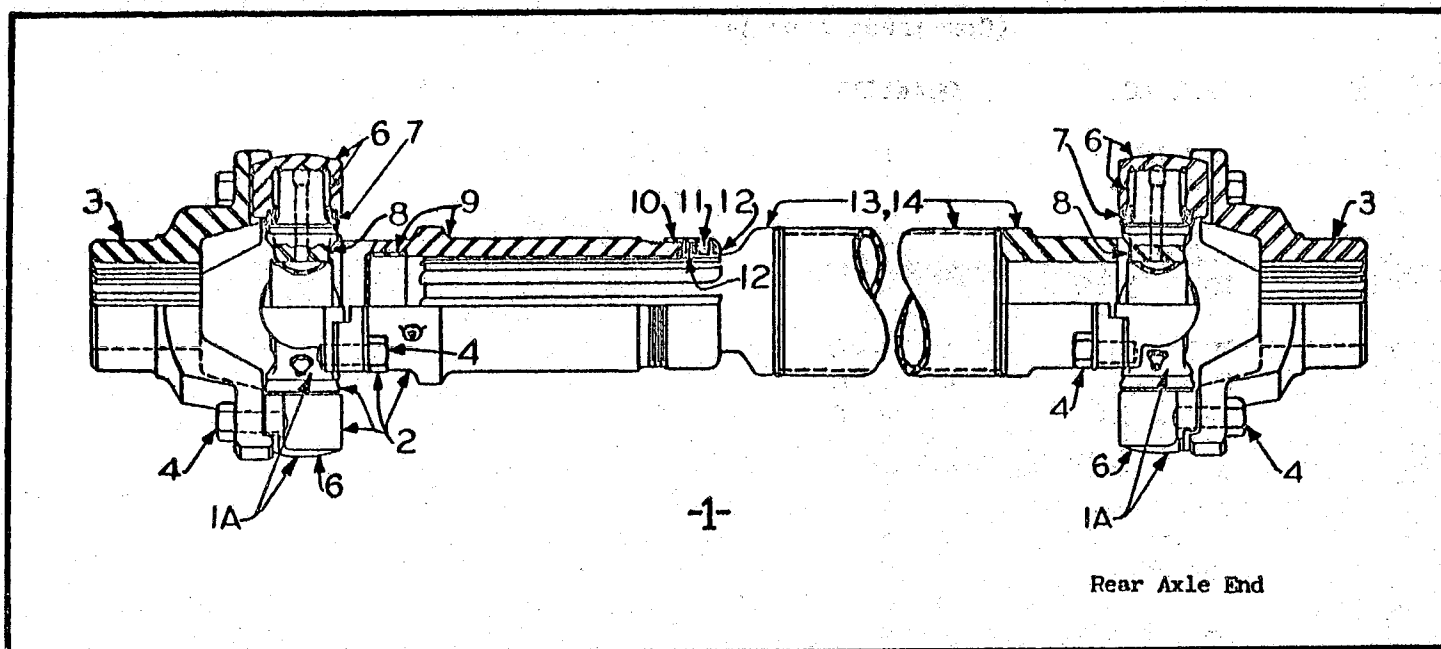
REAR PROPELLER SHAFT (From Transfer Case to Rear Axle Gear Carrier) (Superseded)
