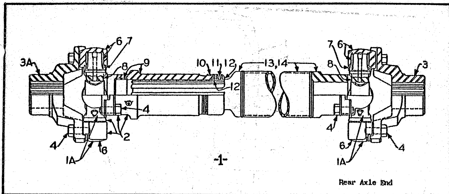
REAR PROPELLER SHAFT (From Transfer Case to Rear Axle Gear Carrier) (Machine # R-100-5476 and up)
