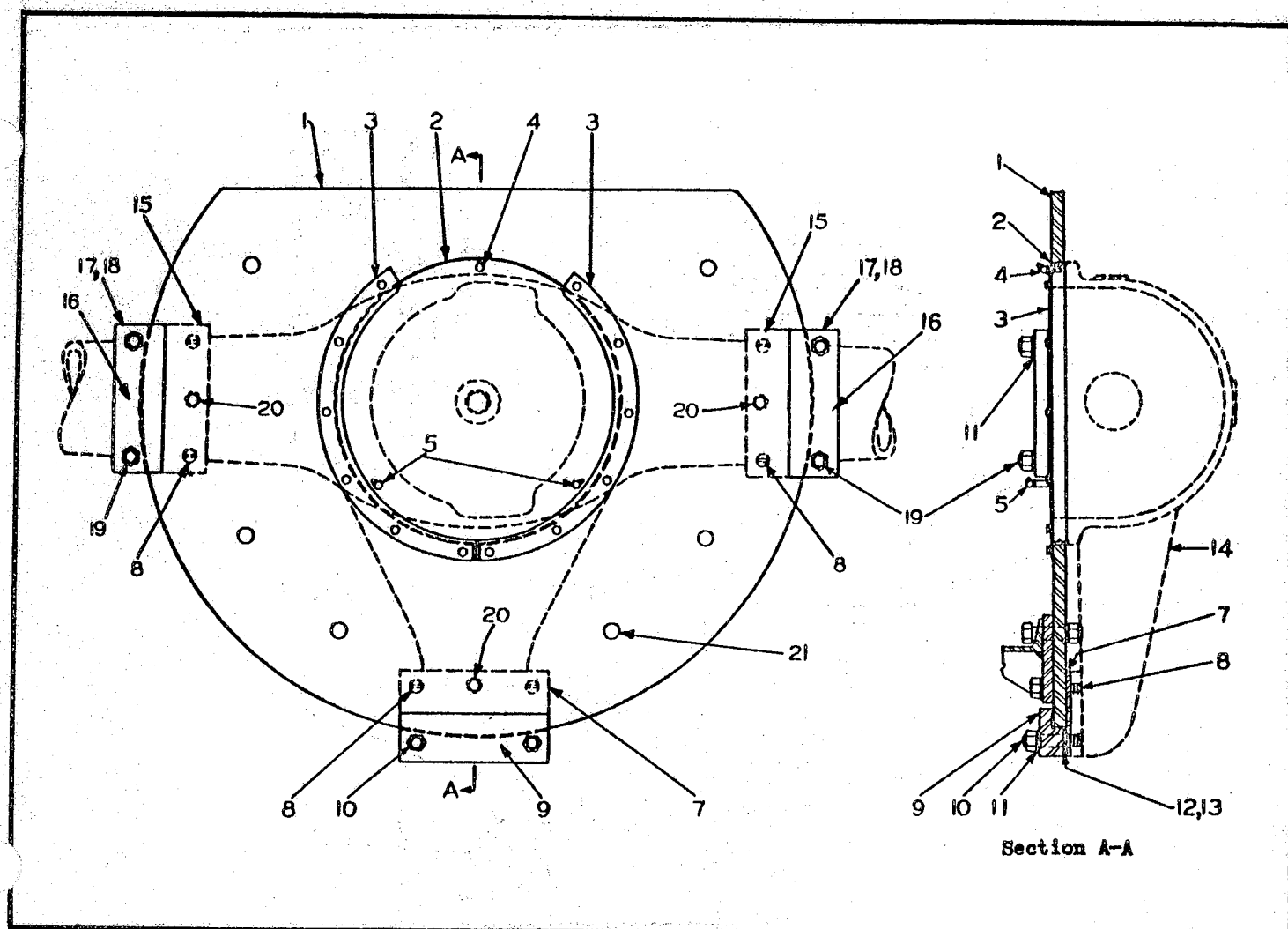
REAR AXLE CIRCLE (On Super Graders)
