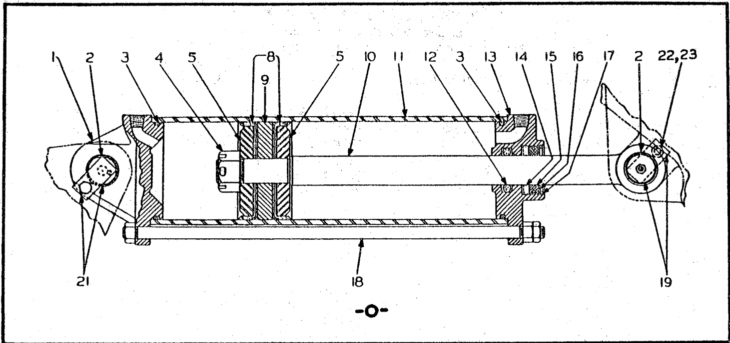
REAR AXLE STEERING RAM (On Pacer 100 - 200)
