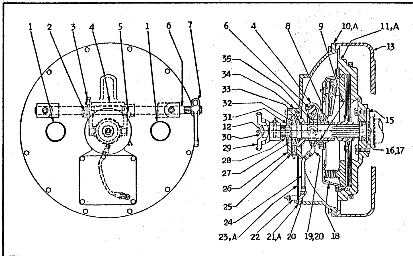
CLUTCH AND SHAFT ASSEMBLY (Dry Clutch or Torque Converter Drive)
