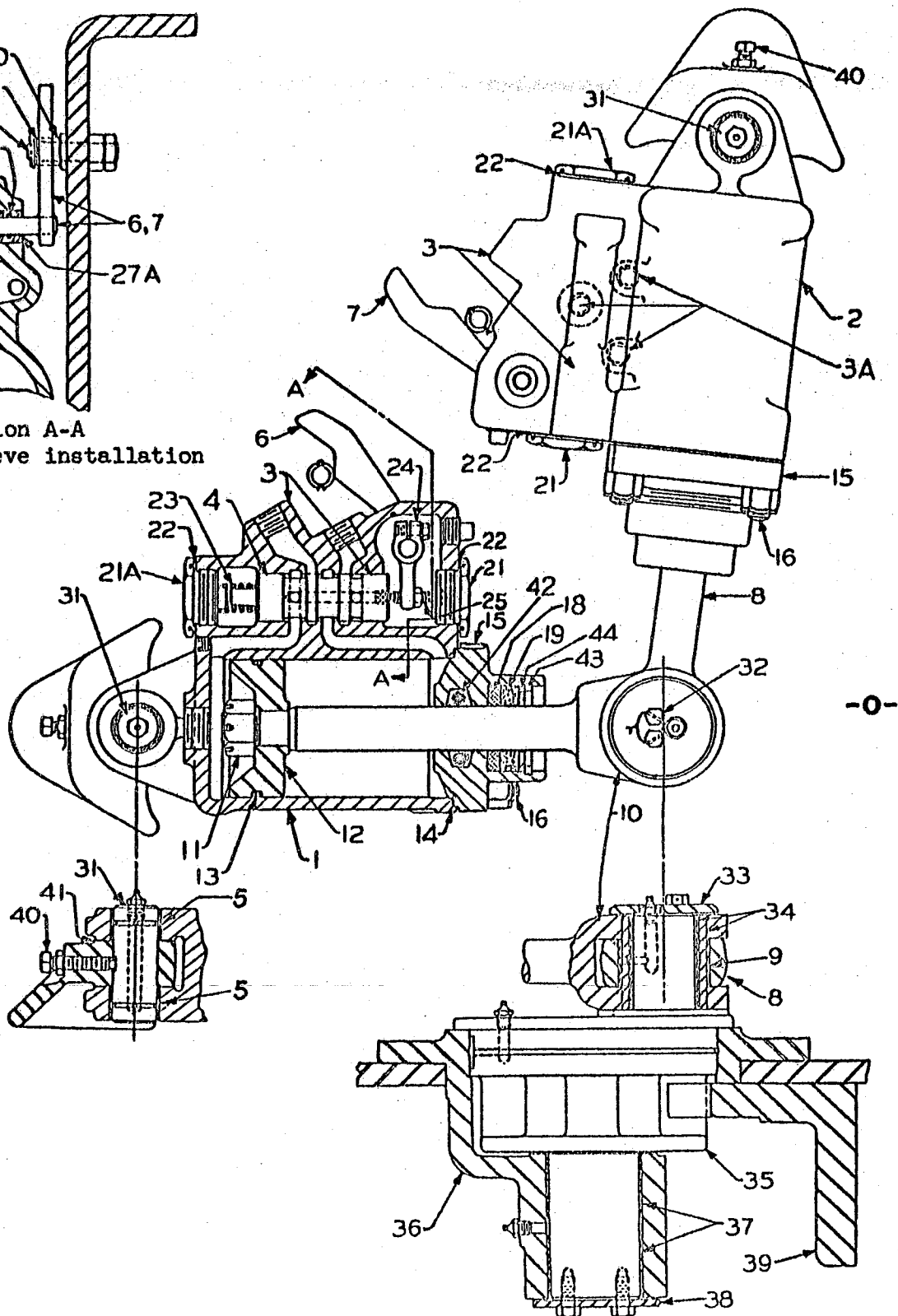
CIRCLE REVERSE HYDRAULIC MOTOR (For Full Reversing Circle)
