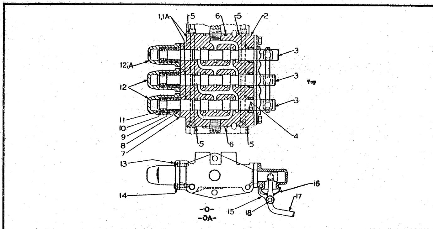
HYDRAULIC CONTROL TRIPLE VALVE
