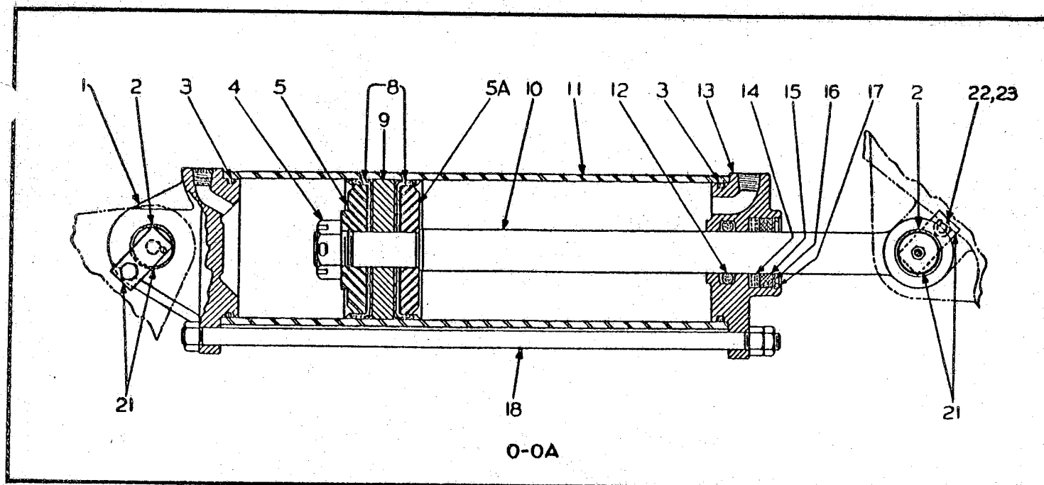
REAR AXLE STEERING RAM (On Super 100 - 200)
