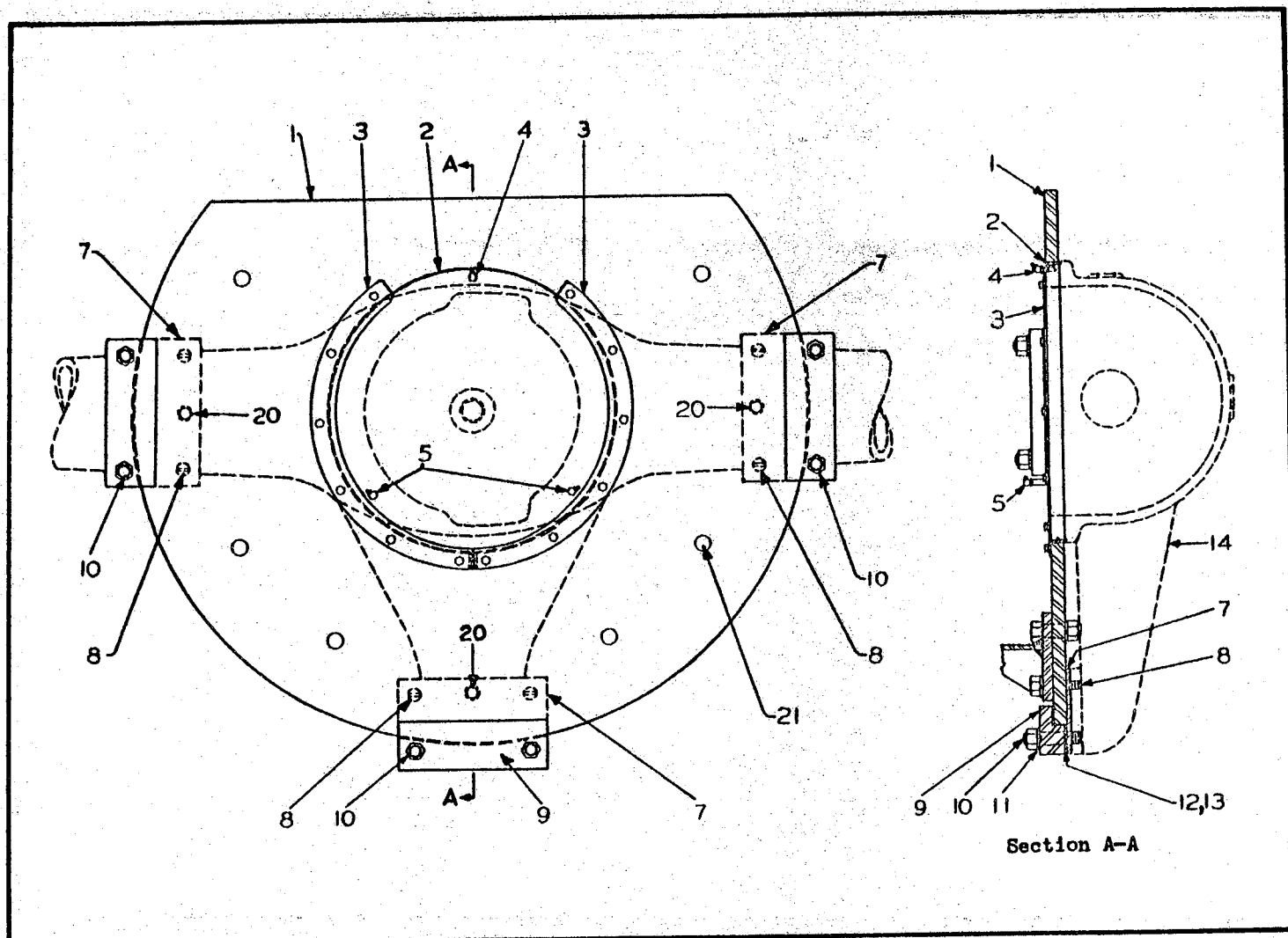
REAR AXLE CIRCLE (On Pacer Graders)
