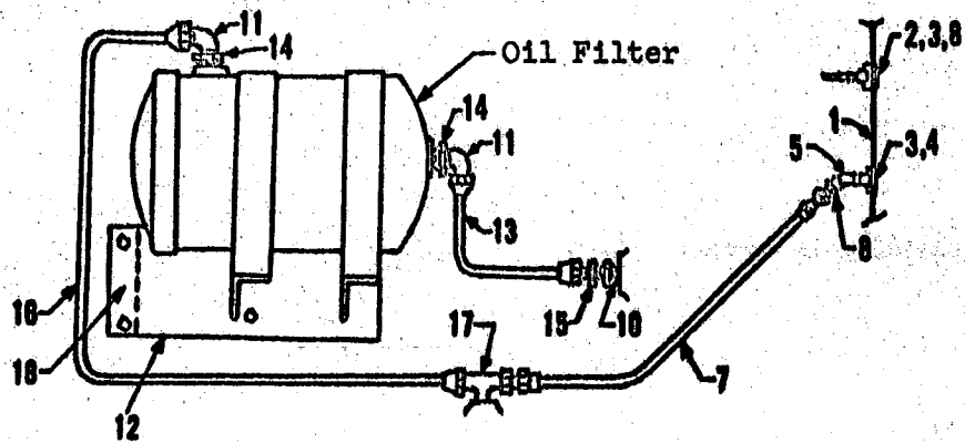
Oil Pressure Lines
