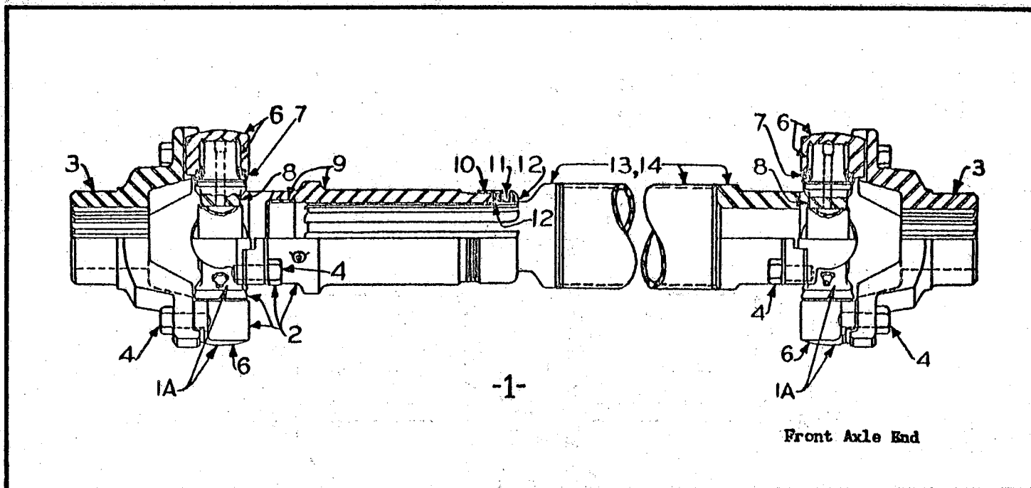
FRONT SECTION OF FRONT PROPELLER SHAFT
