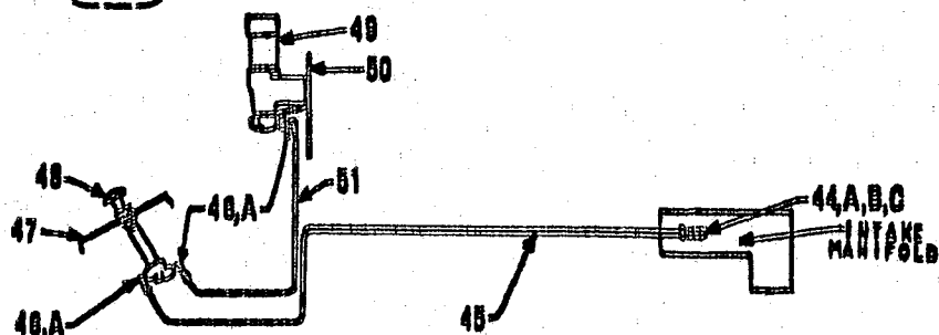
Ether Starting System
