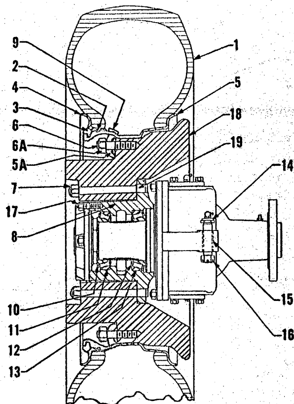
FRONT AXLE STEERING KNUCKLE, WHEEL AND TIRE (On Pacer 200)
