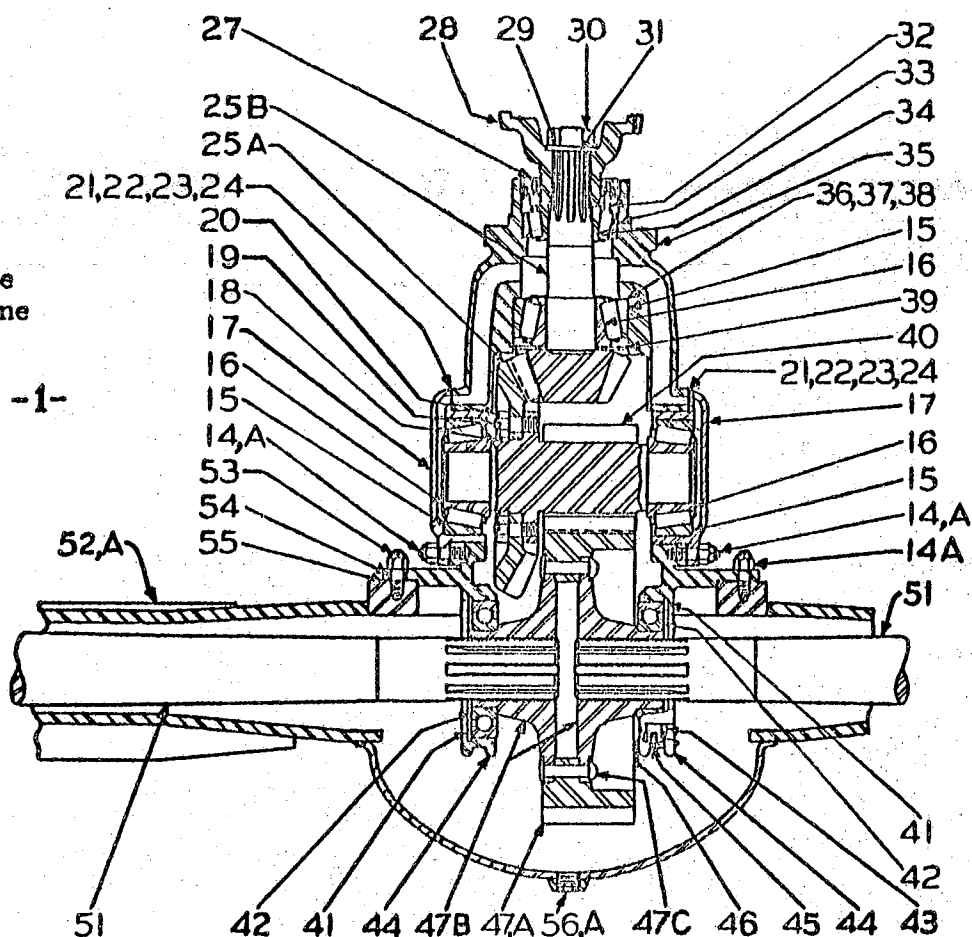
REAR AXLE GEAR CARRIER
