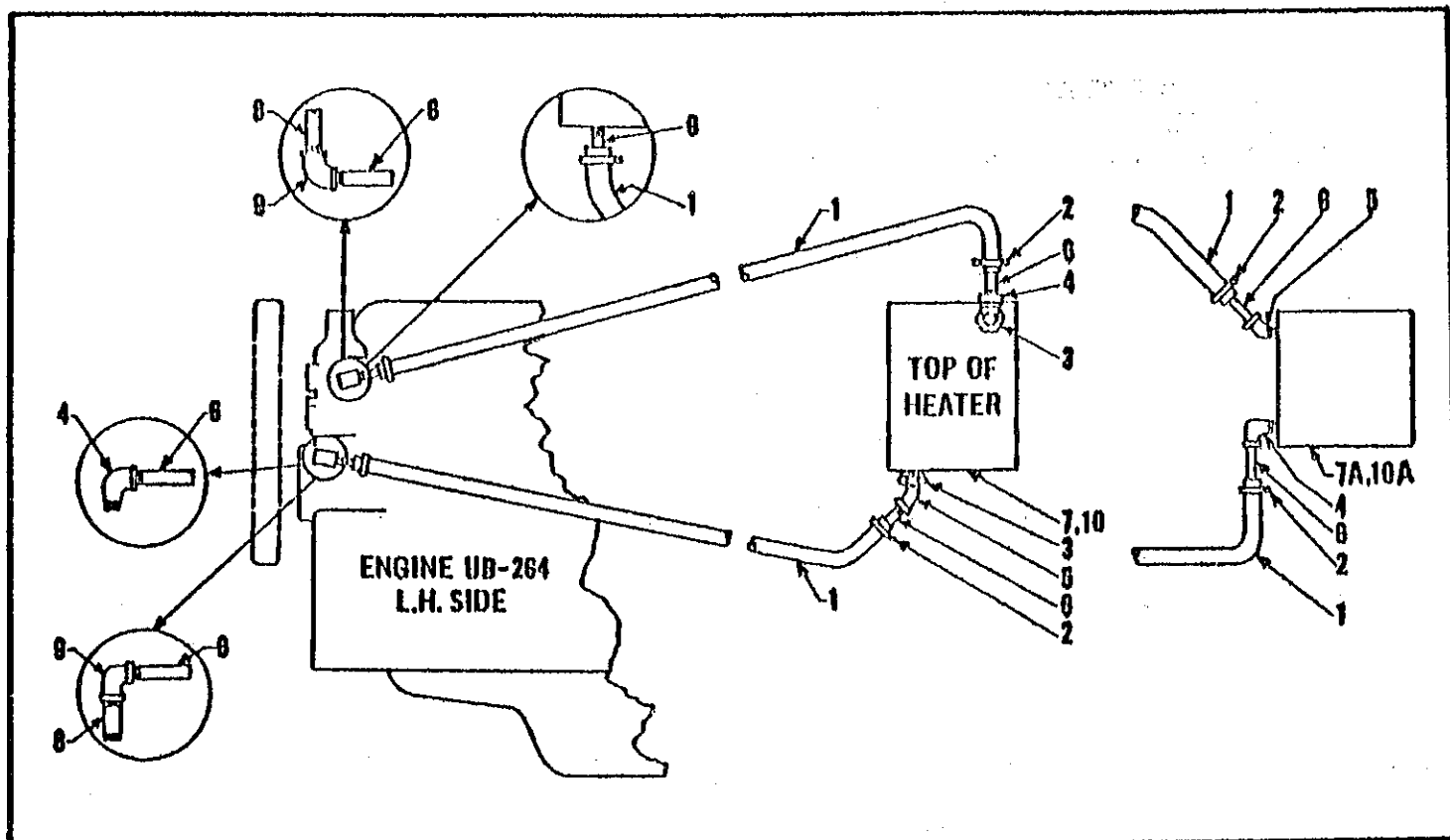
HEATER PIPING DIAGRAM (For IHCo. - UB-264 Engine)
