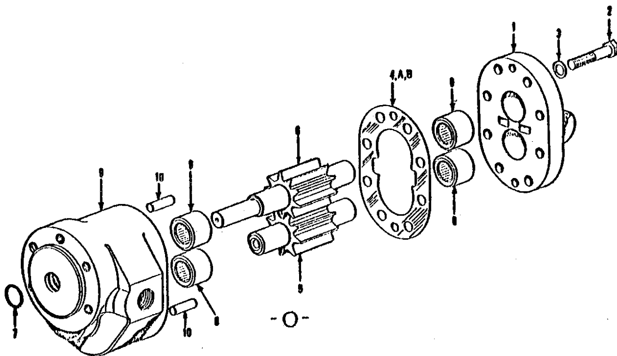
BOOM SWING HYDRAULIC MOTOR
