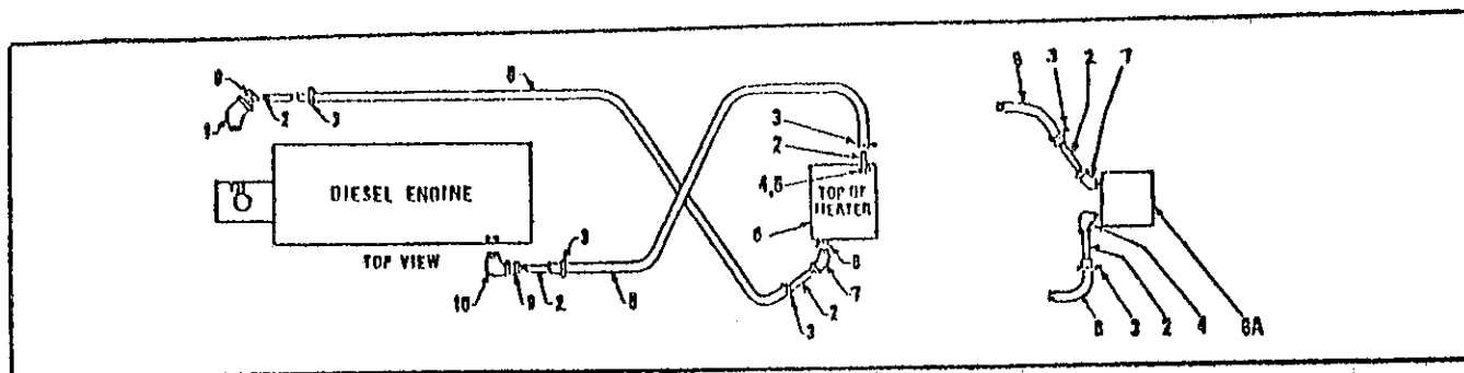
HEATER PIPING DIAGRAM (For GMC-3-71 Engine)
