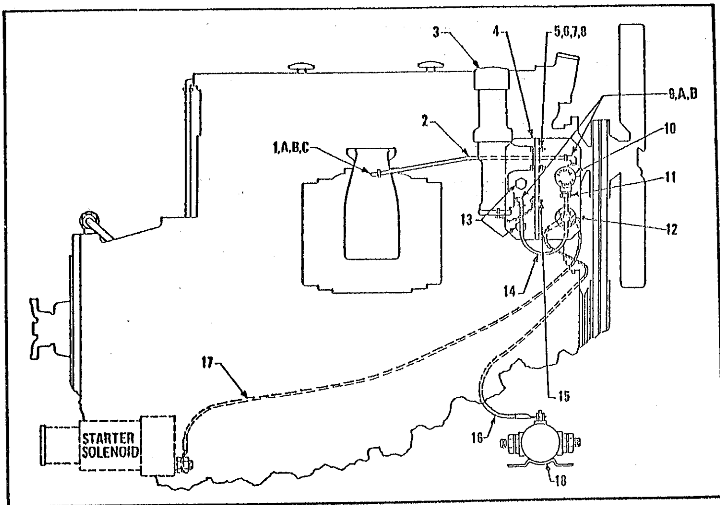
ETHER STARTING SYSTEM (For GMC-3-71 Engine)
