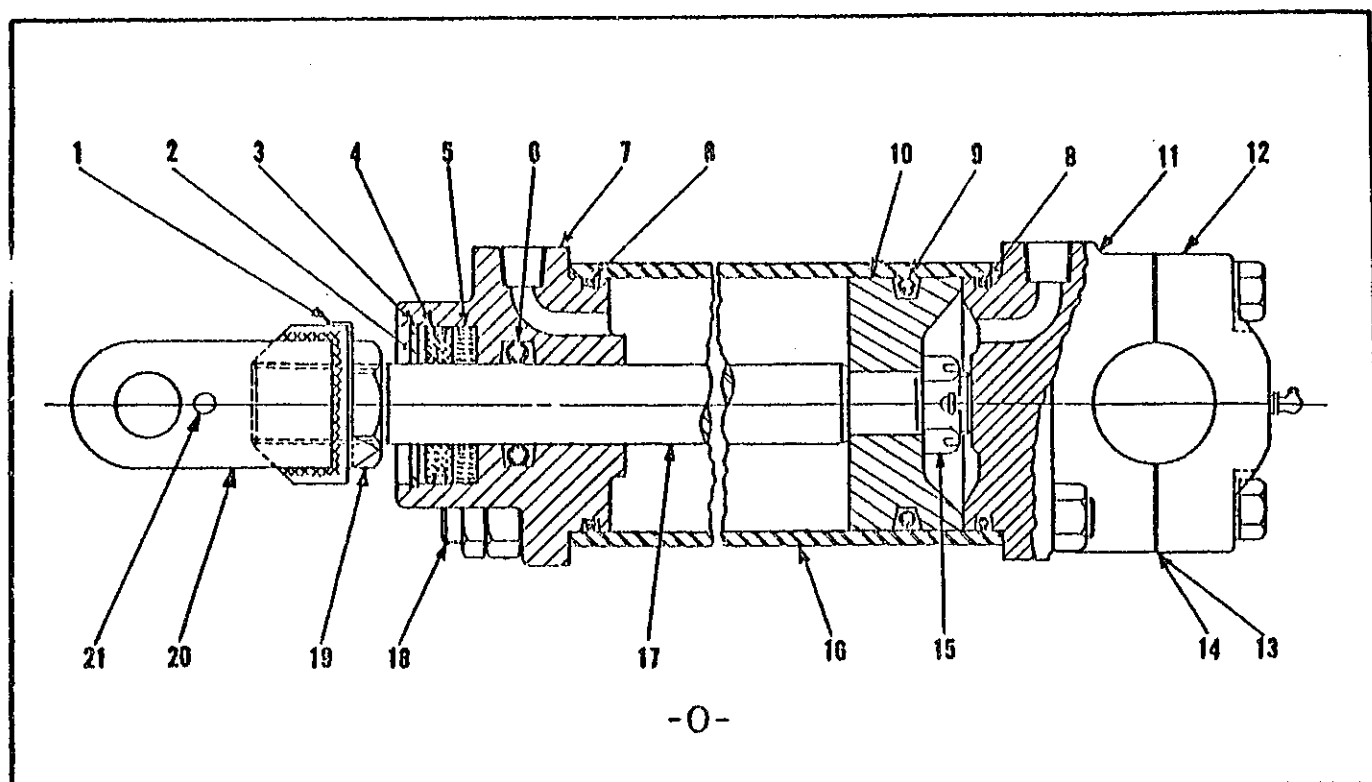
REAR AXLE STEERING RAM (O-RING TYPE PISTON) (Driving Rear Axle)
