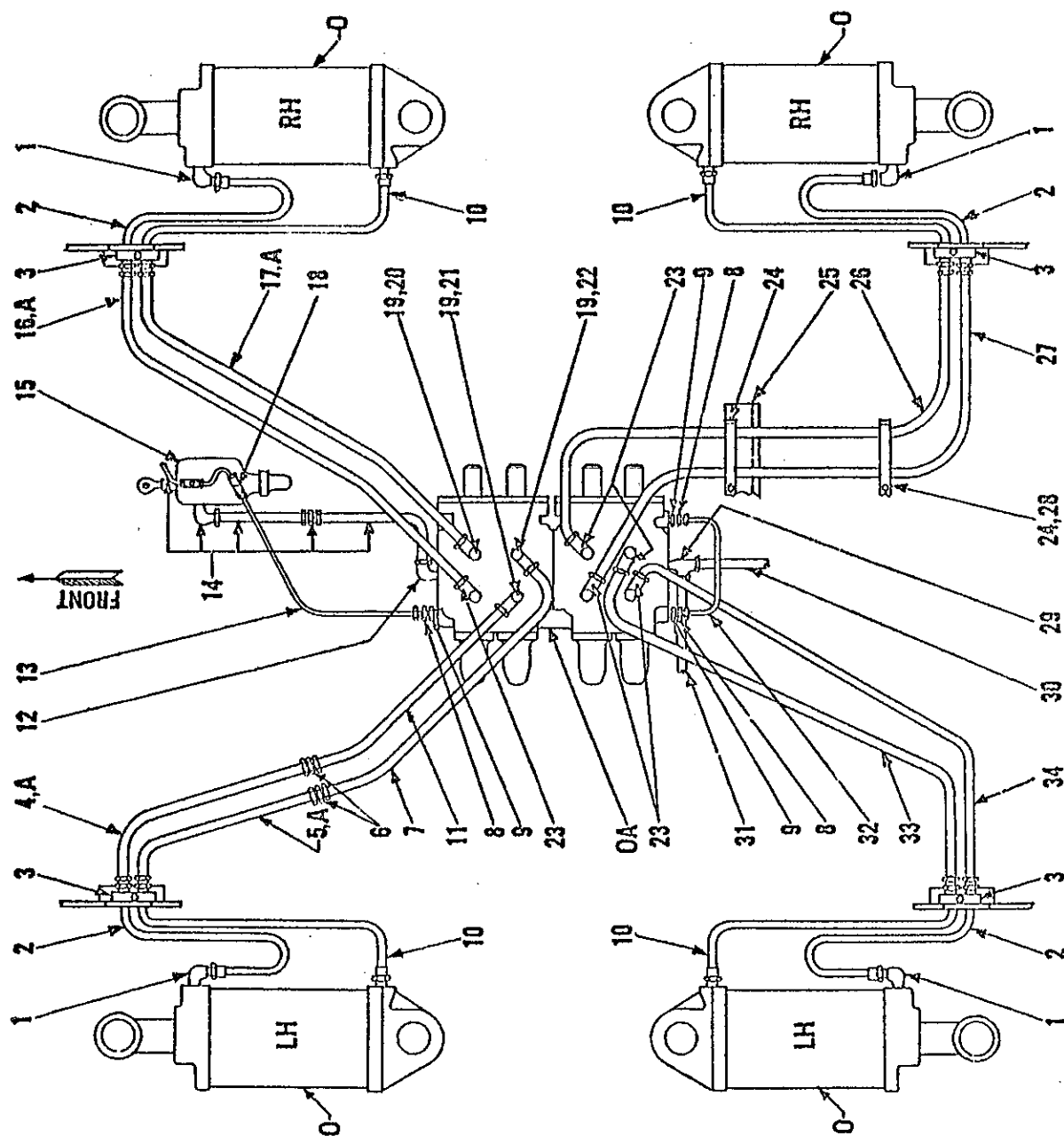
HYDRAULIC OUTRIGGERS HYDRAULIC PIPING DIAGRAM
