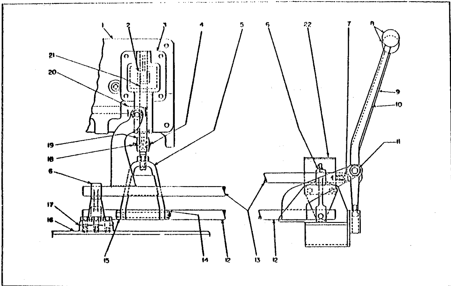
TRANSMISSION SHIFT MECHANISM
