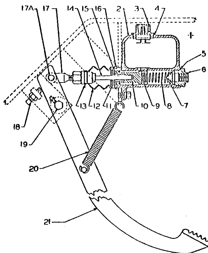
FOOT BRAKE MECHANISM
