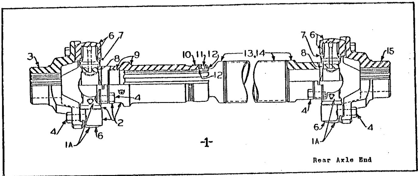
REAR AXLE PROPELLER SHAFT (4-WHEEL DRIVE) (used with either Single or Two Speed Transfer Case)
