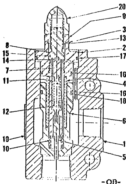
CRANE HYDRAULIC MAIN RELIEF VALVE
