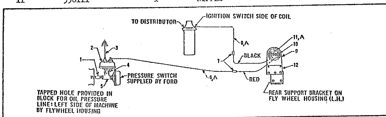
HOURMETER WIRING DIAGRAM (For Ford 332 Engine)
