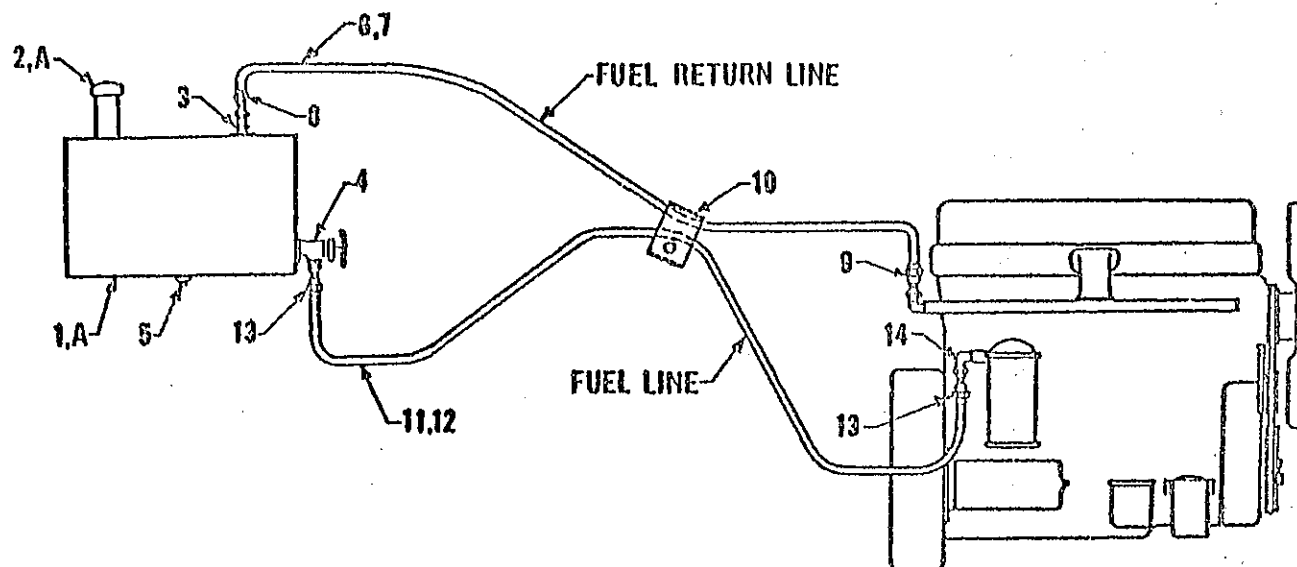
FUEL SYSTEM (FOR GMC-3-71 ENGINE)
