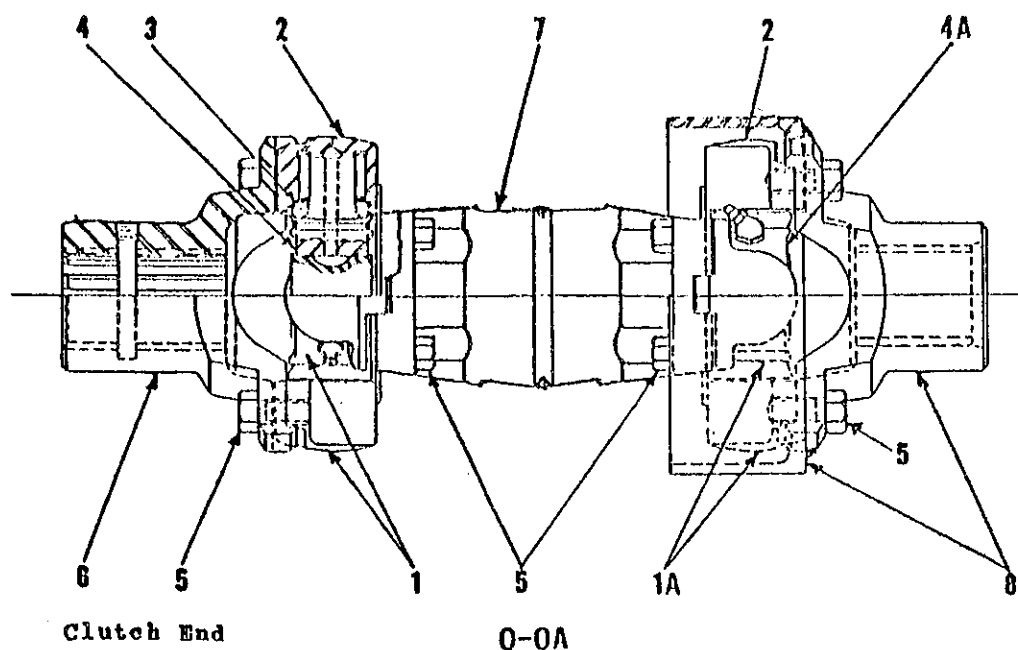
PROPELLER SHAFT - CLUTCH TO TRANSMISSION
