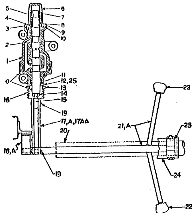
REAR AXLE STEERING VALVE AND CONTROLS
