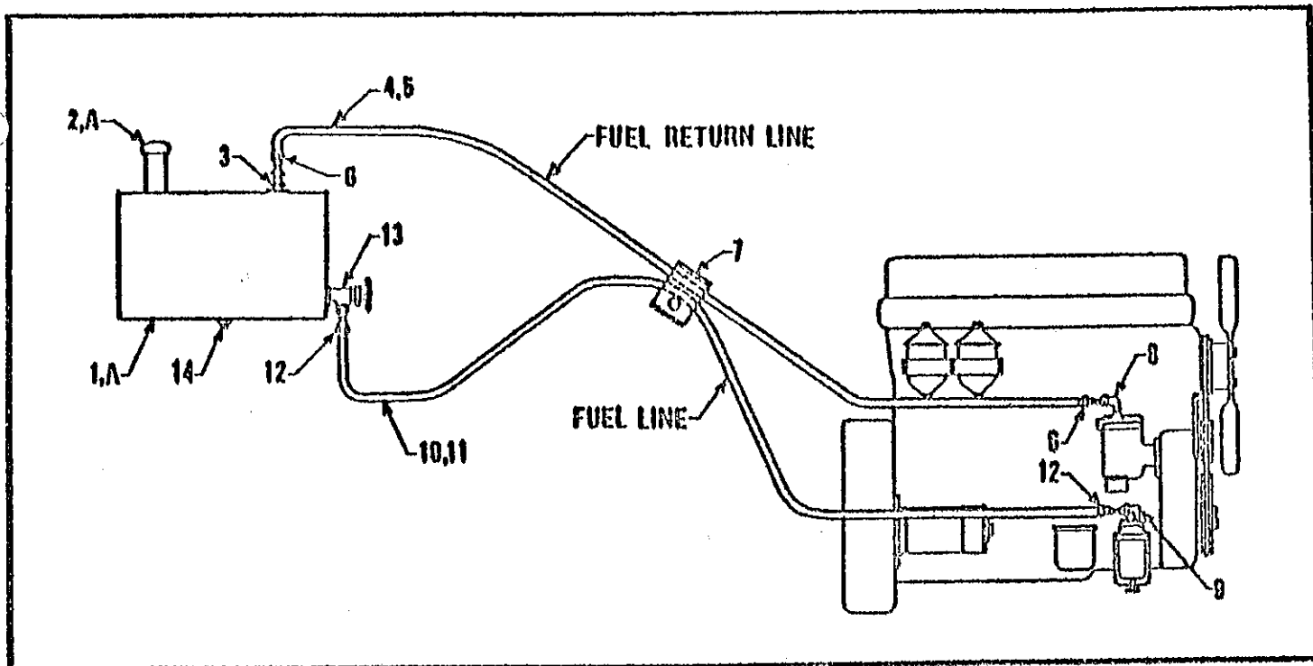
FUEL SYSTEM (For IHCo. - UD-282 and UDT-282 Engines)
