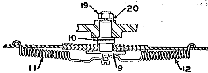
Section C-C
