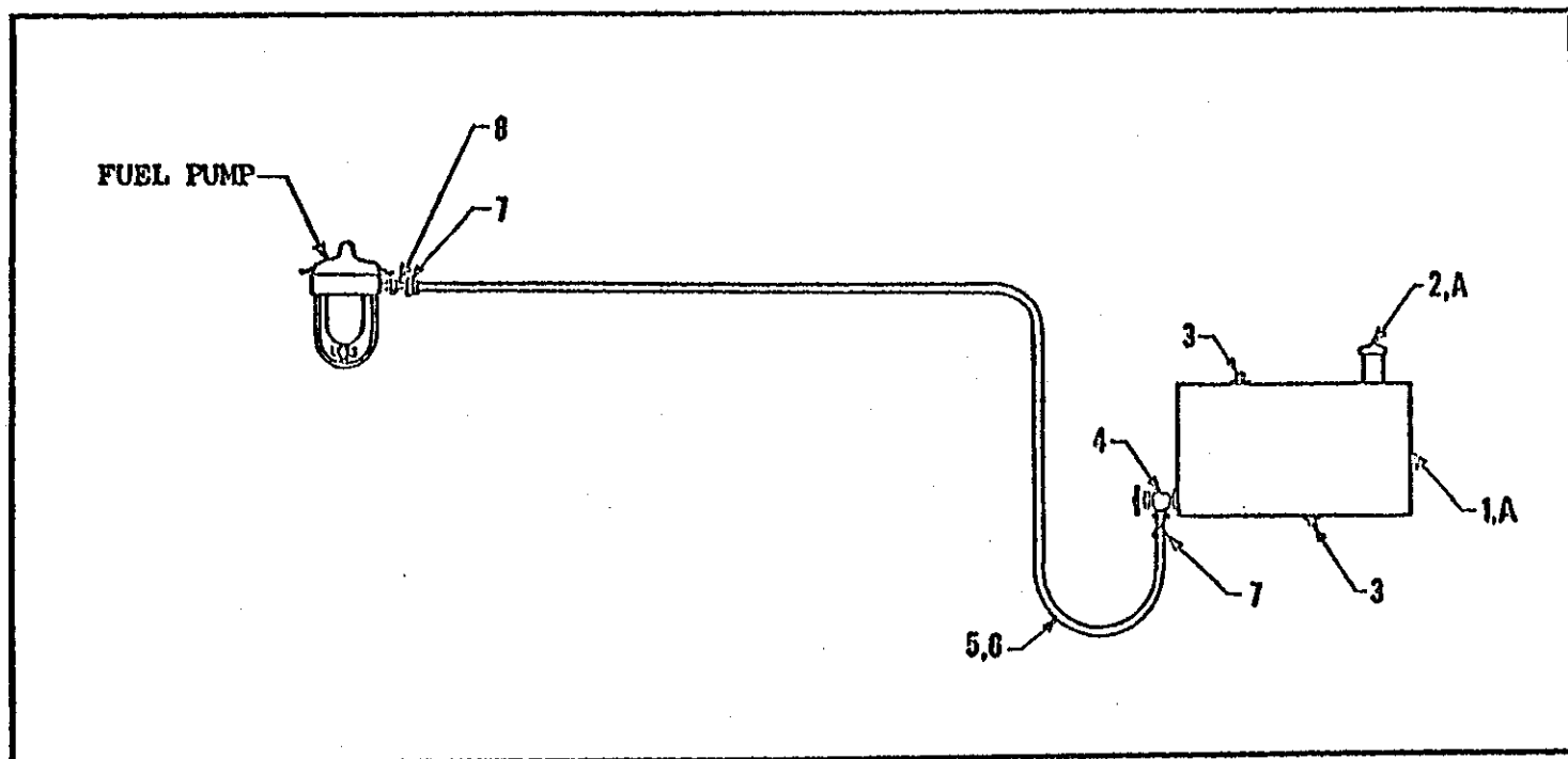
FUEL SYSTEM (For IHC Co. - UB-264 Engine)
