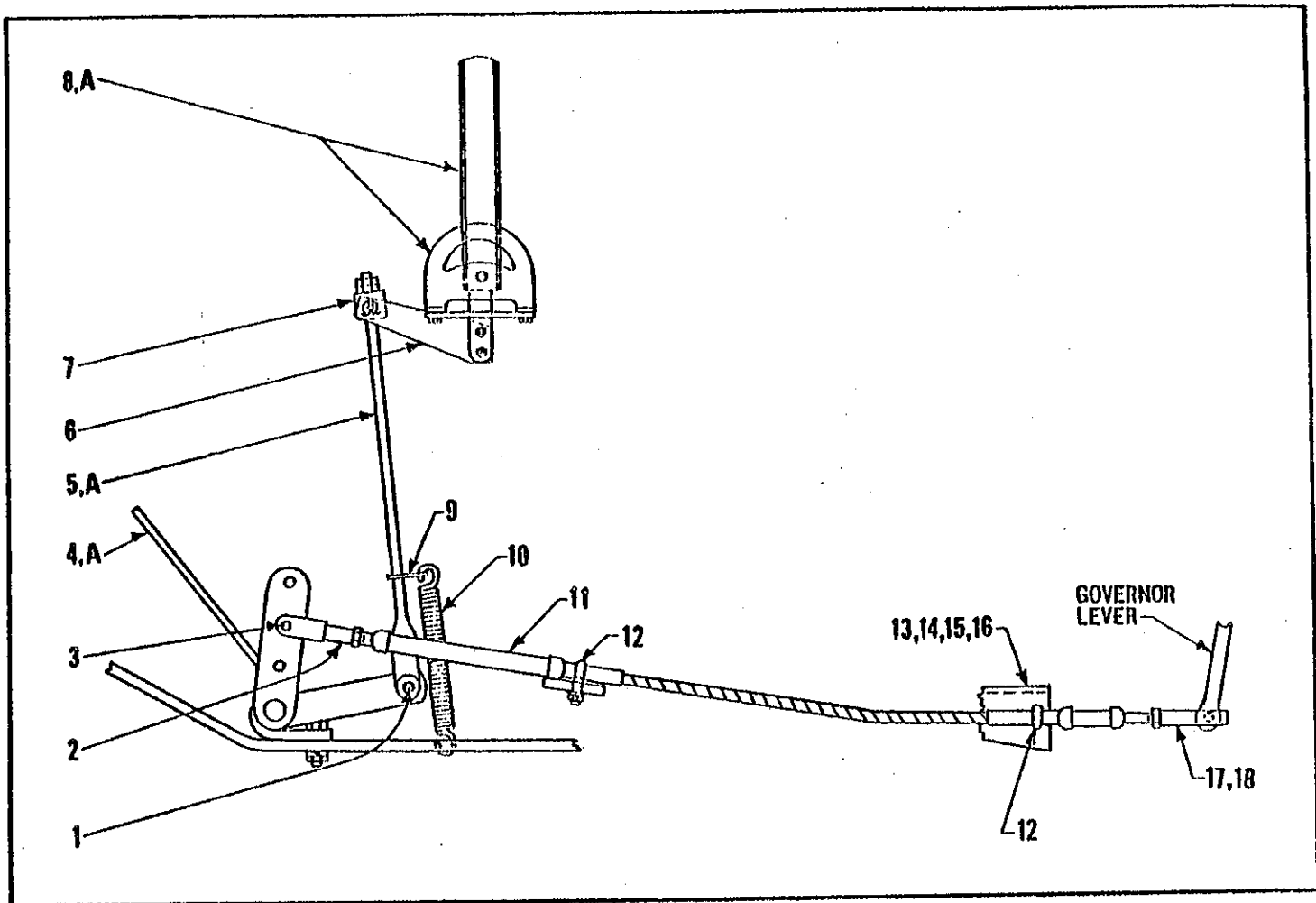
FOOT AND HAND THROTTLE CONTROL
