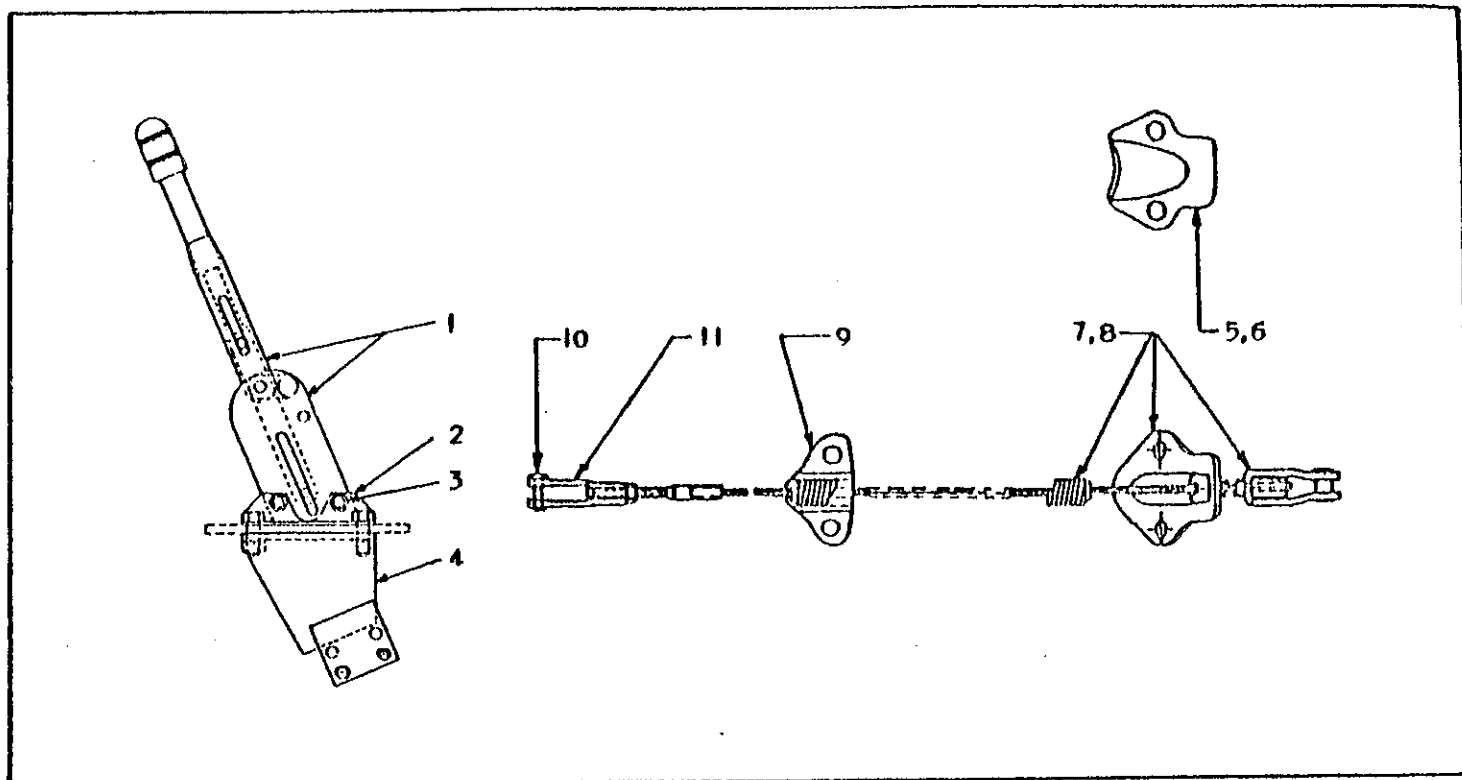
HAND BRAKE MECHANISM
