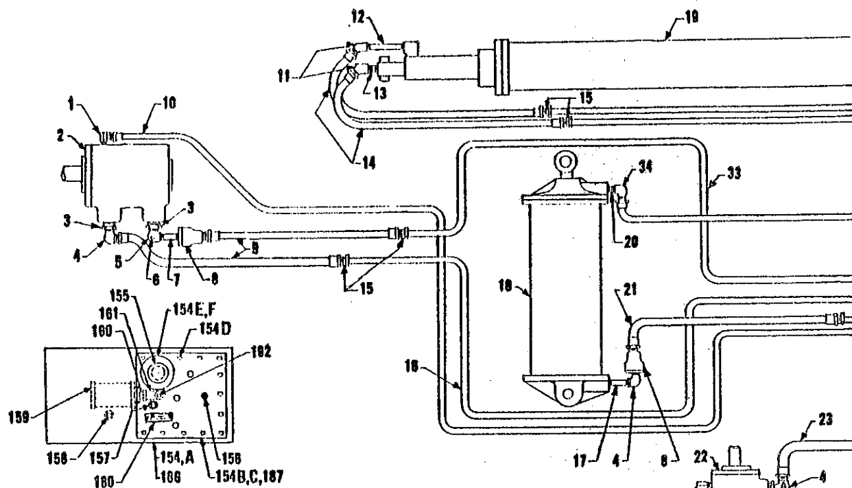
AUXILIARY TOP VIEW OF HYD. OIL TANK
