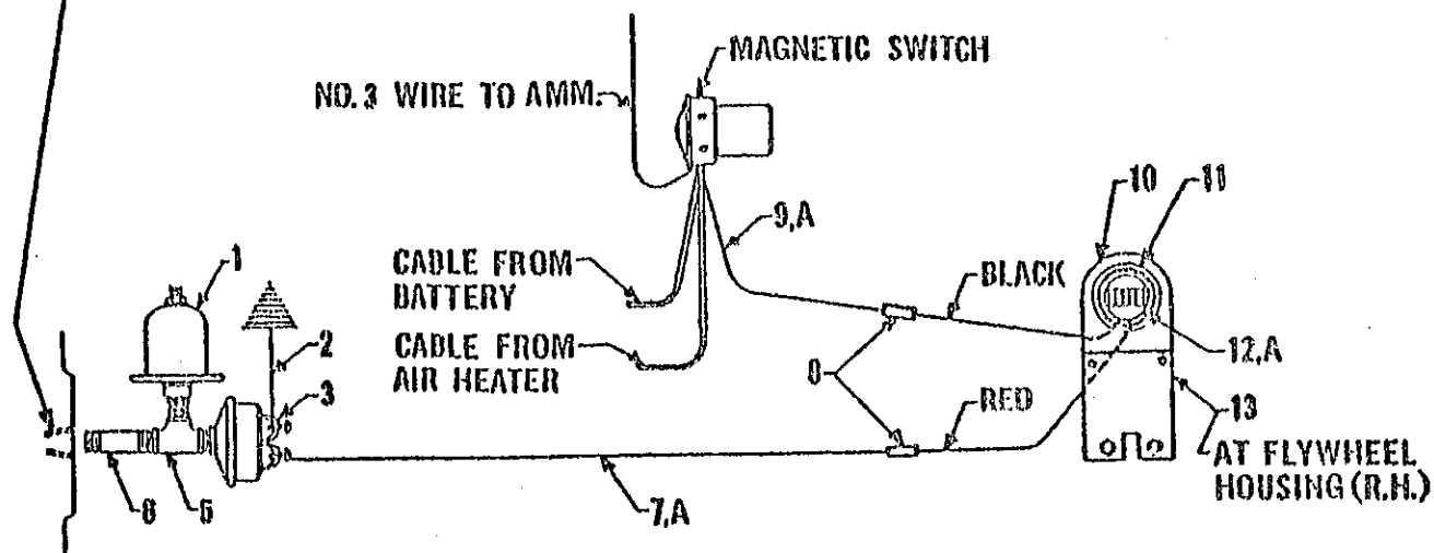
HOURLMETER WIRING DIAGRAM (For IHC Co. - UB-264 Engine)
