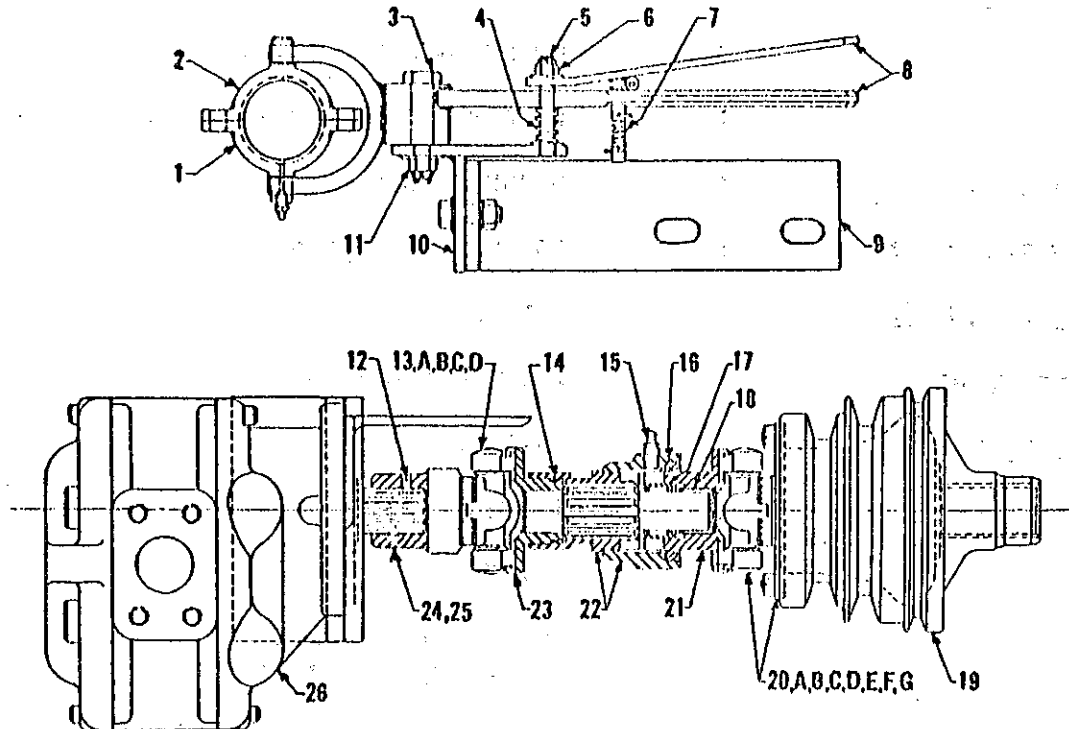
PROPELLER SHAFT - DISCONNECT TYPE - FOR 48 AND 73 G.P.M. HYDRAULIC PUMP DRIVE (For Ford 332 Engines with Mechanical High Speed Governor)
