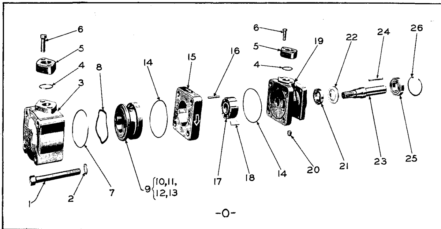
CABLE HOIST HYDRAULIC MOTOR
