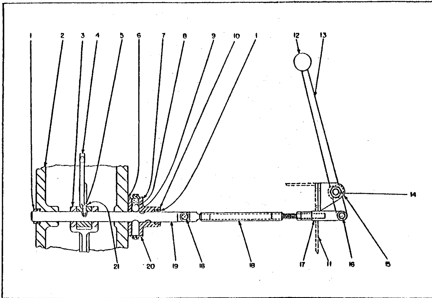
TRANSFER CASE SHIFT MECHANISM (Two Speed Transfer Case)
