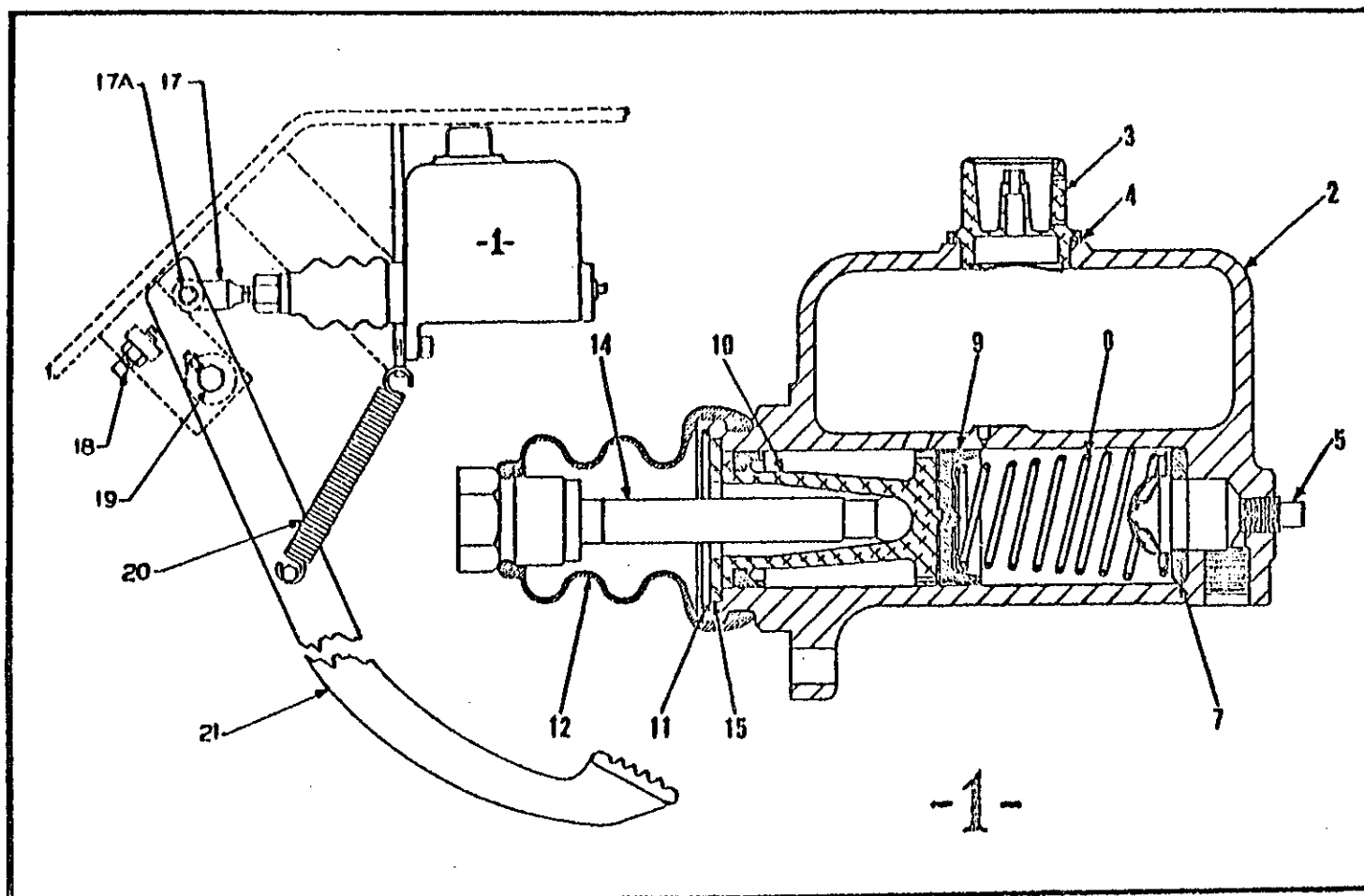
FOOT BRAKE MECHANISM AND MASTER CYLINDER (OUTLET ON SIDE) (2nd Type)
