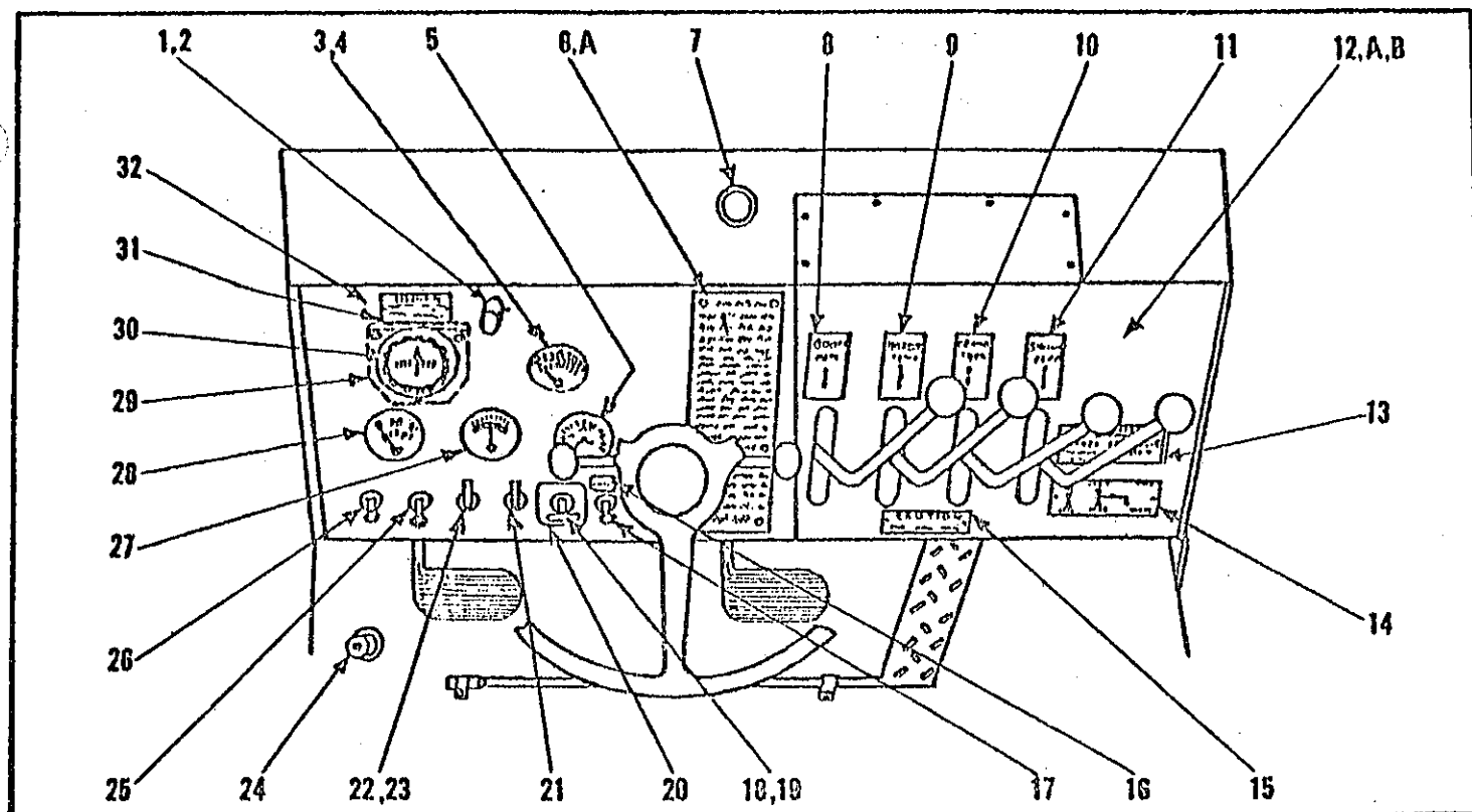
INSTRUMENTS AND CONTROLS
