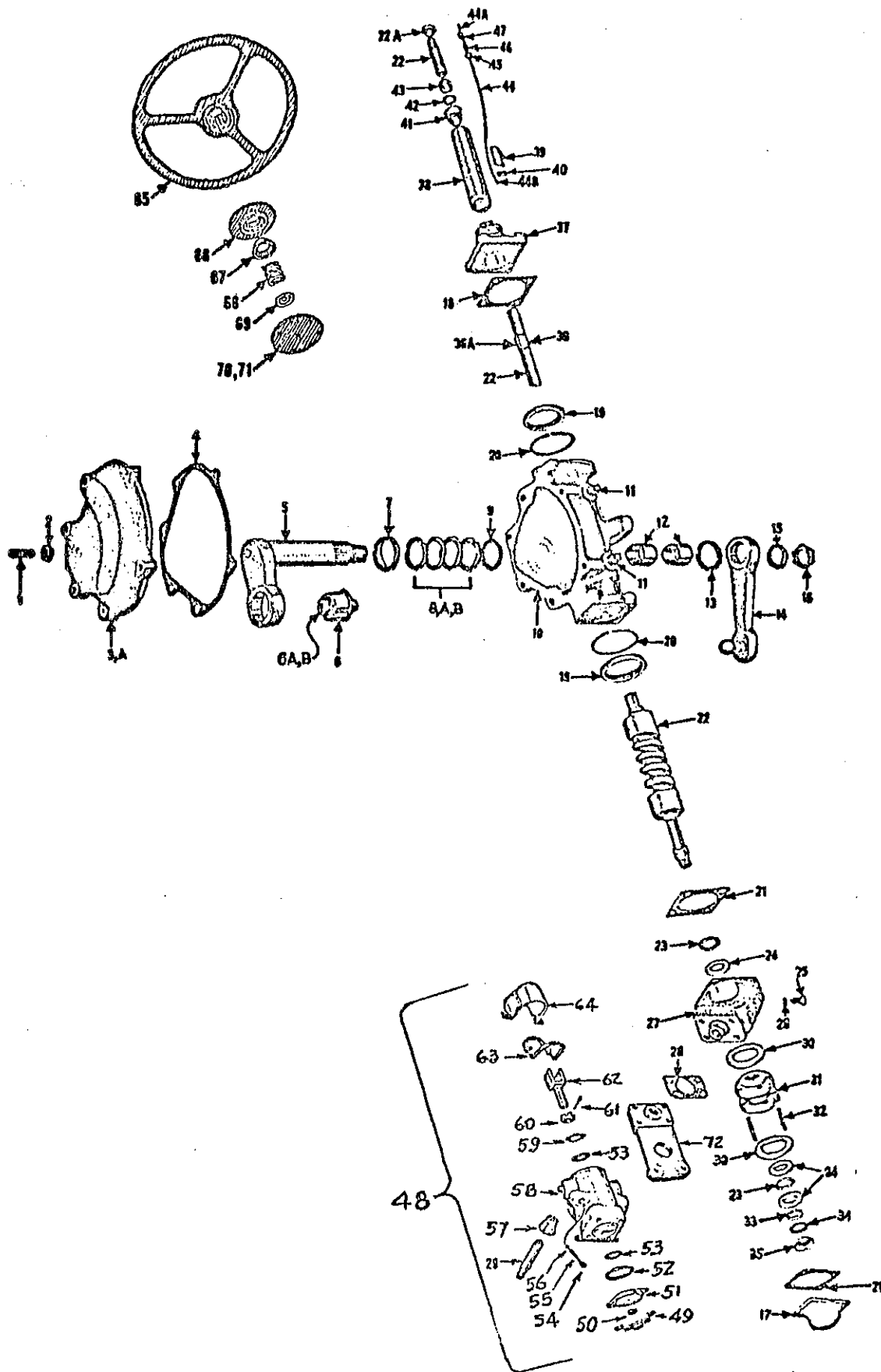
FRONT AXLE STEERING GEAR AND COLUMN (Superseded Page B-5.11 from Serial No. 410-450)
