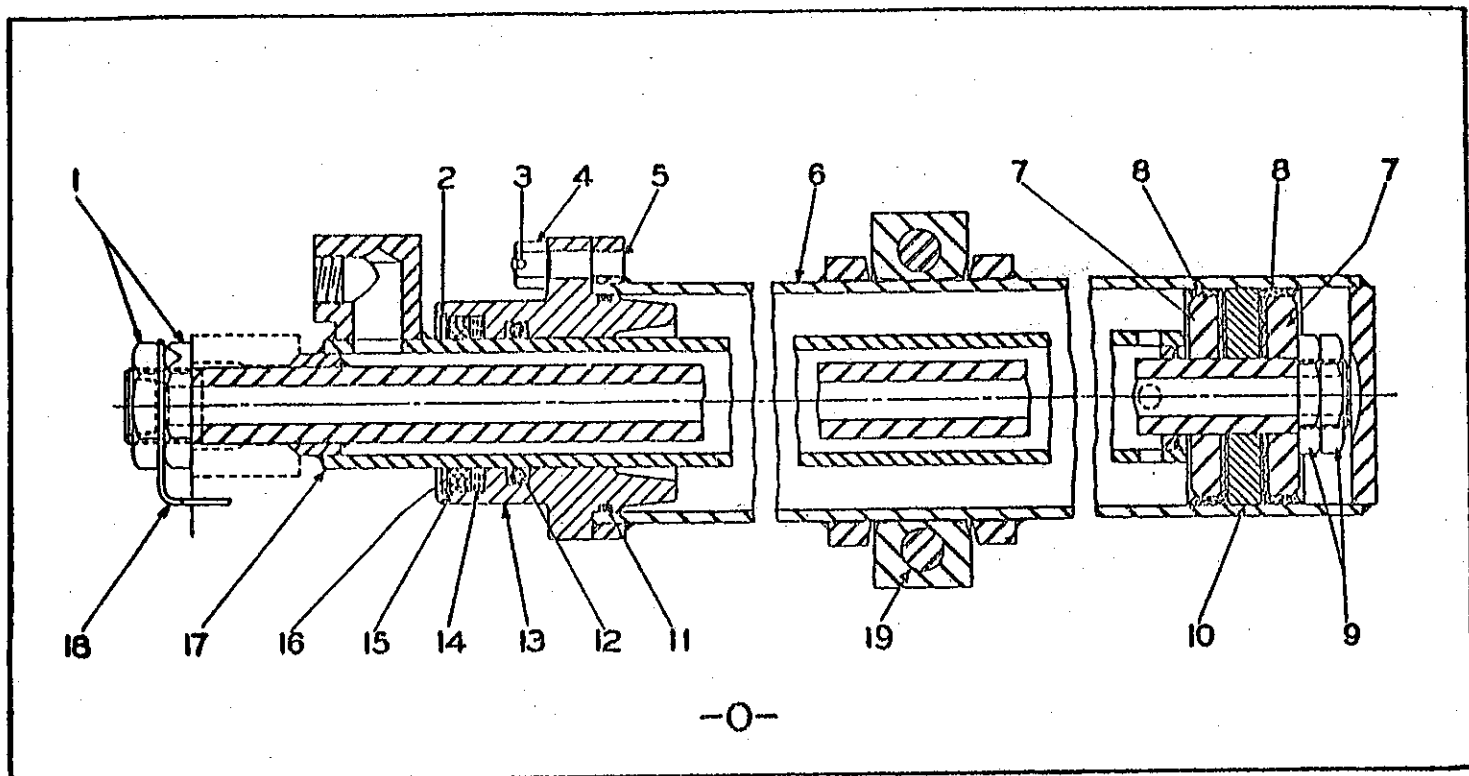
BOOM CROWD RAM
