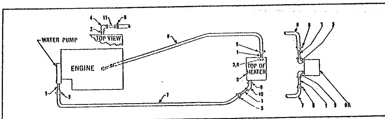
HEATER PIPING DIAGRAM (For Ford 332 Engine)
