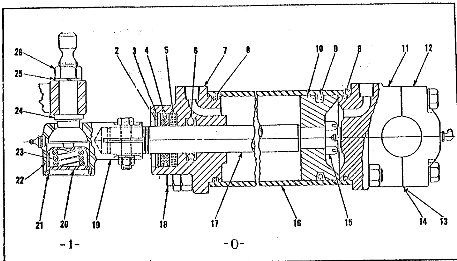
BOOSTER RAM FOR FRONT AXLE STEERING (With Non-Integral Control Valve)
