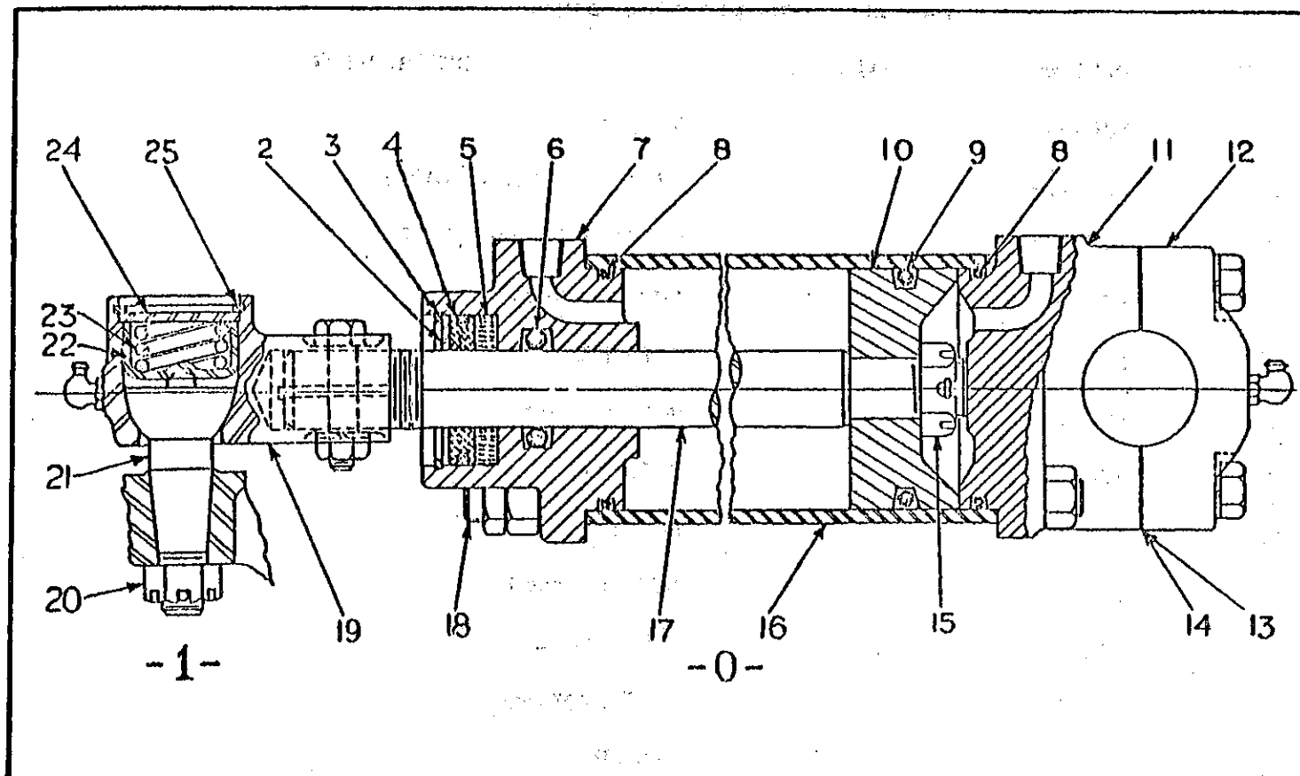
REAR AXLE STEERING RAM (Non-Driving Rear Axle)
