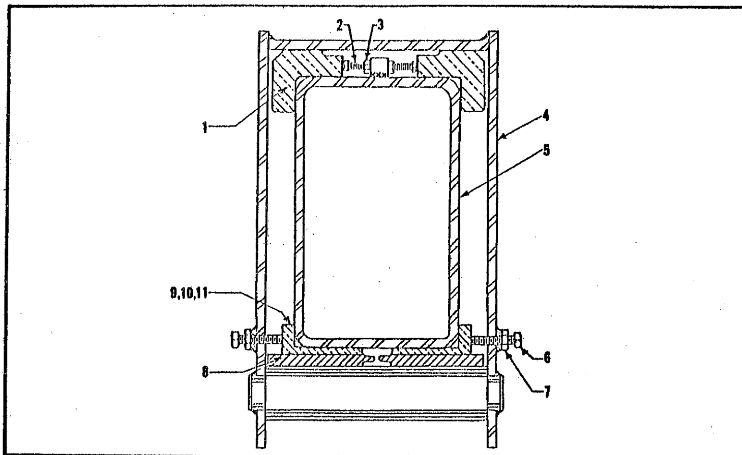
BOOM UPPER REAR AND LOWER FRONT SHOES
