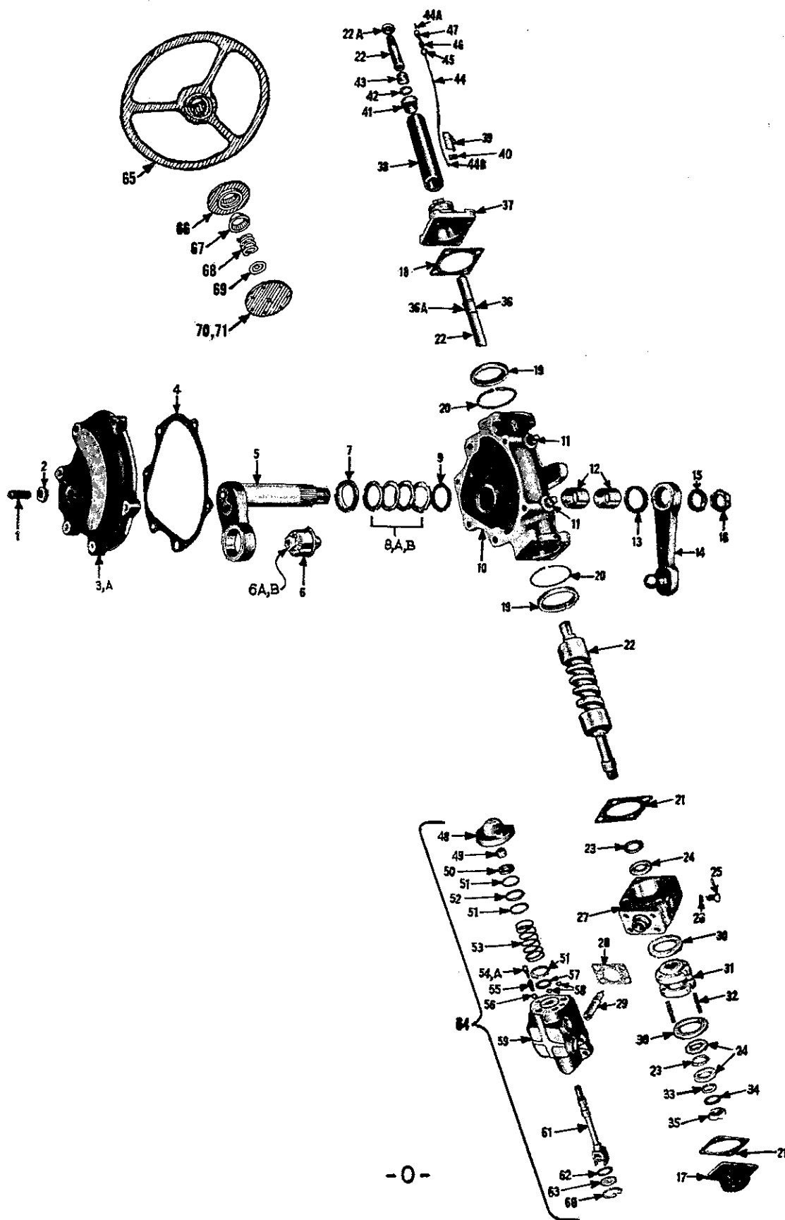
FRONT AXLE STEERING GEAR AND COLUMN
