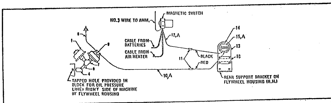
HOURLMETER WIRING DIAGRAM (For GMC-3-71 Engine)
