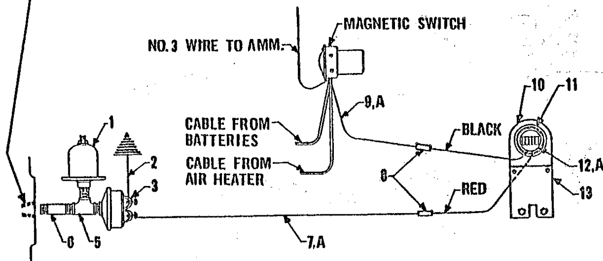
HOURLMETER WIRING DIAGRAM (For IHCo. - UD-282 and UDT-282 Engines)
