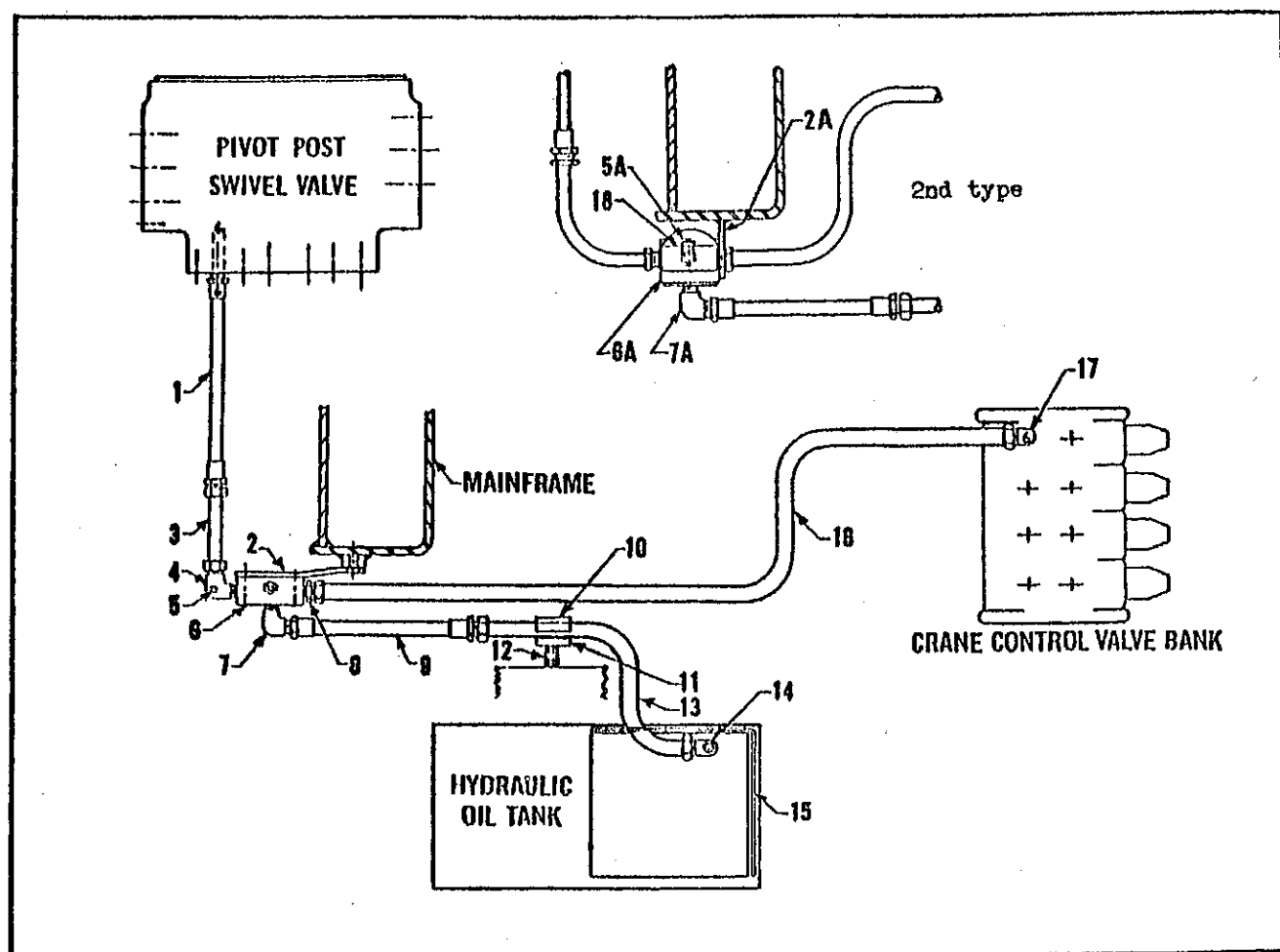
SAFE LOAD RELIEF VALVE
