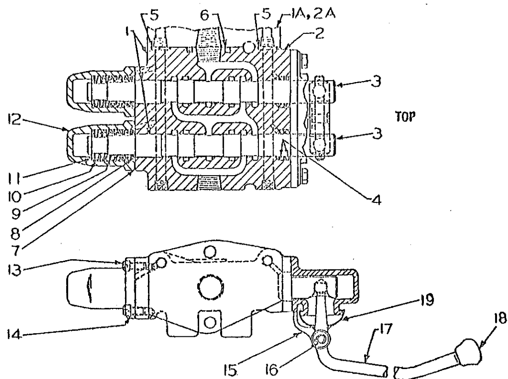
HYDRAULIC OUTRIGGER CONTROL VALVE
