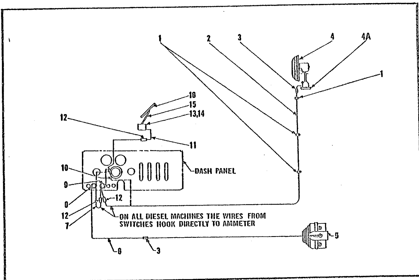
HEATER, DEFROSTER AND WINDSHIELD WIPER WIRING DIAGRAM
