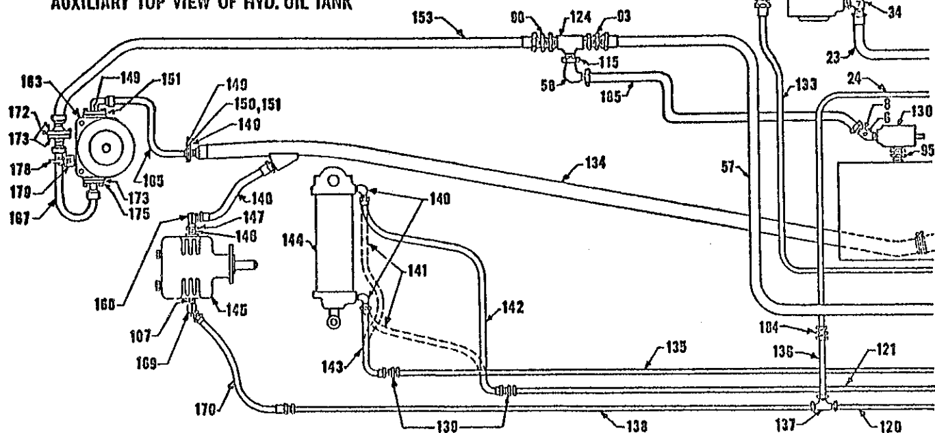
AUXILIARY TOP VIEW OF HYD. OIL TANK
