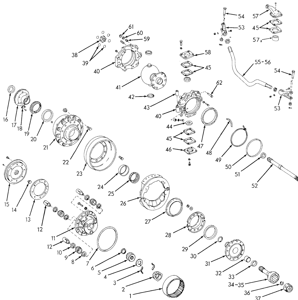
SHAFT AND HUB (Steering Axle)
