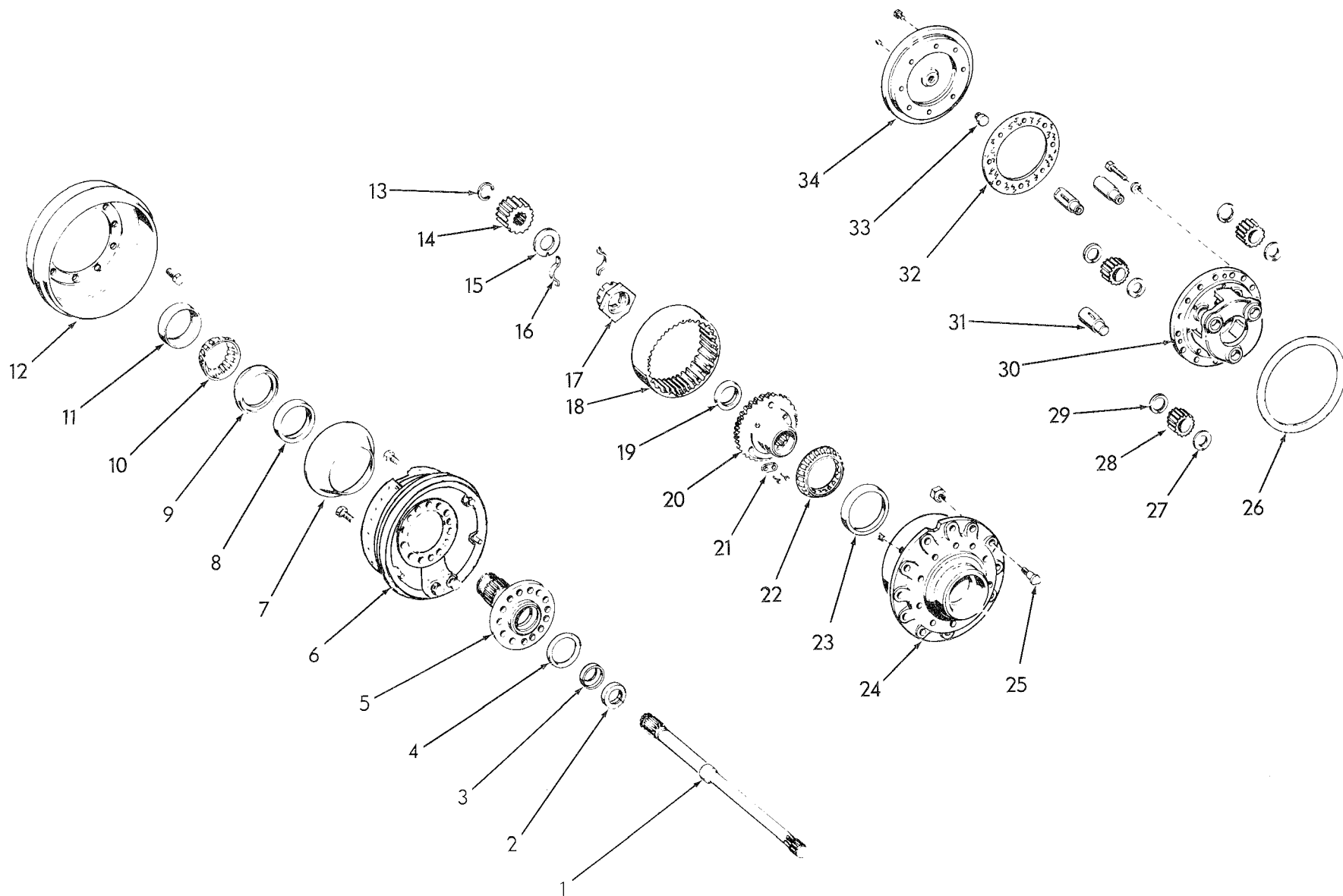
SHAFT AND HUB-RIGID AXLE
