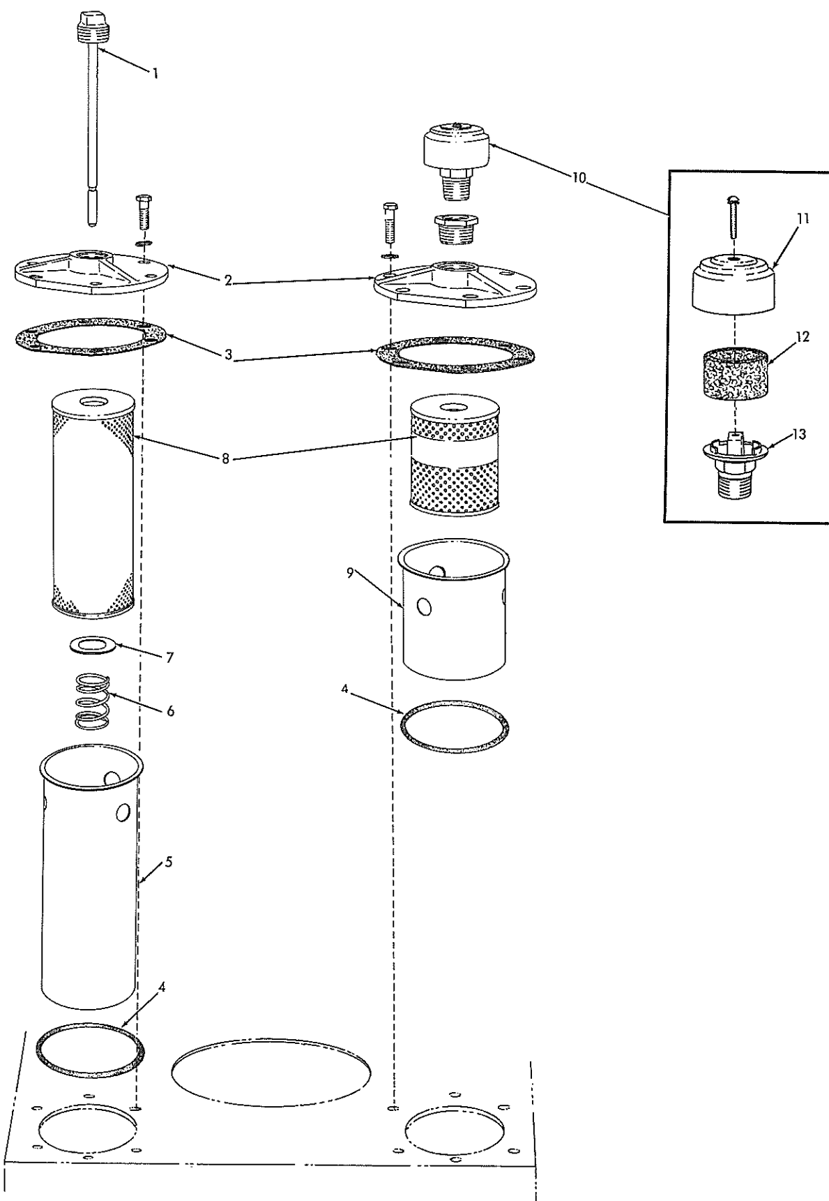
OIL FILTER, AIR FILTER AND BREATHER
