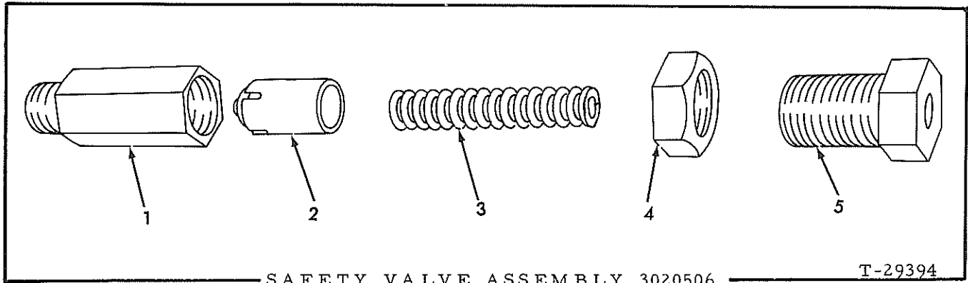
SAFETY VALVE ASSEMBLY 3020506
