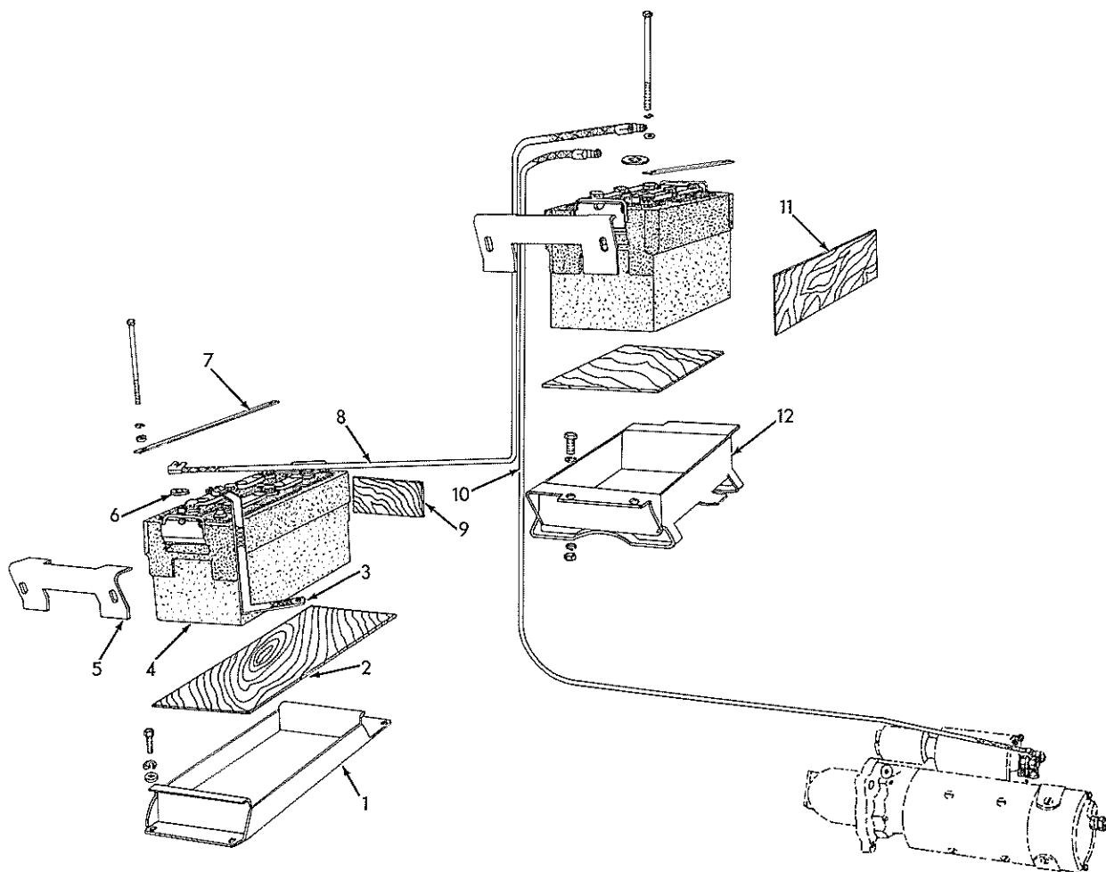
BATTERY AND SUPPORT GROUP
