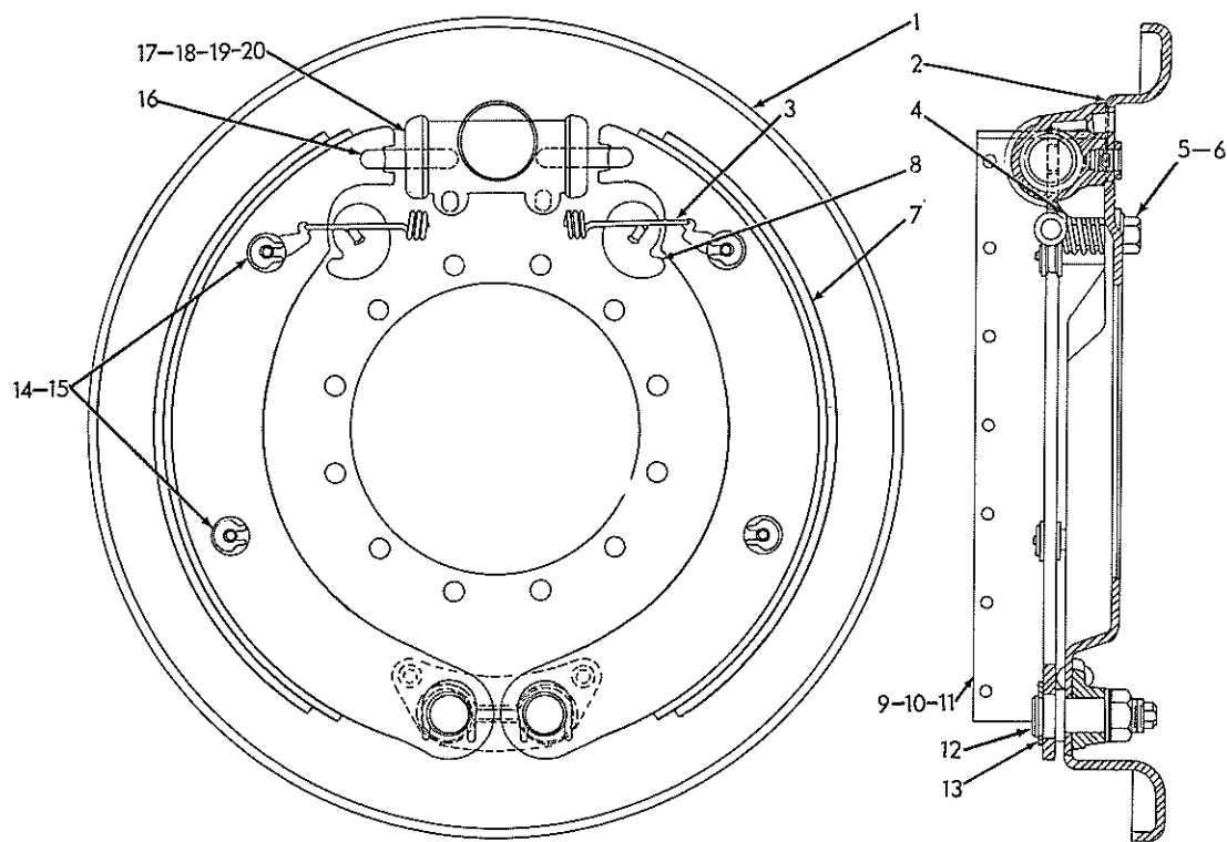
BRAKE ASSEMBLY (Steering Axle)
