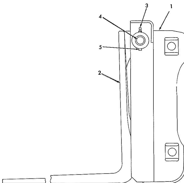
LIFT FORK
