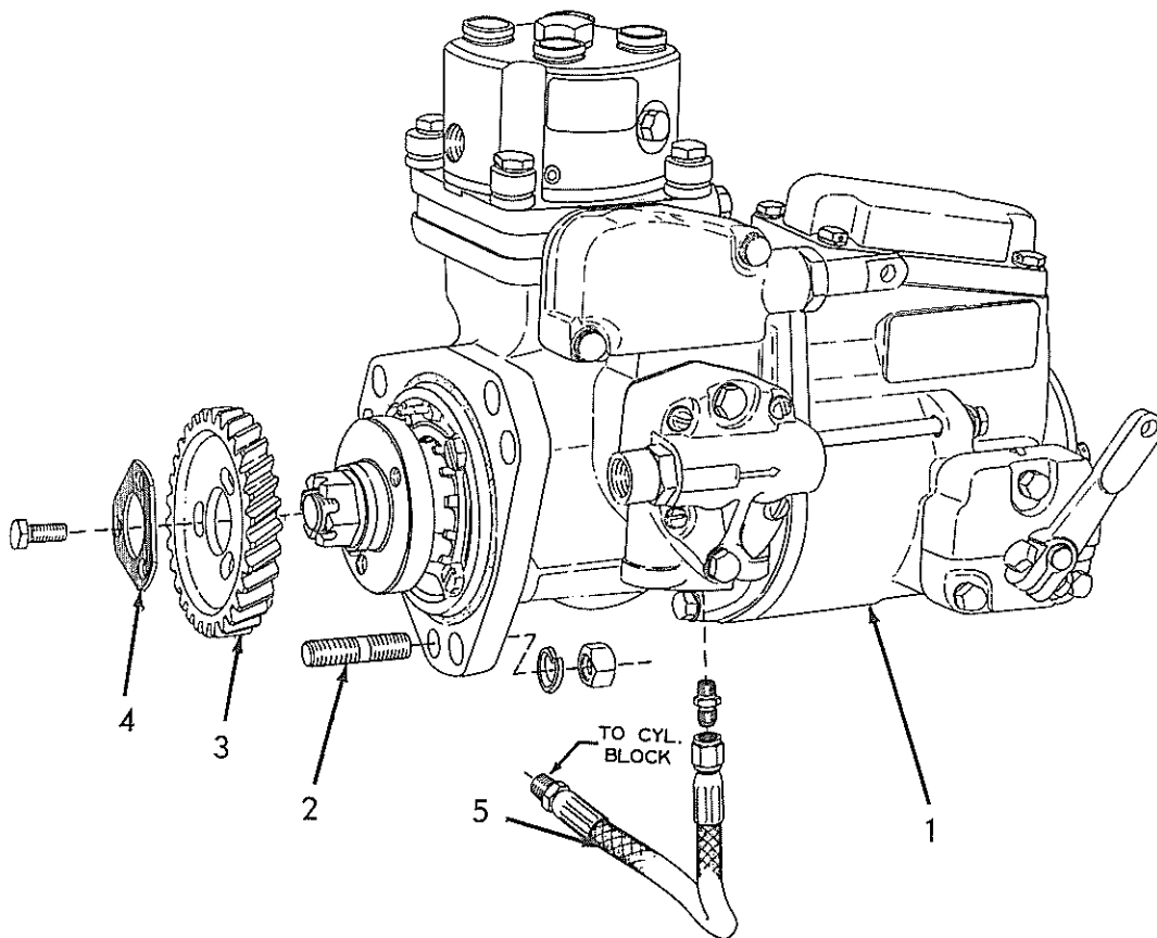
FUEL INJECTION PUMP
