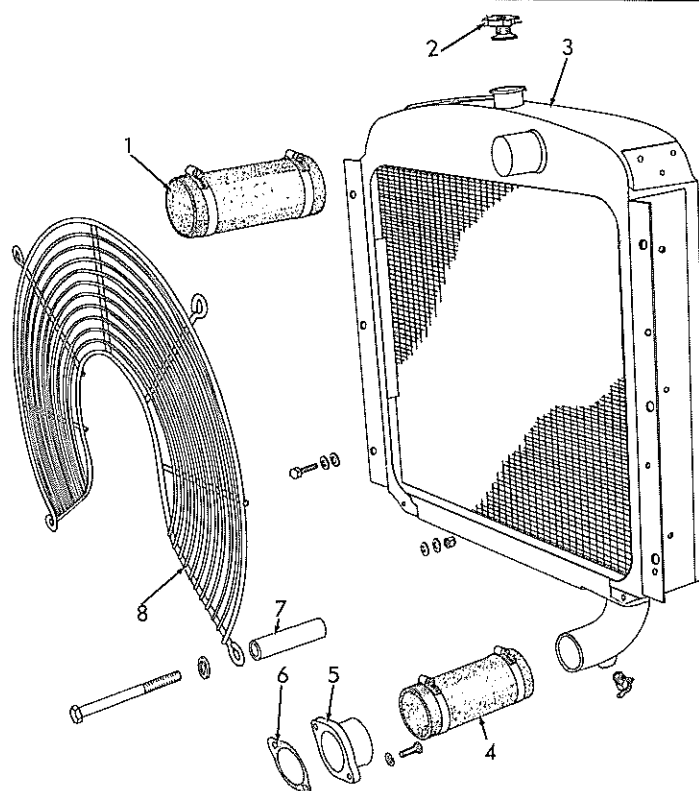
RADIATOR
