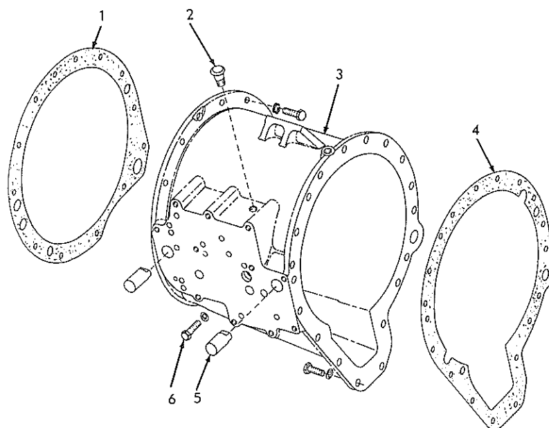
PLANETARY AND CLUTCH HOUSING
