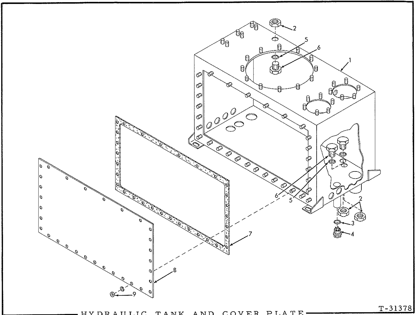
HYDRAULIC TANK AND COVER PLATE
