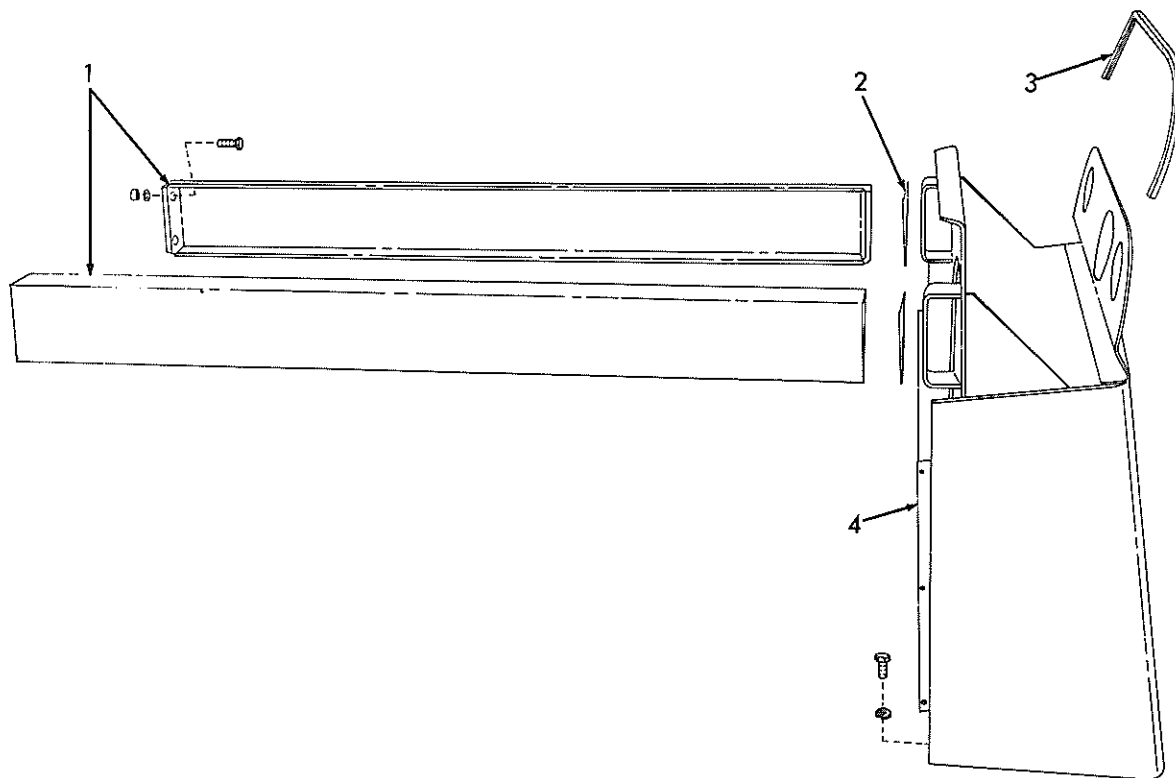
RADIATOR SUPPORT
