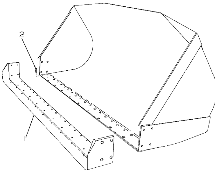
BUCKET
