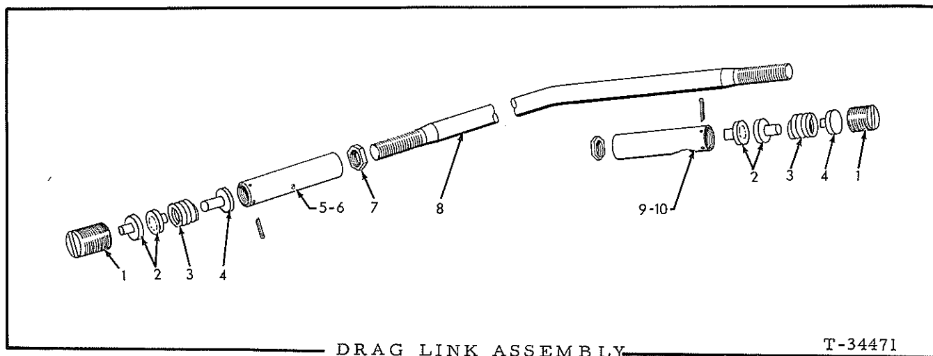
DRAG LINK ASSEMBLY
