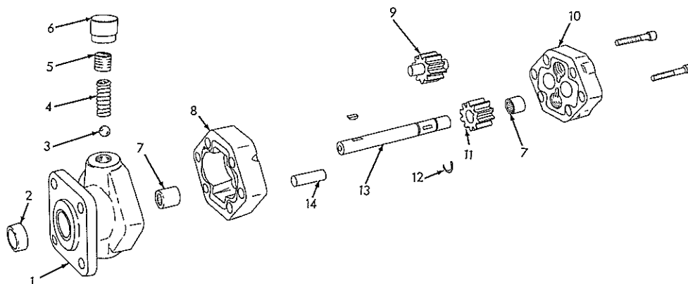
POWER STEERING PUMP ASSEMBLY 3033580
