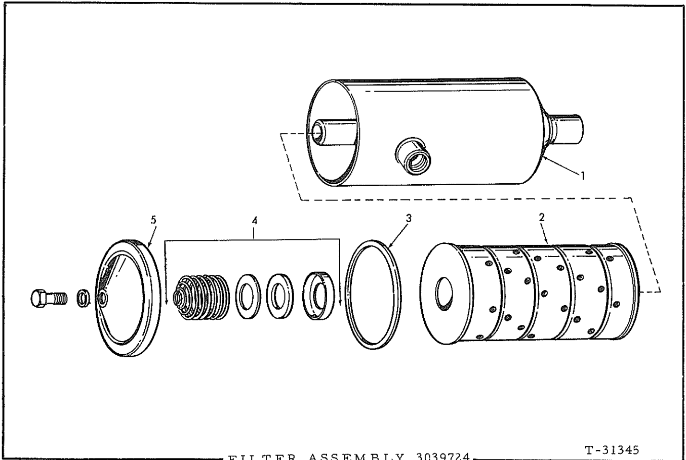
FILTER ASSEMBLY 3039724
