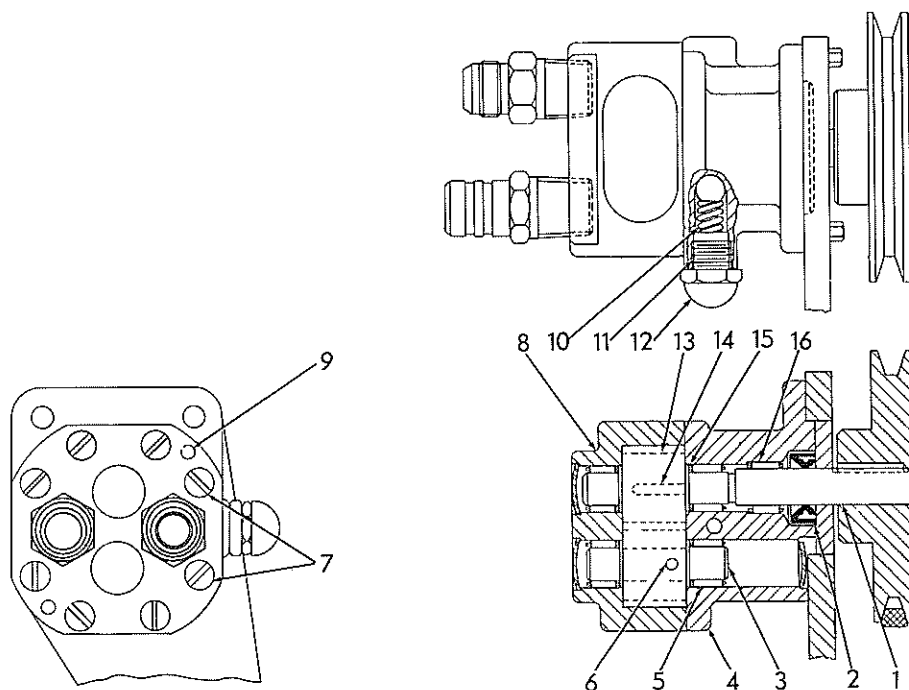
POWER STEERING PUMP ASSEMBLY 3014738
