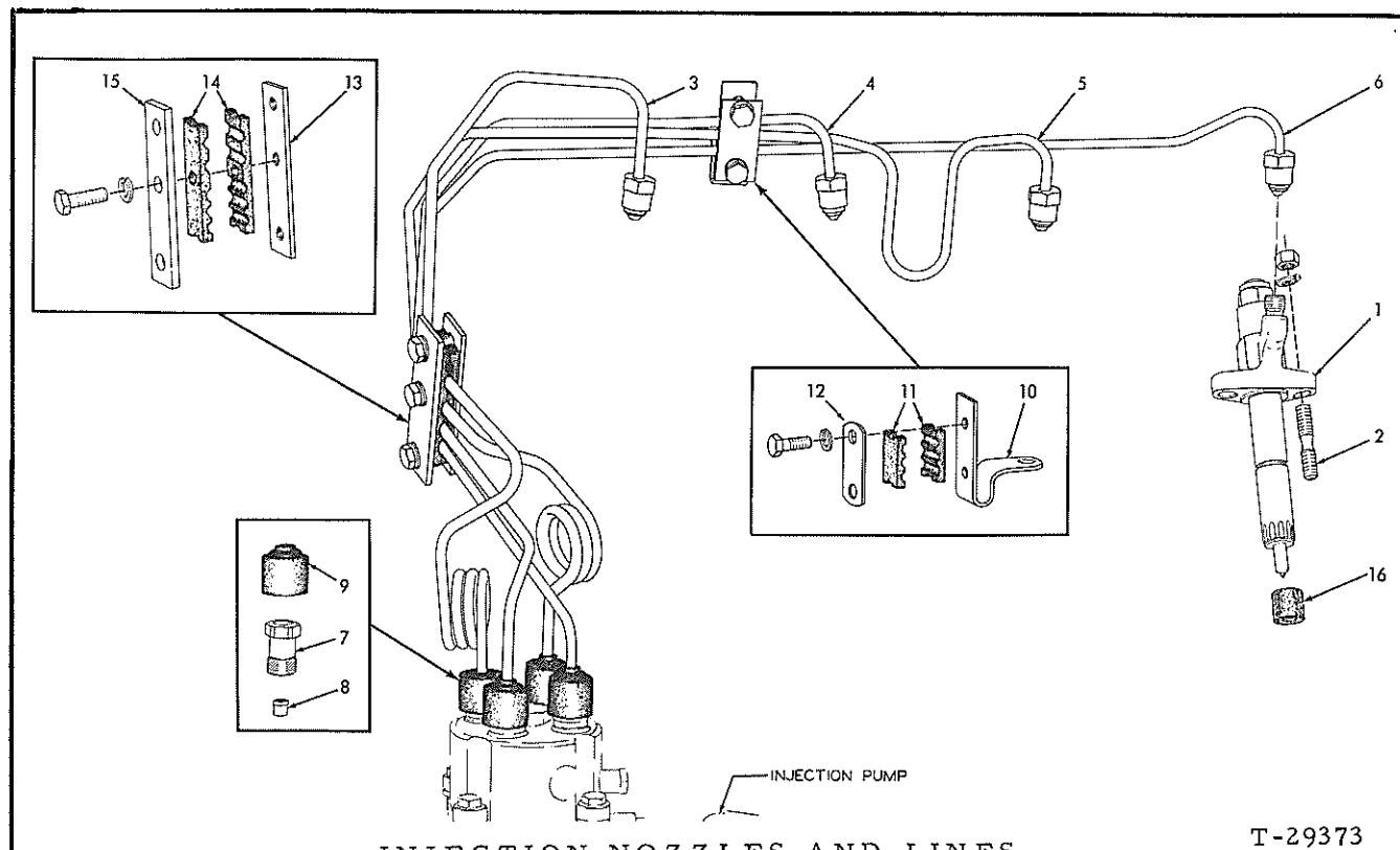
INJECTION NOZZLES AND LINES
