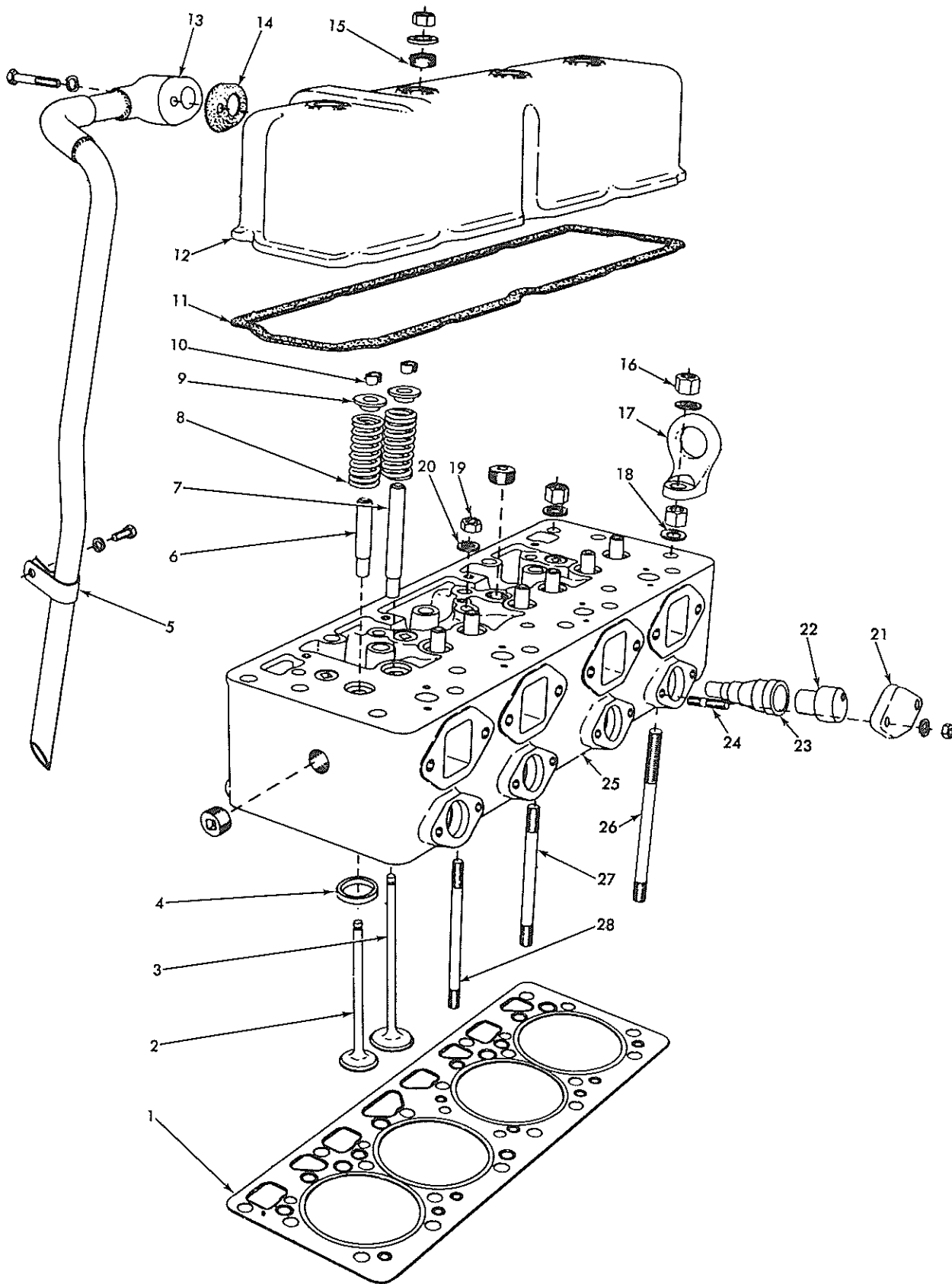
CYLINDER HEAD
