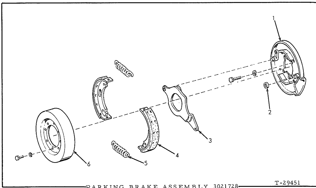
PARKING BRAKE ASSEMBLY 3021728
