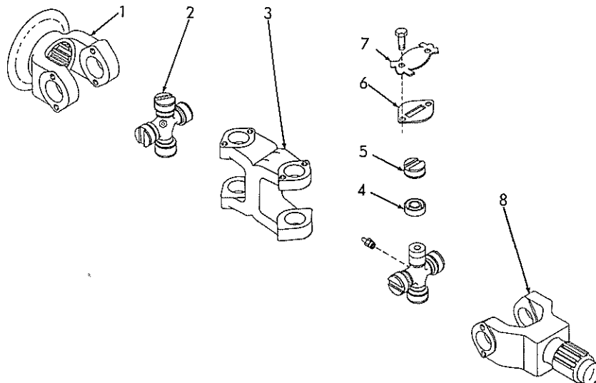
JOINT ASSEMBLY 3024882
