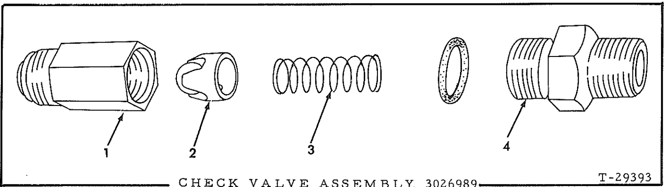
CHECK VALVE ASSEMBLY 3026989
