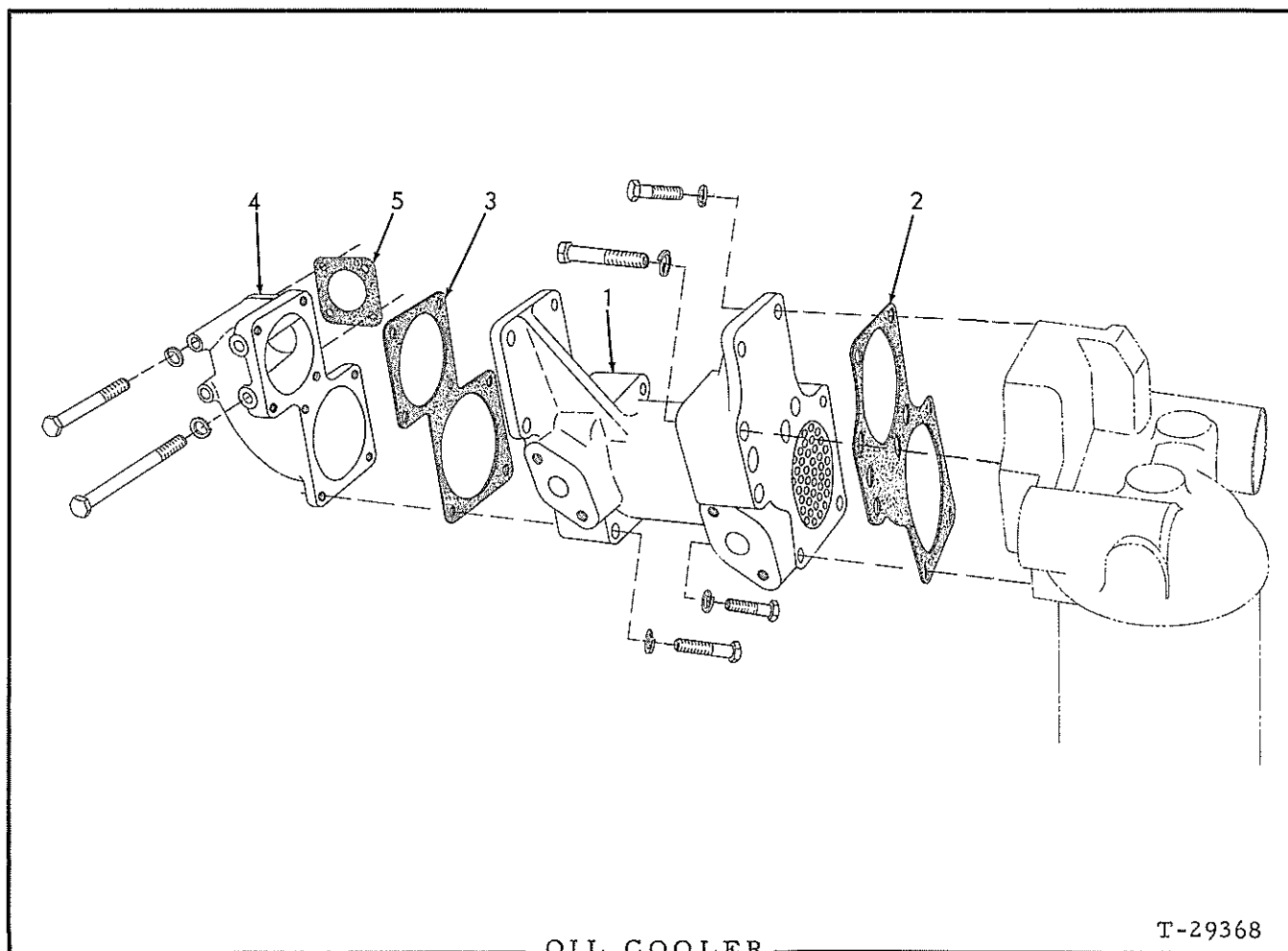
OIL COOLER
