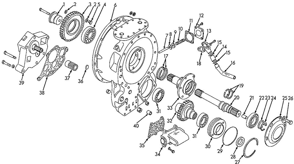
CONVERTER HOUSING AND DRIVE GEARS
