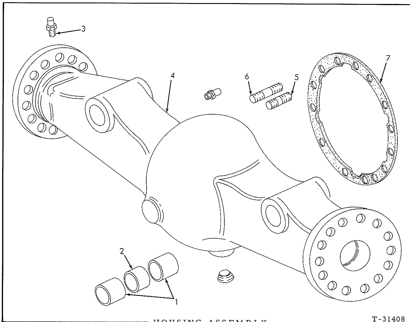
HOUSING ASSEMBLY (Rigid Axle)
