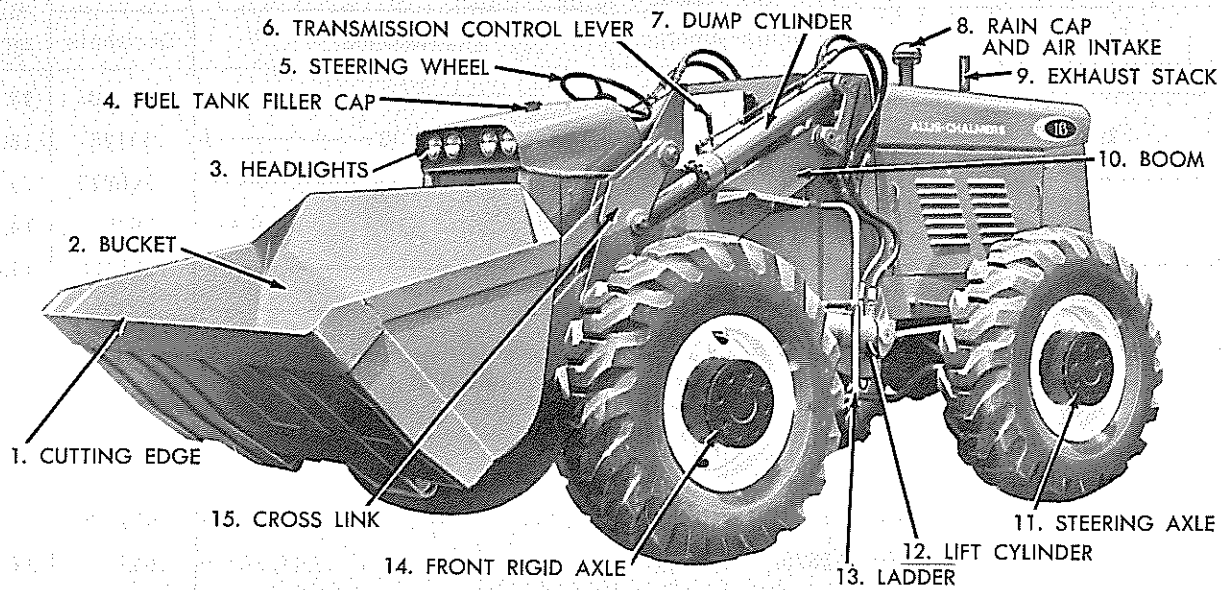
MODEL TL16 (Diesel) TRACTOR LOADER
