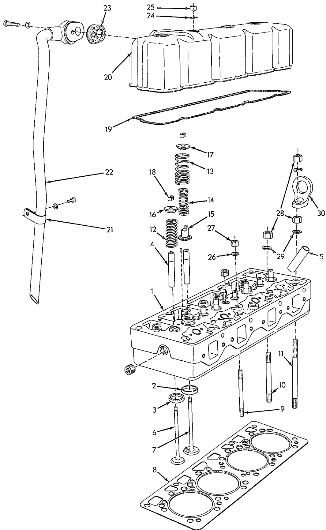
CYLINDER HEAD
