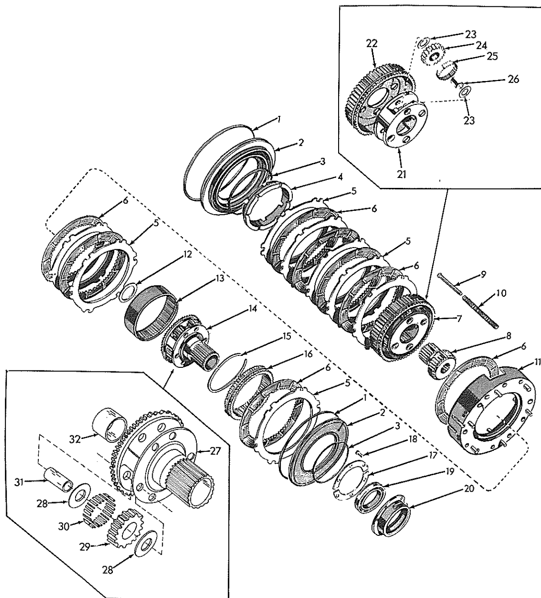
FORWARD AND REVERSE PLANETARIES AND CLUTCHES T-34432
