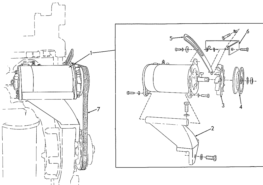
GENERATOR
