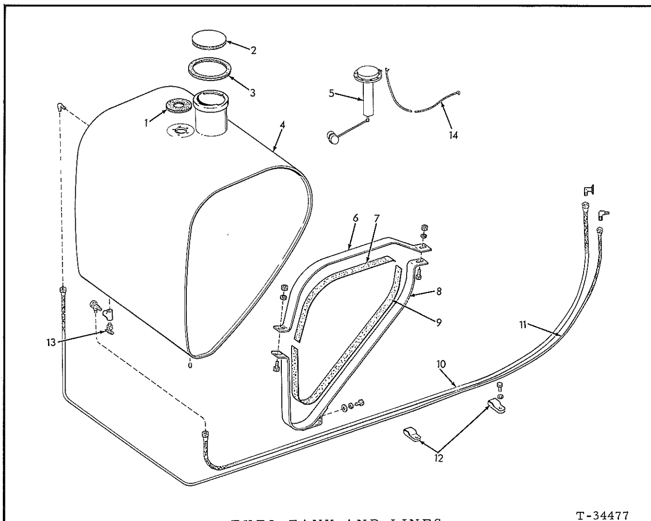
FUEL TANK AND LINES
