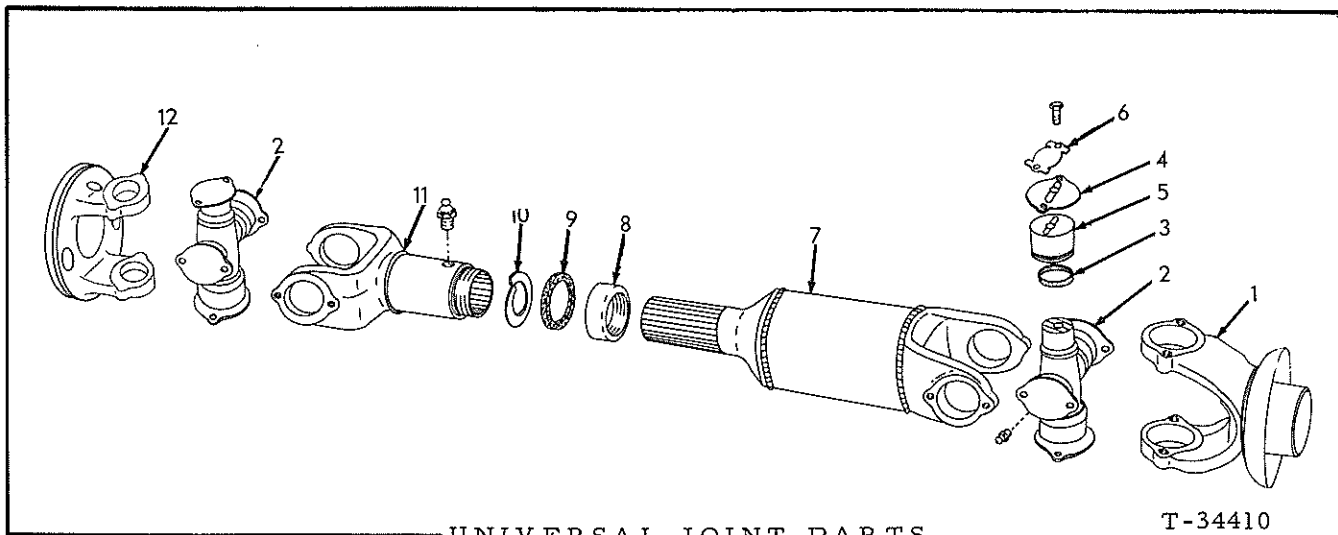
UNIVERSAL JOINT PARTS
