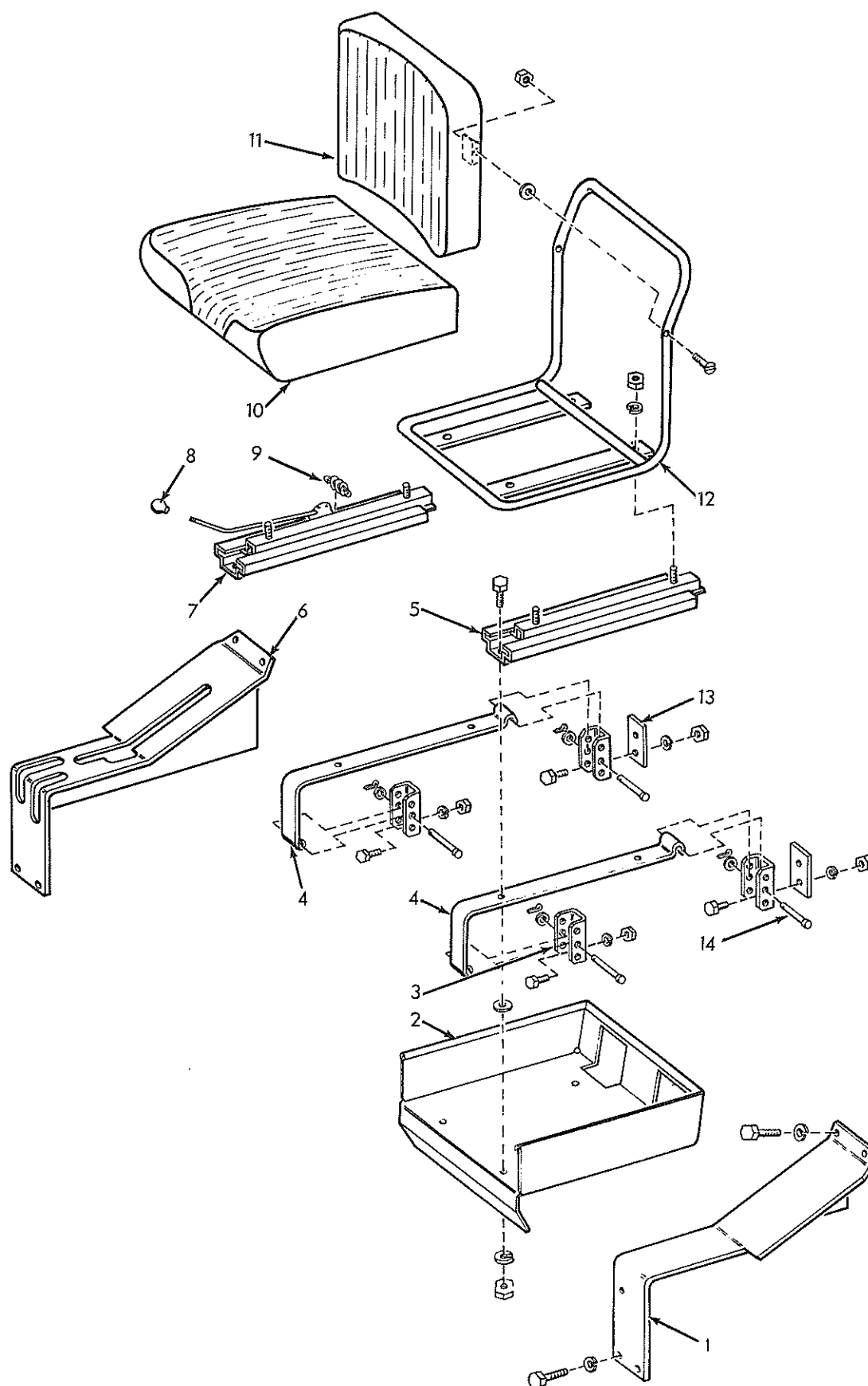
SEAT GROUP
