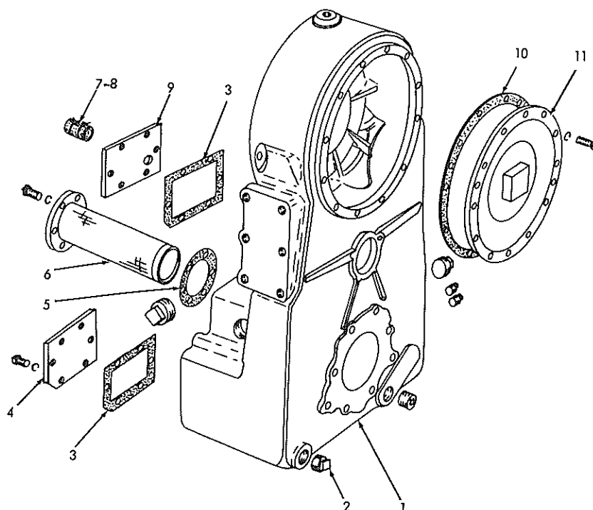
TRANSFER HOUSING AND FILTER
