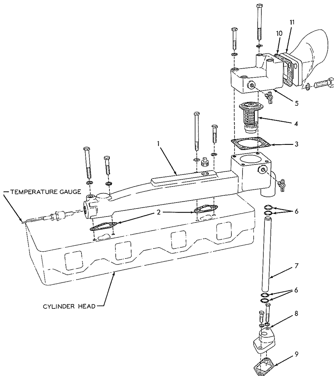
WATER OUTLET MANIFOLD
