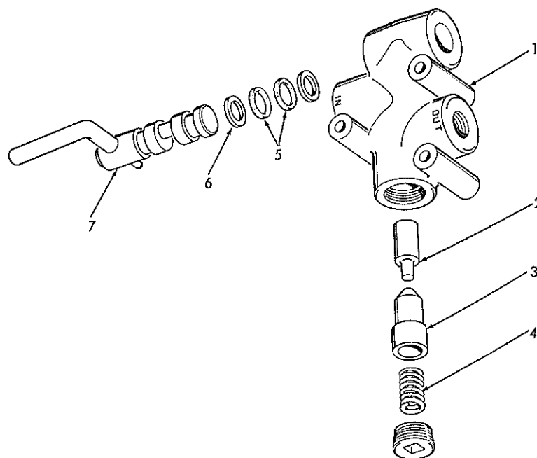
CLUTCH CUTOFF VALVE ASSEMBLY 3012490
