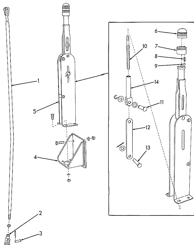
PARKING BRAKE CONTROL GROUP
