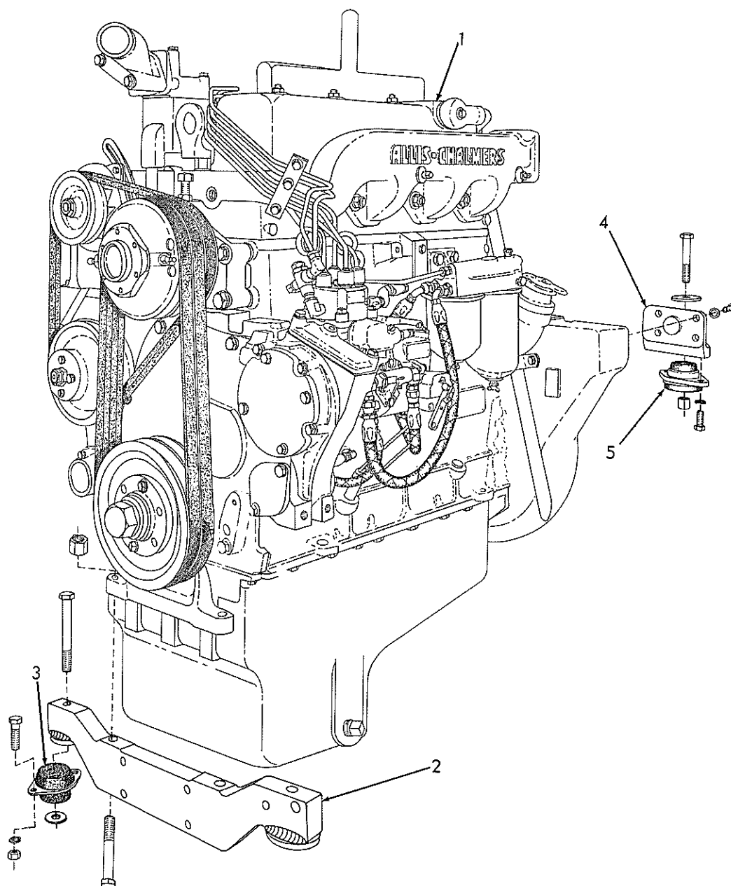
ENGINE AND MOUNTING
