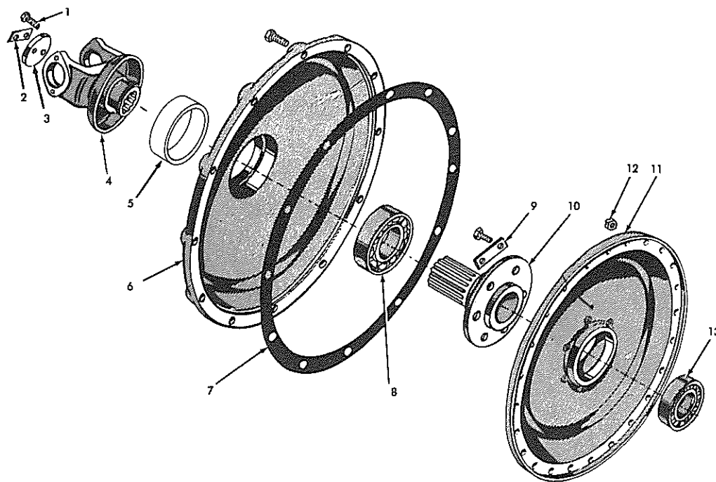
TORQUE CONVERTER COVER AND DRIVE GROUP T-36574
