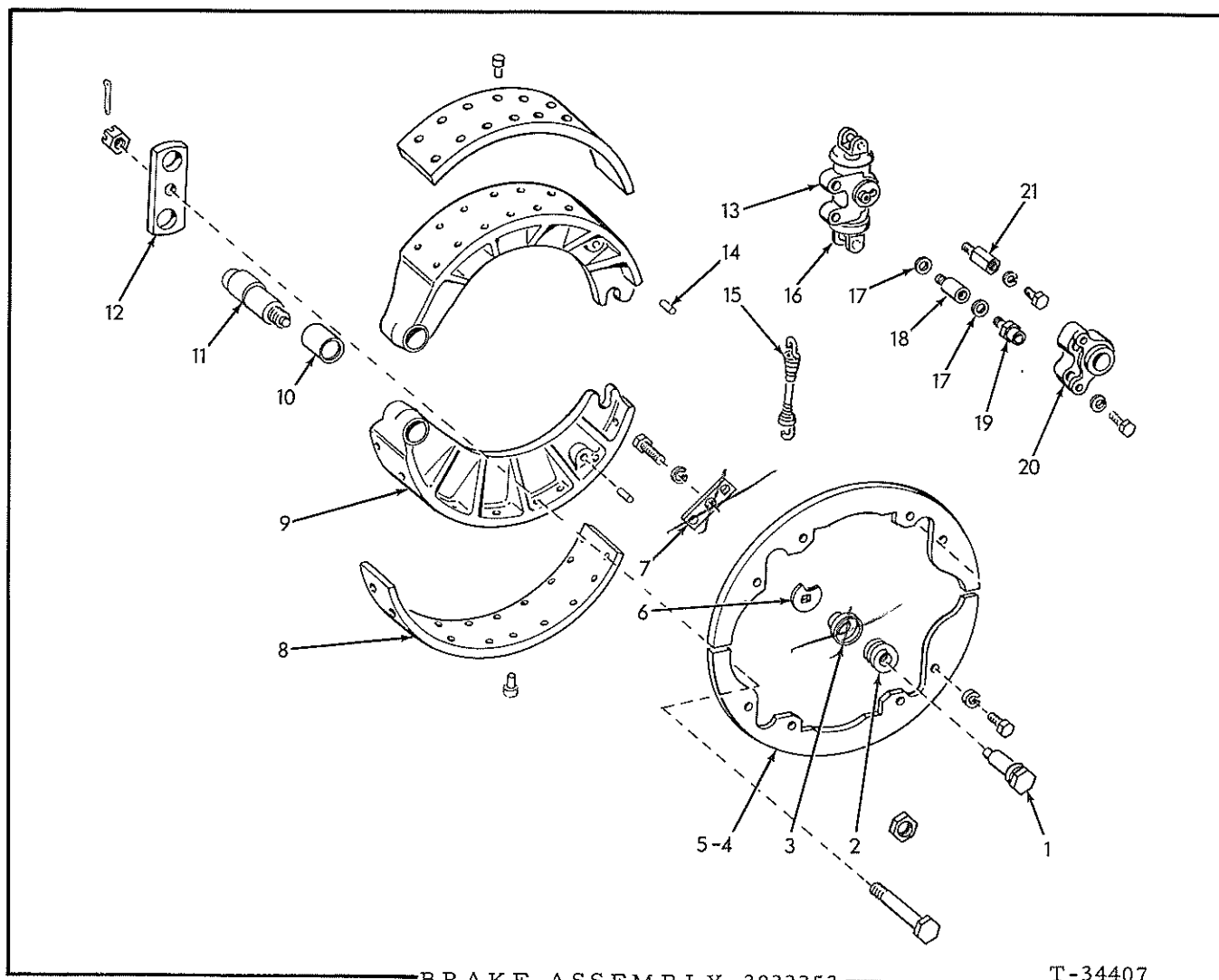
BRAKE ASSEMBLY 3022253 (Steering Axle)
