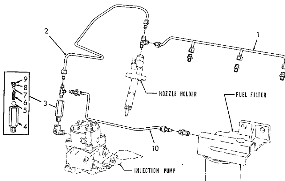
FUEL INJECTION RETURN LINES
