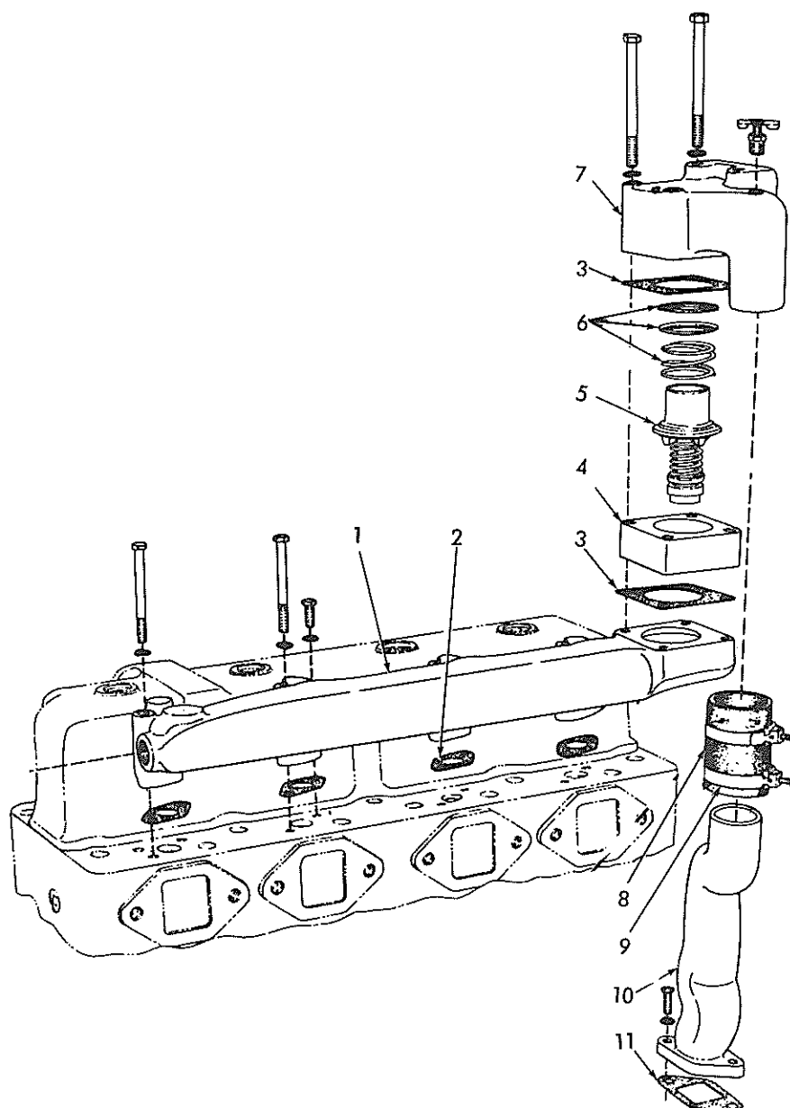
WATER OUTLET MANIFOLD
