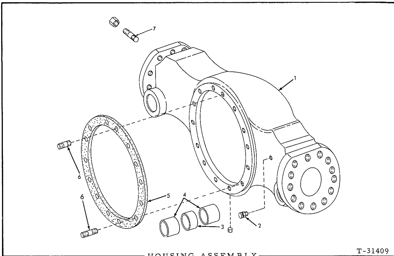
HOUSING ASSEMBLY (Steering Axle)
