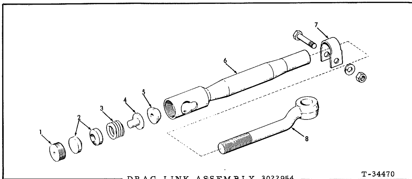
DRAG LINK ASSEMBLY 3022954
