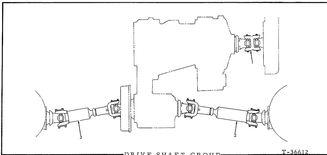
DRIVE SHAFT GROUP
