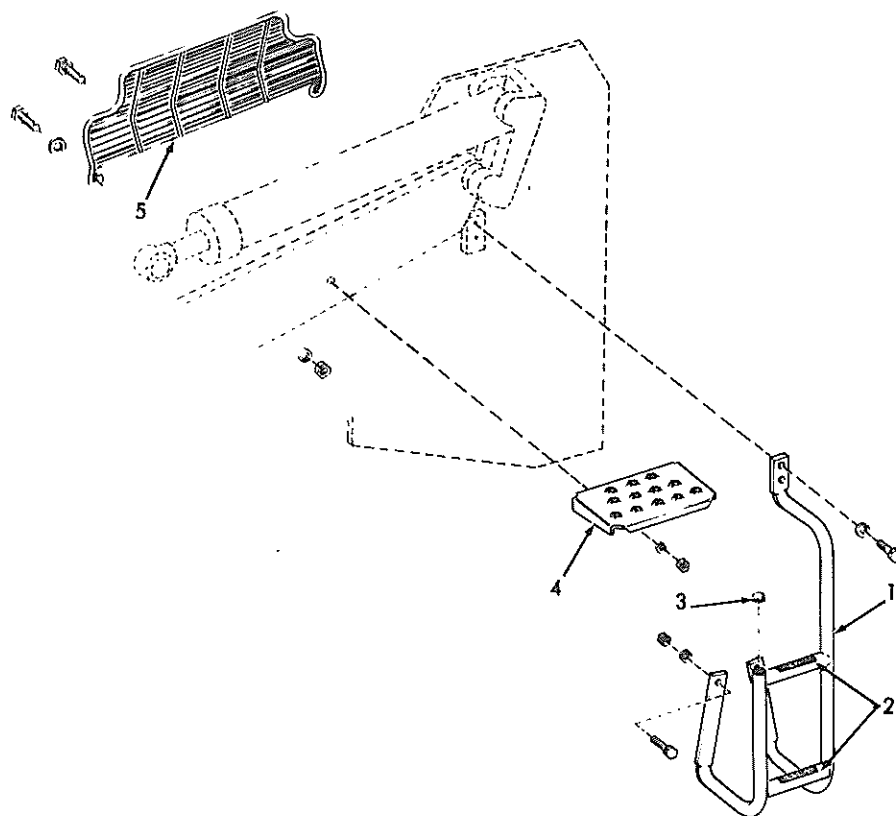
LADDER AND GUARD GROUP
