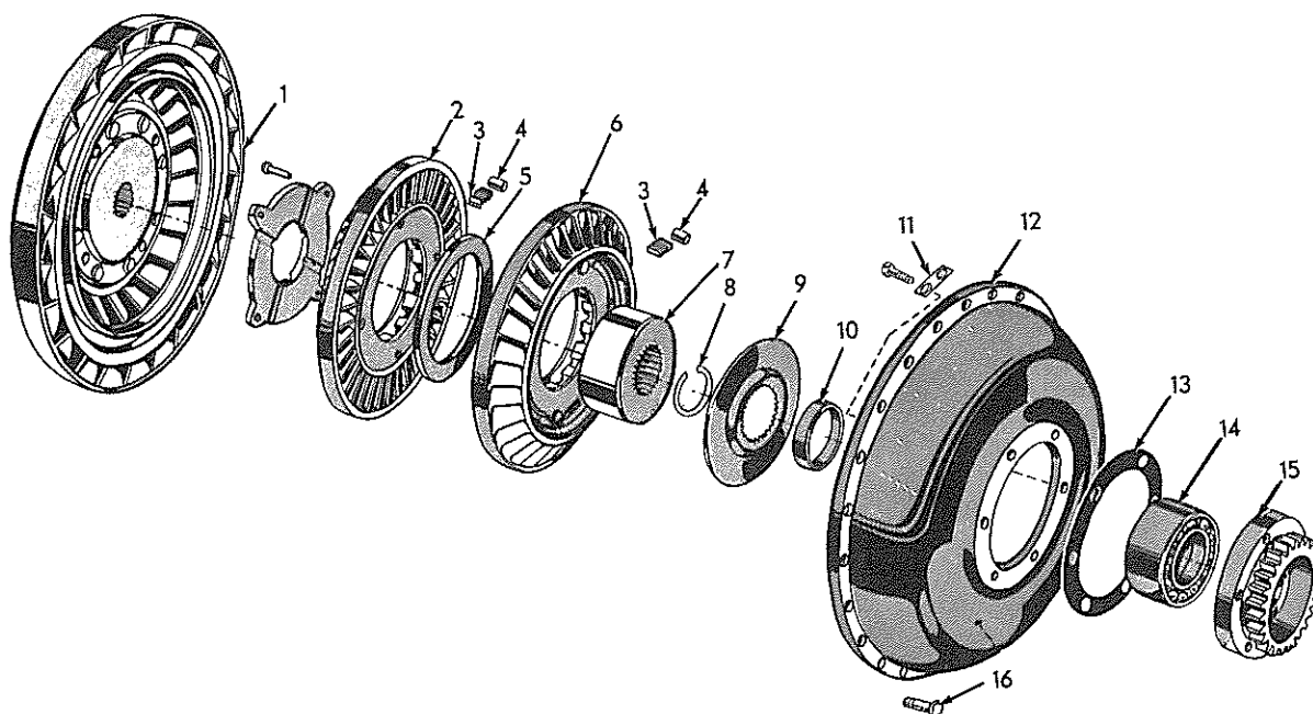
TORQUE CONVERTER PUMP GROUP
