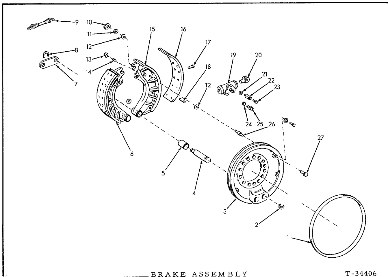
BRAKE ASSEMBLY (Rigid Axle)
