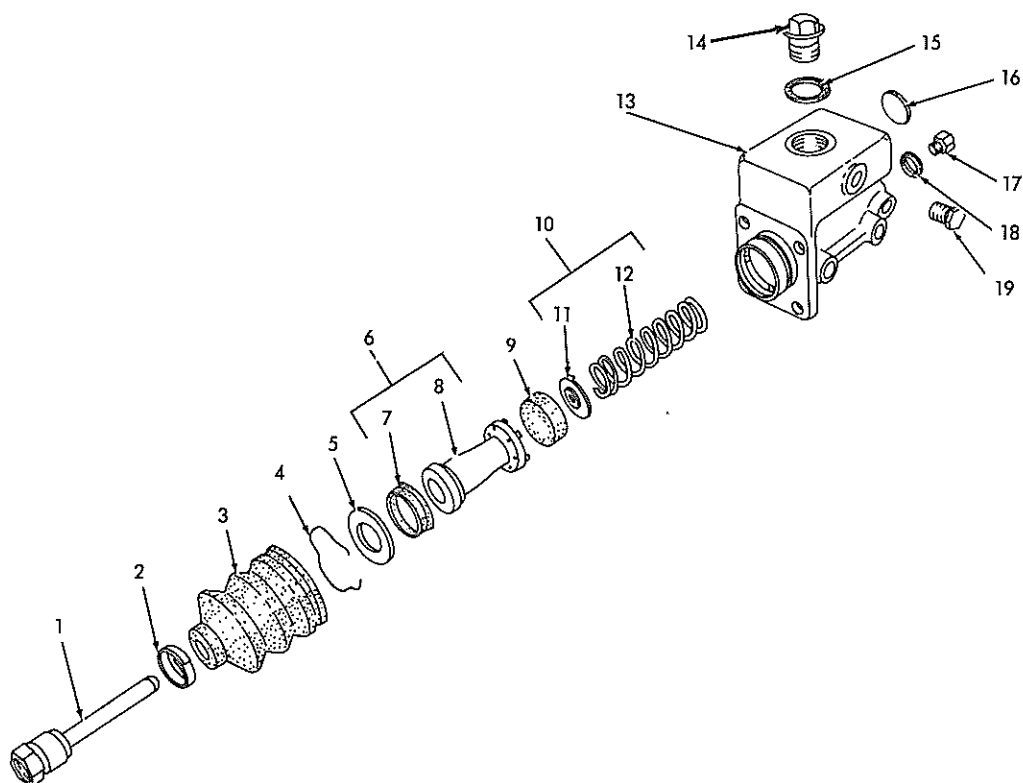
MASTER CYLINDER ASSEMBLY
