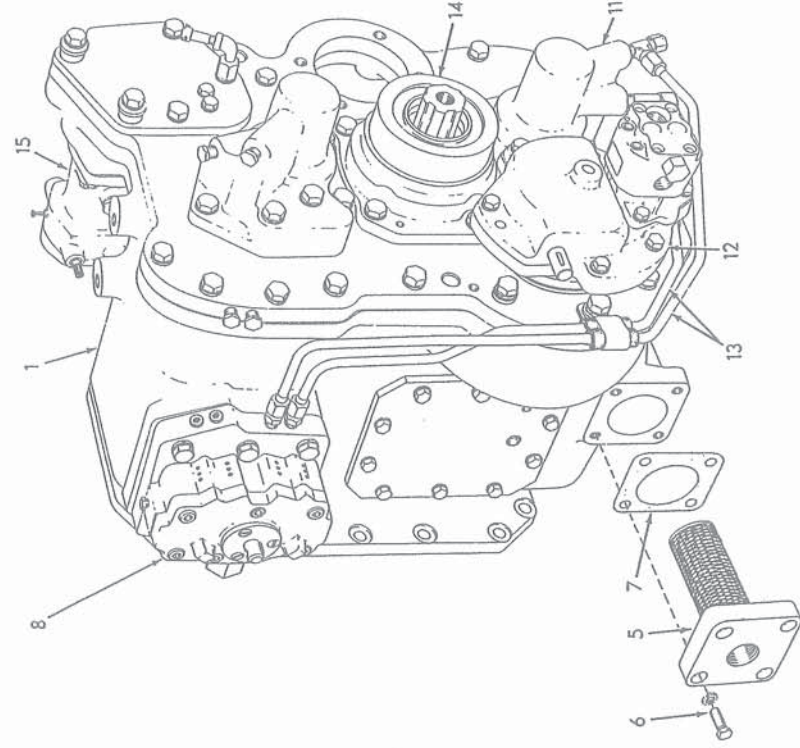
RIGHT FRONT VIEW
