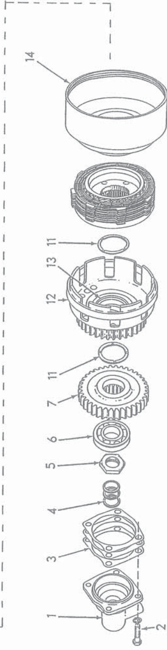
TRANSMISSION BOTTOM SHAFT
