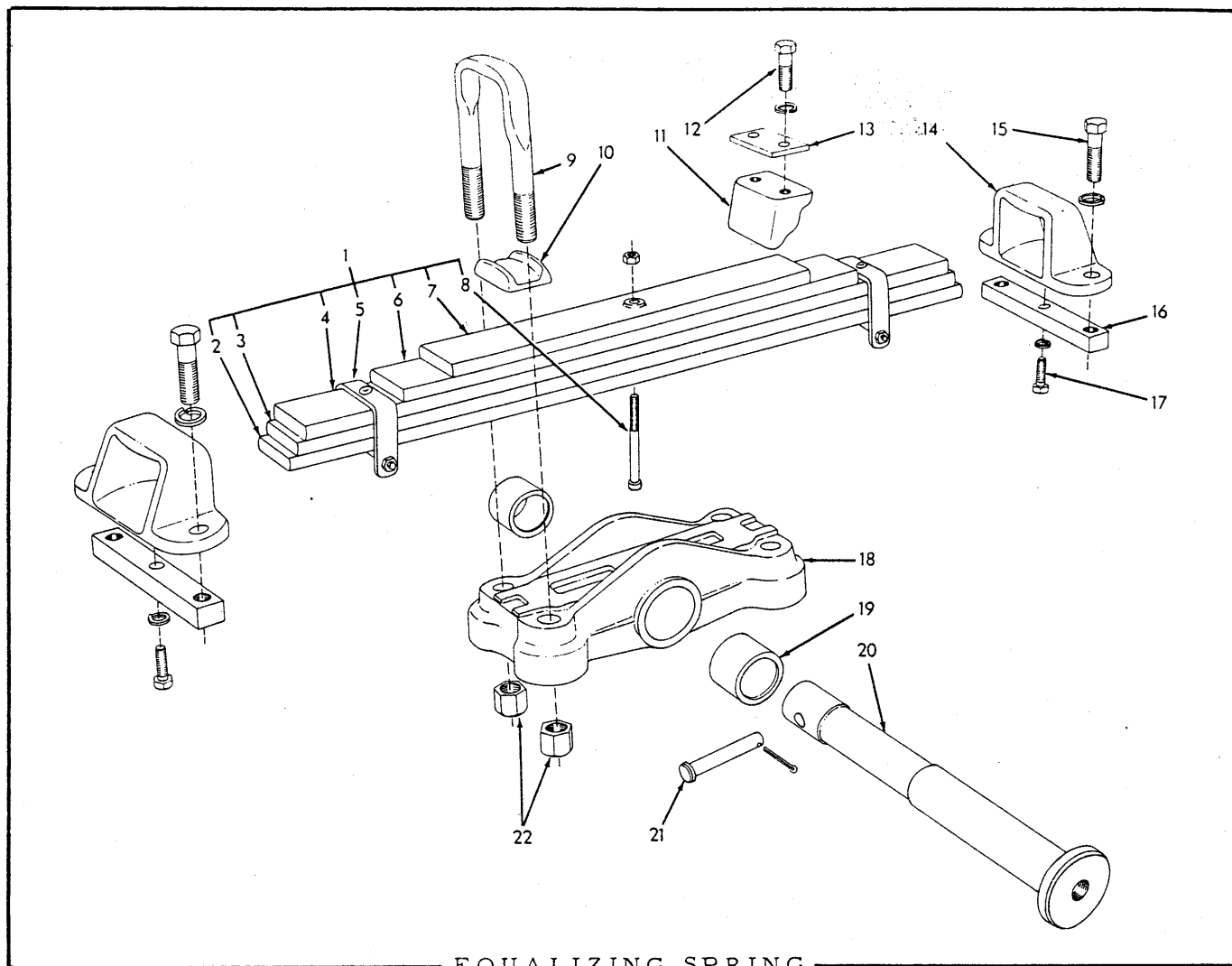
EQUALIZING SPRING
