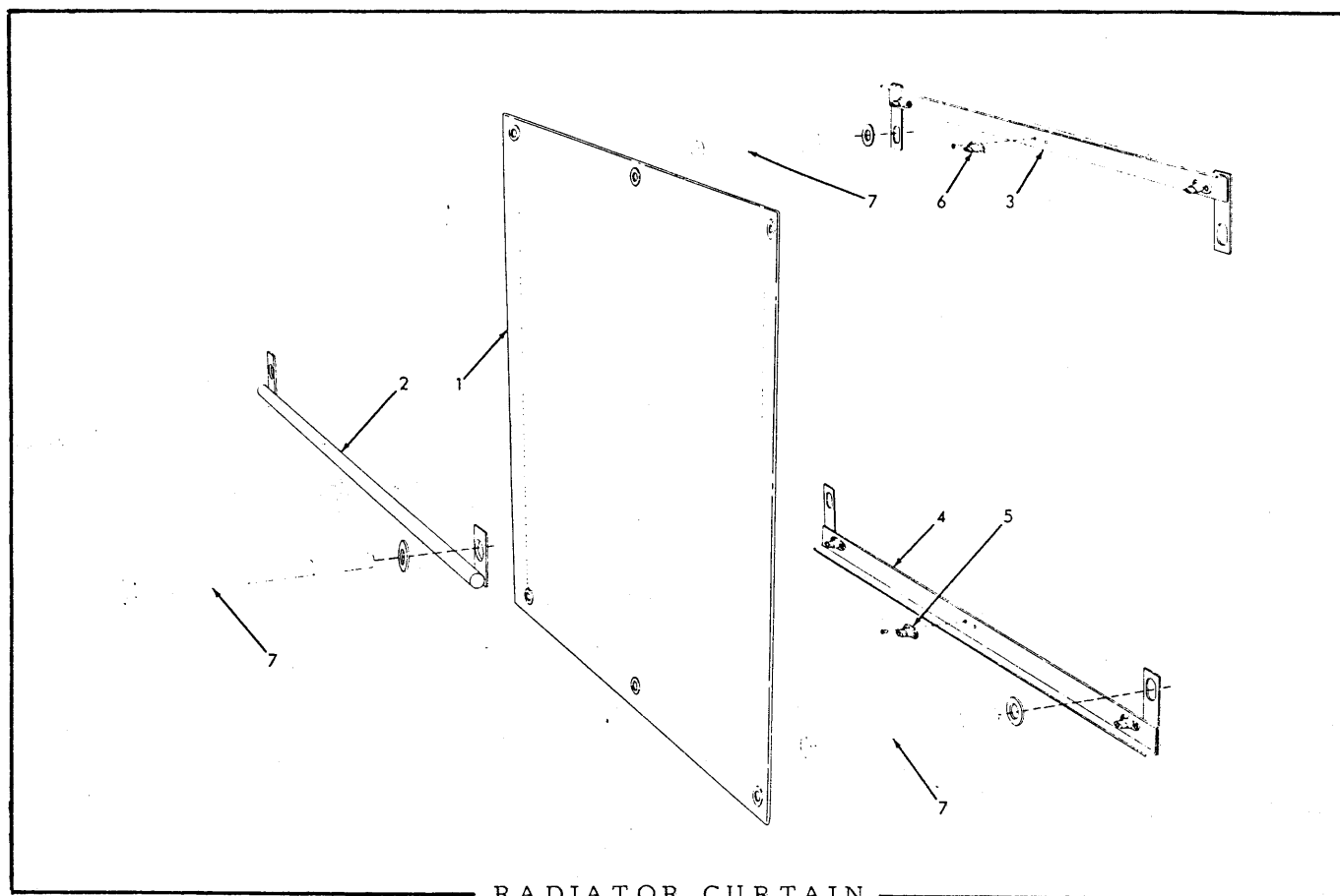
RADIATOR CURTAIN
