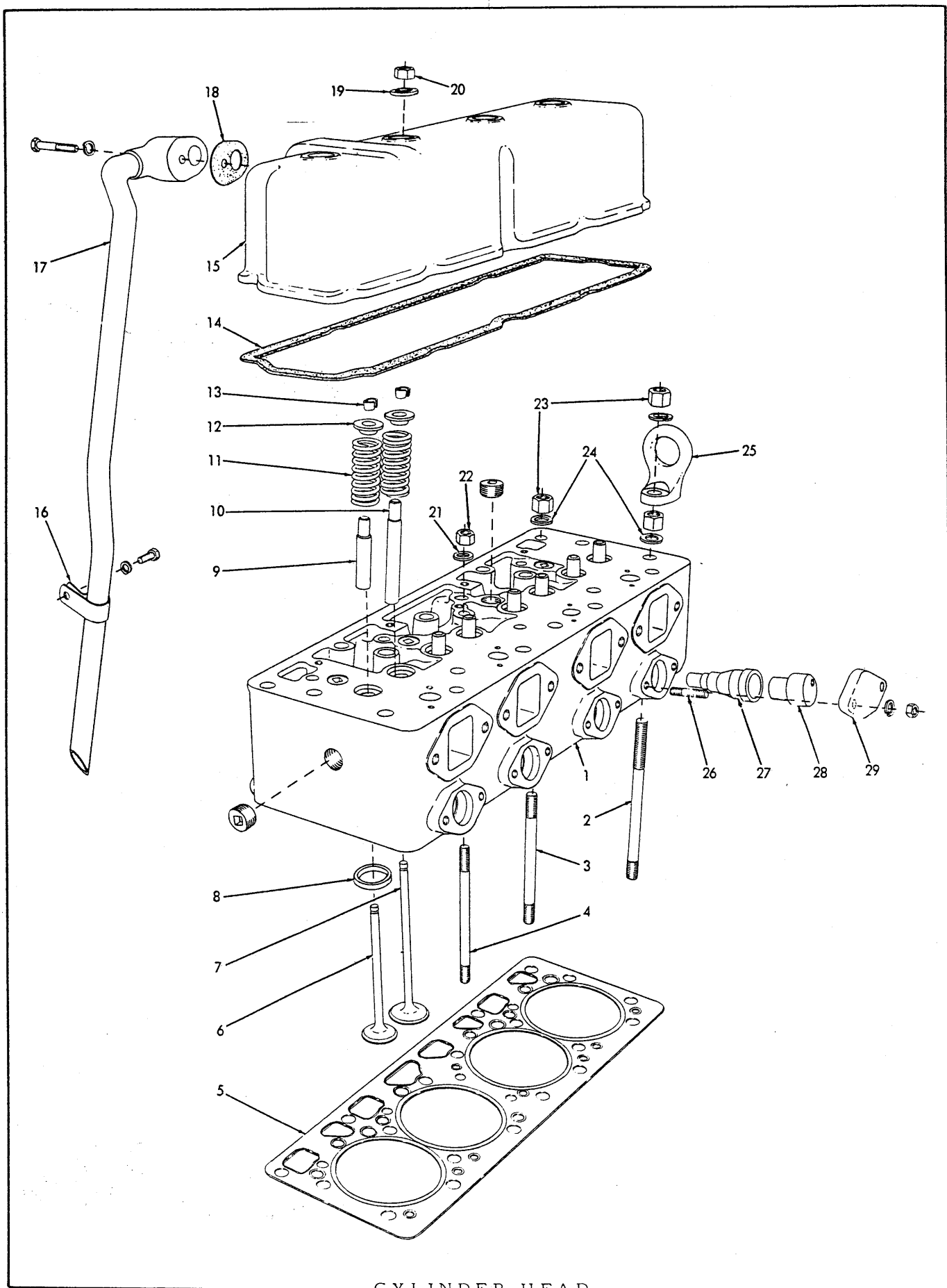
CYLINDER HEAD
