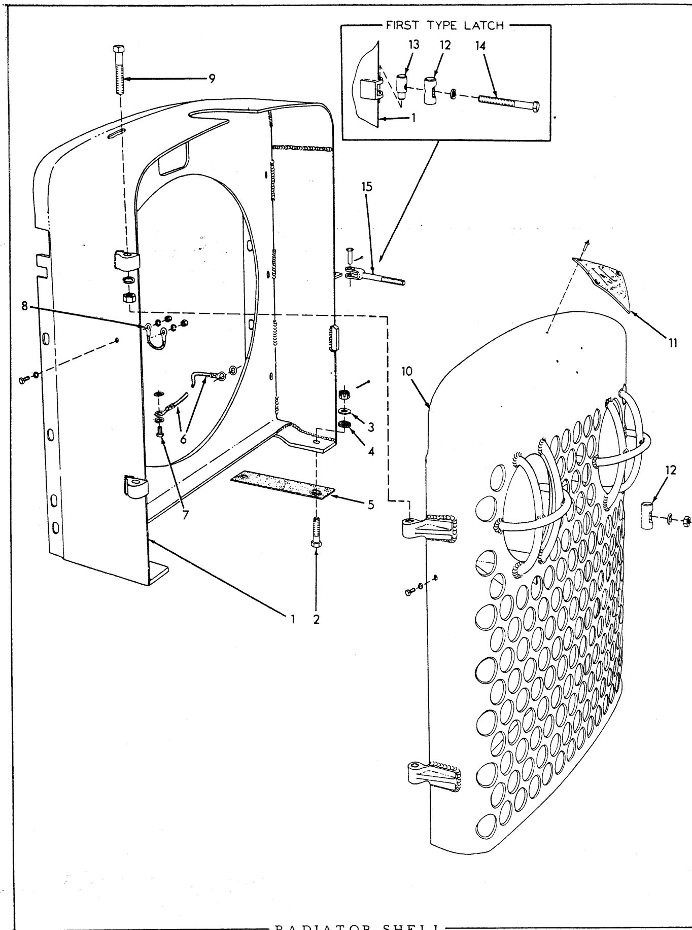
RADIATOR SHELL
