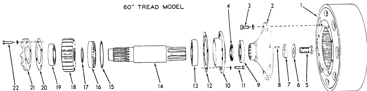
FINAL DRIVE PINION SHAFT
