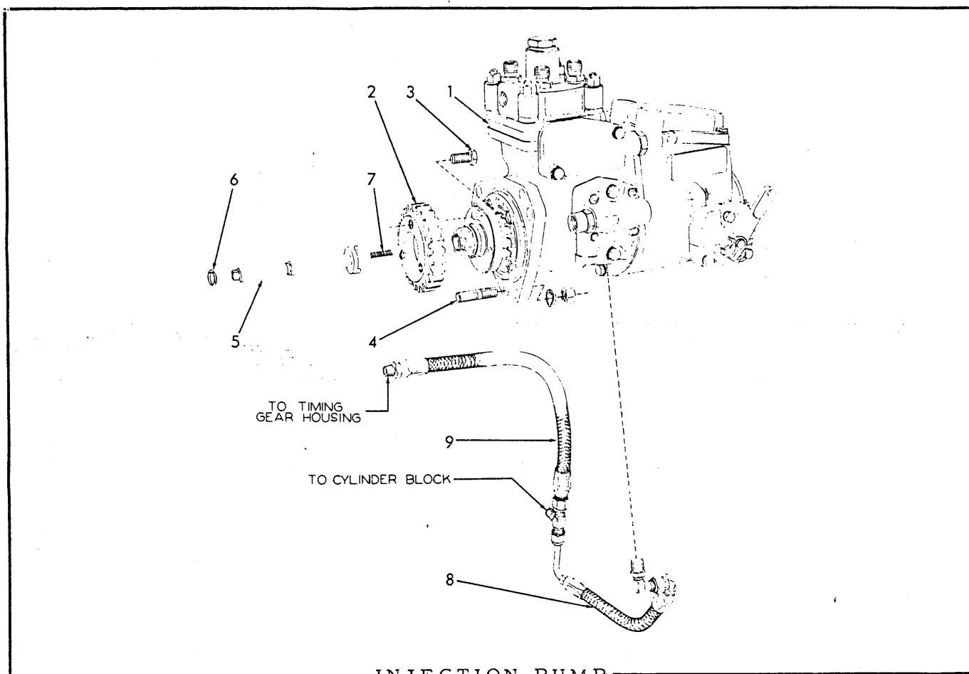
INJECTION PUMP
