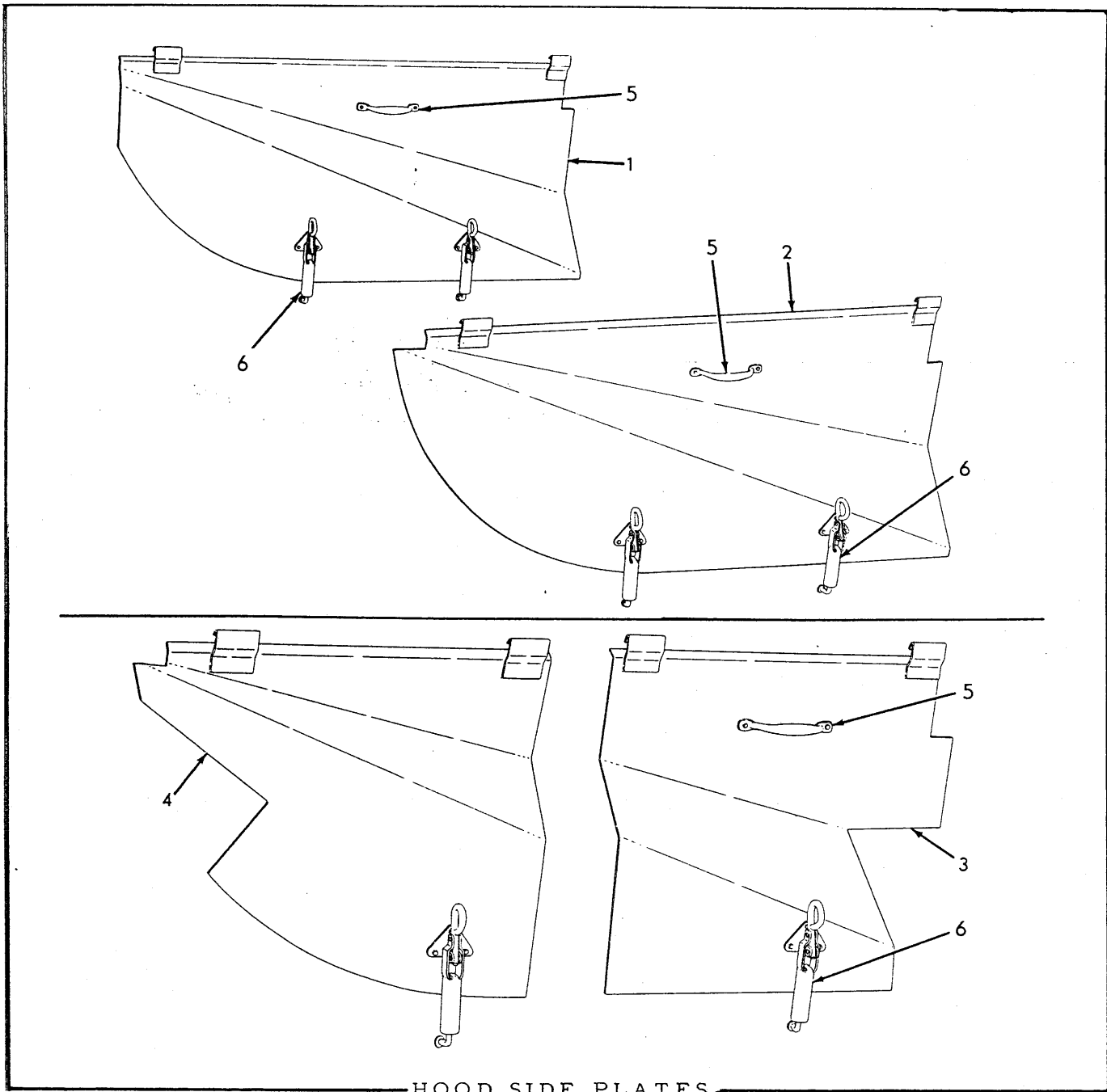
HOOD SIDE PLATES
