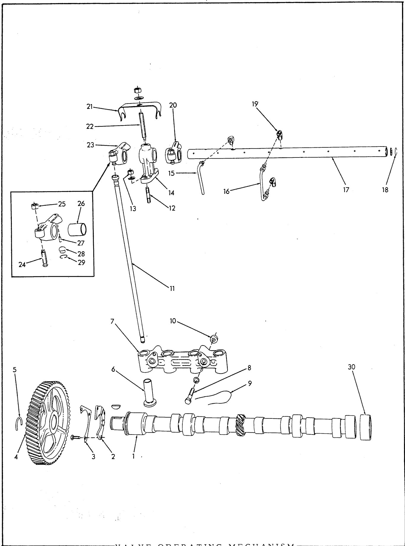
VALVE OPERATING MECHANISM
