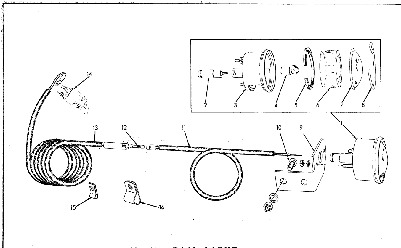
TAIL LIGHT
