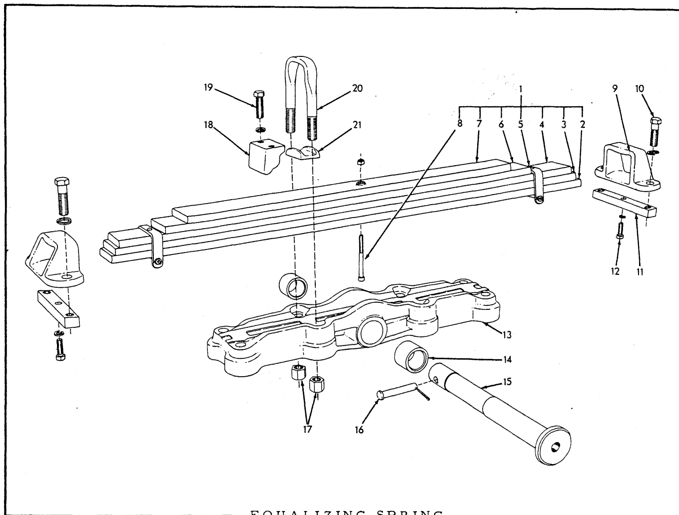
EQUALIZING SPRING
