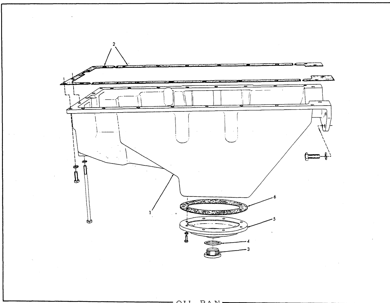
OIL PAN
