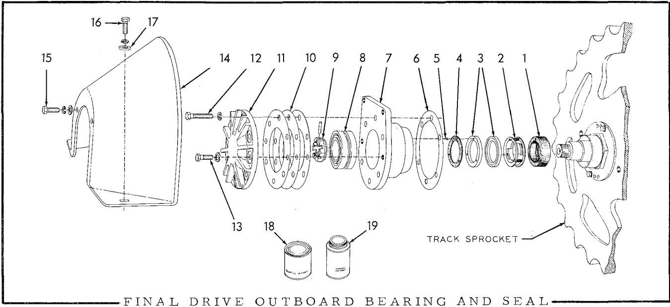
FINAL DRIVE OUTBOARD BEARING AND SEAL
