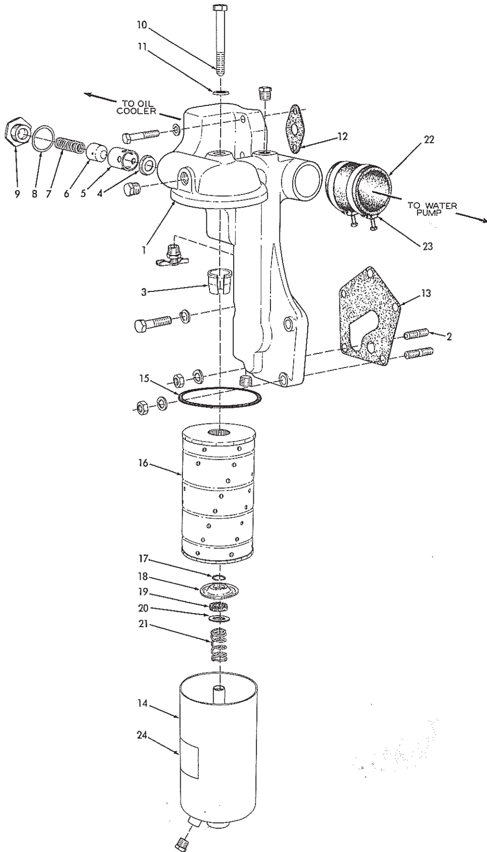
OIL FILTER
