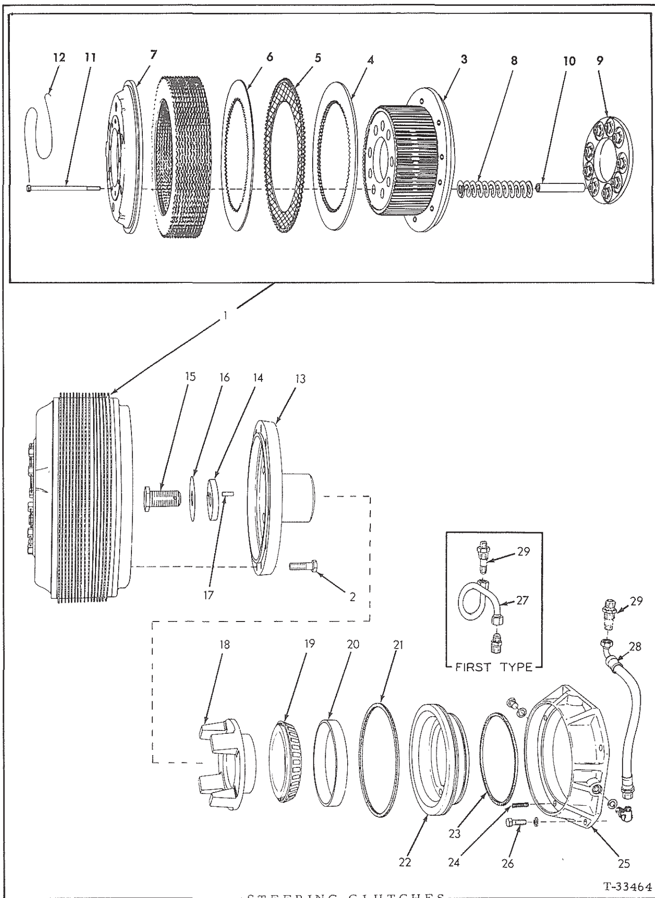
STEERING CLUTCHES
