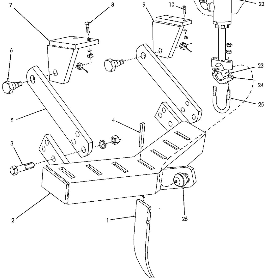
SCARIFIER (First type)
