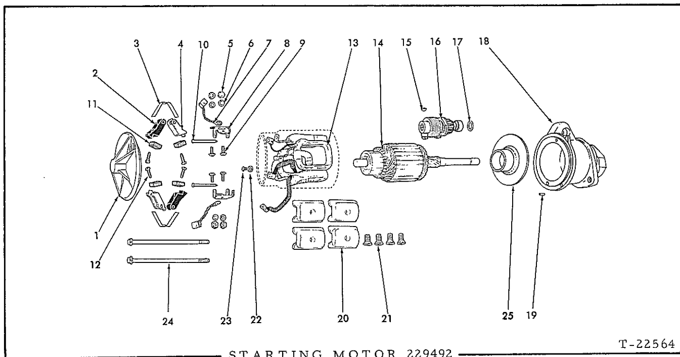
STARTING MOTOR 229492
