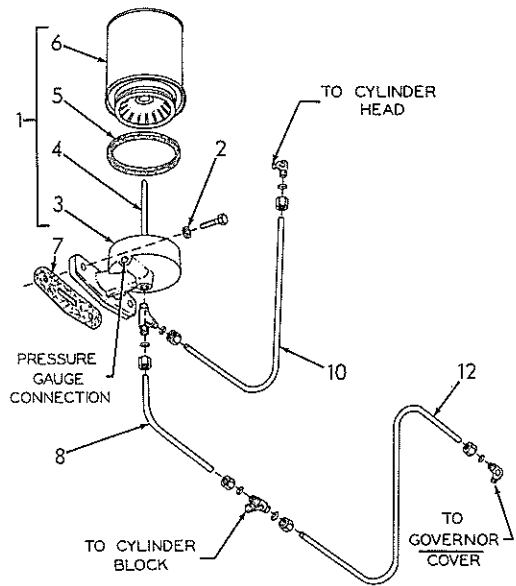
MODEL WD-45 ENGINE
