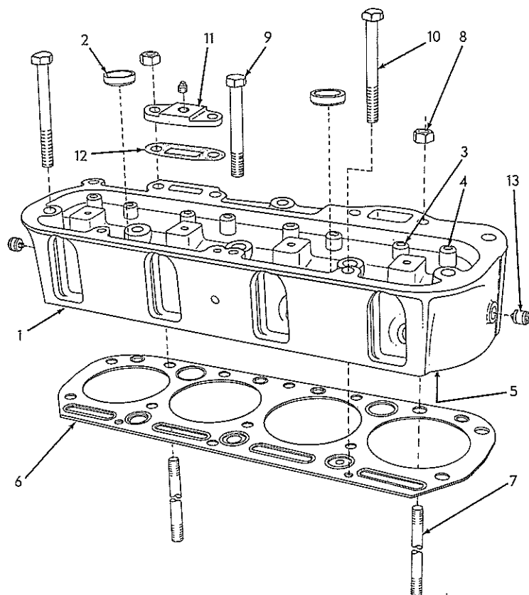
CYLINDER HEAD
