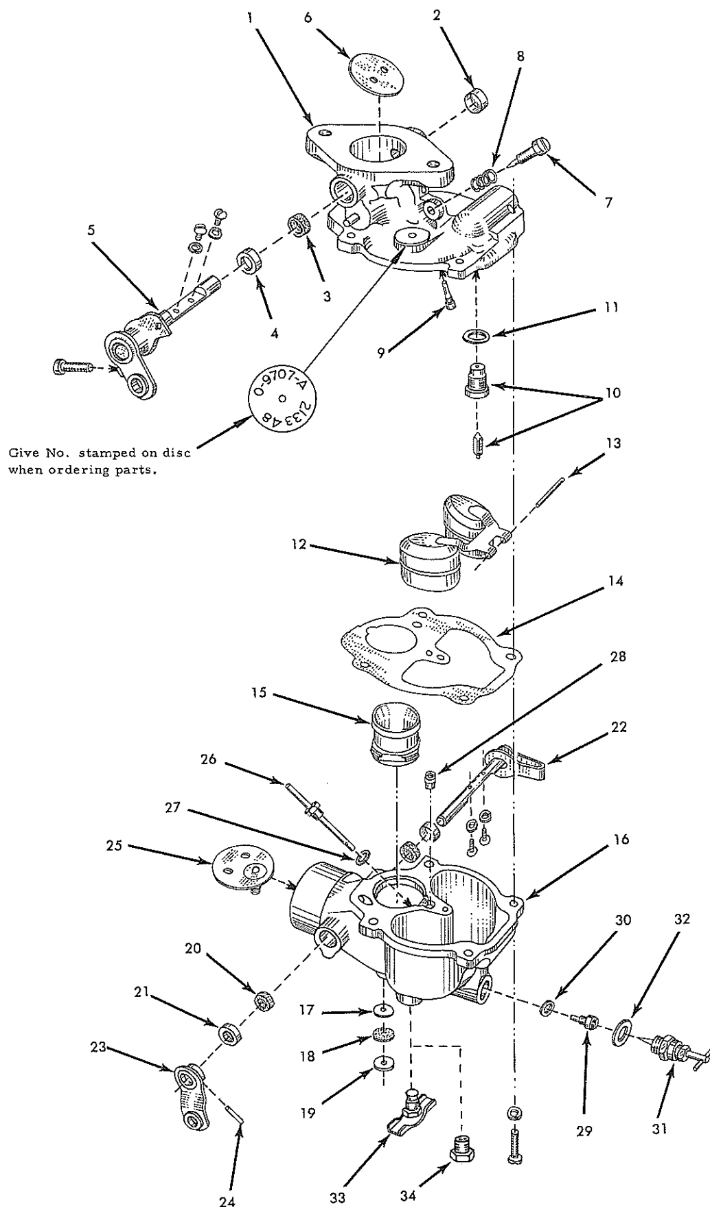
CARBURETOR ASSEMBLY 213348
