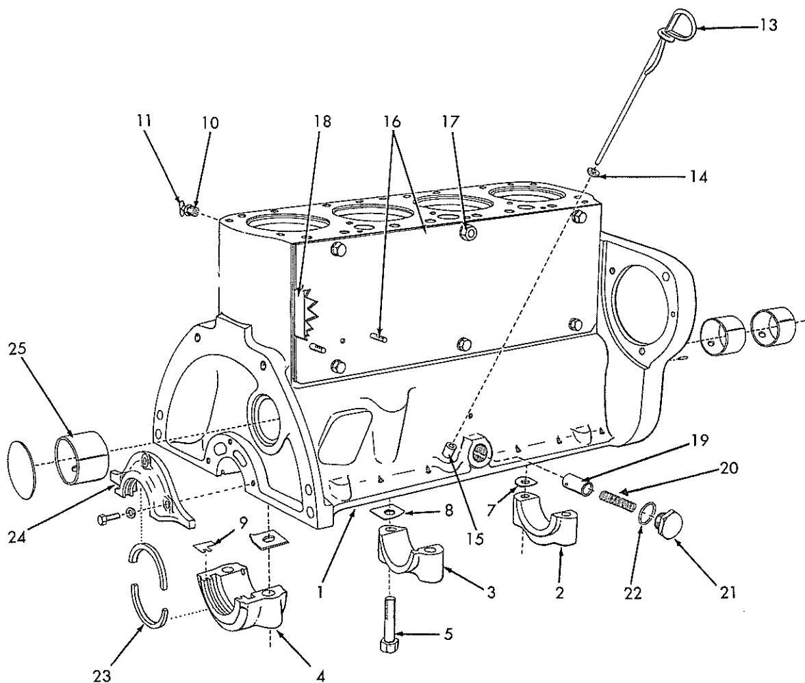
CYLINDER BLOCK
