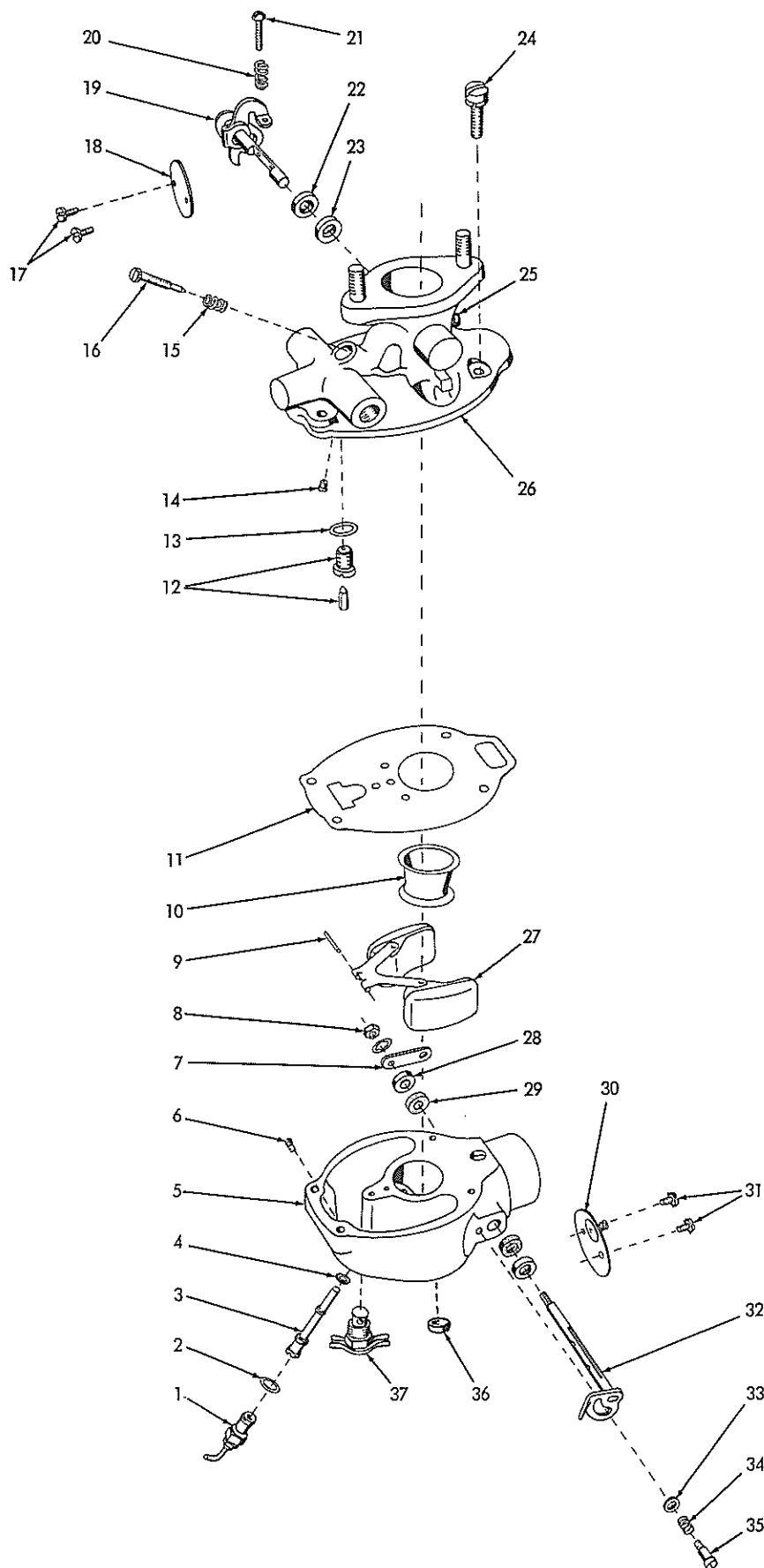
CARBURETOR ASSEMBLIES 226275 and 231431
