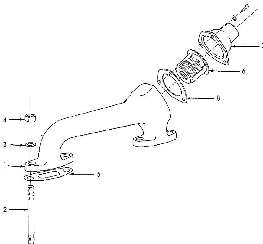
WATER MANIFOLD
