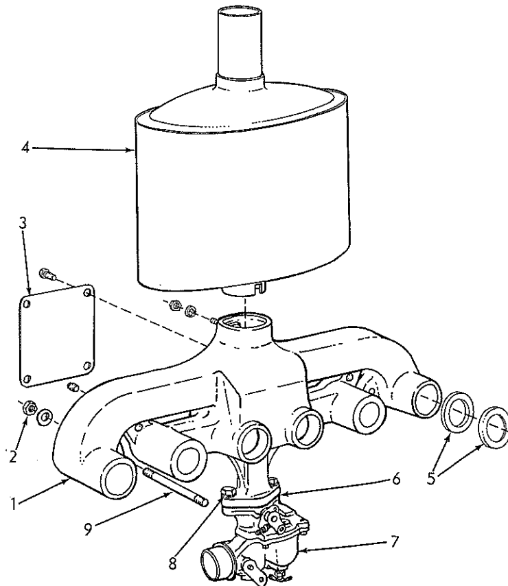
MANIFOLD AND CARBURETOR (For gasoline)
