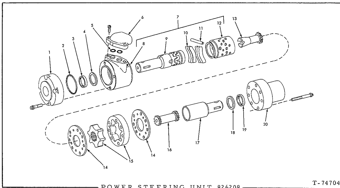
POWER STEERING UNIT 826208
