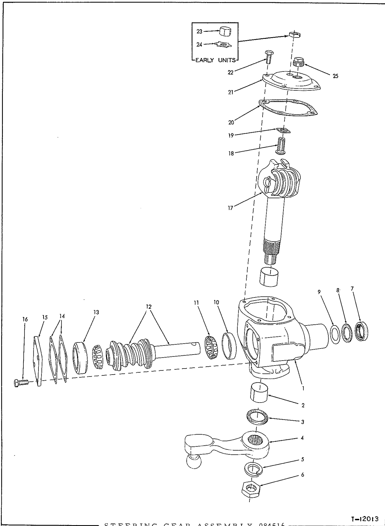
STEERING GEAR ASSEMBLY 084516
