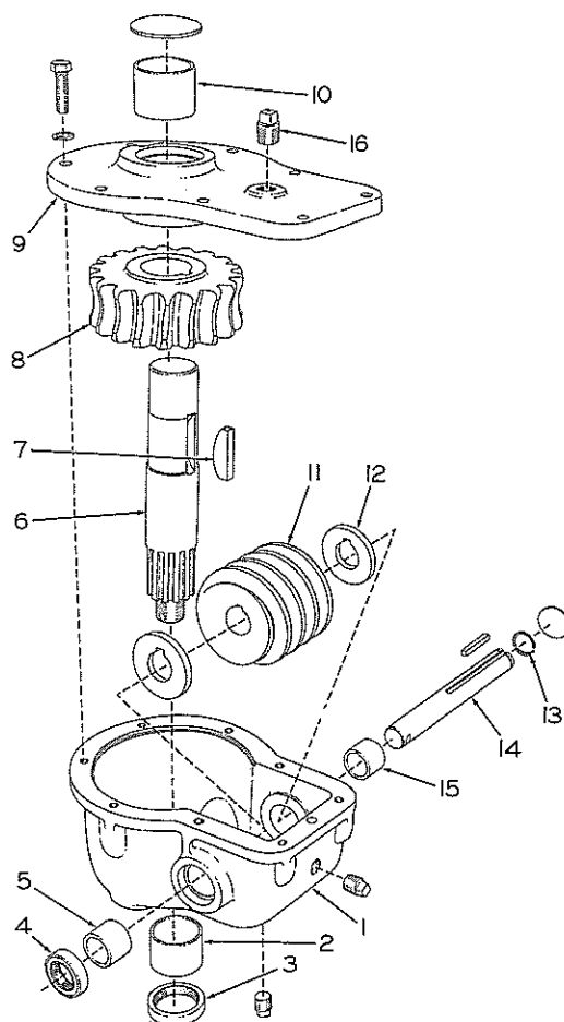
CIRCLE TURN PARTS
