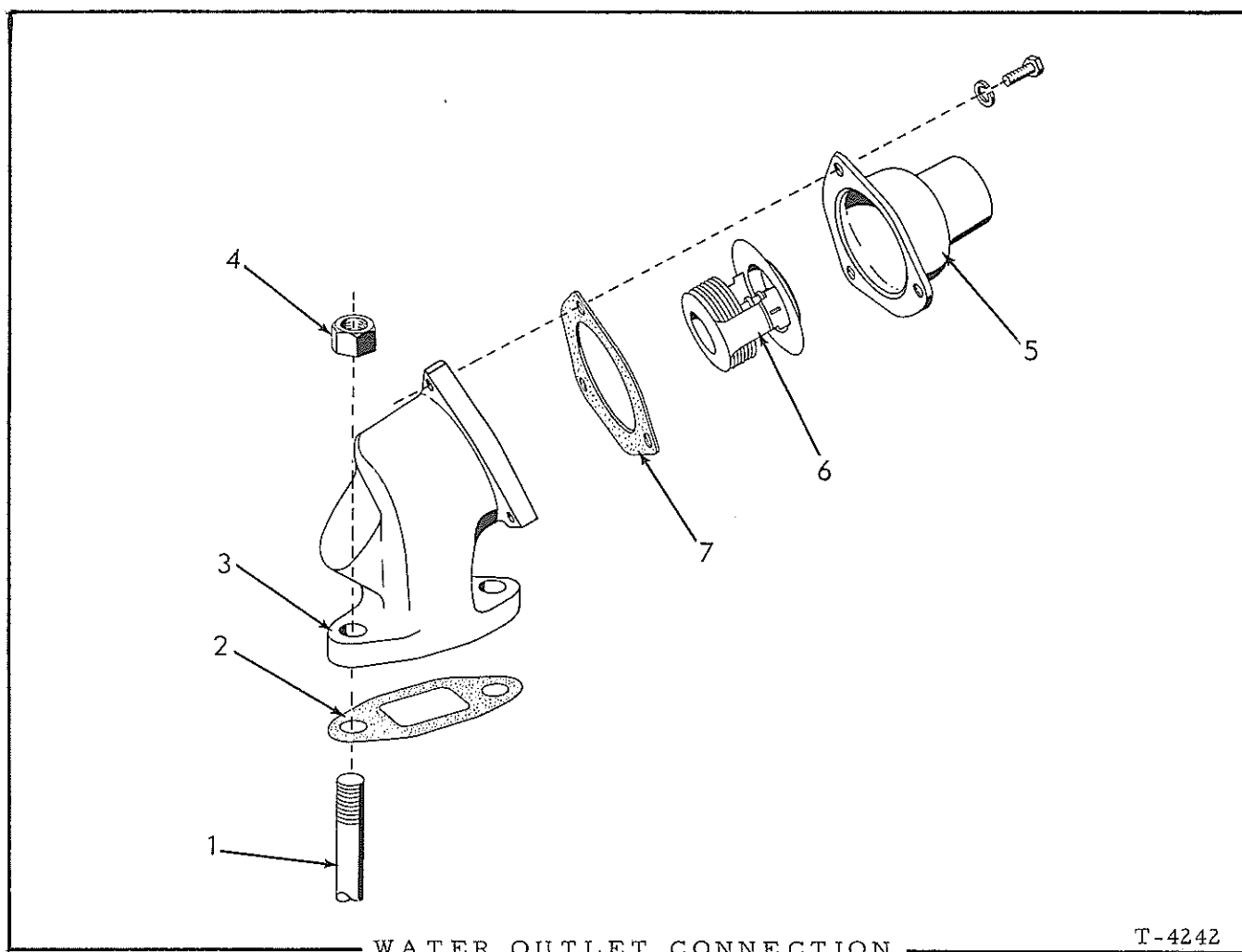
WATER OUTLET CONNECTION
