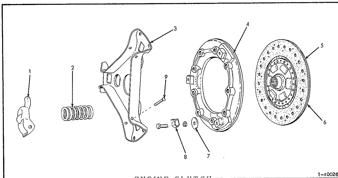
ENGINE CLUTCH (Auburn)
