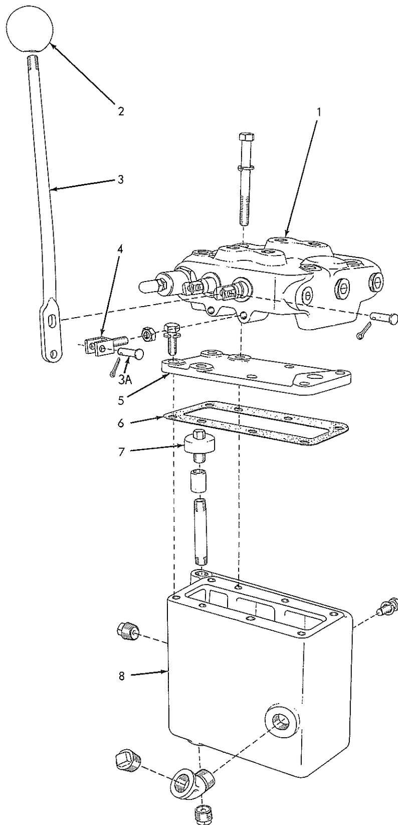
HYDRAULIC CONTROLS (First type)
