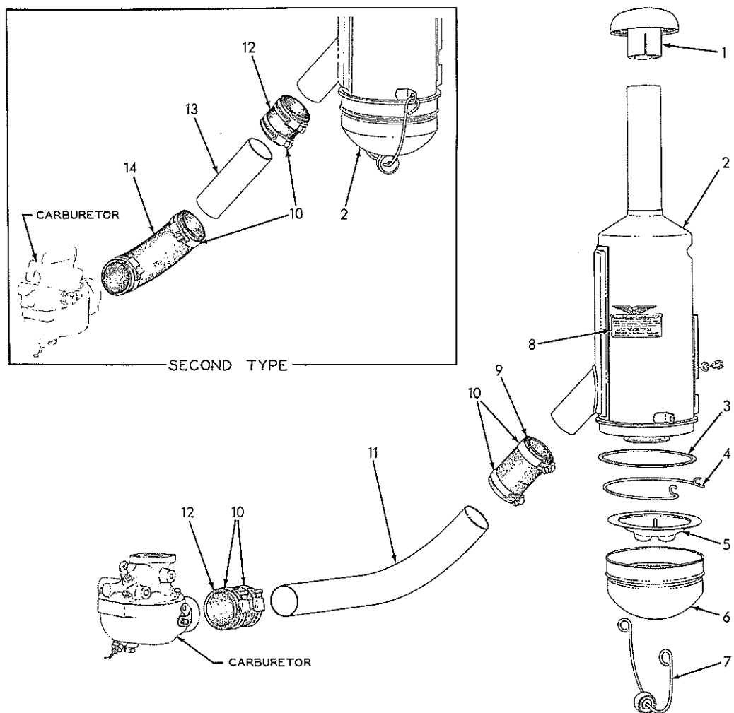
AIR CLEANER (Oil-bath)
