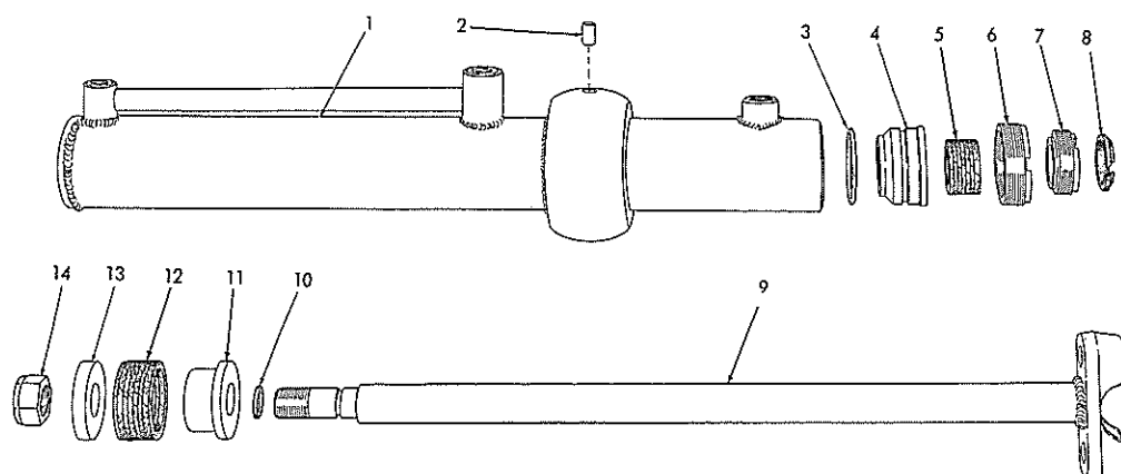
LIFT CYLINDER PARTS (HUSCO)
