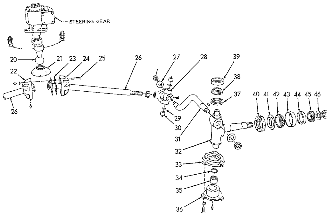
WHEEL LEAN STEERING LINKAGE DETAILS (Second type) T-12578
