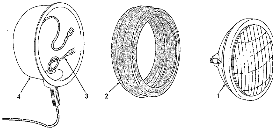
HEAD LIGHT PARTS
