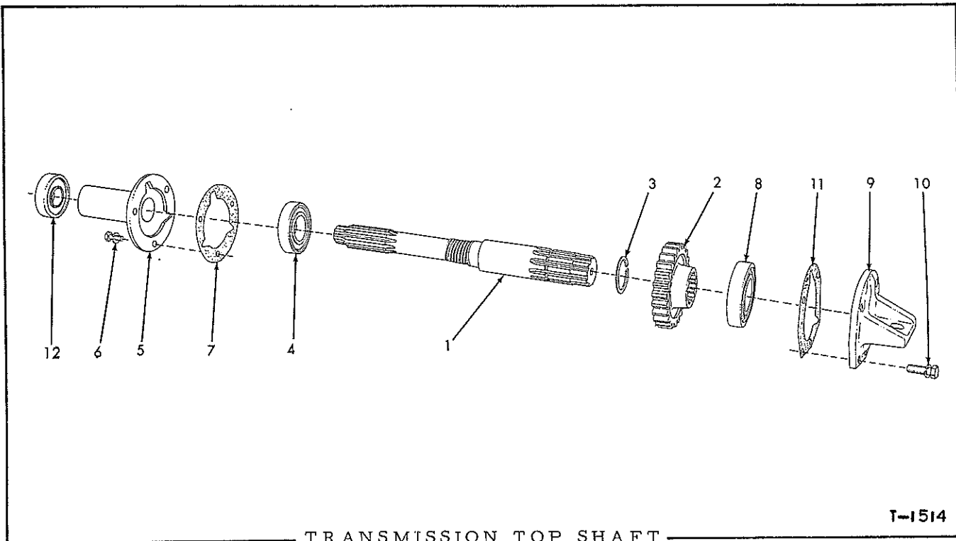
TRANSMISSION TOP SHAFT
