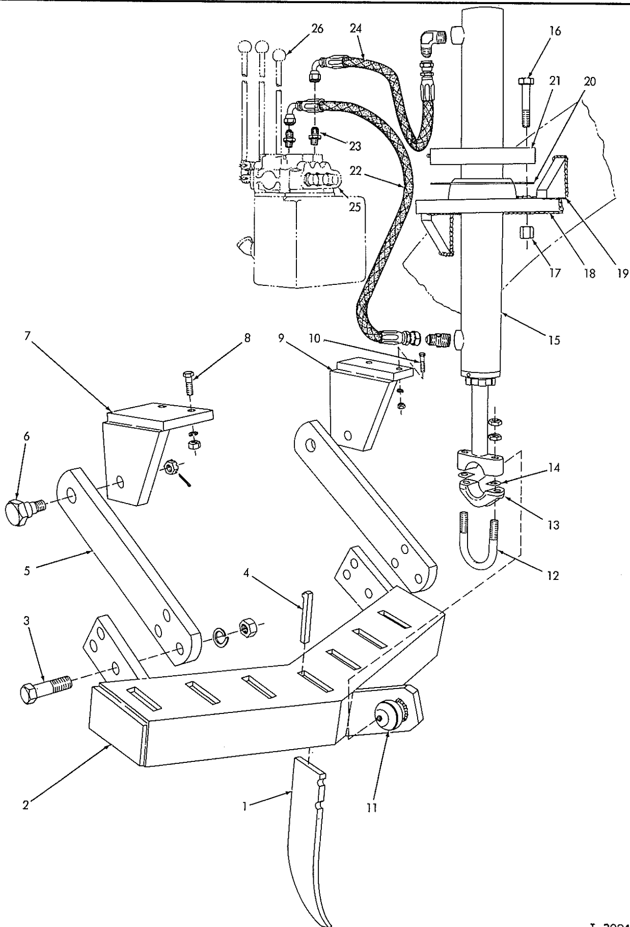
SCARIFIER (Second type)
