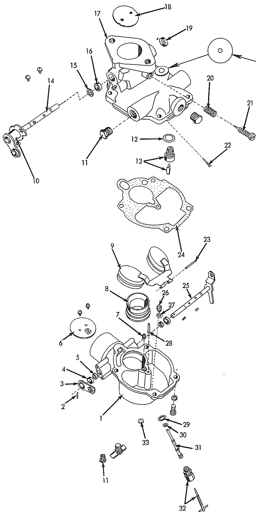
CARBURETOR ASSEMBLY 229342
