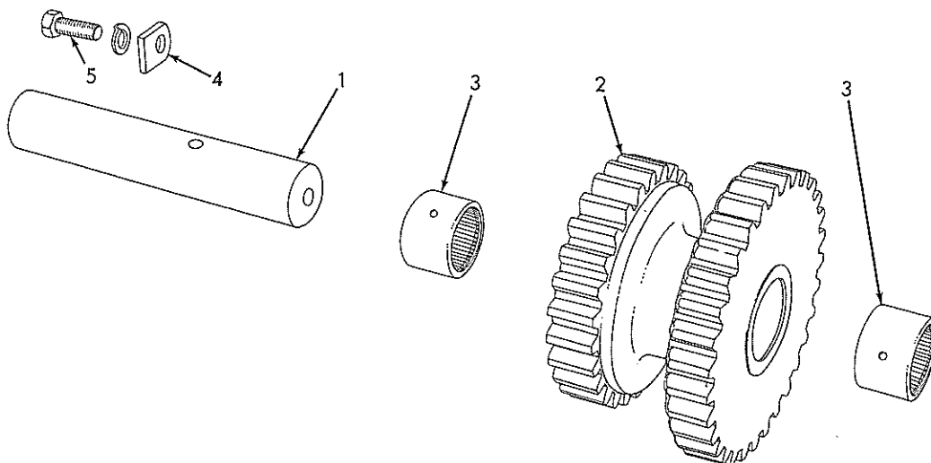
TRANSMISSION REVERSE SHAFT
