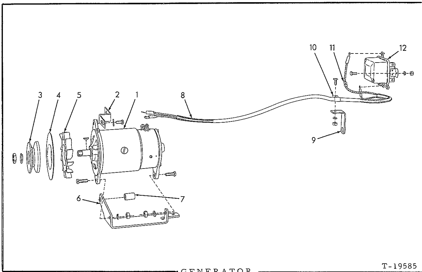
GENERATOR
