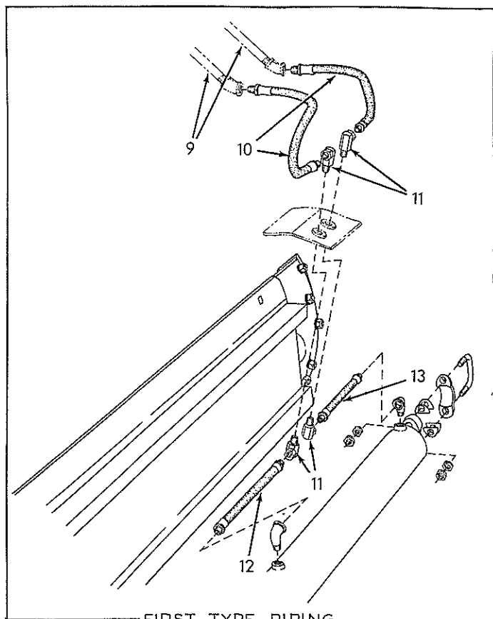
FIRST TYPE PIPING
