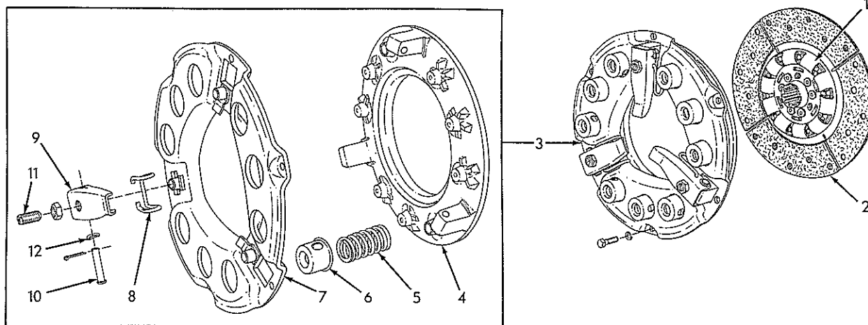
ENGINE CLUTCH (Rockford)
