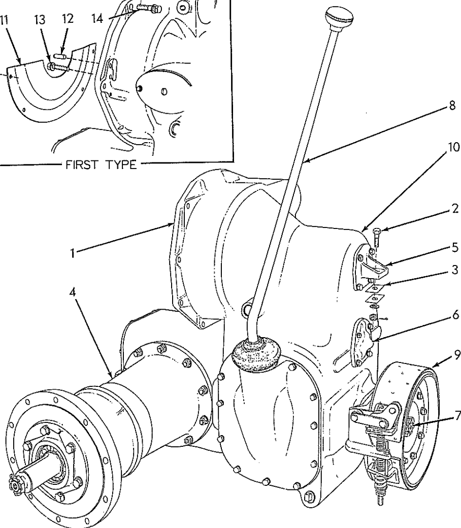
TRANSMISSION AND REAR AXLE
