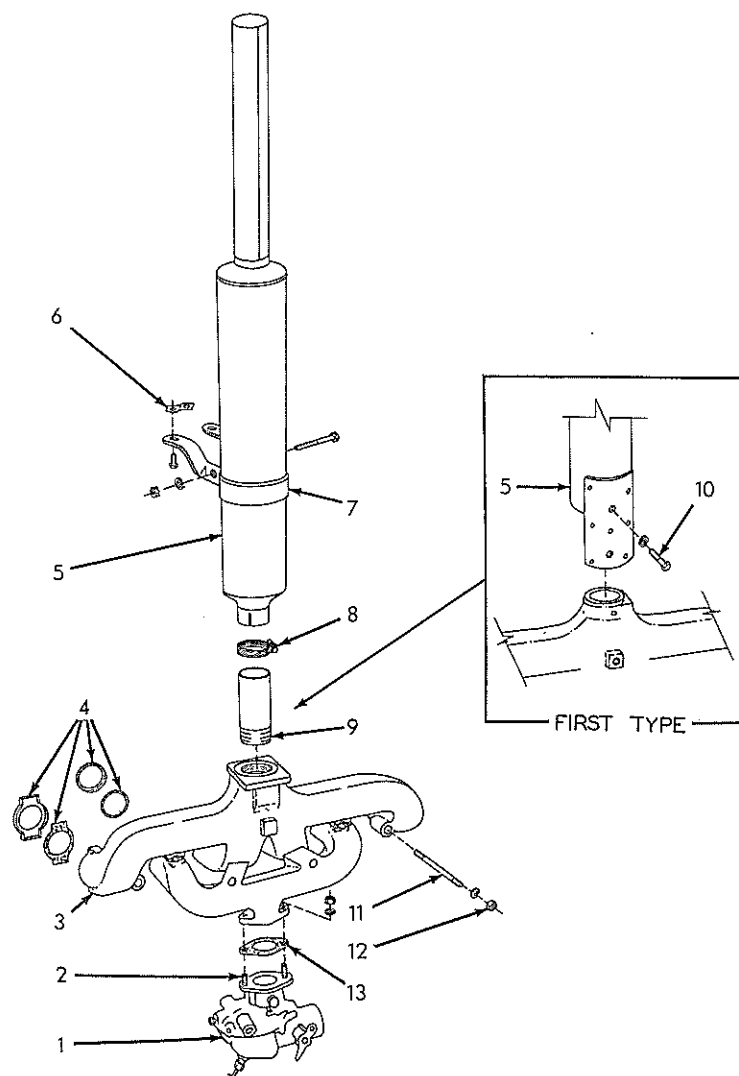
MANIFOLD AND CARBURETOR (For gasoline)
