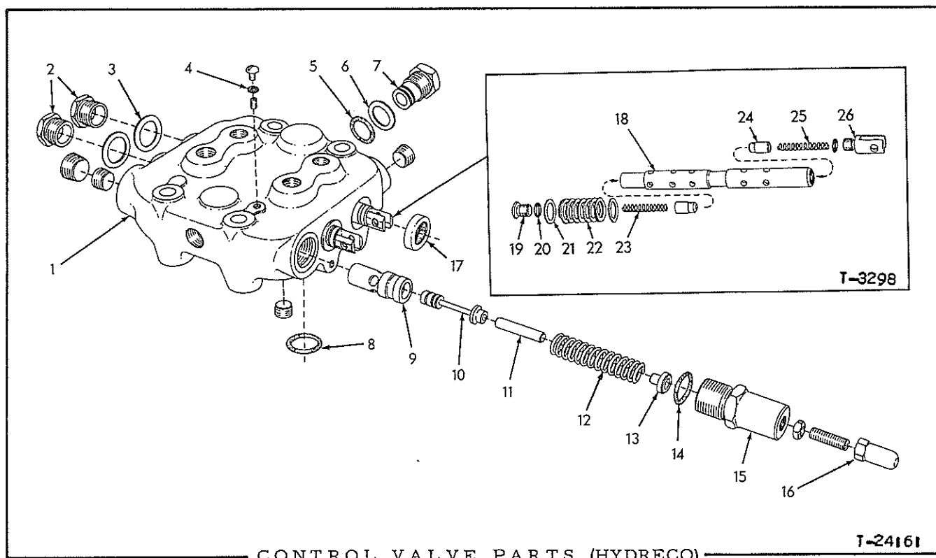
CONTROL VALVE PARTS (HYDRECO)
