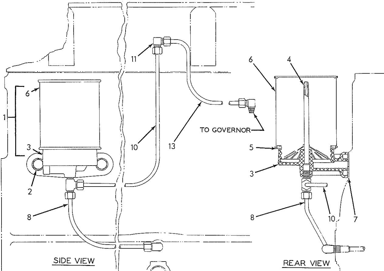
MODEL 17 ENGINE
