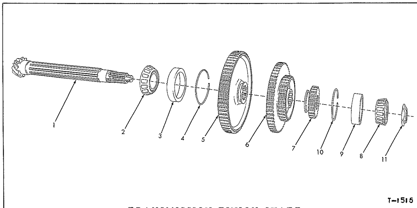
TRANSMISSION PINION SHAFT
