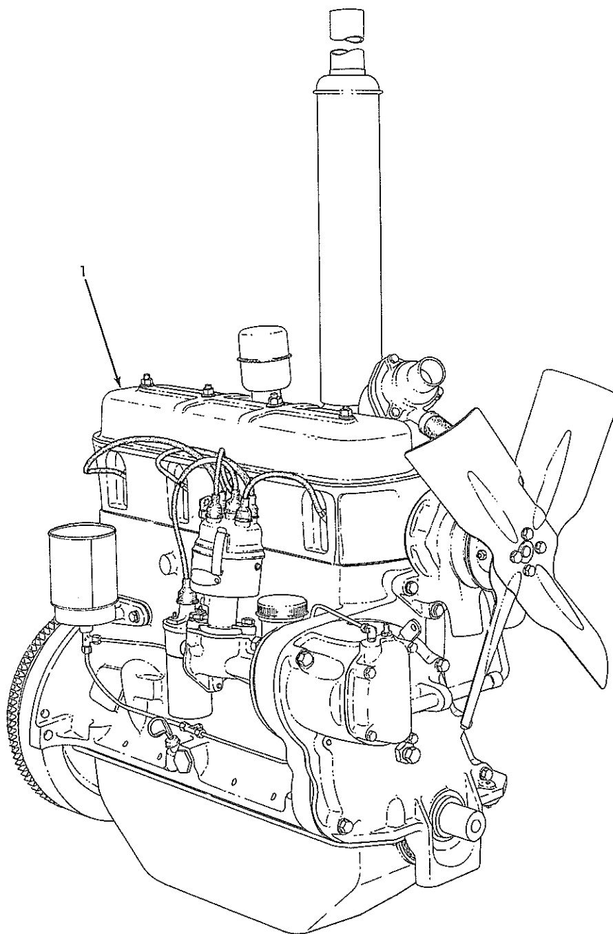
ENGINE ASSEMBLY (Model WD-45)
