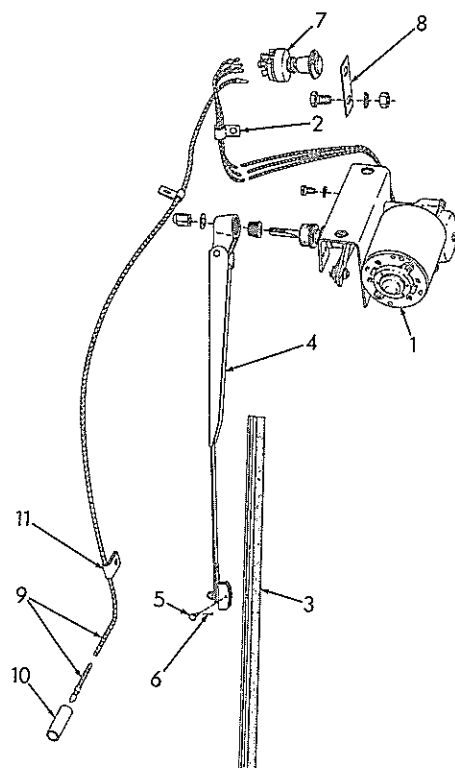
WINDSHIELD WIPER
