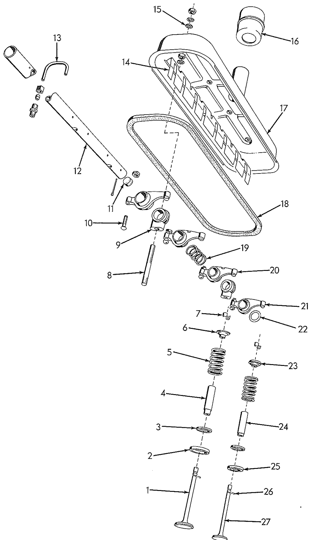
VALVES AND ROCKER ARMS (Second type)
