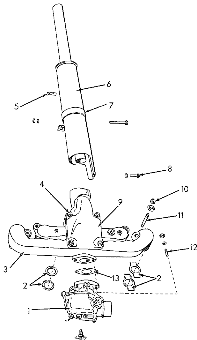
MANIFOLD AND CARBURETOR (For low-grade fuels)
