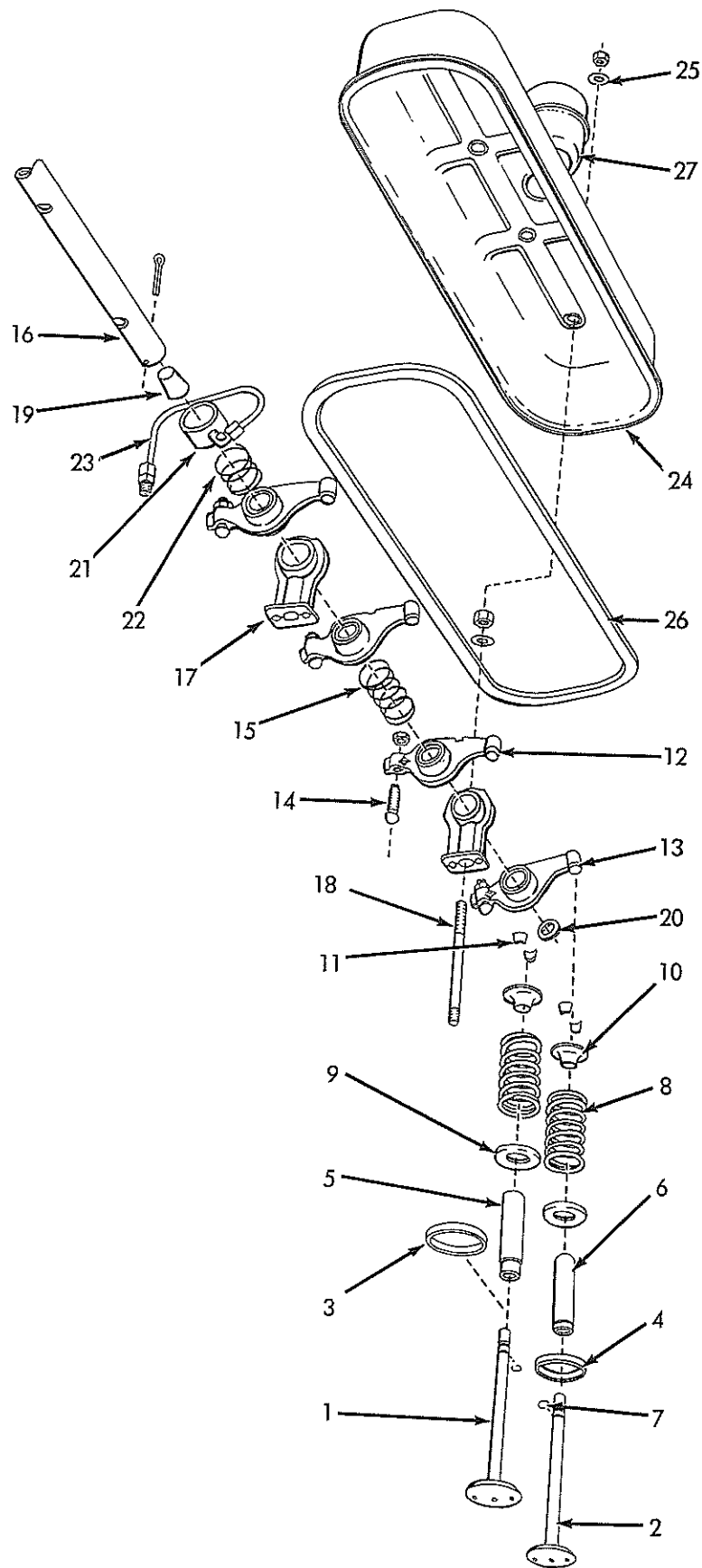
VALVES AND ROCKER ARMS (First type)
