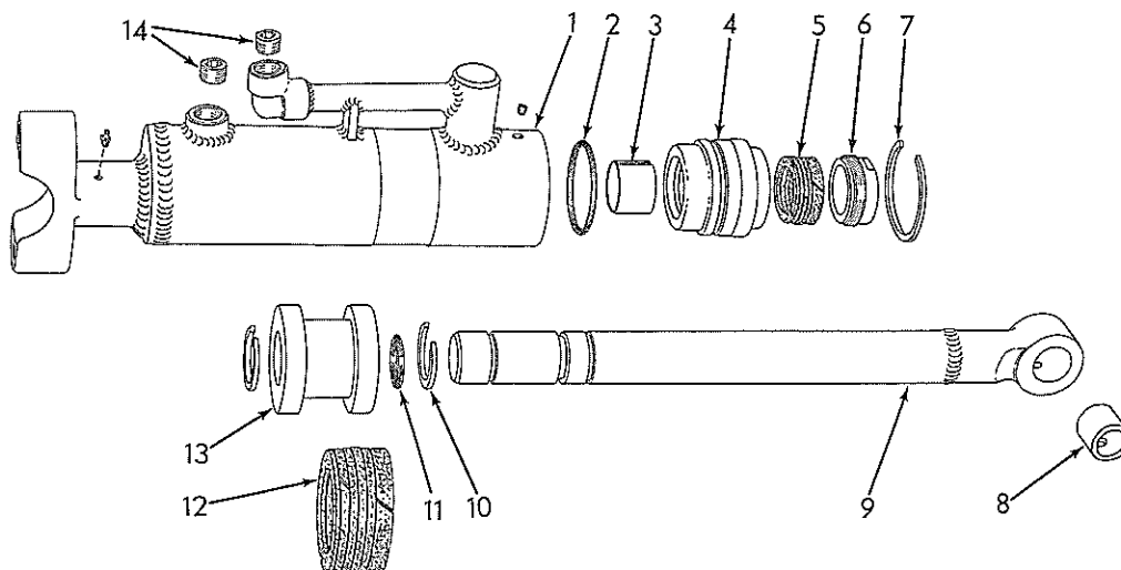
WHEEL LEAN CYLINDER PARTS (HYDRECO)
