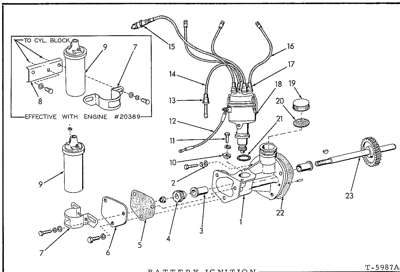
BATTERY IGNITION
