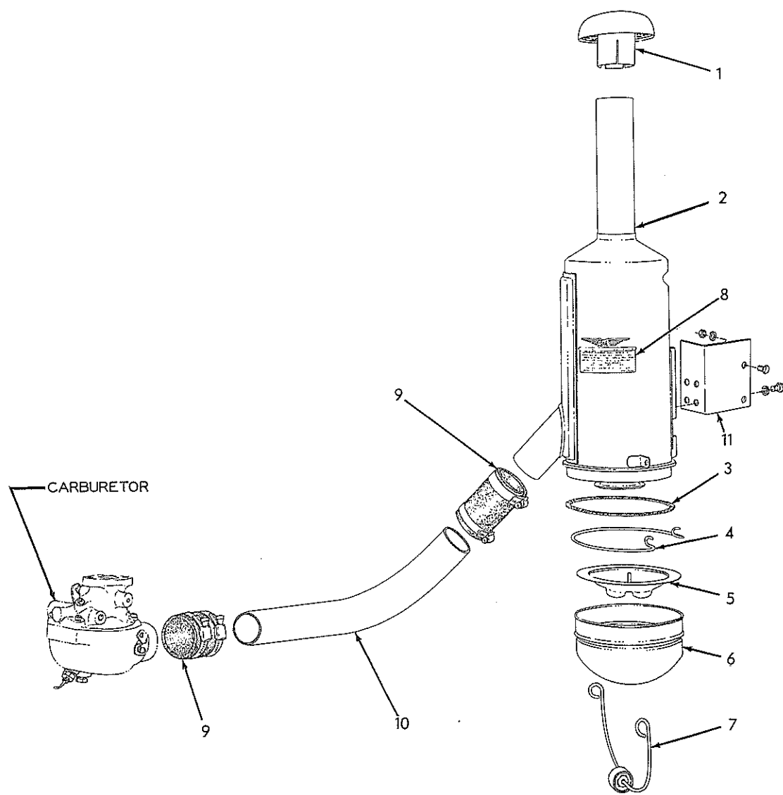
AIR CLEANER (Oil-bath)
