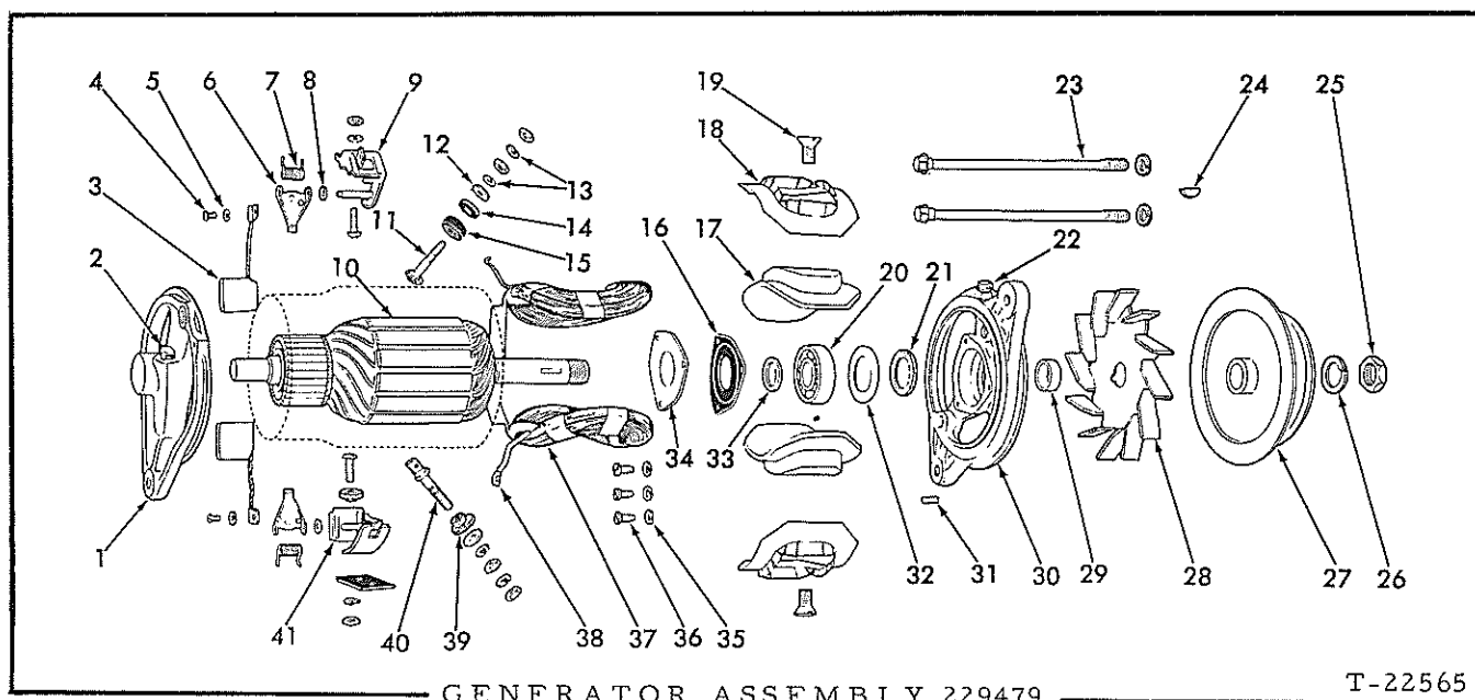
GENERATOR ASSEMBLY 229479
