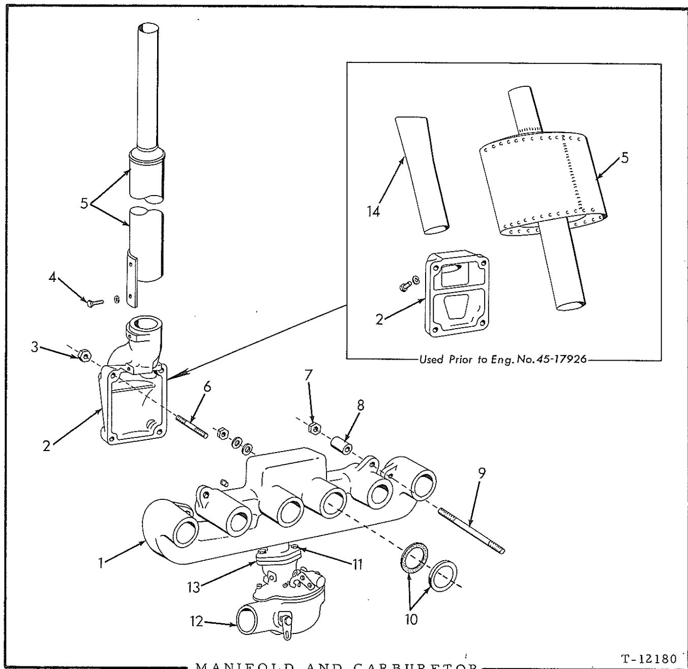
MANIFOLD AND CARBURETOR (For gasoline and low-grade fuels)
