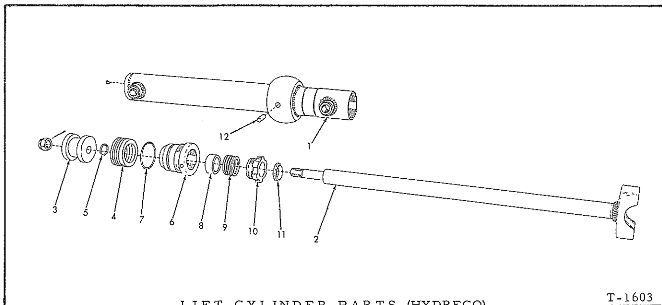
LIFT CYLINDER PARTS (HYDRECO)
