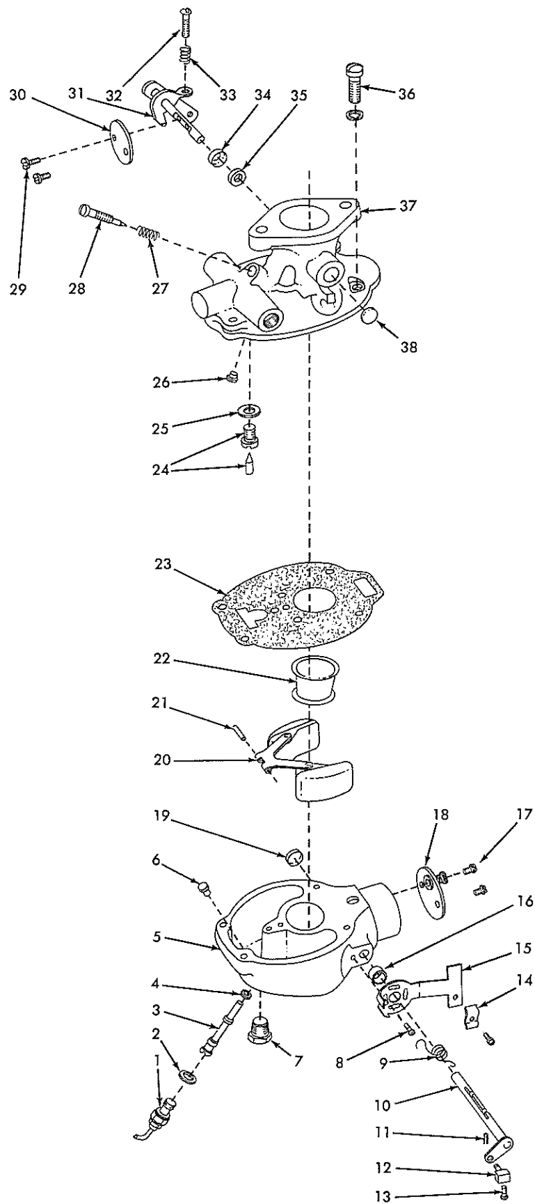
CARBURETOR ASSEMBLY 239961
