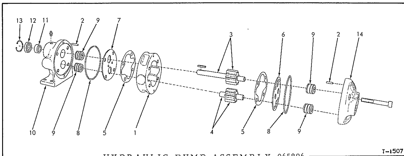
HYDRAULIC PUMP ASSEMBLY 065896
