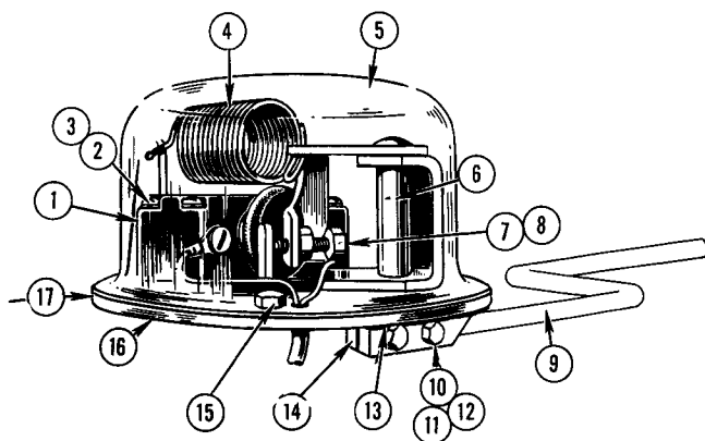
FIG. 3074C LIMIT SWITCH
