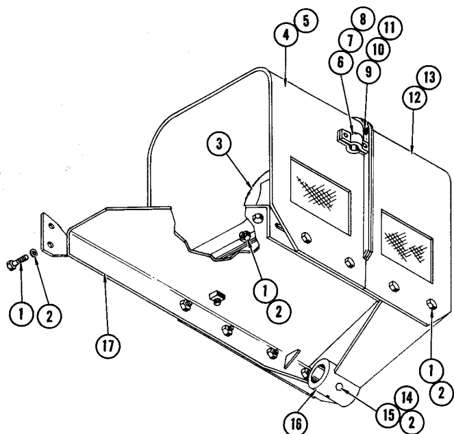
FIG. 3074A MOTOR COVER
