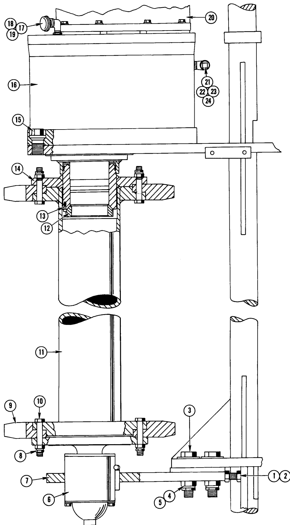
FIG. 3086 ELEVATOR DRIVE
