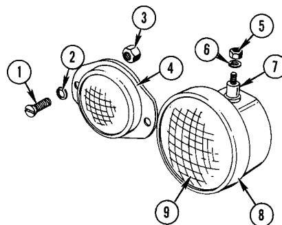
FIG. 3074D TAIL LIGHT & REFLECTOR
