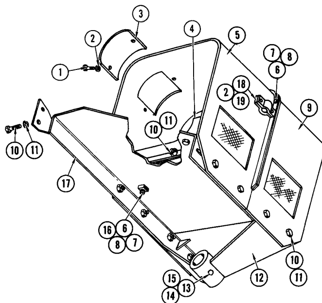
FIG. 3074B MOTOR COVER
