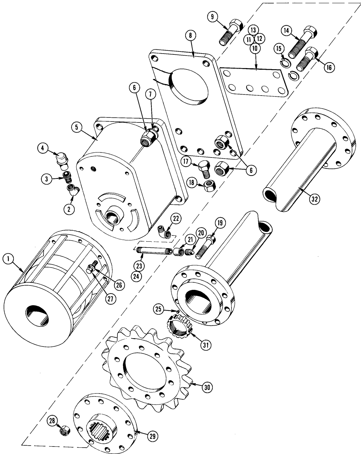
FIG. 3063 ELEVATOR DRIVE
