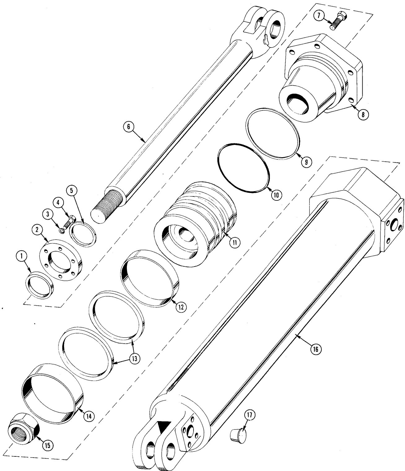
FIG. 3043 HYDRAULIC CYLINDER (HOIST, TAILGATE & ROLLING BOTTOM)
