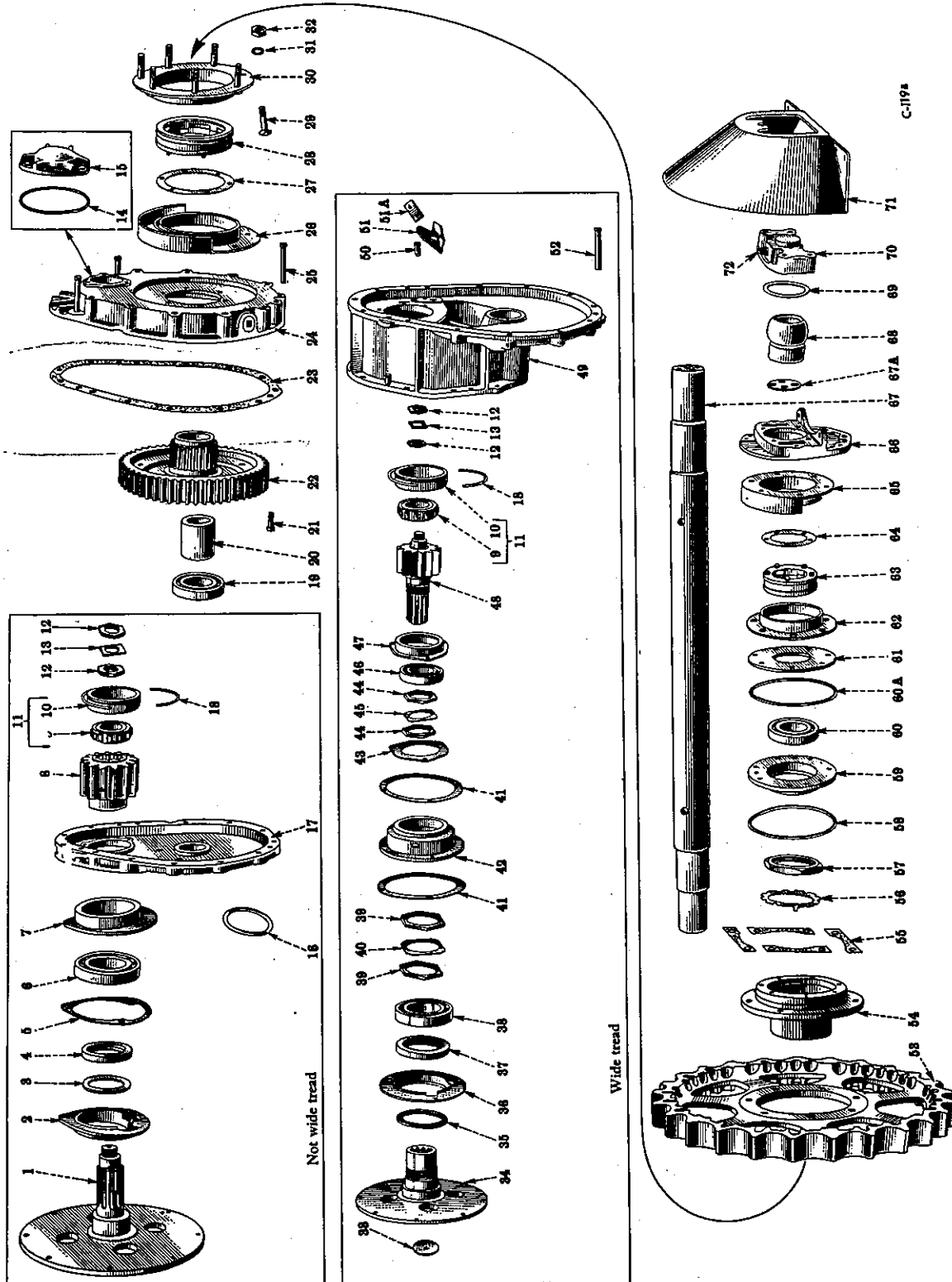
TRACK DRIVE—SPROCKET DRIVE, SHAFT, PINION AND SPROCKET TRACK FRAME PIVOT SHAFT
