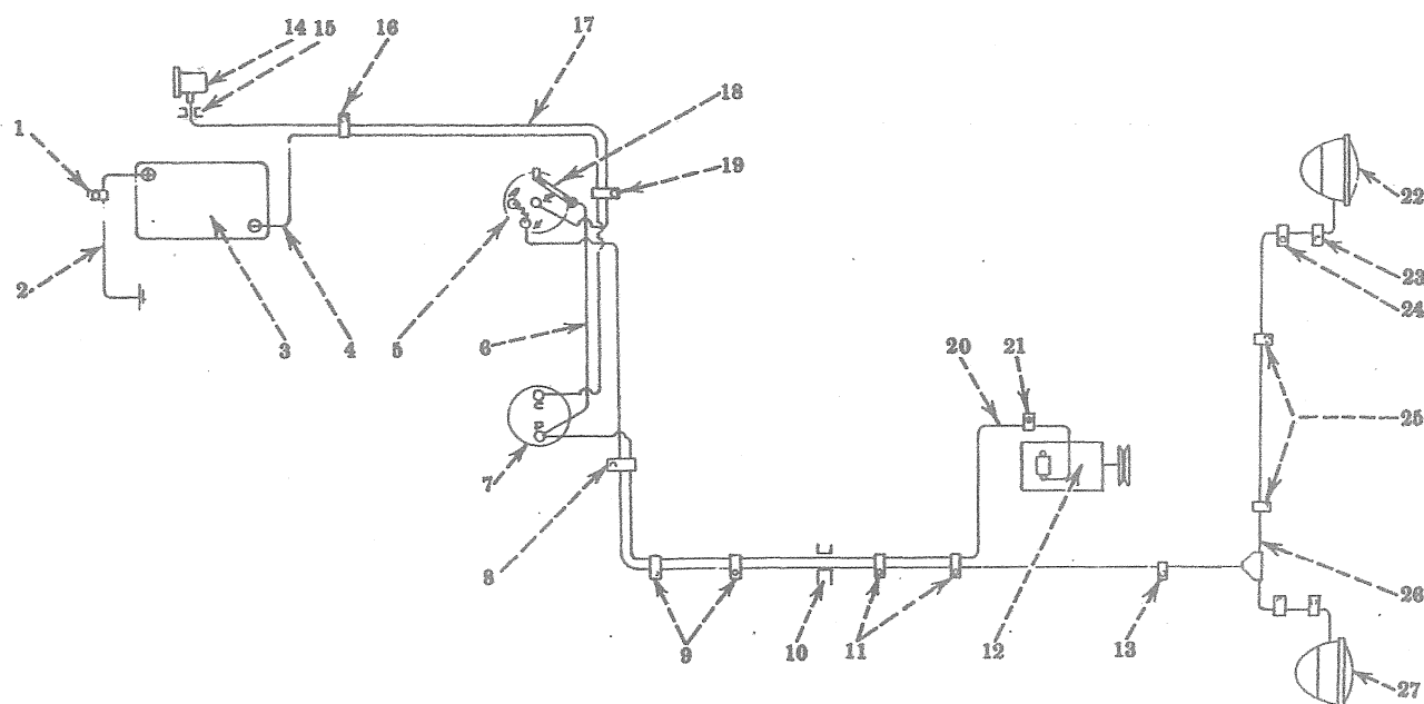
Wiring Diagram—Electric Lighting—special
