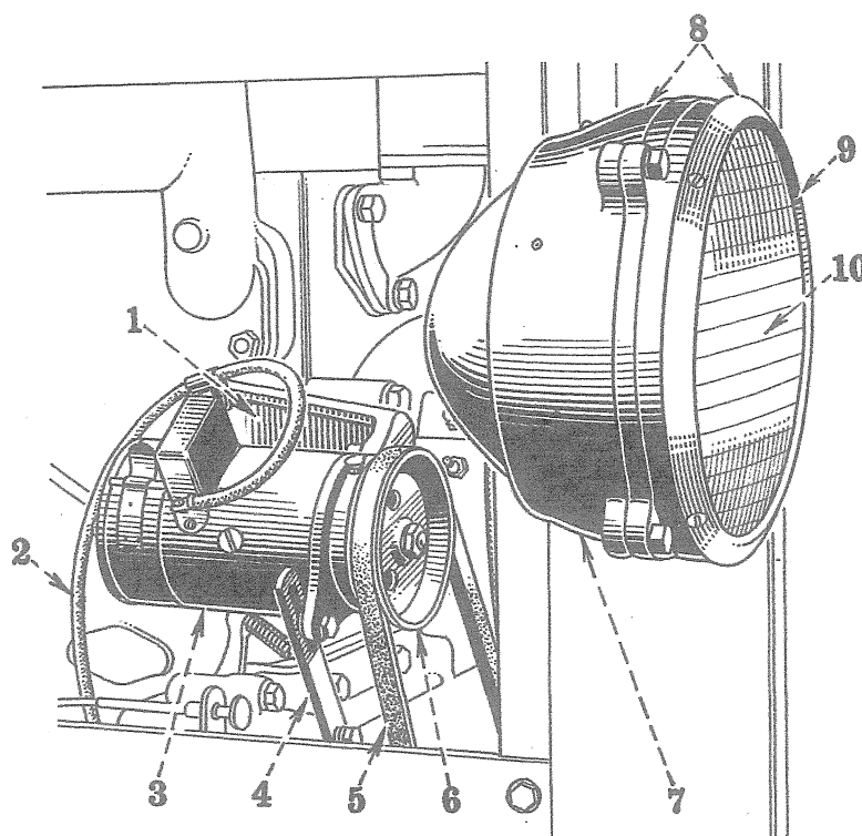
Front Lamp and Generator Mounting—Electric Lighting—special (Delco-Remy) (Diesel)
