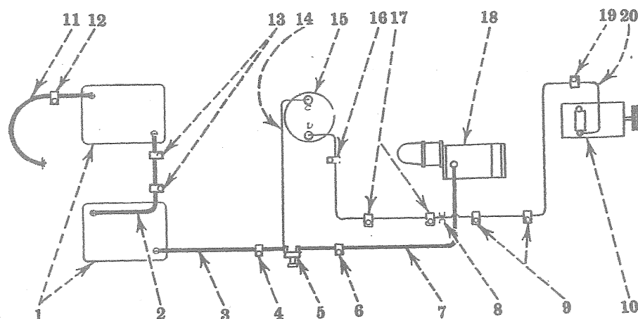
Wiring Diagram—Electric Starting—special (Delco-Remy) (Rear battery mounting) (Diesel)
