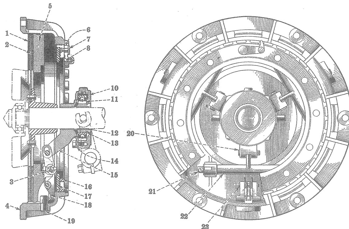
Over-Center Clutch (Hand Operated)
