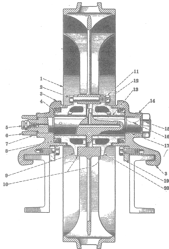
Front Idler
