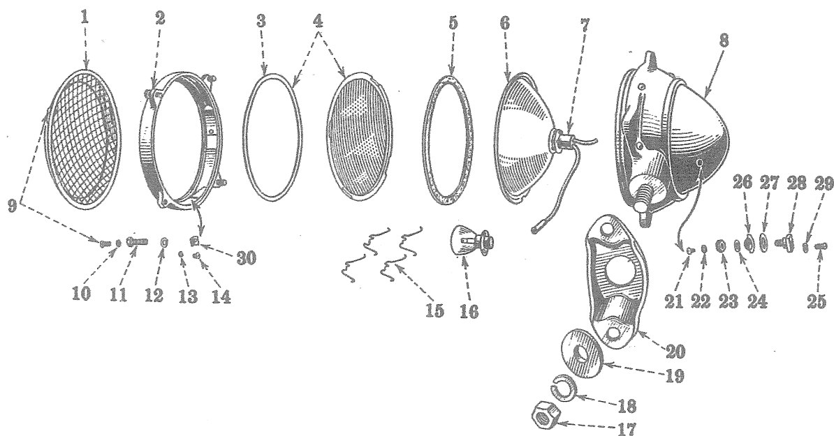
Head Lamp (Armored Type)
