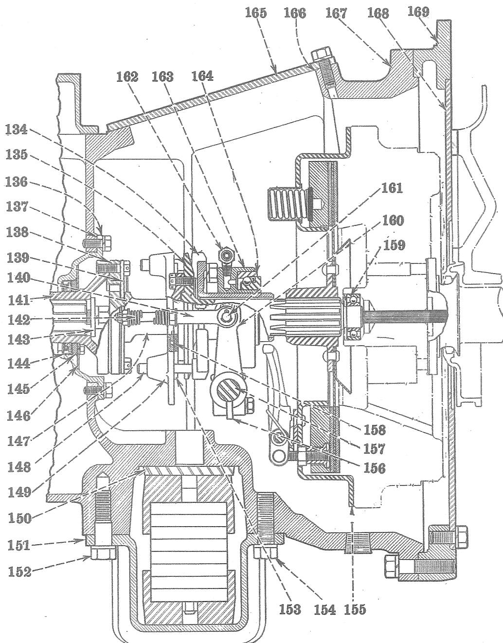
Single Plate Clutch and Clutch Control (Foot Operated—special) Equalizer Spring, Clutch and Transmission Joints also Main Frames
