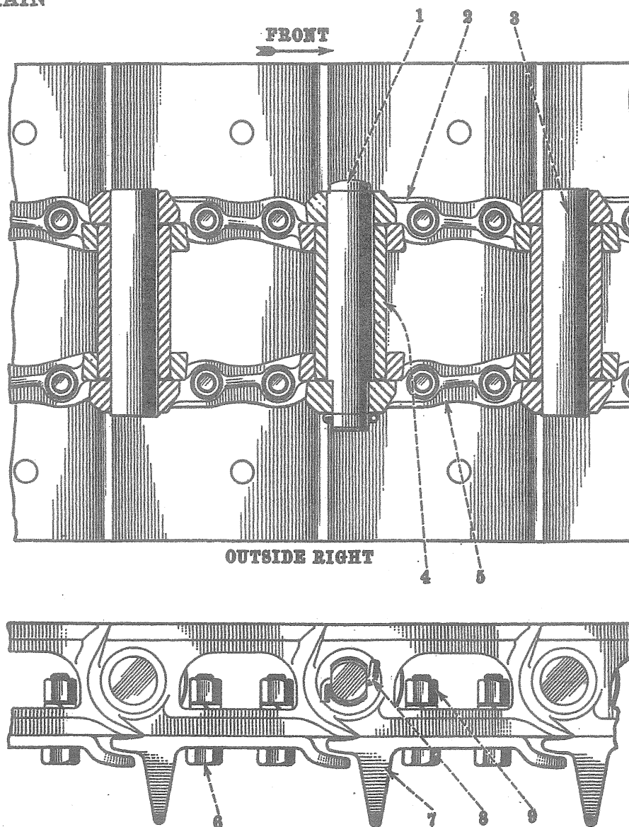
Track Chain.
