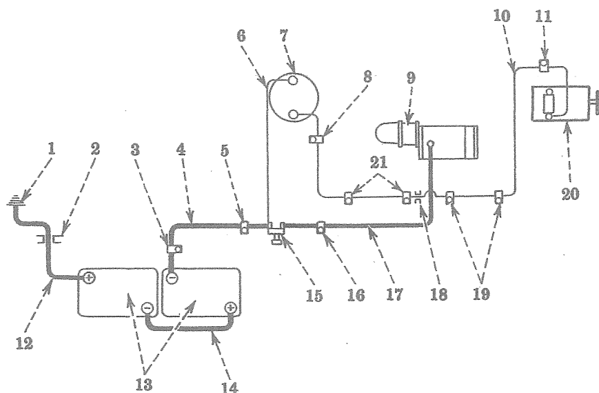
Wiring Diagram—Electric Starting—special
