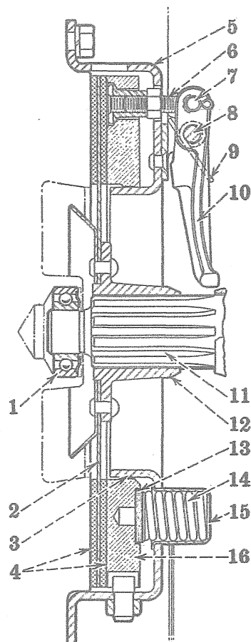
Single Plate Clutch, 14" (Foot Operated—special)
