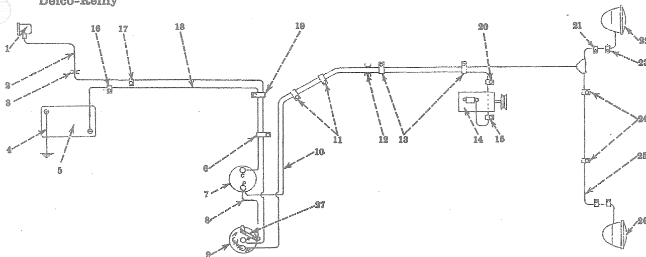
Wiring Diagram—Electric Lighting—special
