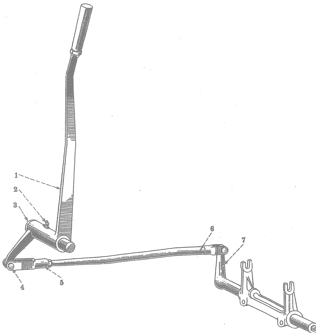
Clutch Lever and Connections (Hand Operated Over-Center Clutch)
