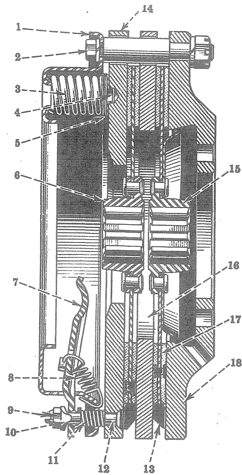
Steering Clutch, 10" (Double Plate)
