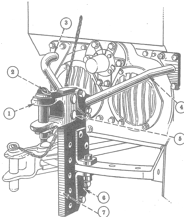
High Hitch Draw Bar—(Special)
