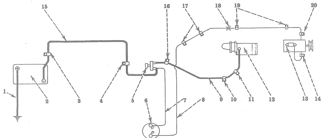
Wiring Diagram—Electric Starting—special
