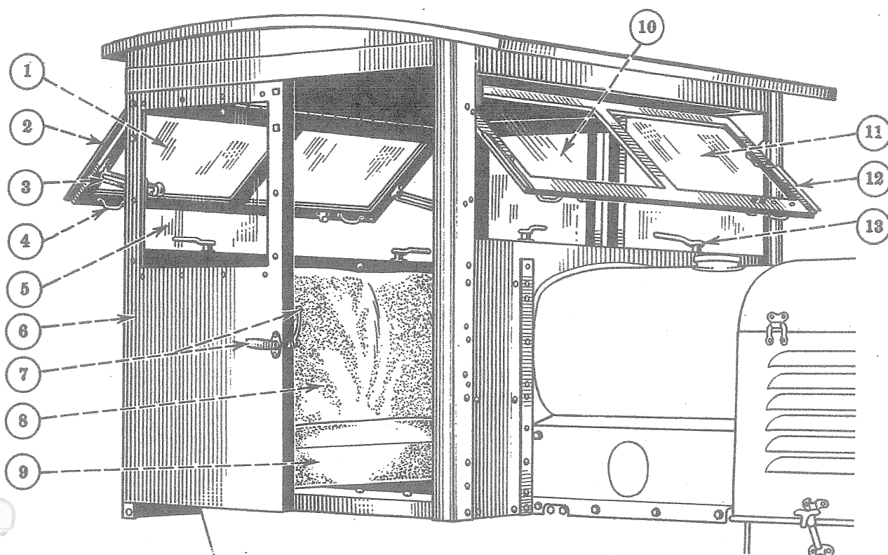
Cab— (Special)
