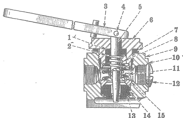
40728 DA Coupler, complete
