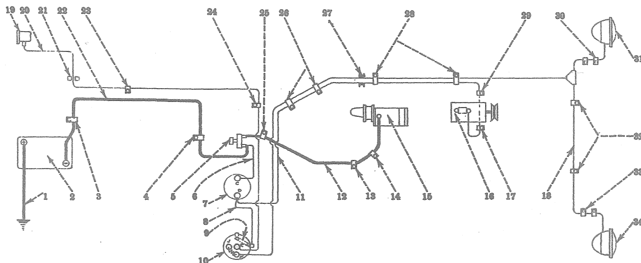
Wiring Diagram—Electric Lighting and Starting—special
