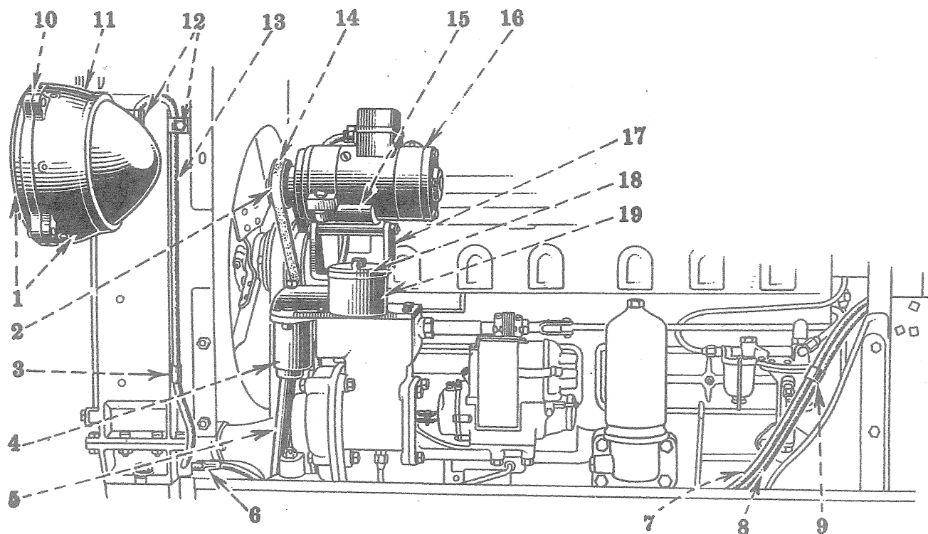
Front Lamp and Generator mounting
