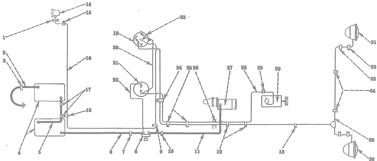
Wiring Diagram—Electric Lighting and Starting—special
