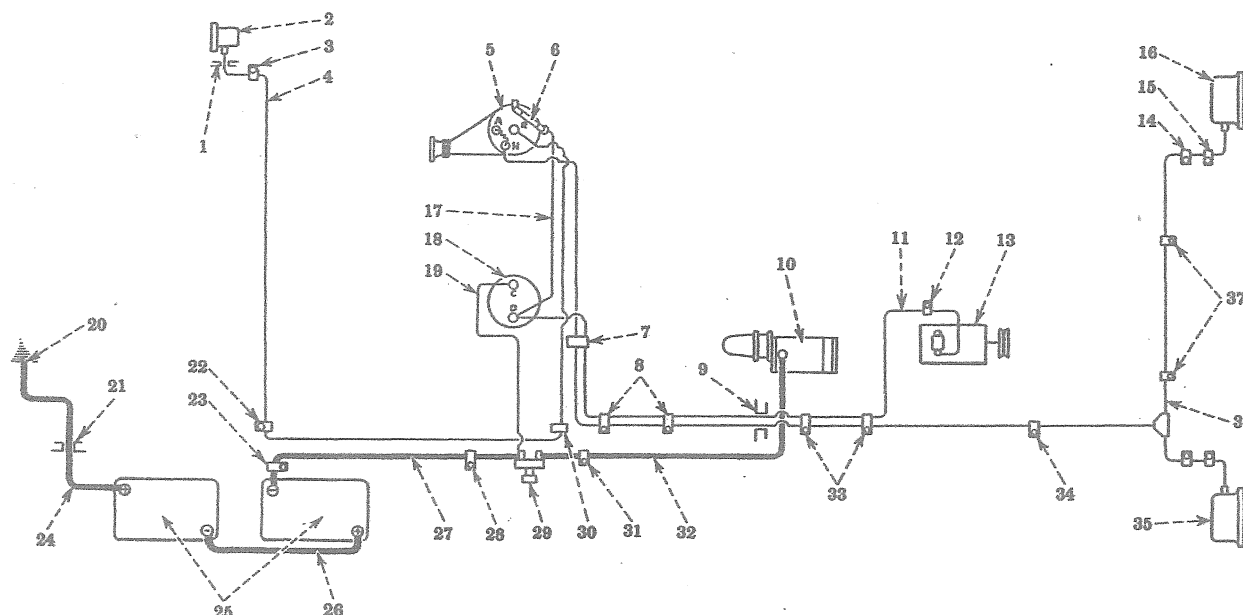
Wiring Diagram—Electric Lighting and Starting—special (Delco-Remy) (Side battery mounting) (Diesel)
