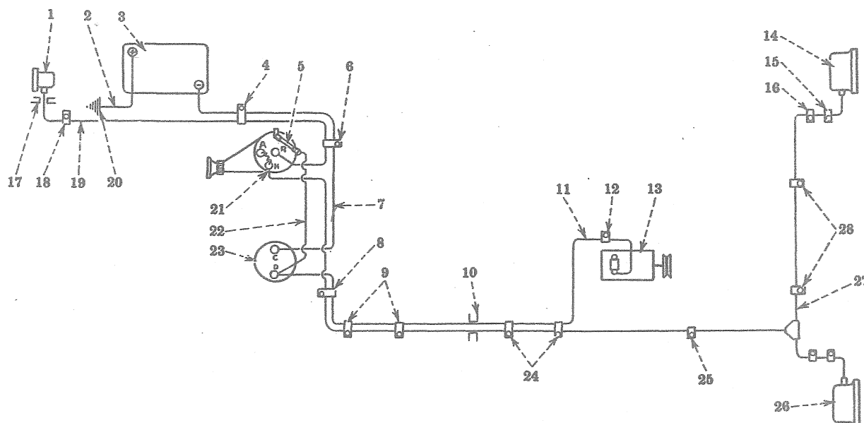
Wiring Diagram—Electric Lighting—Special (Delco-Remy)
