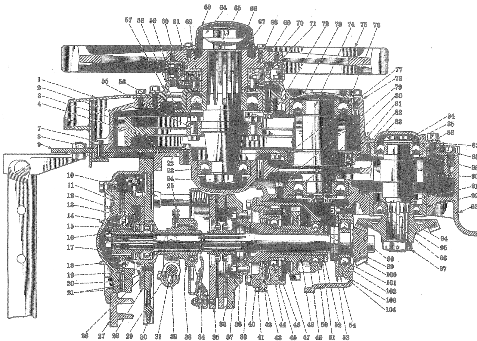
Track Drive—Left Side View. —Sprocket Drive, Pinion and Intermediate Drive, Steering Clutch Drive Shaft and Gear, Steering Clutch, Control and Disc Brake.
