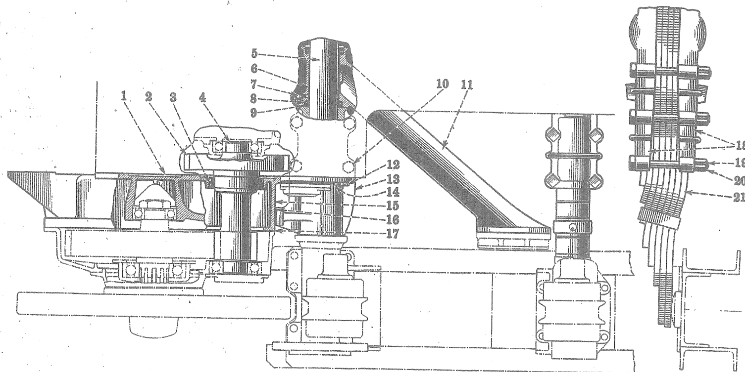
Track Frame, Equalizer Spring, Sprocket Drive, Pinion and Intermediate Drive.
