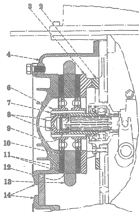
Double Disc Brake (Special)
