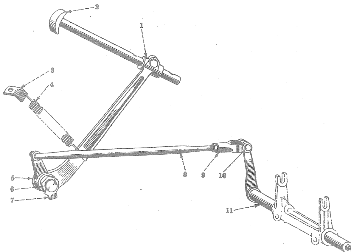
Clutch Pedal and Connections (Foot Operated—Special)
