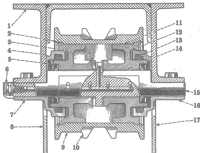
Track Roller
