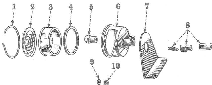
Tail Lamp (Electric Lighting—Special)
