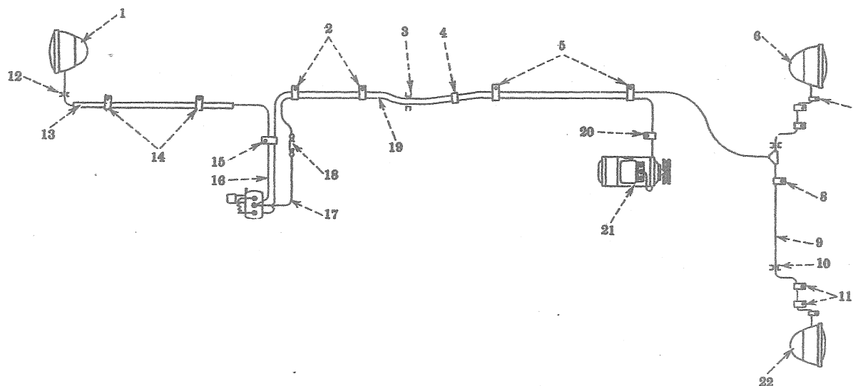
Wiring Diagram—Electric Lighting—Special
