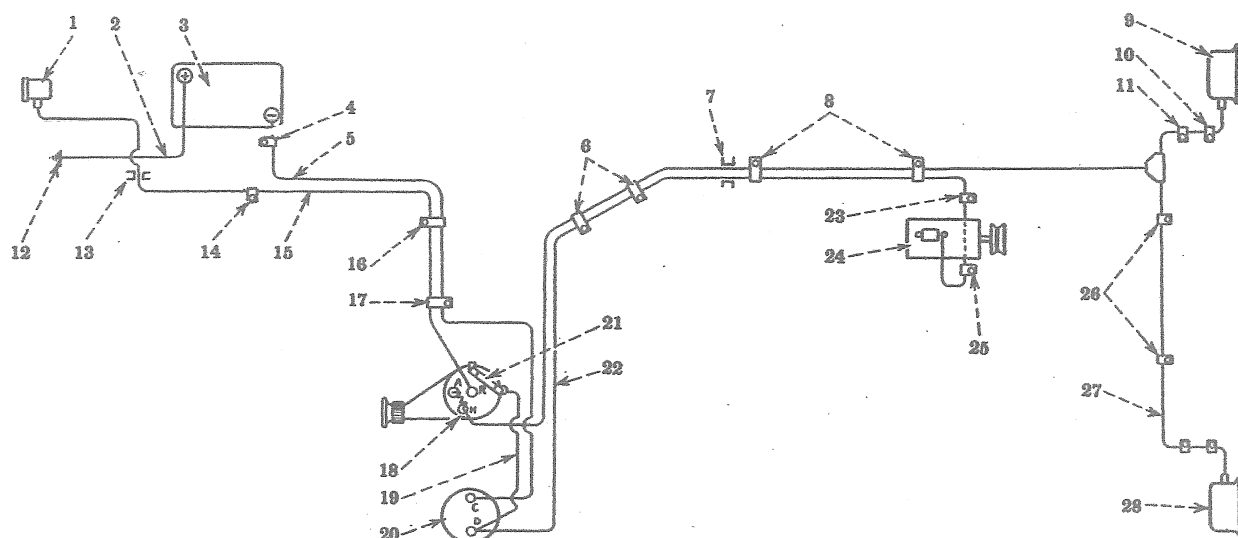
Wiring Diagram—Electric Lighting—Special
