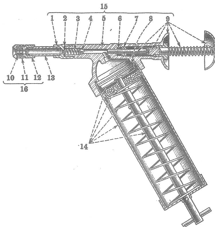
Lubricator Compressor—QA 3612
