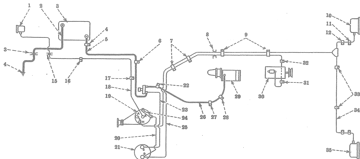
Wiring Diagram—Electric Lighting and Starting—special
