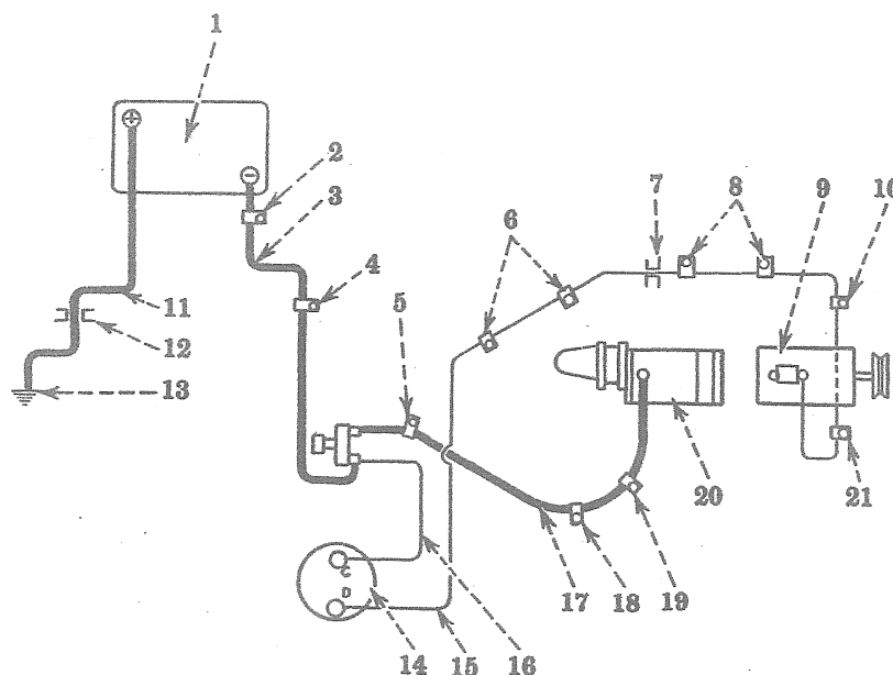
Wiring Diagram—Electric Starting—special
