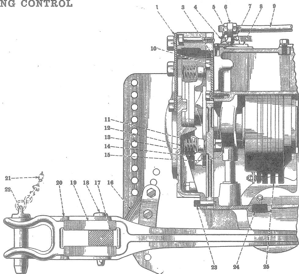
Steering Control, Steering Clutch and Brake, Drawbar and Power Take-off Opening Cover
