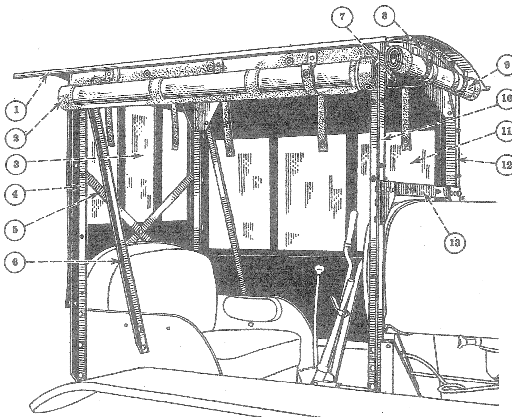
Canopy Top and Curtains (Special)
