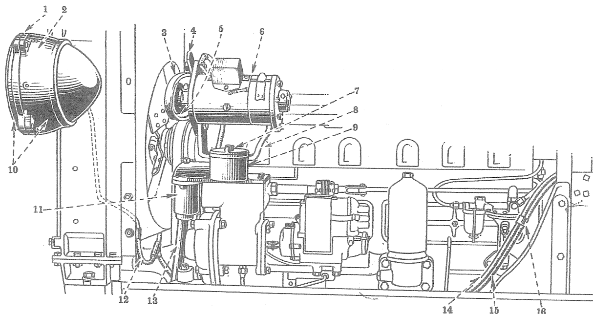
Front Lamp and Generator Mounting—Electric Lighting—Special (Delco-Remy) (not Diesel)
