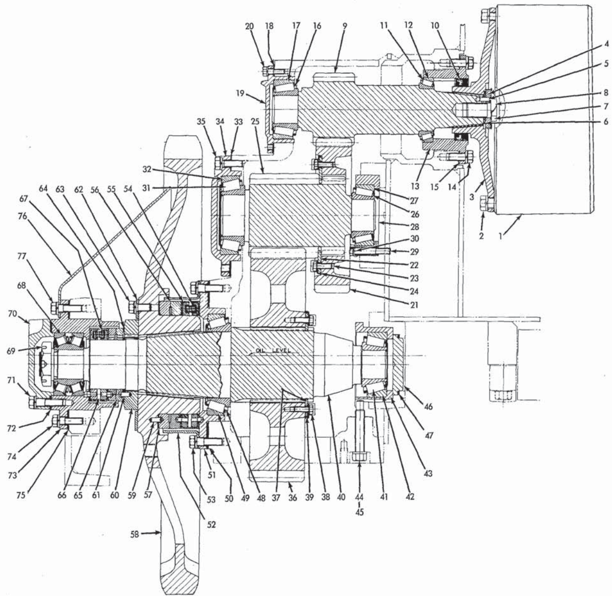
FINAL DRIVE
