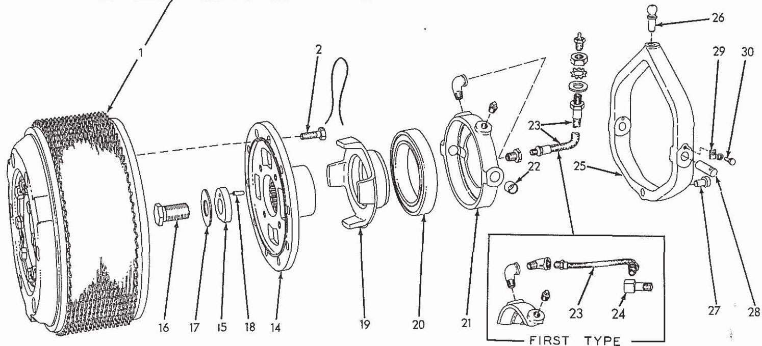
STEERING CLUTCHES (First type)
