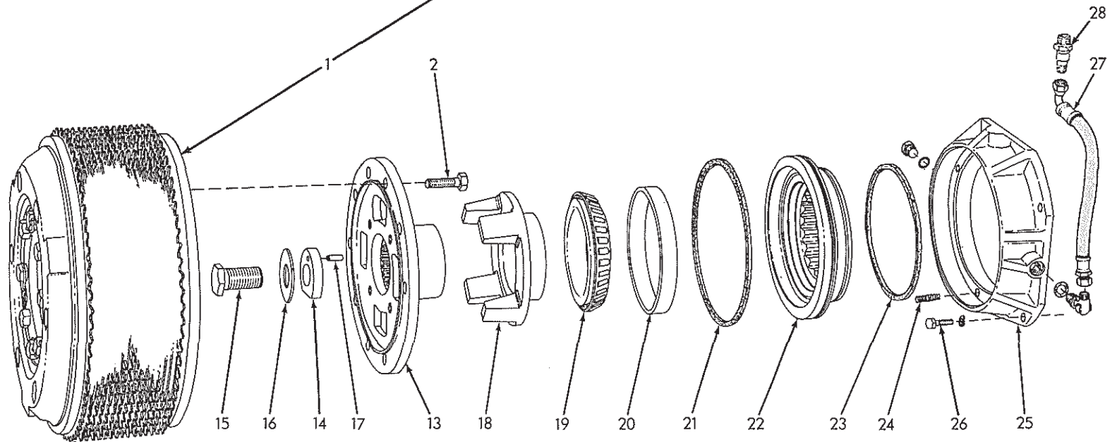
STEERING CLUTCHES (Second type Models HD11 E EC)
