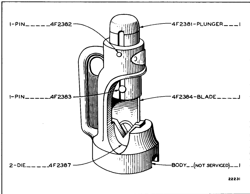
CABLE CUTTER
