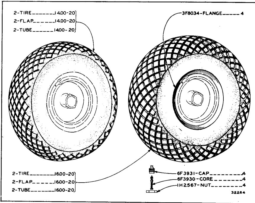
TIRES AND FLANGES—With Tubes Serial No. 2W5001 to 2W5259 inclusive
