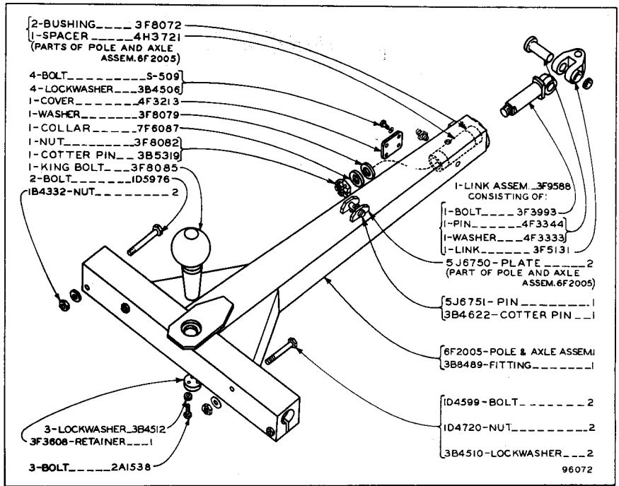
POLE AND AXLE Effective with Serial No. 2W6432
