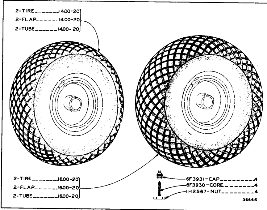
TIRES—With Tubes Serial No. 2W5260 to 2W5748 inclusive
