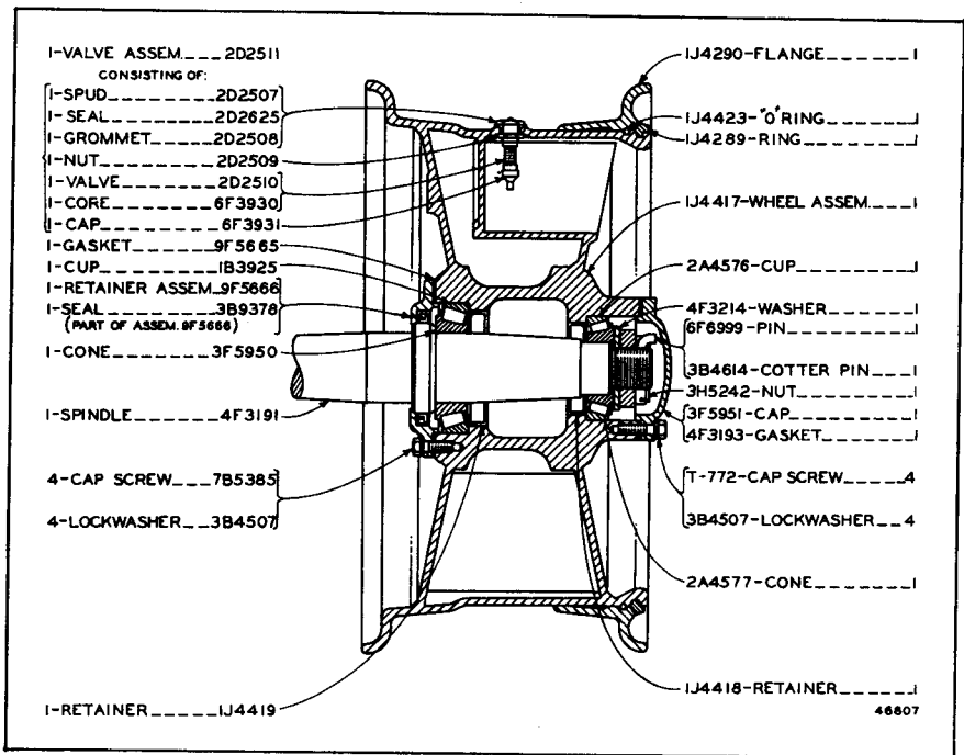
FRONT WHEEL AND AXLE (2 Groups Req'd.) Effective with Serial No. 2W5749
