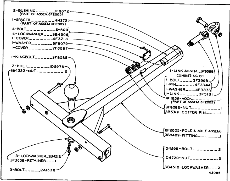
POLE AND AXLE Effective with Serial No. 2W5749
