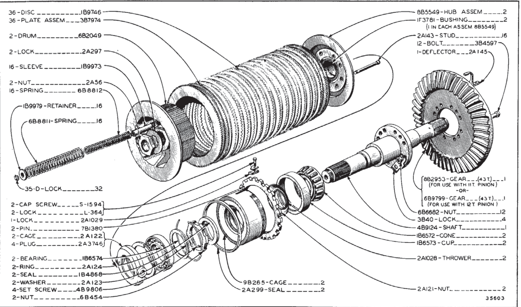
STEERING CLUTCH Effective with Serial No. 8R5103 Refer to Page 114 for special parts
