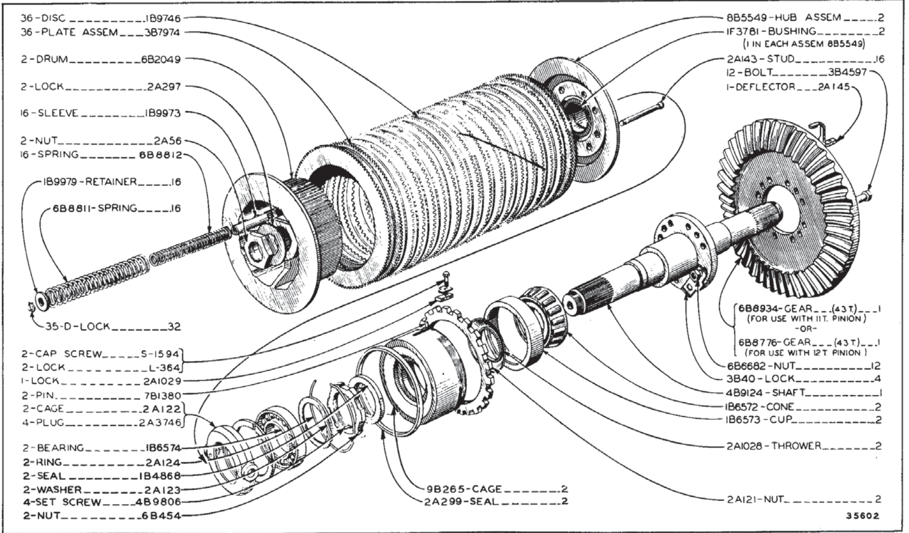
STEERING CLUTCH Serial No. 8R1 to 8R5102 Inclusive Refer to Page 114 for special parts
