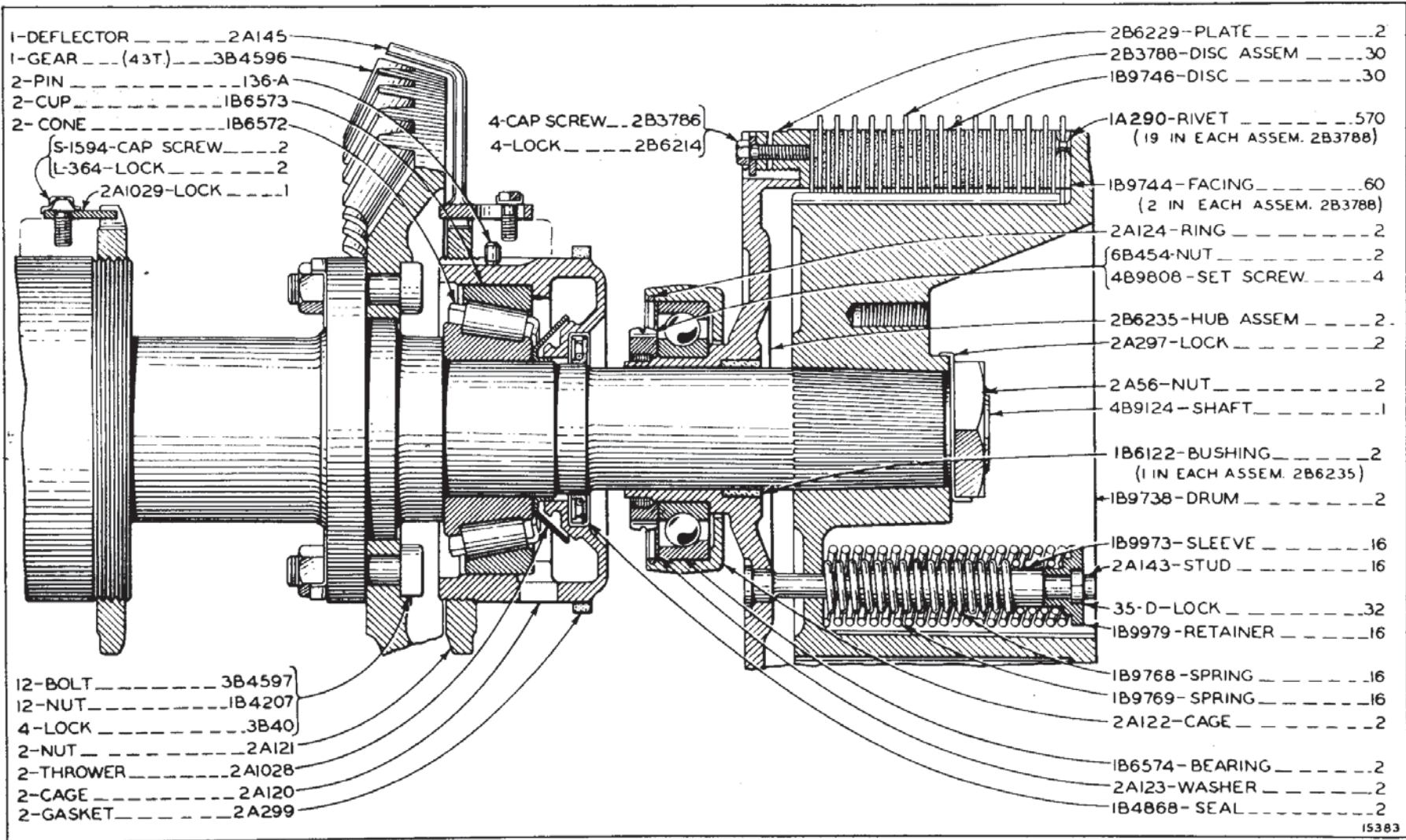
STEERING CLUTCH (Machines 1H2409 to 1H4685 Inclusive)
