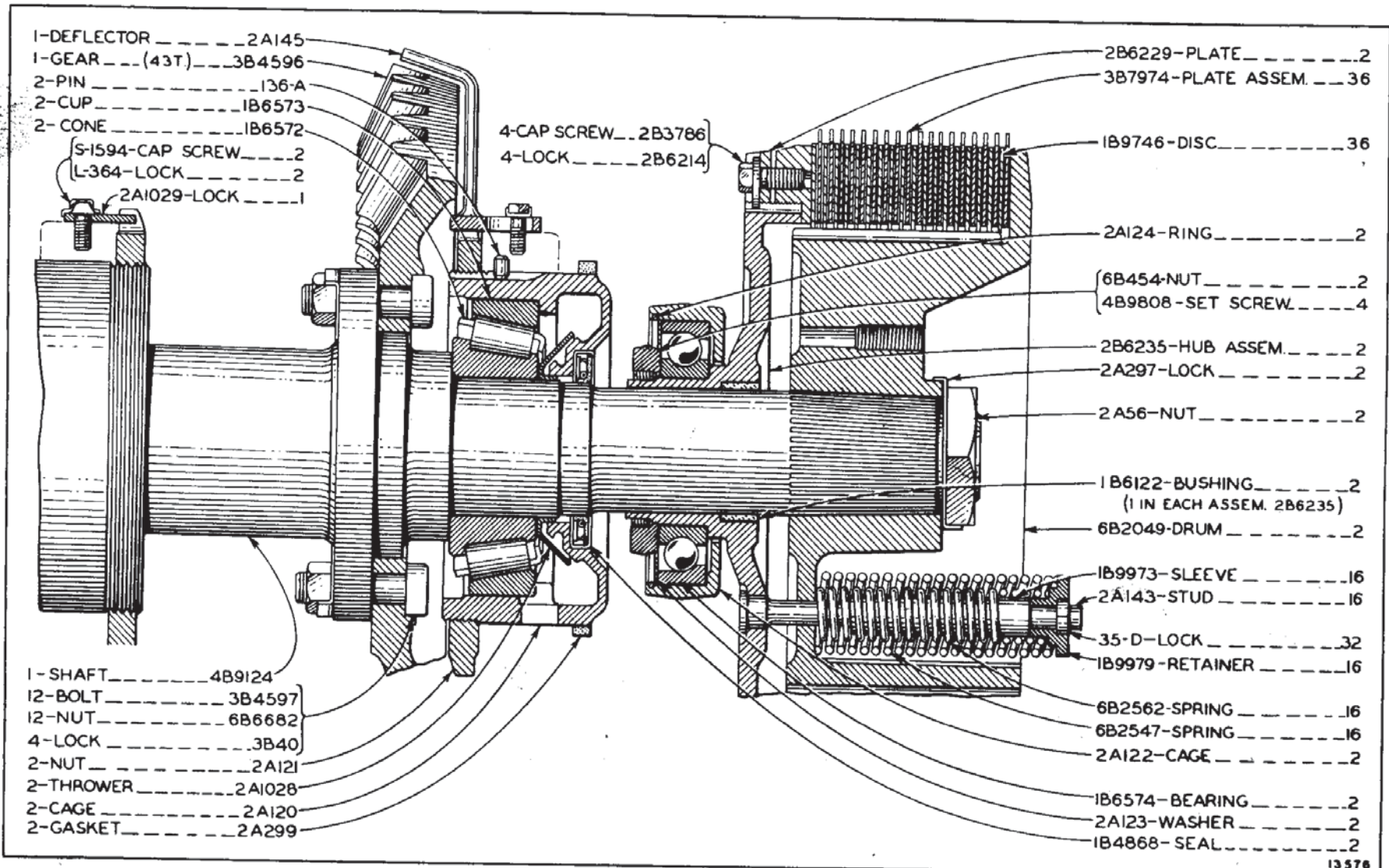
STEERING CLUTCH (Effective with Machine 1H4686)
