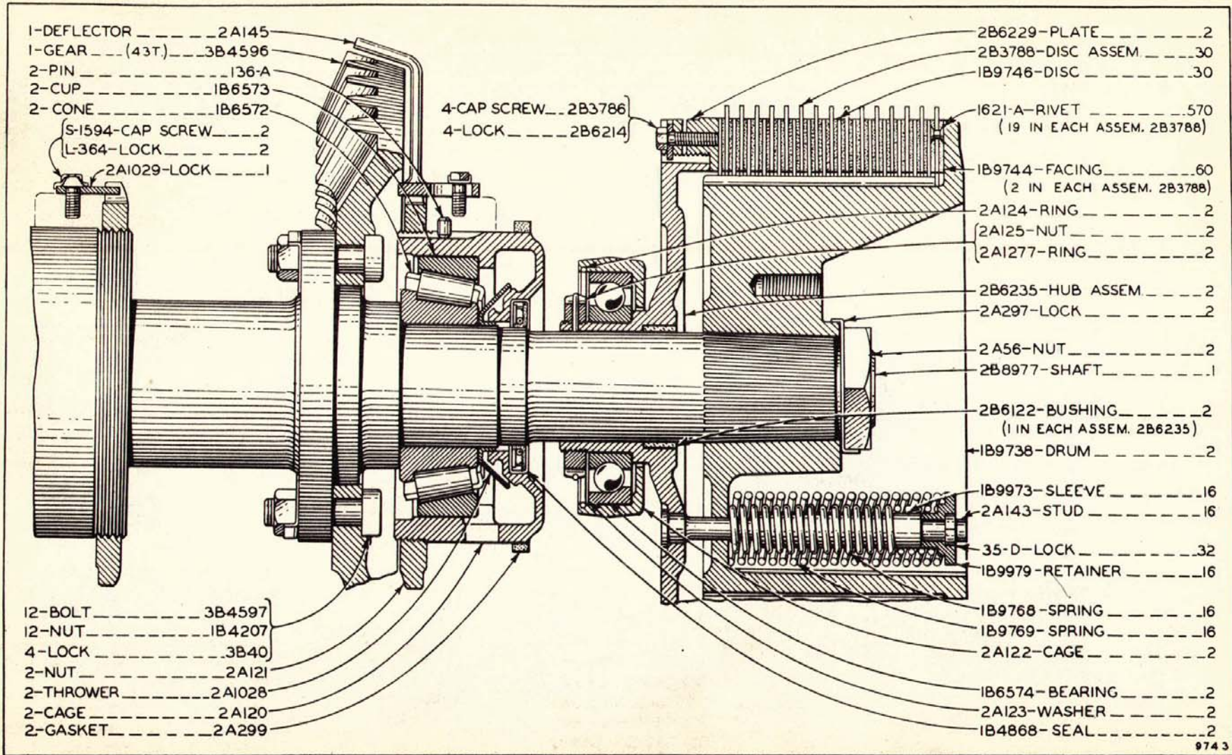
STEERING CLUTCH (Effective with Machine 1H904)
