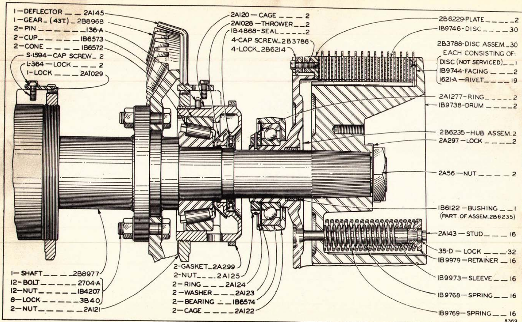
STEERING CLUTCH (Machines 1H1 to 1H903 Inclusive)
