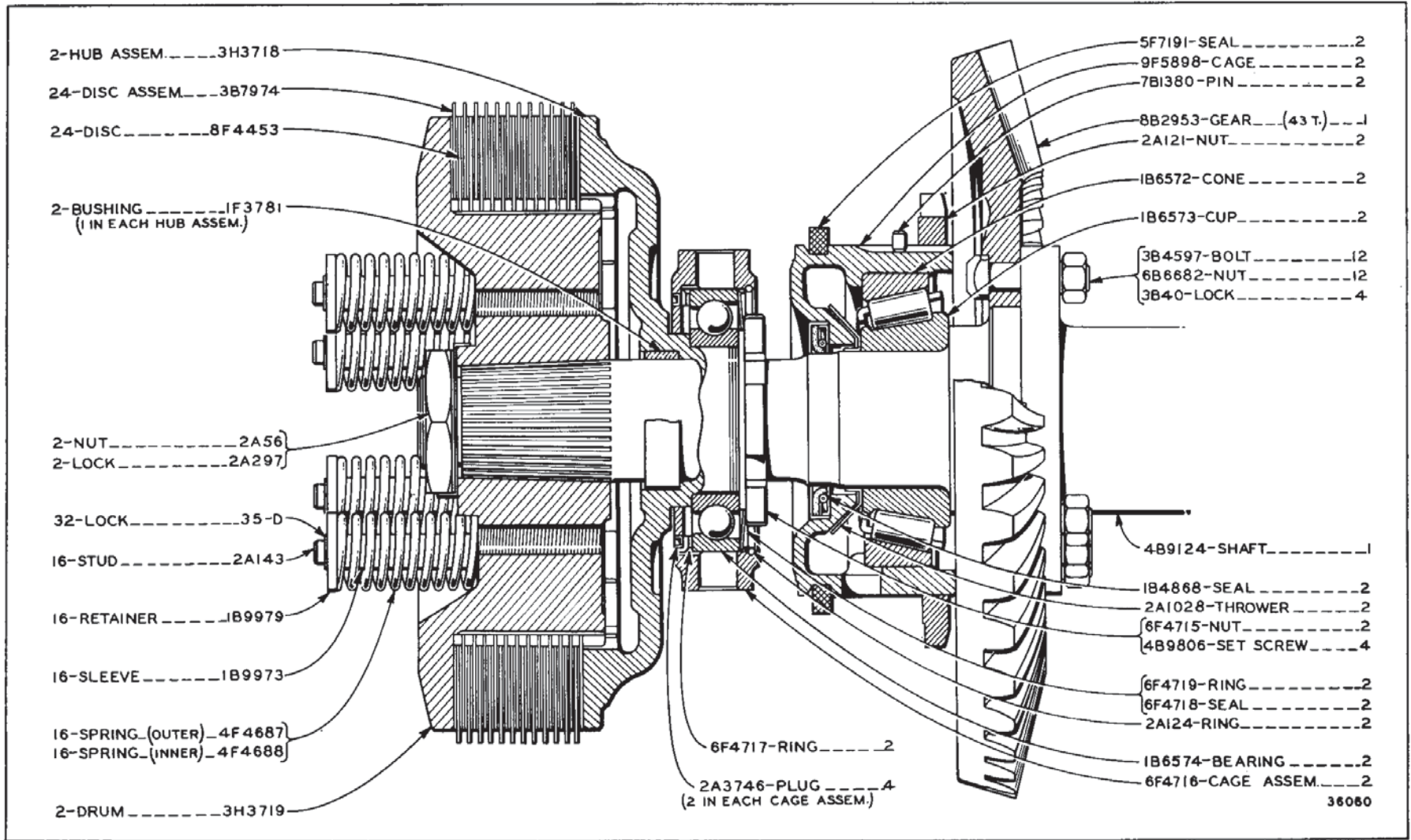
STEERING CLUTCH Serial No. 13A1 to 13A2227 inclusive
