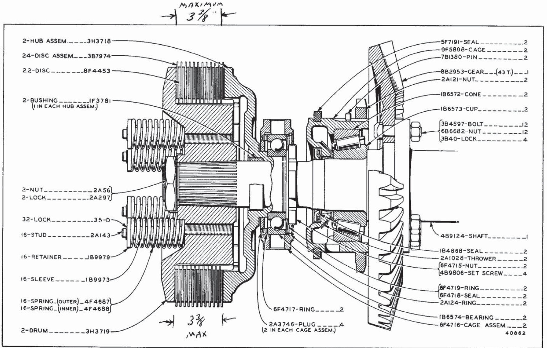
STEERING CLUTCH Effective with Serial No. 13A2228
