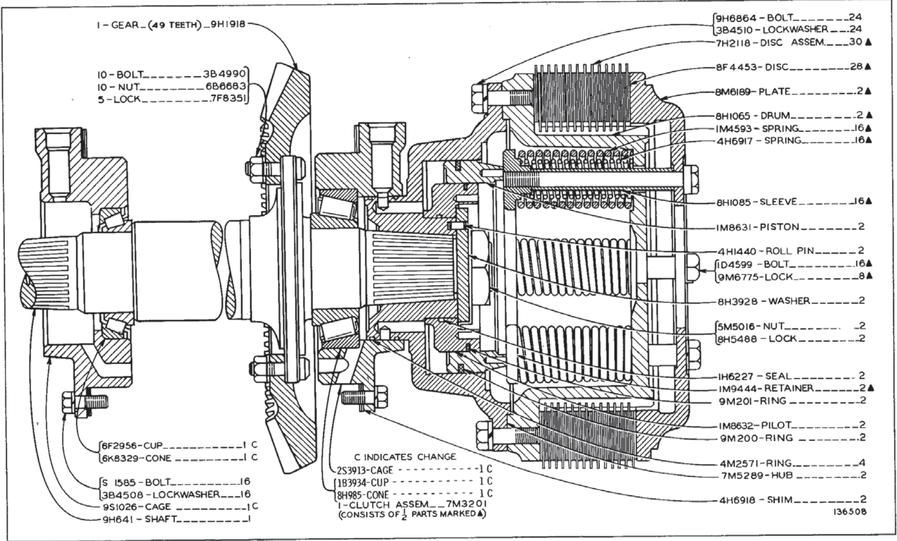
STEERING CLUTCH (9H4147 N/S) Serial No. 46A24433 to 46A26923 inclusive
