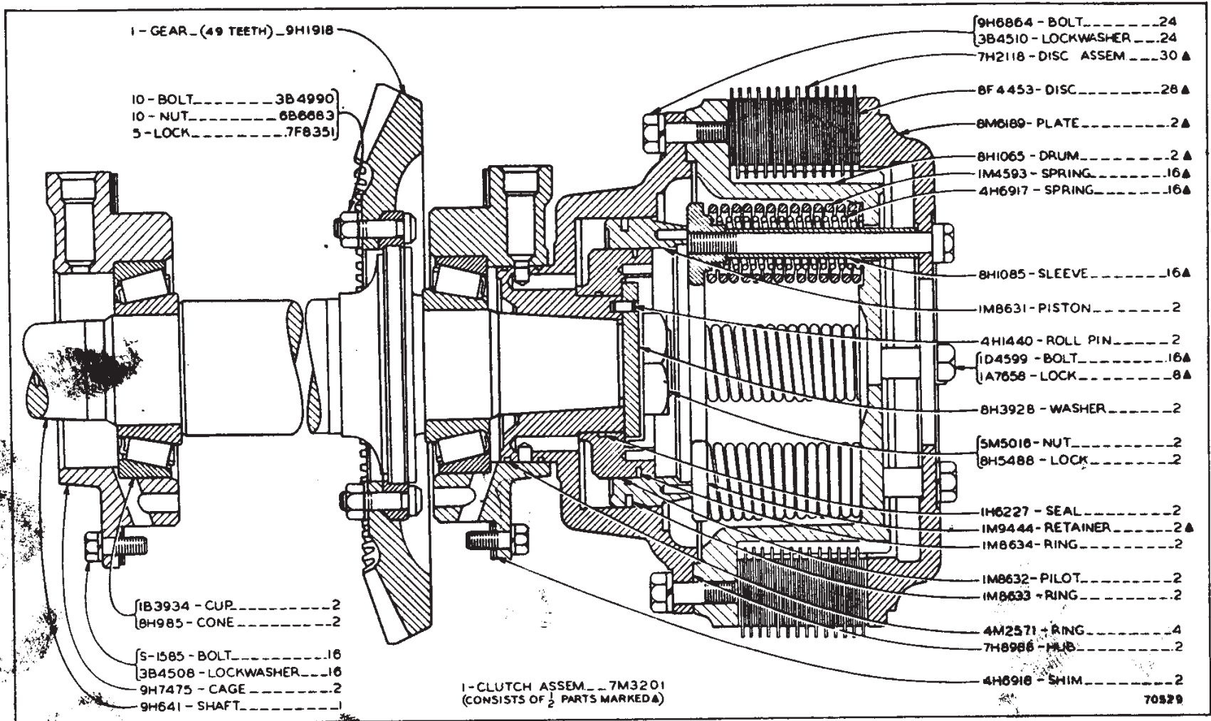
STEERING CLUTCH
