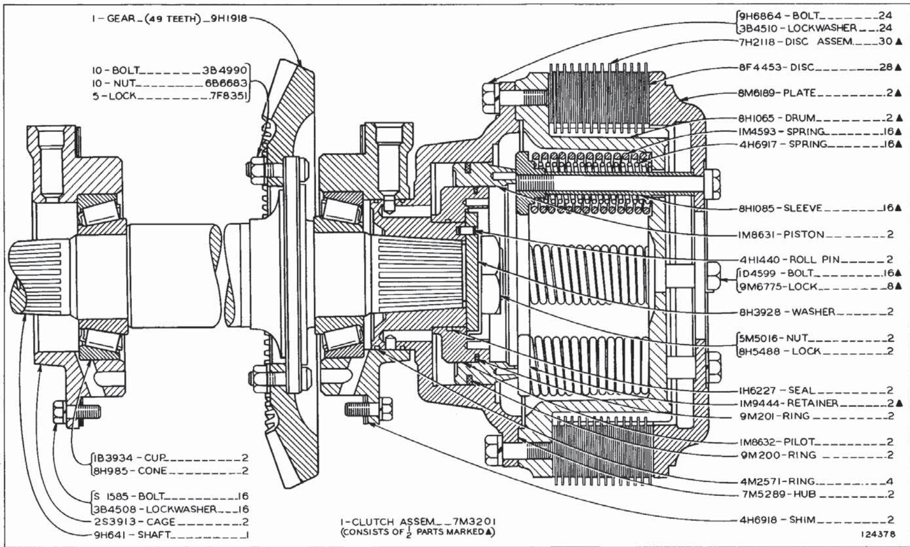
STEERING CLUTCH Serial No. 46A10725 to 46A21038 inclusive
