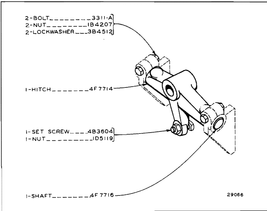
8F8905 SHEAVE HITCH GROUP No. 75 Bulldozer Serial No. 17C1 to 17C5000 and 84C1—Up
