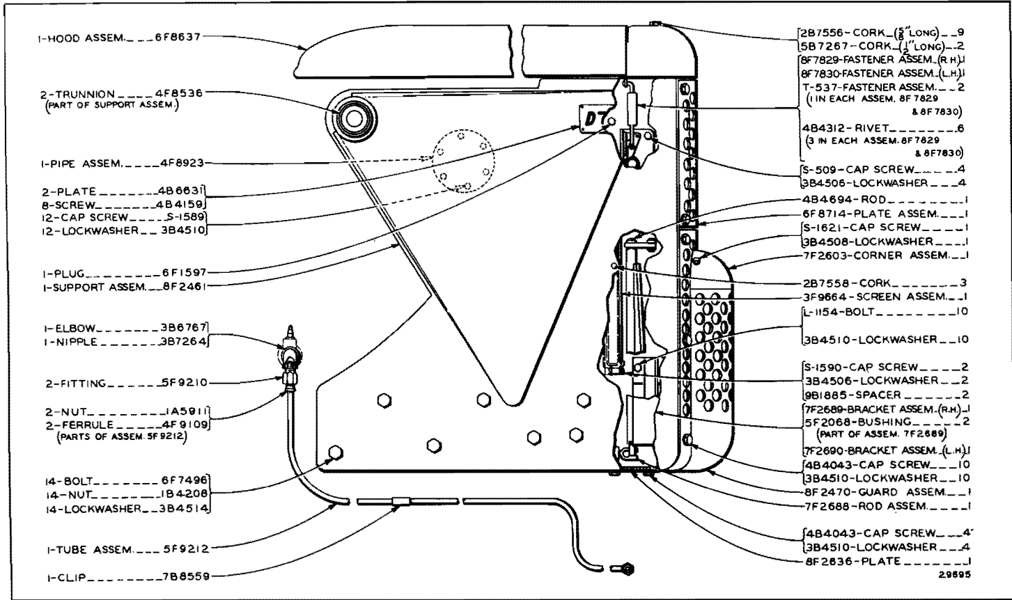
8F2462 CYLINDER SUPPORT AND RADIATOR GUARD GROUP For use on D7 Tractors having Serial No. 7M1 to 7M9999 and 3T1 to 3T11972 inclusive
