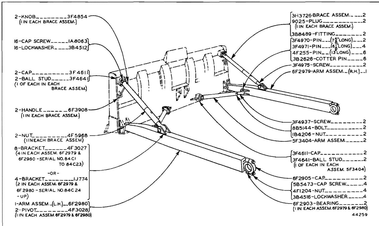
5F5338 PUSH ARM AND BRACE GROUP No. 75 Bulldozer Serial No. 17C1 to 17C5000 and 84C1—Up
