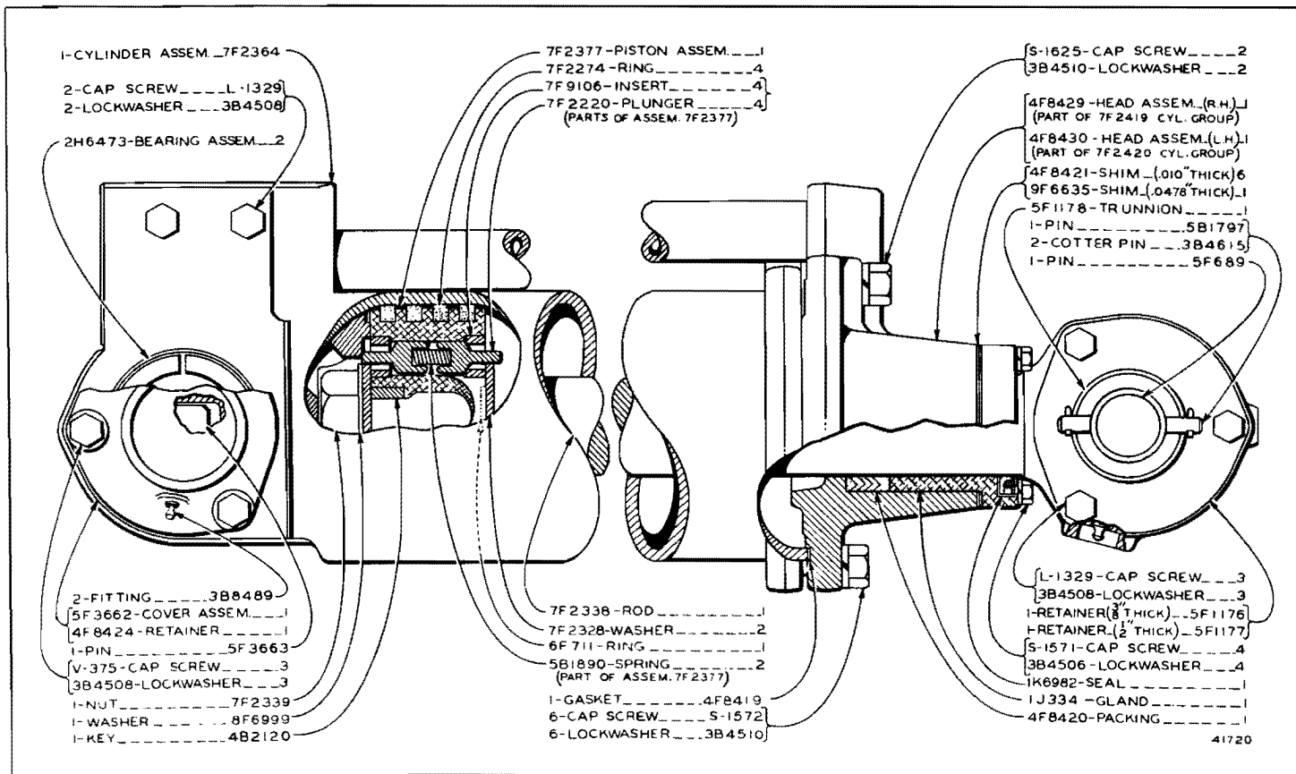
7F2419 HYDRAULIC CYLINDER GROUP—R. H. 7F2420 HYDRAULIC CYLINDER GROUP—L. H.
