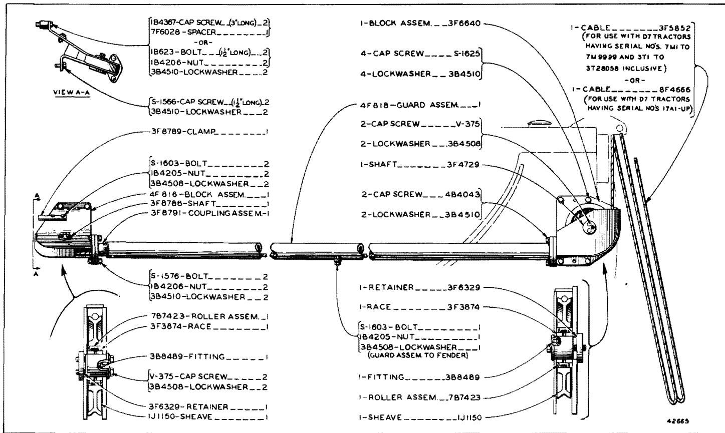
4F819 CABLE AND GUARD GROUP For use with No. 25 Cable Control
