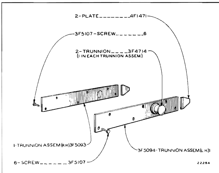
4F6218 TRUNNION GROUP
