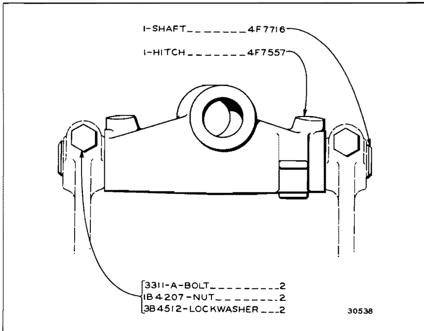
8F8906 SHEAVE HITCH GROUP Effective with No. 7A Bulldozer Serial No. 17C5001—Up
