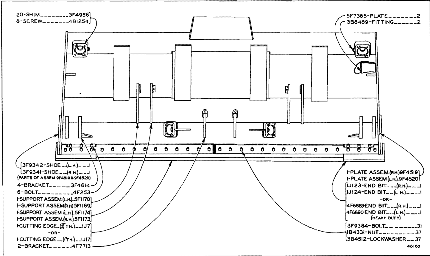
8F8909 BLADE GROUP No. 7S Bulldozer Serial No. 17C1 to 17C5000 and 84C1—Up
