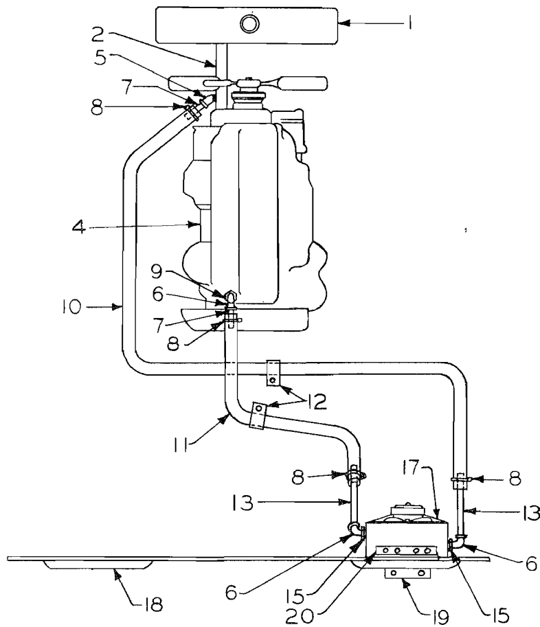
Figure 48. Heater Piping Diagram for UD-14A Engine
