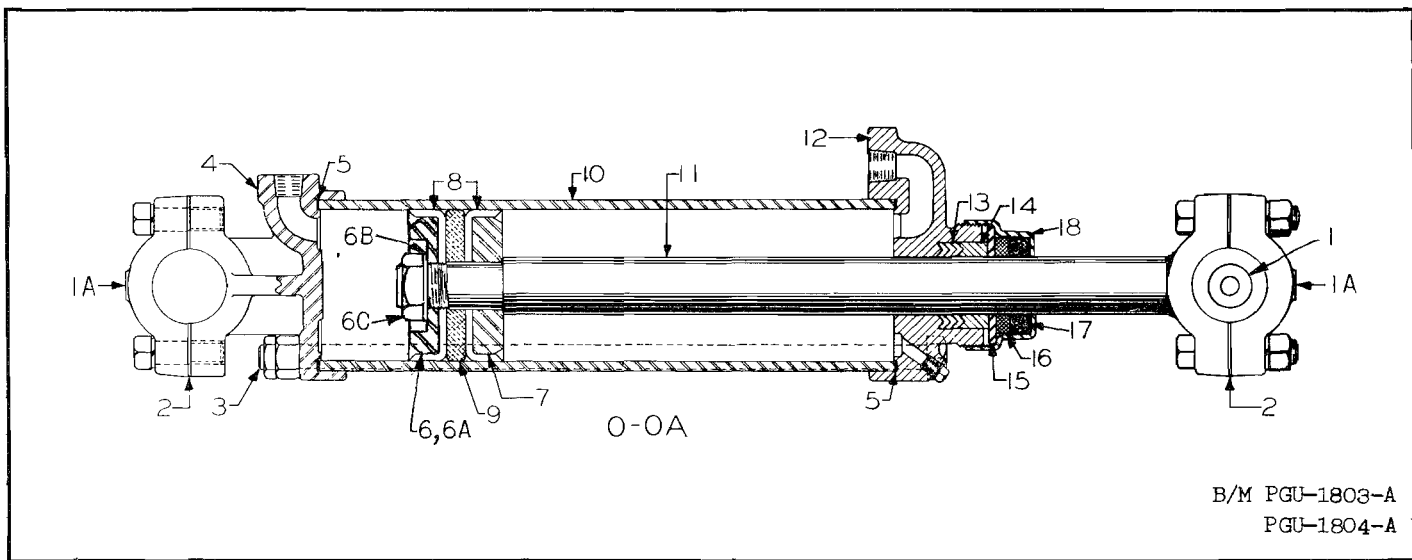
Figure 78. Rear Roller Ram
