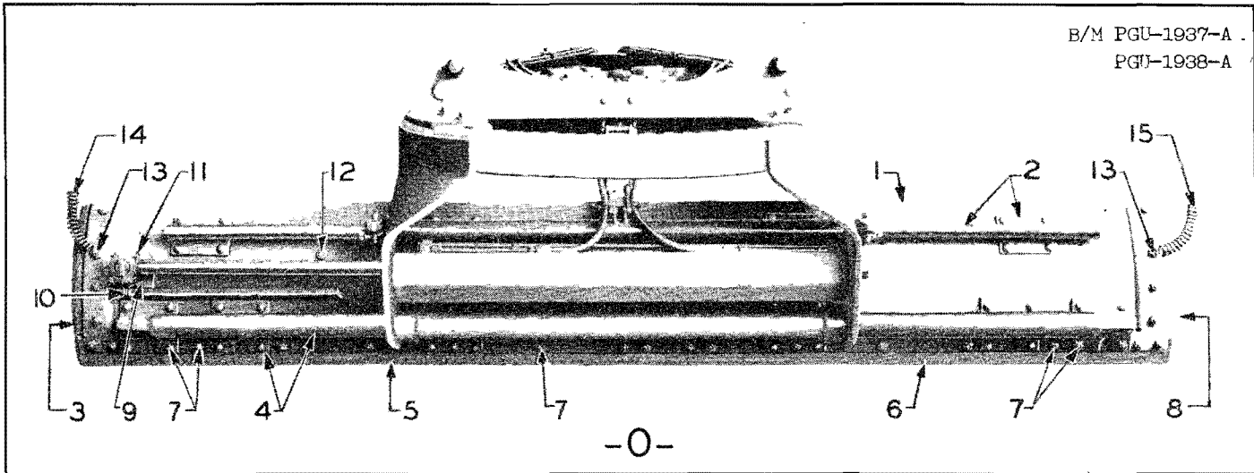
Figure 13A. Blade
