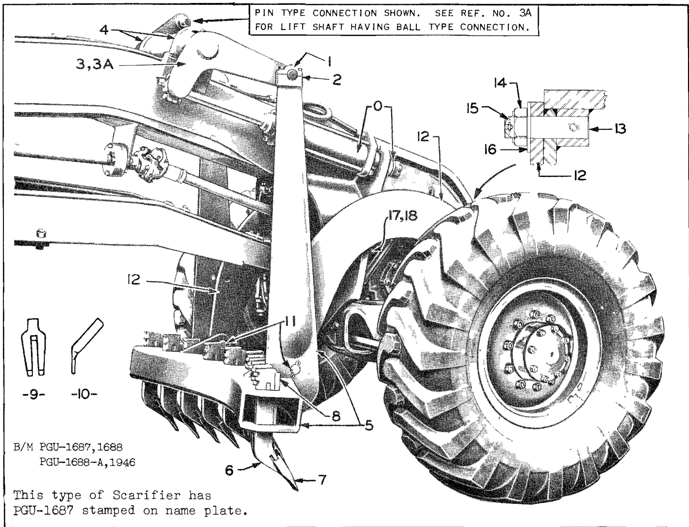
Figure 52. Scarifier
