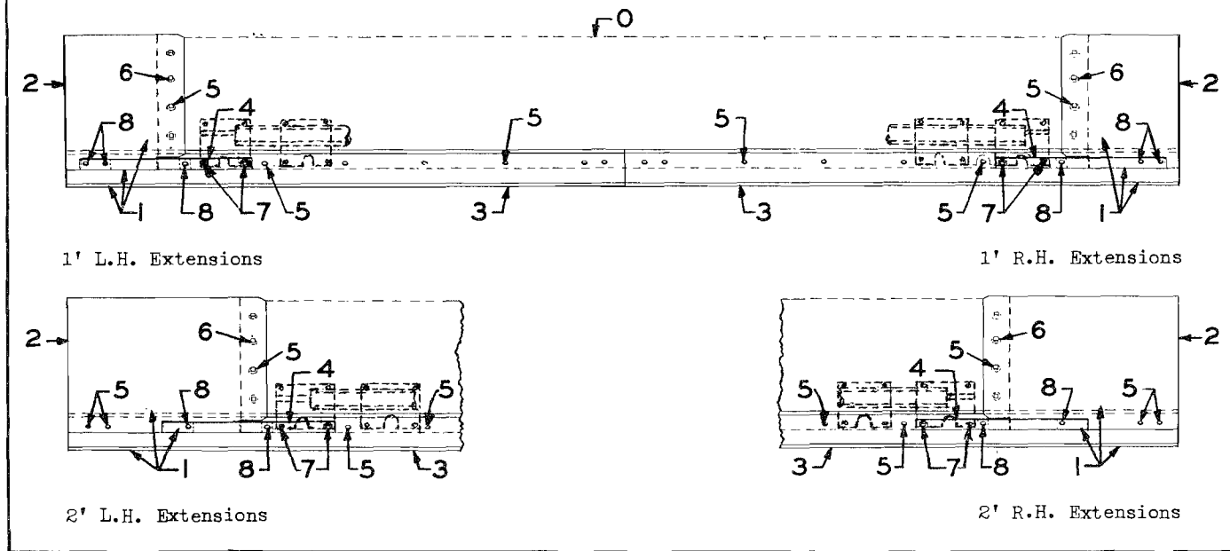
Figure 14A. Blade Extensions and Cutting Edges
