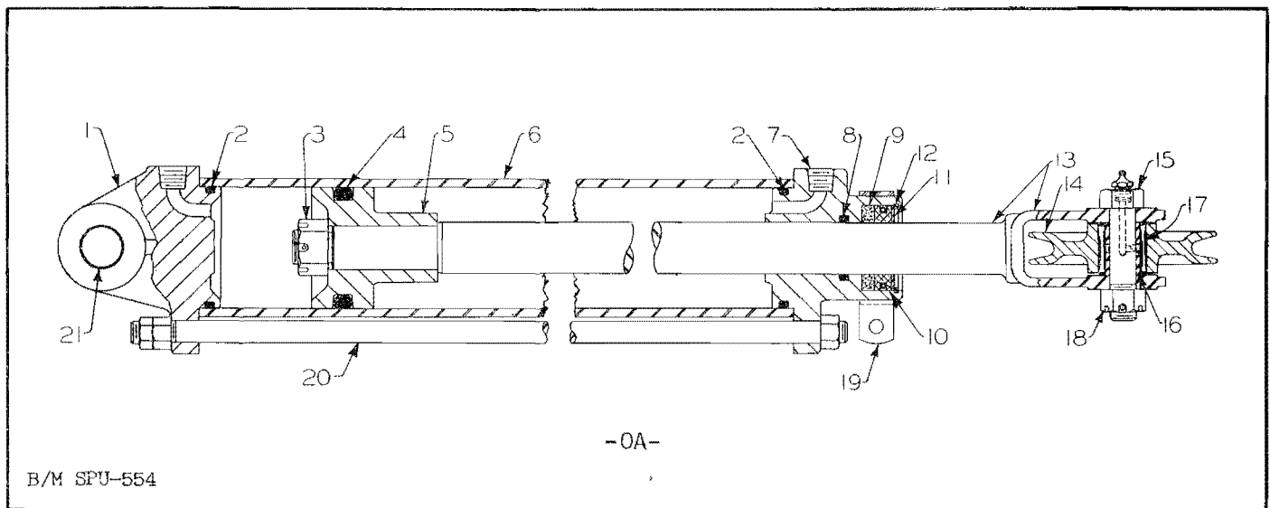
Figure 88. Snow Wing Front Lift Ram
