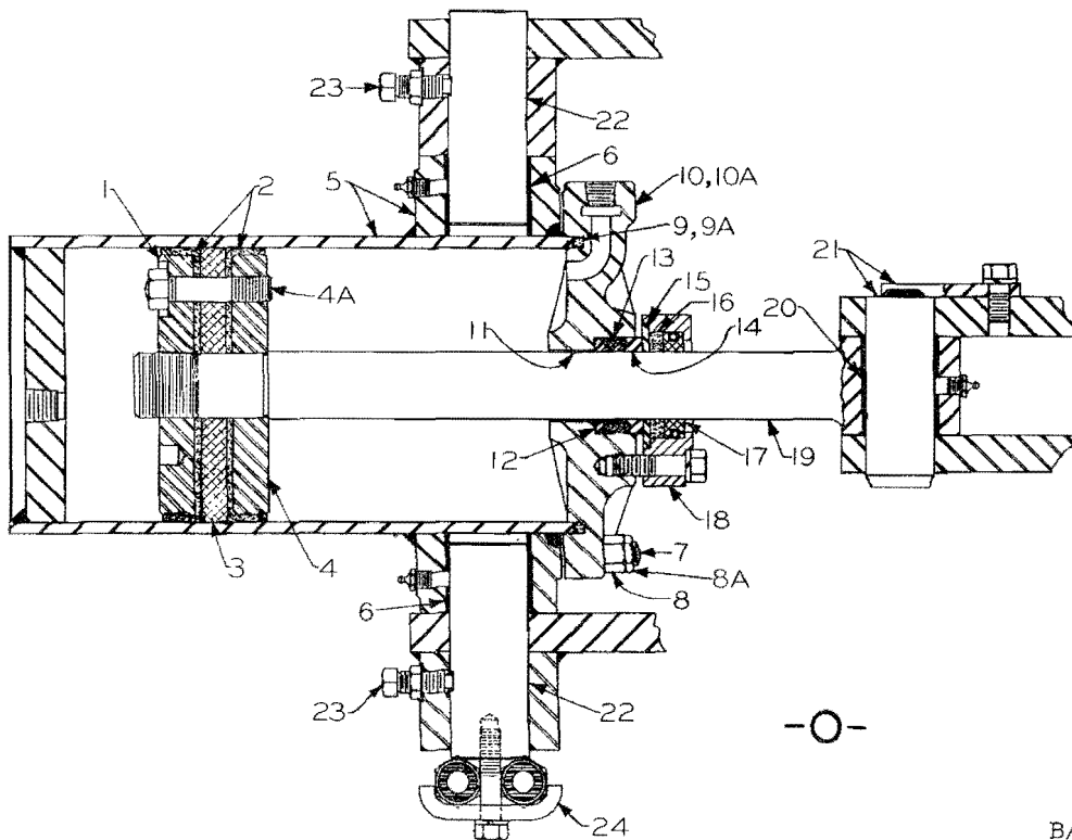
Figure 7A. High Lift Ram (Machines H-322 and up)
