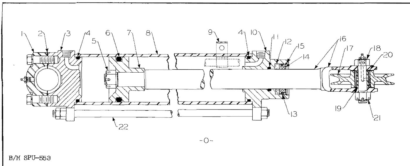
Figure 87. Snow Wing Rear Lift Ram
