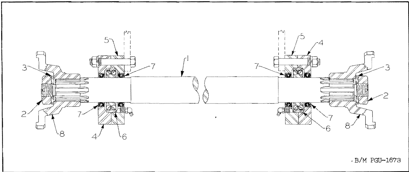
Figure 16. Center Section of Front Propeller Shaft
