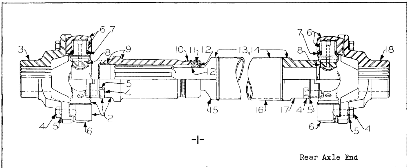
Figure 37. Rear Propeller Shaft
