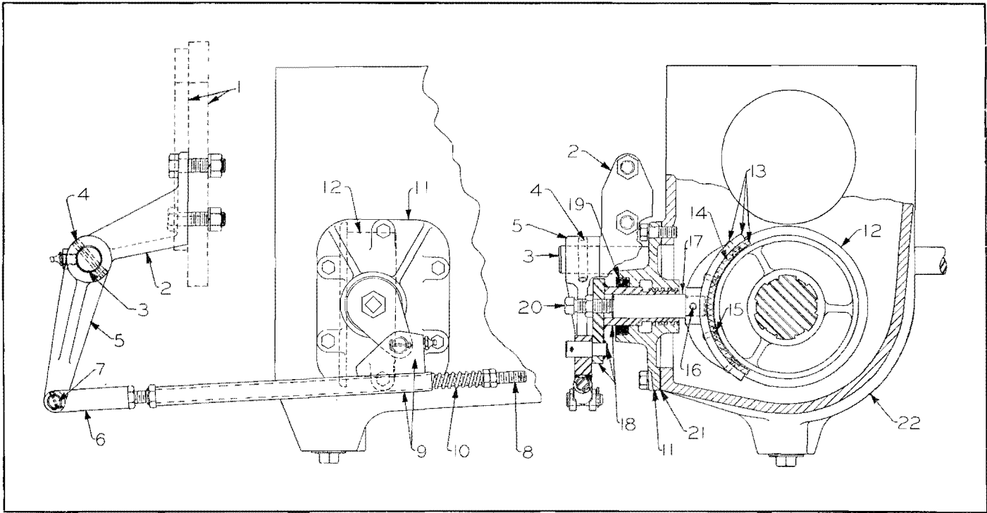
Figure 22. Clutch Brake
