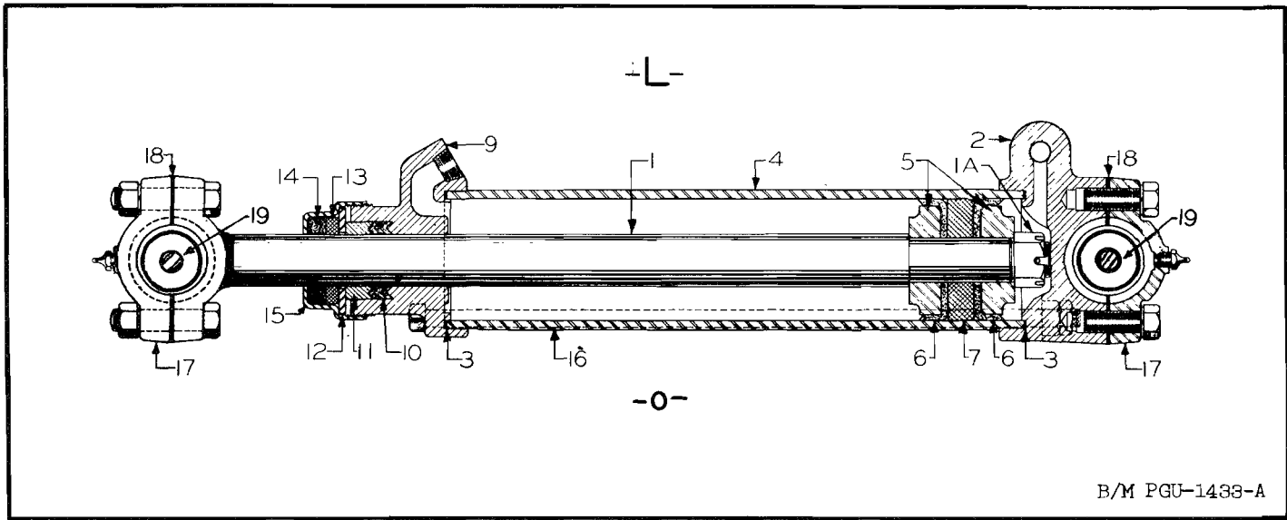
Figure 73. Conveyor Loader Lift Ram
