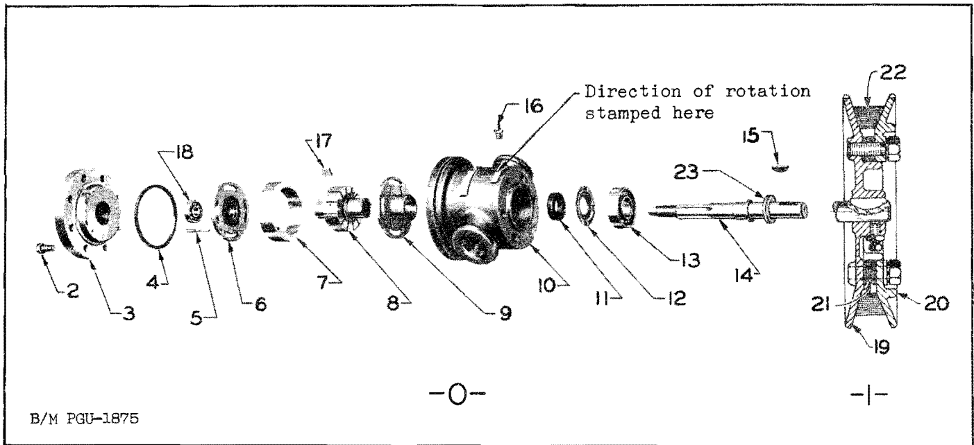
Figure 39. Hydraulic Pump and Pulley for UD-14A Engine
