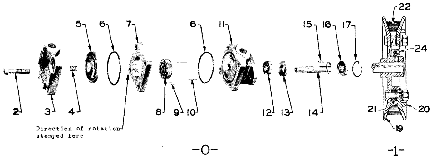
Figure 38B. Hydraulic Pump and Pulley for UD-14A Engine (Machines H-2540 and up)
