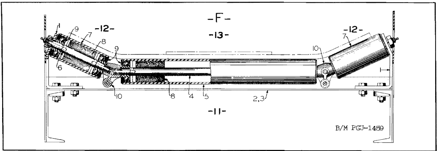
Figure 67. Conveyor Loader Intermediate Carrying Roller
