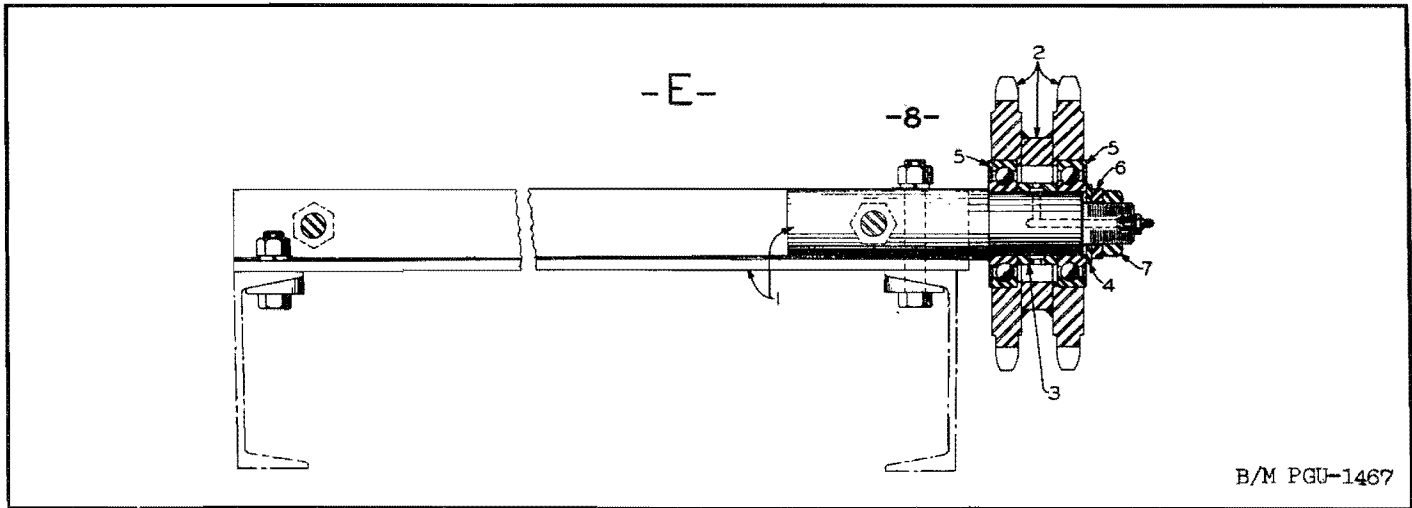
Figure 72. Conveyor Loader Countershaft
