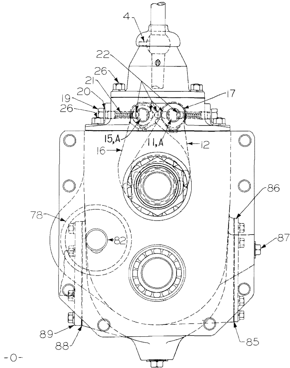
Figure 19B. Transmission
