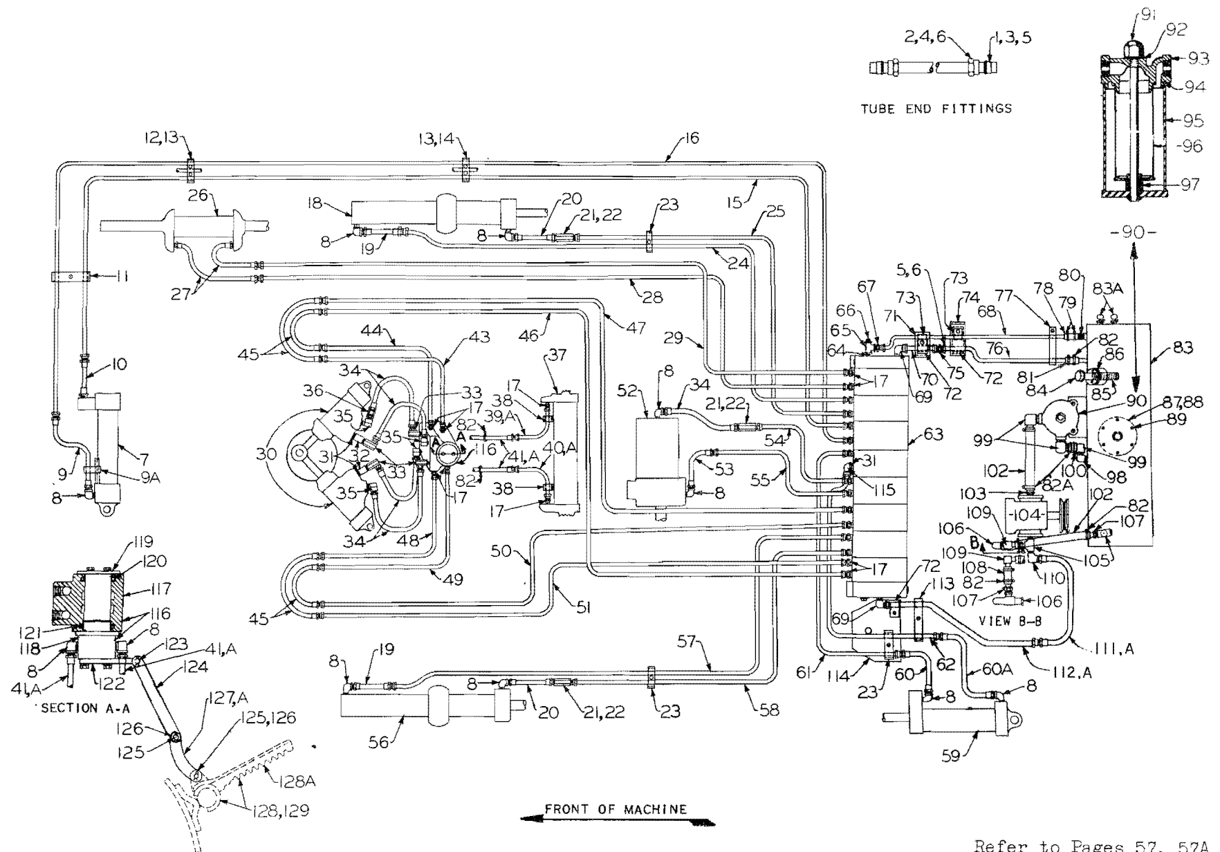
Figure 38. Hydraulic Piping Diagram for UD-14A Engine
