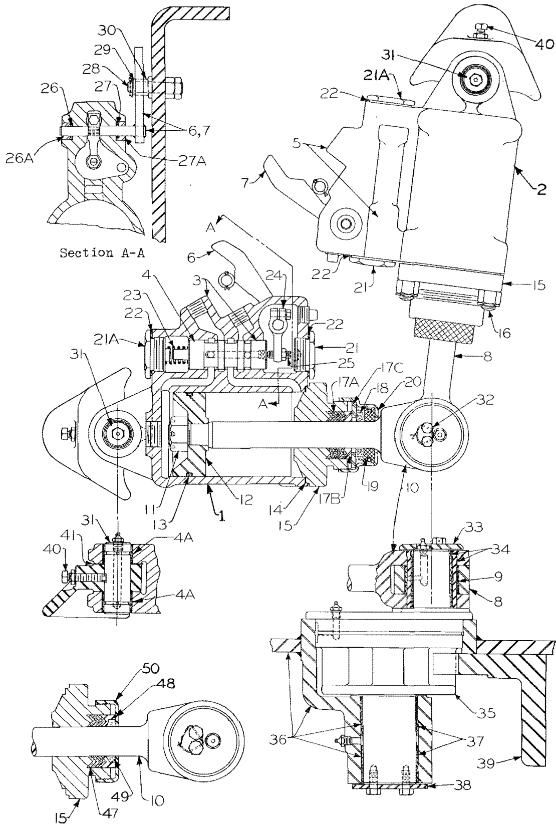
Figure 10. Circle Reverse Hydraulic Motor
