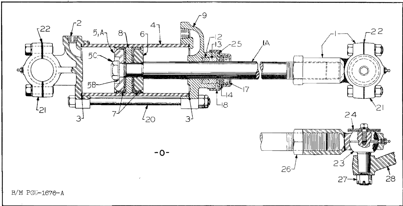
Figure 36. Rear Axle Steering Ram
