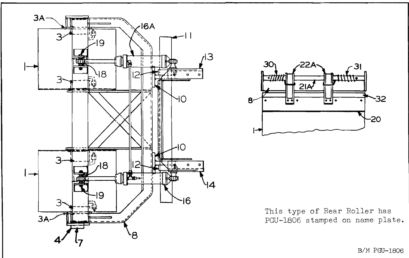
Figure 77. Rear Roller
