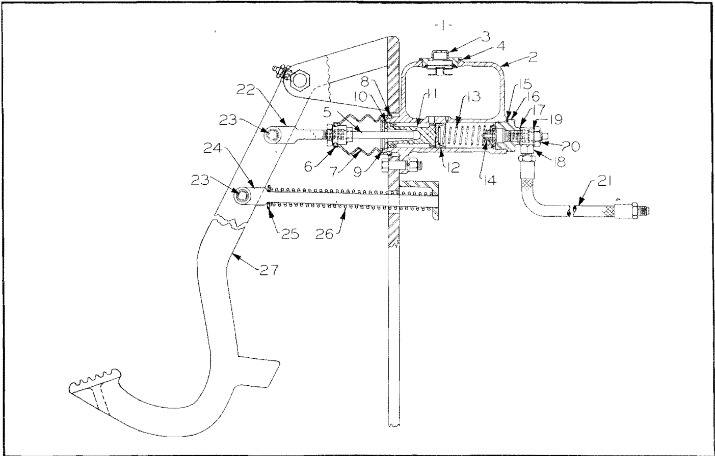
Figure 25. Foot Brake Mechanism
