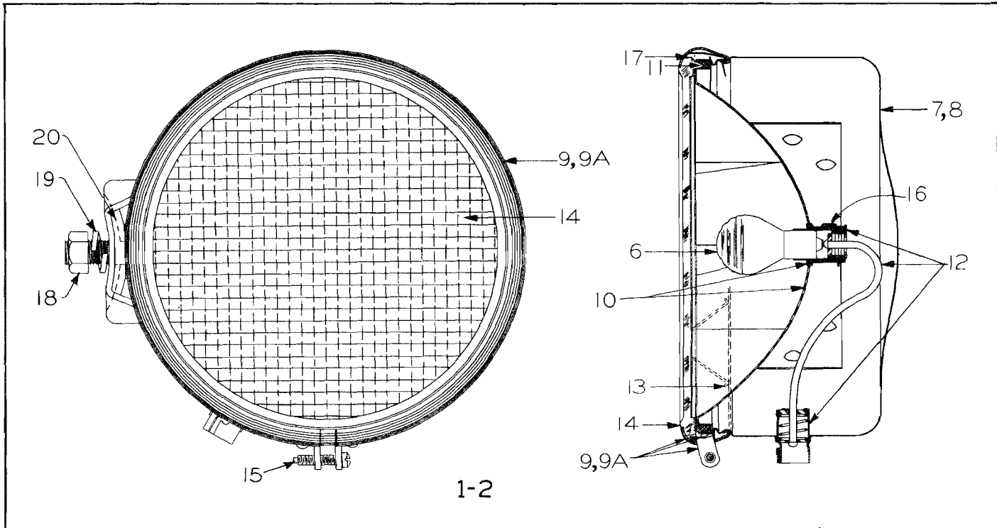
Figure 51. Headlights
