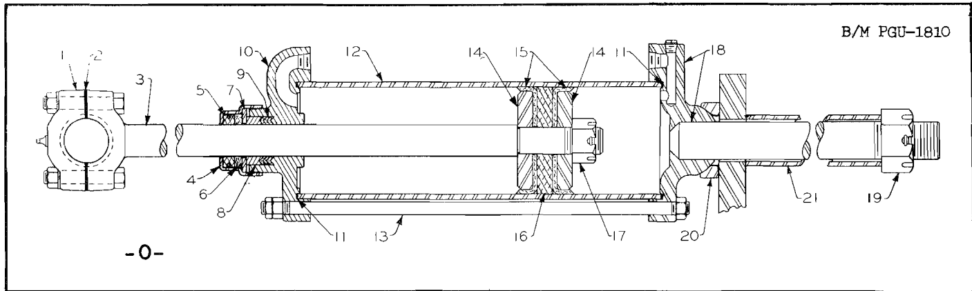
Figure 54. Scarifier Ram (1st type) (Also used with Bulldozer and front Snow Plows)
