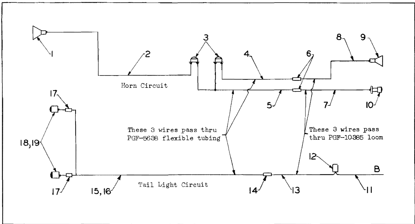
Figure 58. Conveyor Loader Tail Light and Horn Circuit
