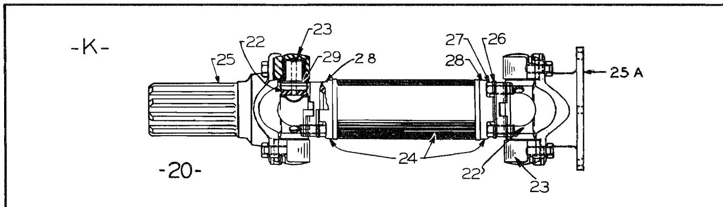
Figure 63. Conveyor Loader Propeller Shaft (Power Take-off to Engine Pulley) for UD-14A Engine
