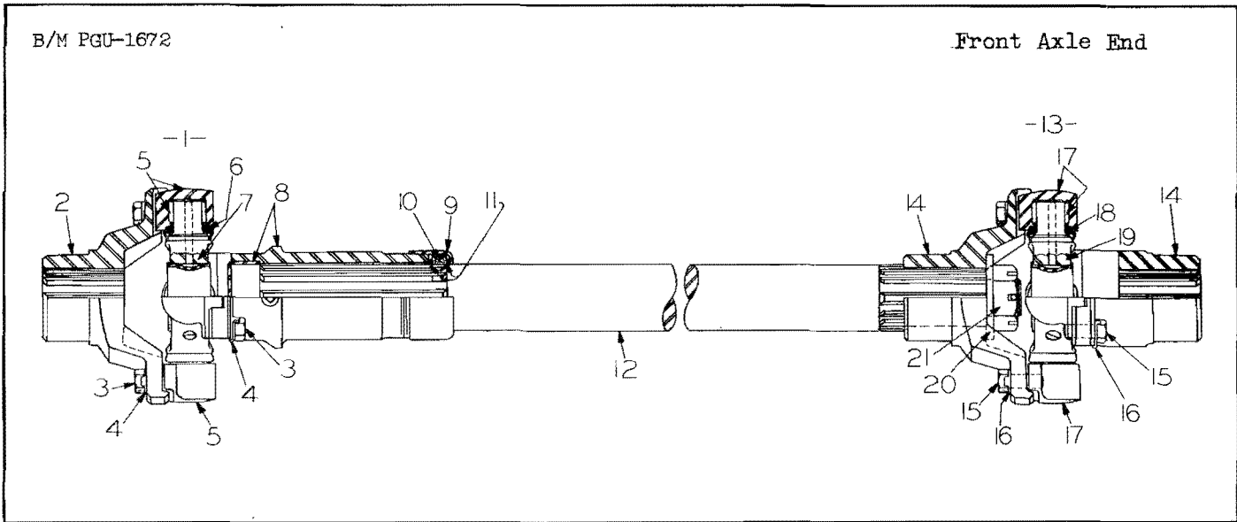
Figure 15. Front Section of Front Propeller Shaft
