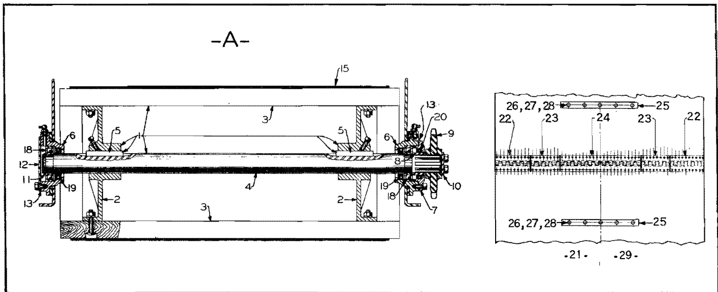
Figure 65. Conveyor Loader Head Drum and Belt
