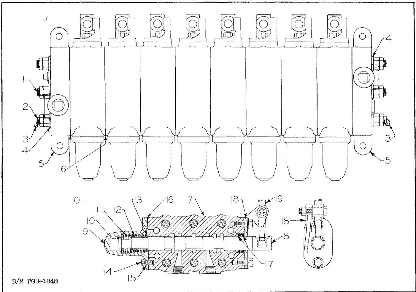
Figure 40. Hydraulic Valve Mechanism
