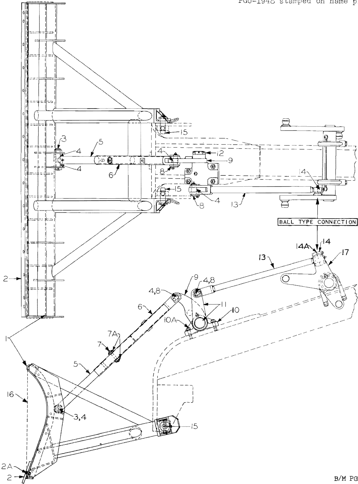
Figure 55. Bulldozer (2nd type)
