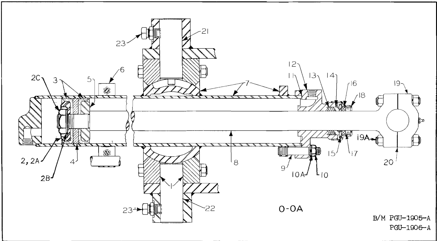
Figure 8. Blade Lift Ram
