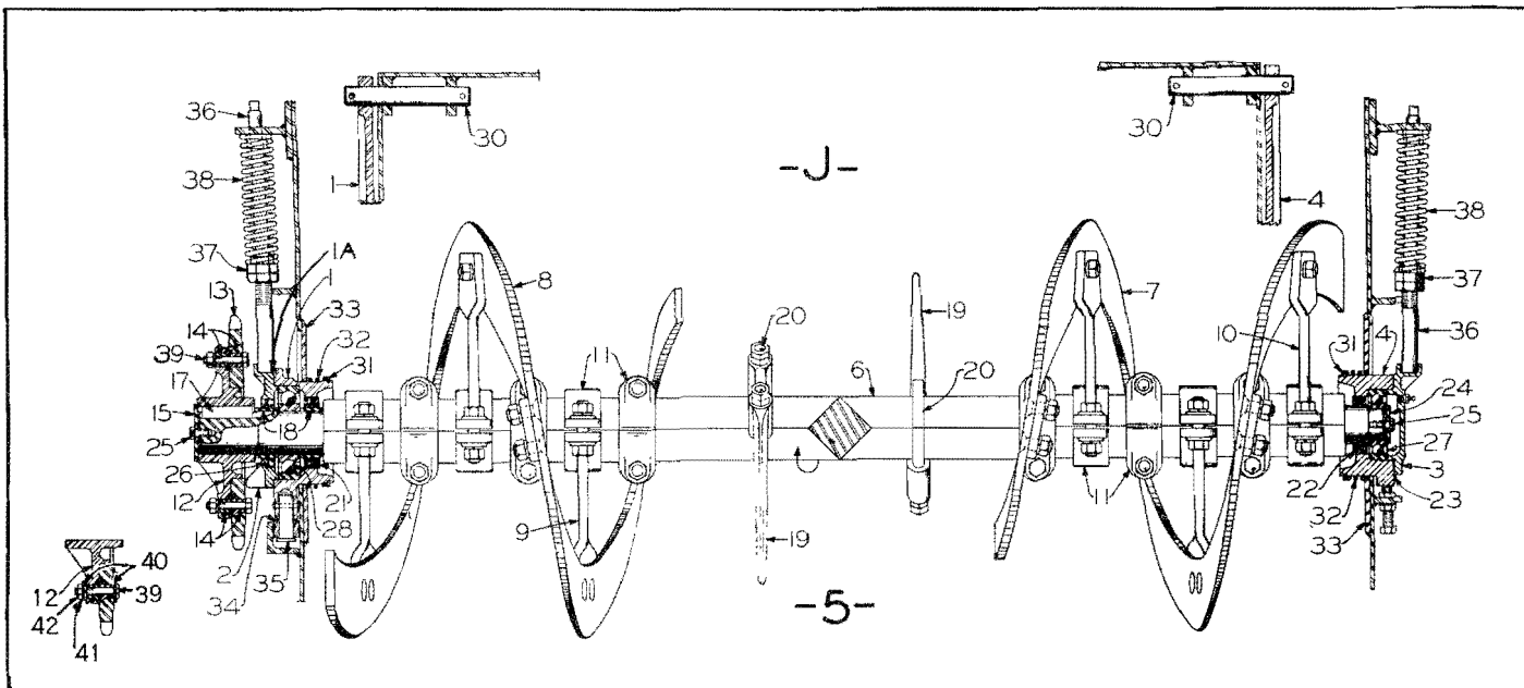
Figure 64. Conveyor Loader Feeder Shaft
