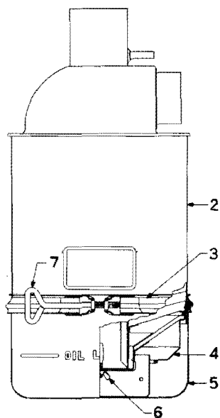
Figure 45. Air Cleaner for UD-14A Engine (Clamp ring type)
