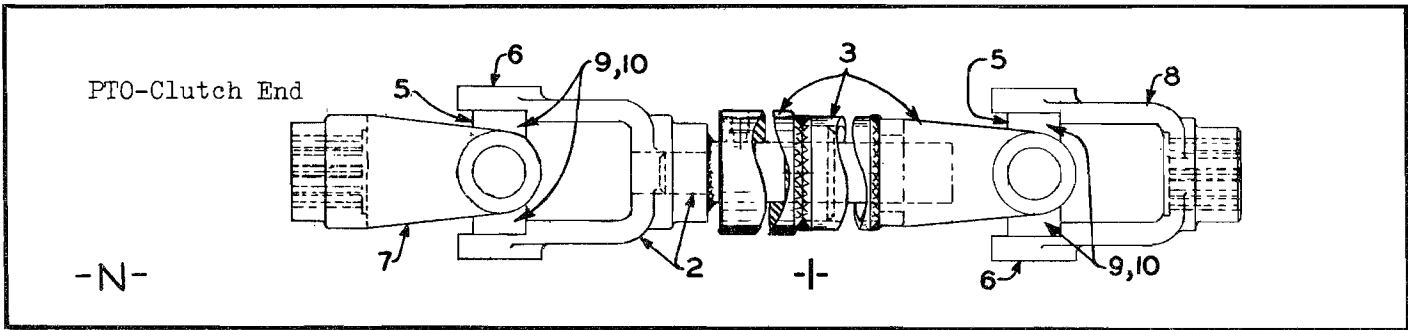
Figure 62. Conveyor Loader Propeller Shaft (Power Take-off to Bevel Gear Drive)
