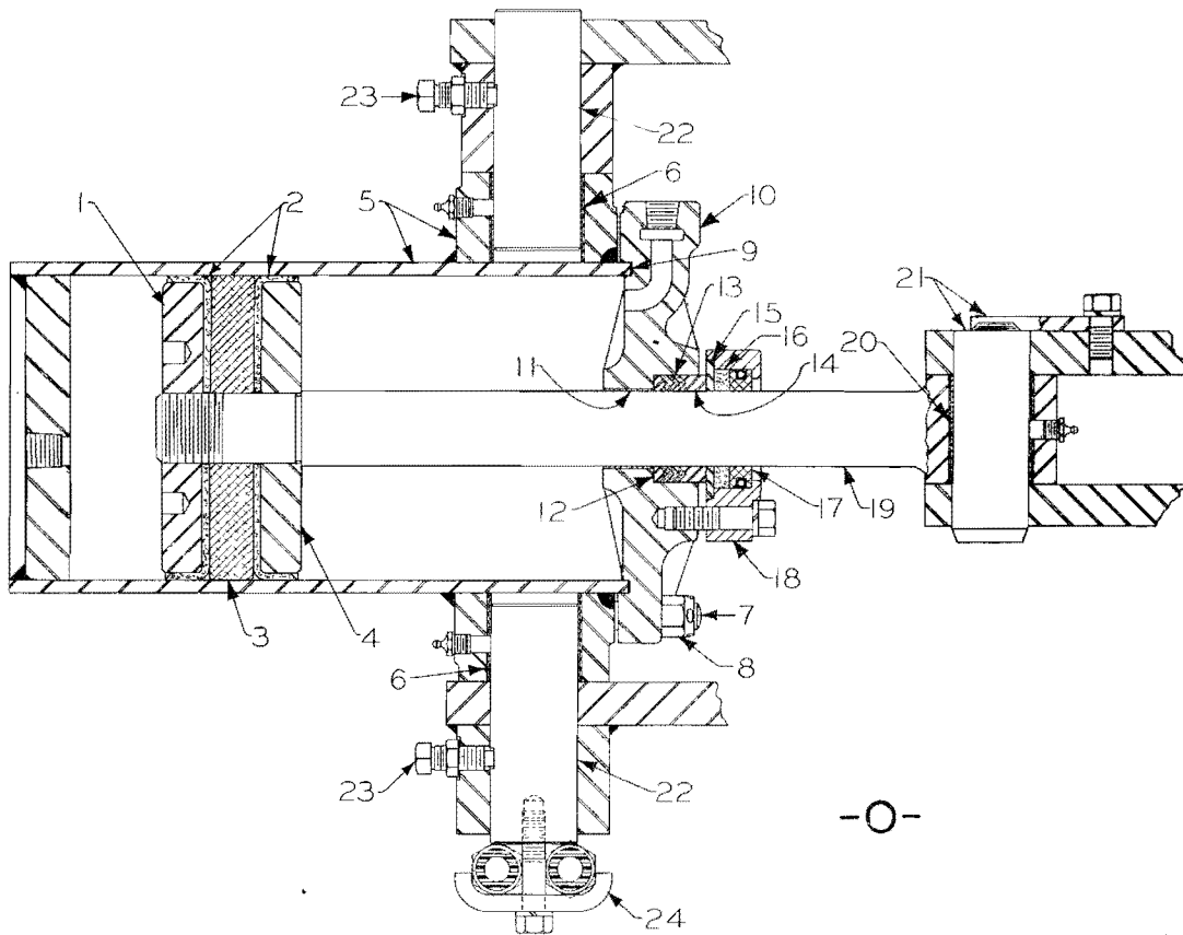
Figure 7. High Lift Ram (Machines H-100 to H-320 inclusive)
