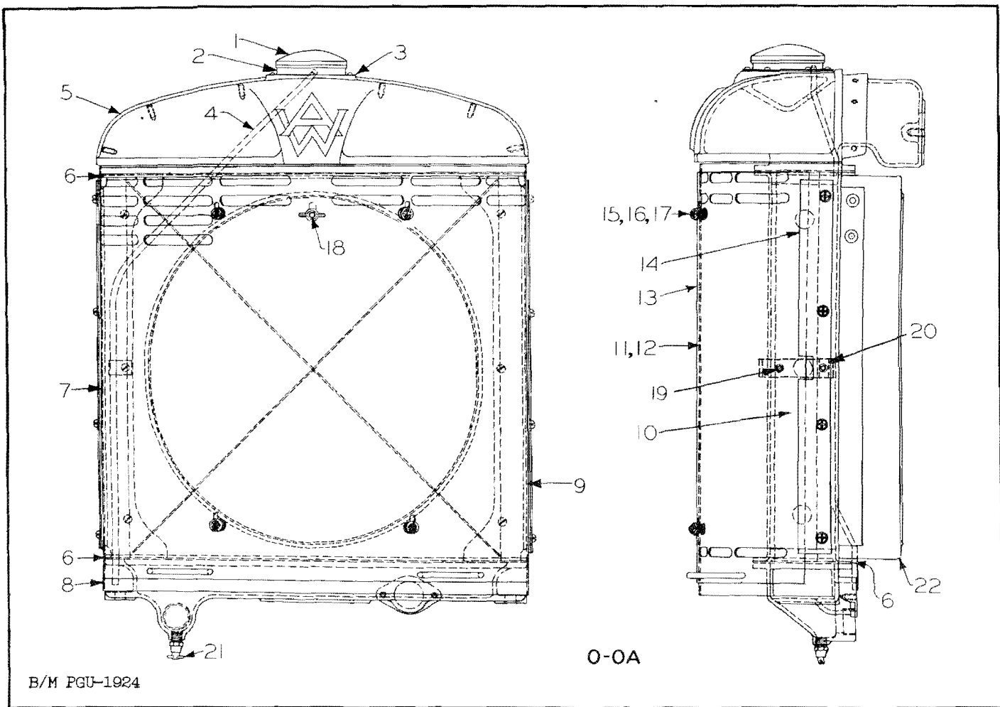
Figure 47. Radiator and Shutter for UD-14A Engine
