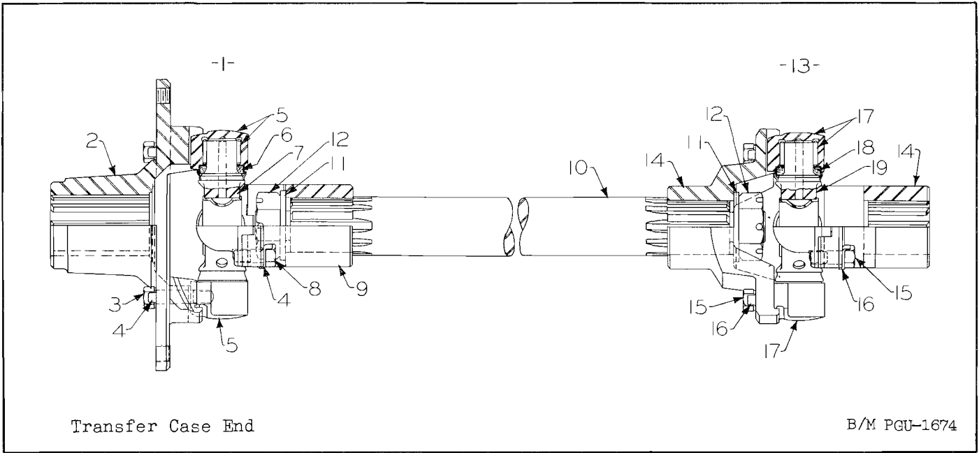
Figure 17. Rear Section of Front Propeller Shaft
