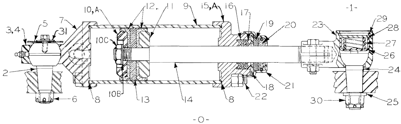
Figure 6. Front Axle Steering Ram
