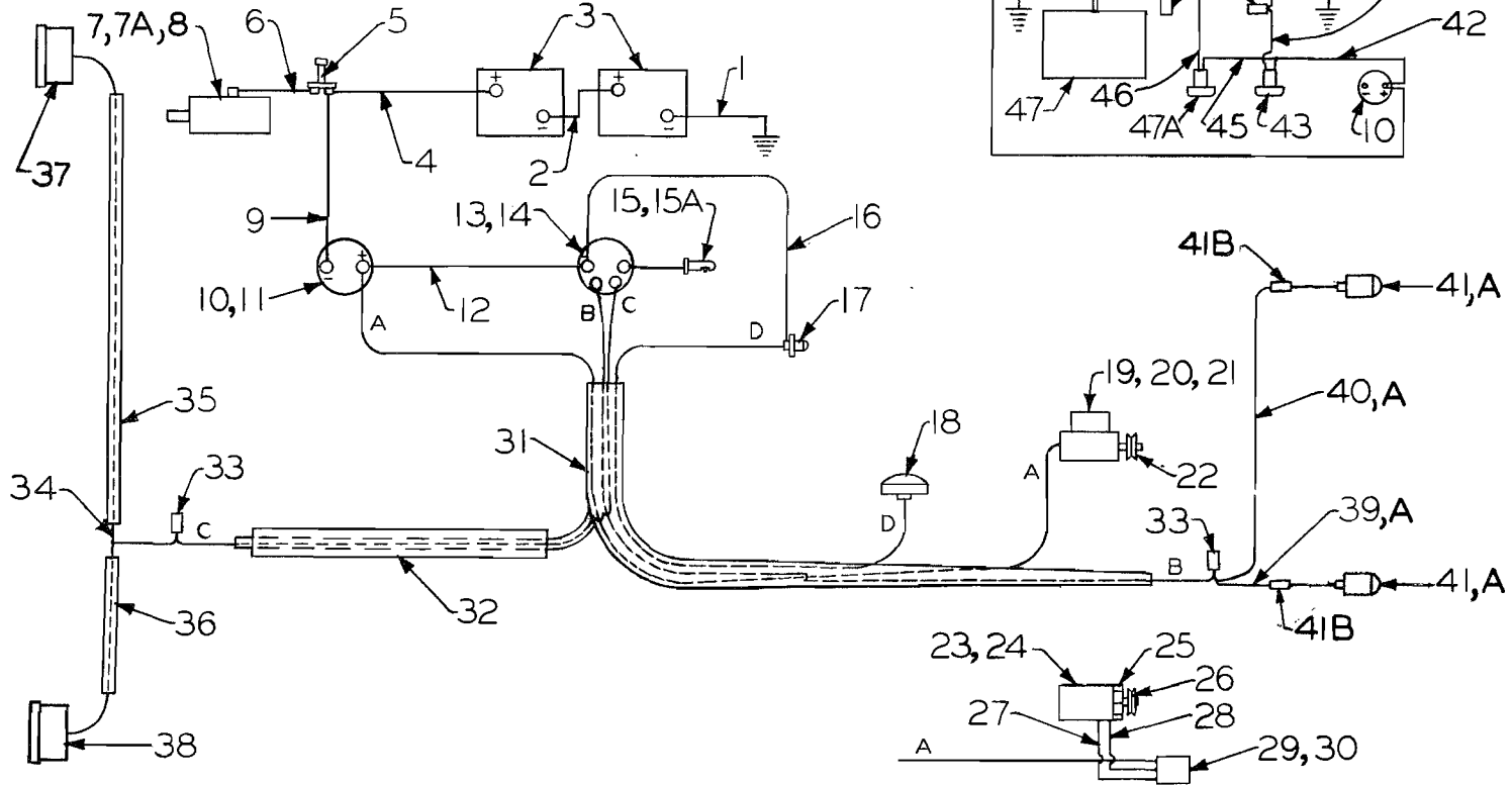
Wiring for heavy duty generator
