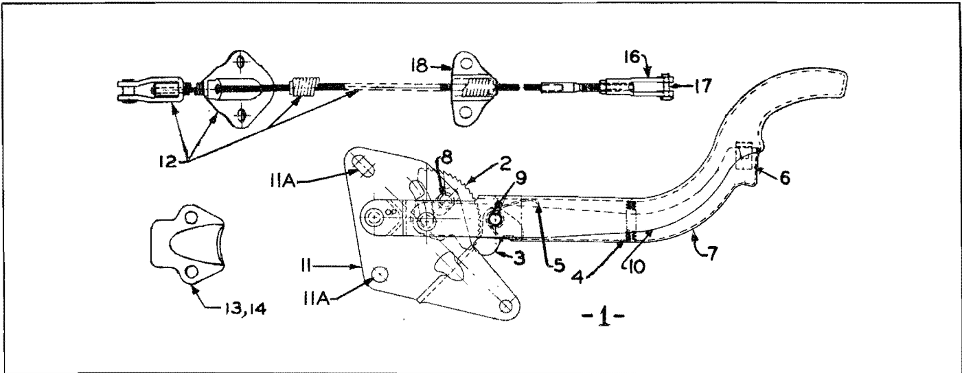
Figure 26. Hand Brake Mechanism
