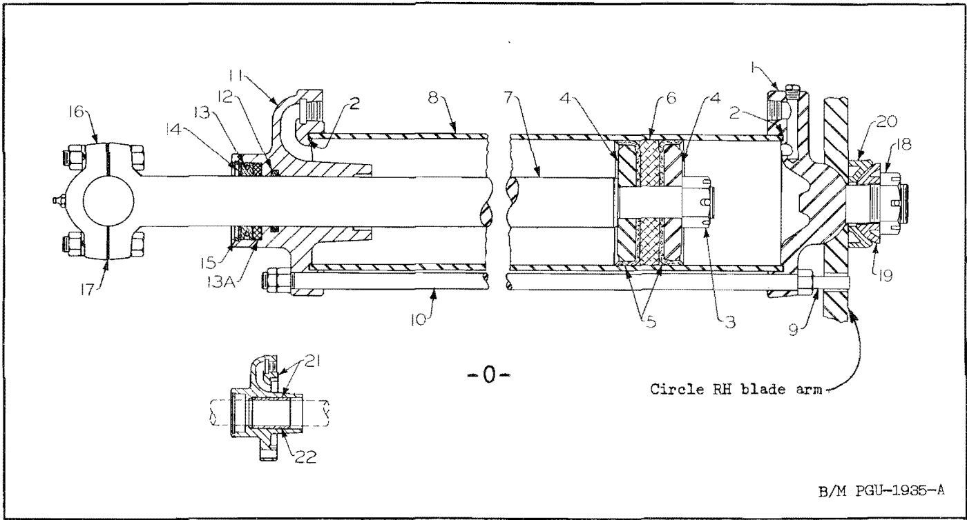
Figure 9A. Blade Side Shift Ram (Machines H-904 and up)
