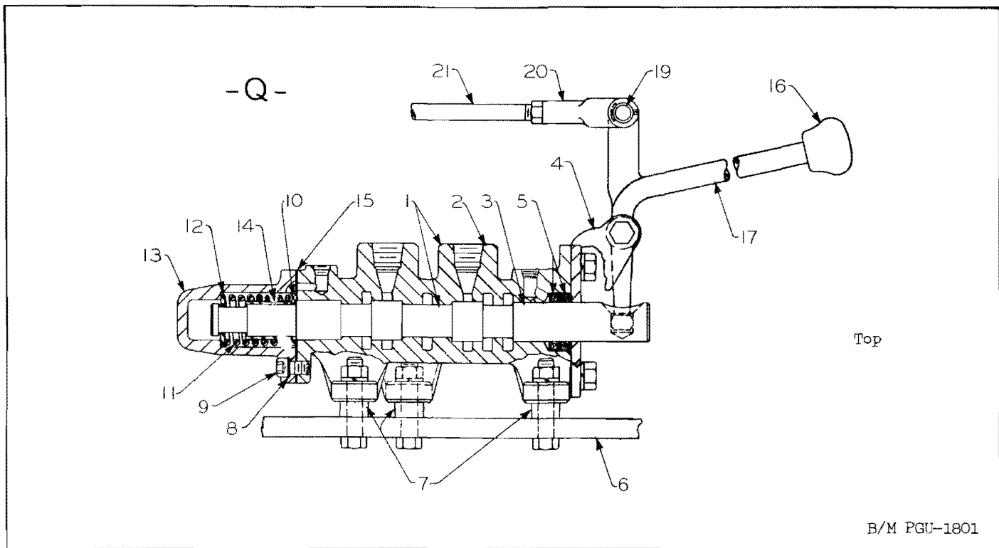
Figure 75. Conveyor Loader Hydraulic Control Valve
