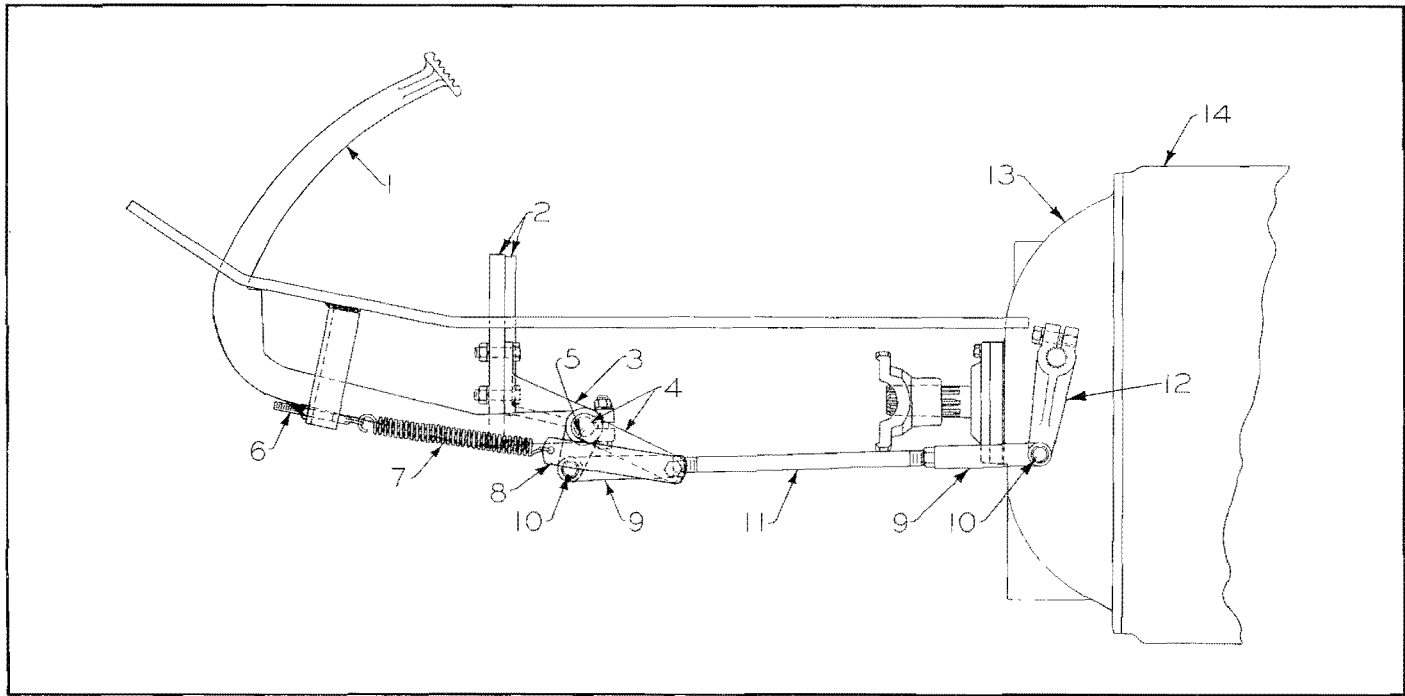
Figure 28. Clutch Operating Mechanism for UD-14A Engine
