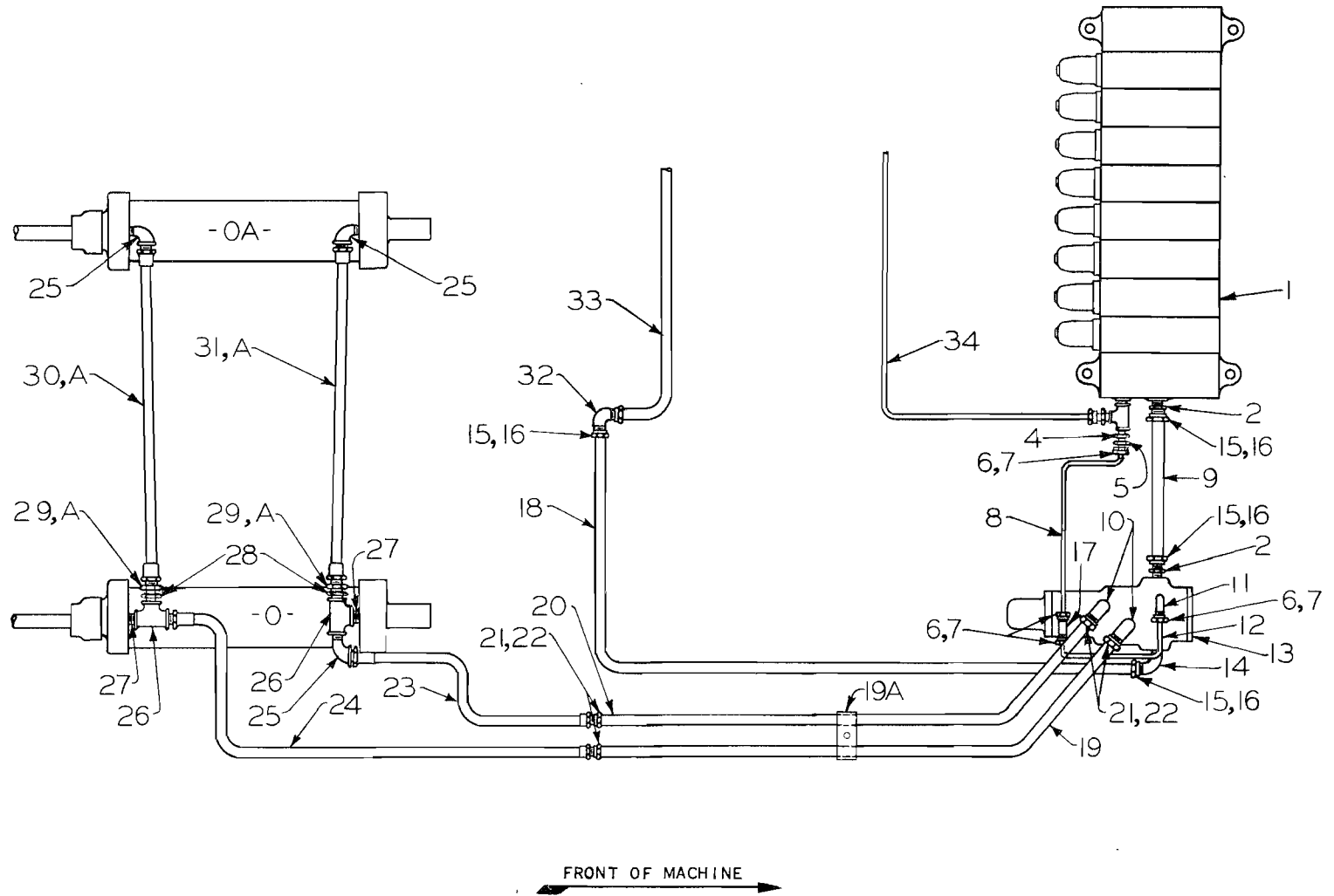
Figure 79. Rear Roller Hydraulic System (Piping Diagram)
