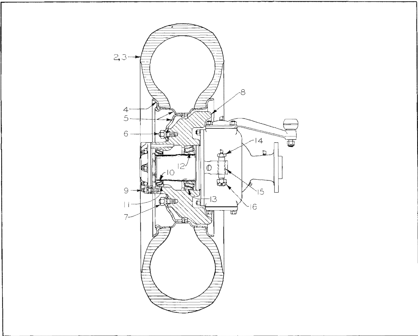
Figure 33. Left Rear Axle Steering Knuckle, Wheel and Tire
