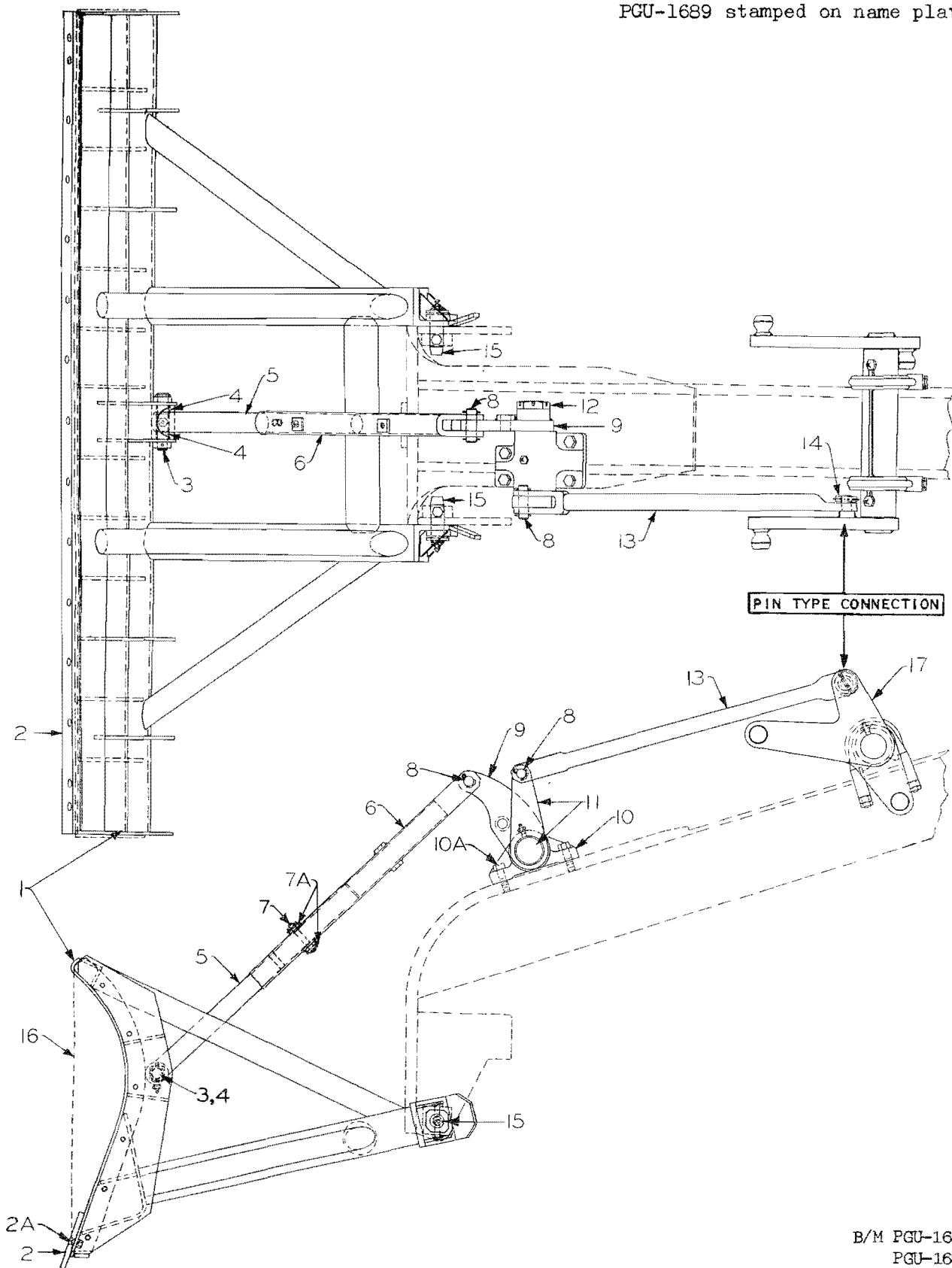
Figure 53. Bulldozer (1st type)
