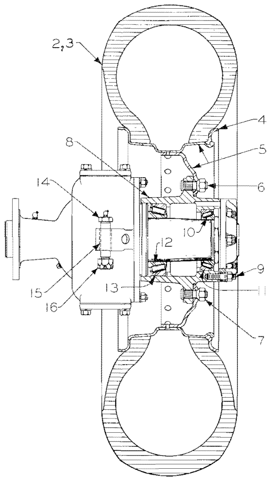
Figure 34. Right Rear Axle Steering Knuckle, Wheel and Tire
