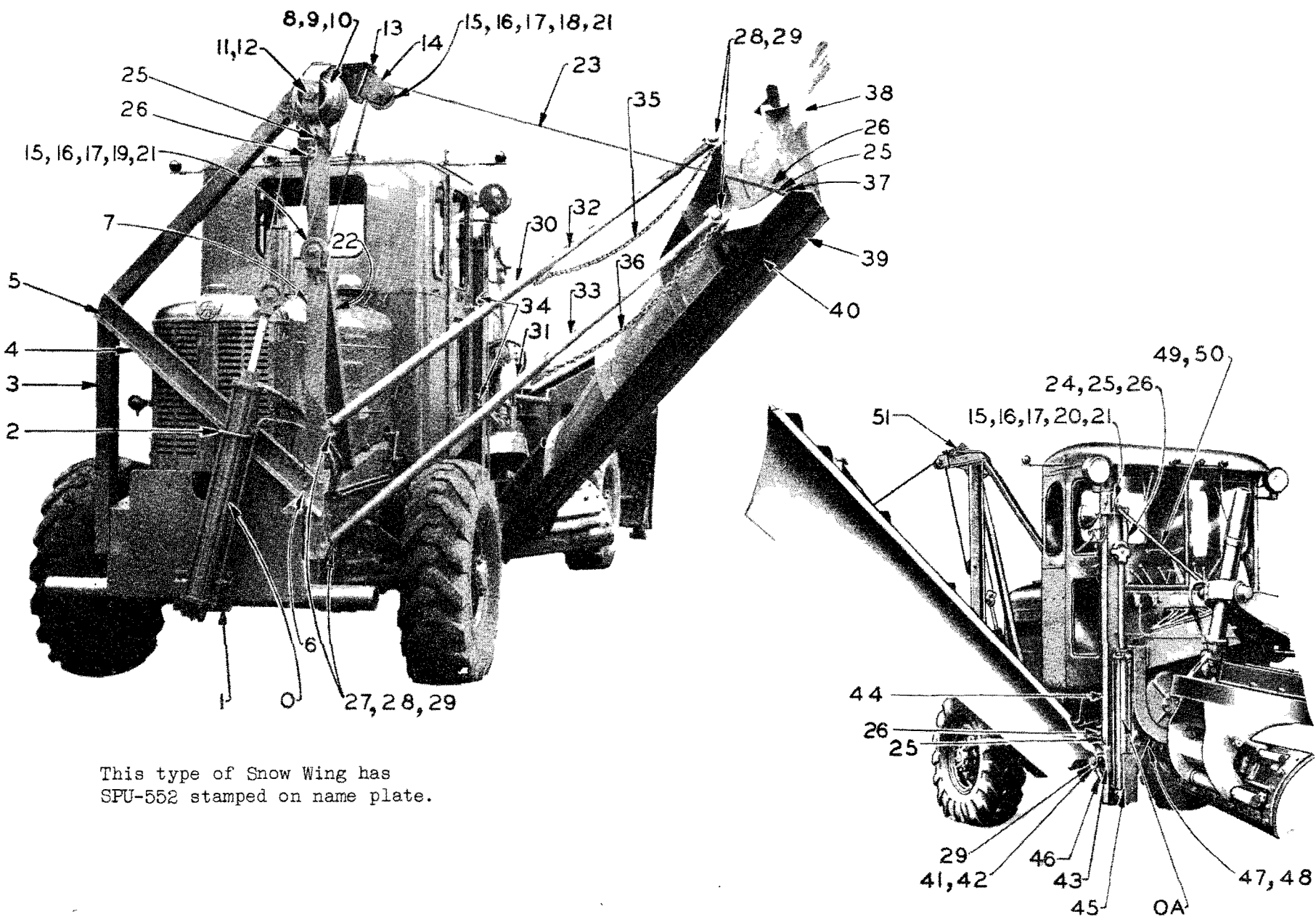
Figure 85. Snow Wing
