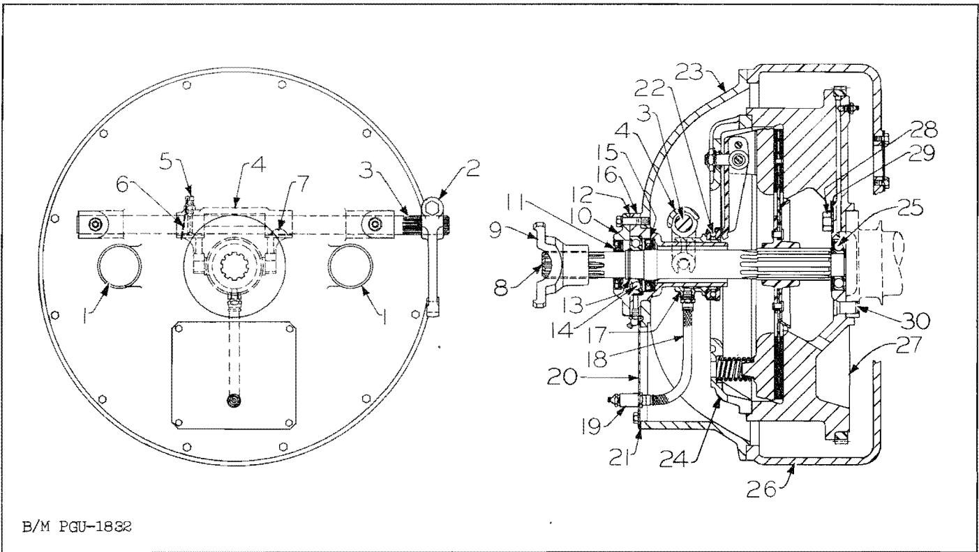
Figure 27. Clutch and Shaft Assembly for UD-14A Engine
