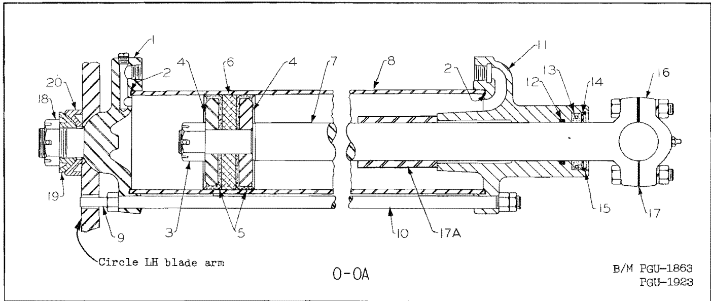
Figure 9. Blade Side Shift Ram (Machines H-100 to H-902 inclusive)
