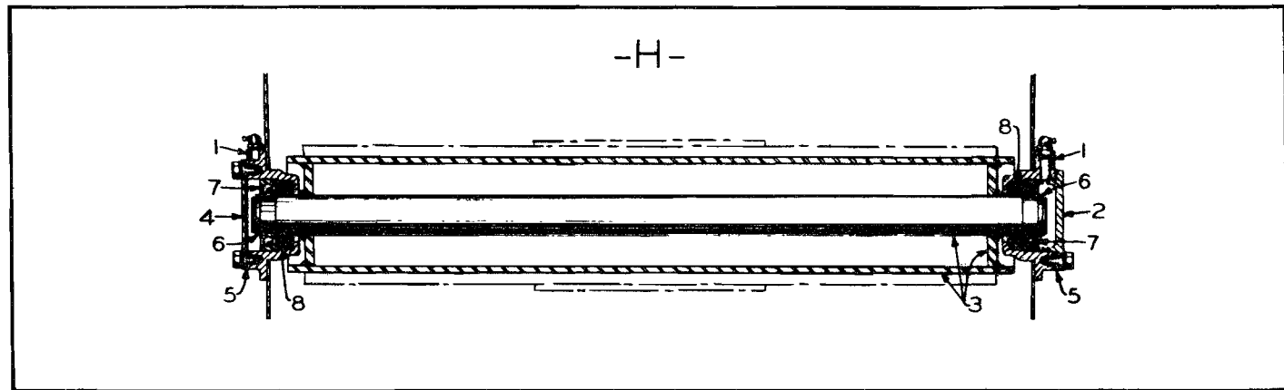
Figure 70. Conveyor Loader Tail Pulley
