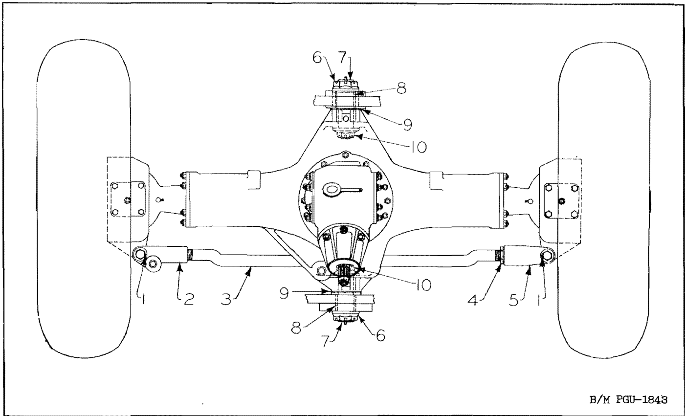
Figure 5. Front Axle Tie Rod and Axle Support
