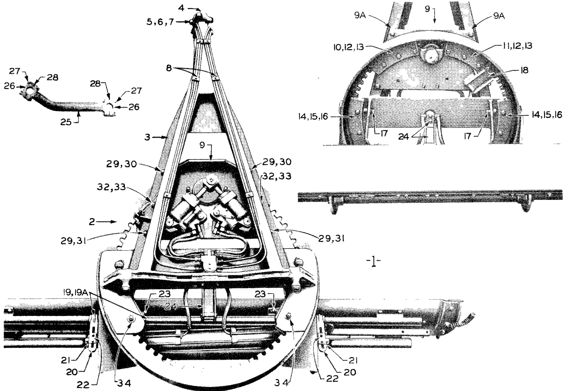
Figure 11. Circle and Draw Bar (Machines H-100 to H-902 inclusive)
