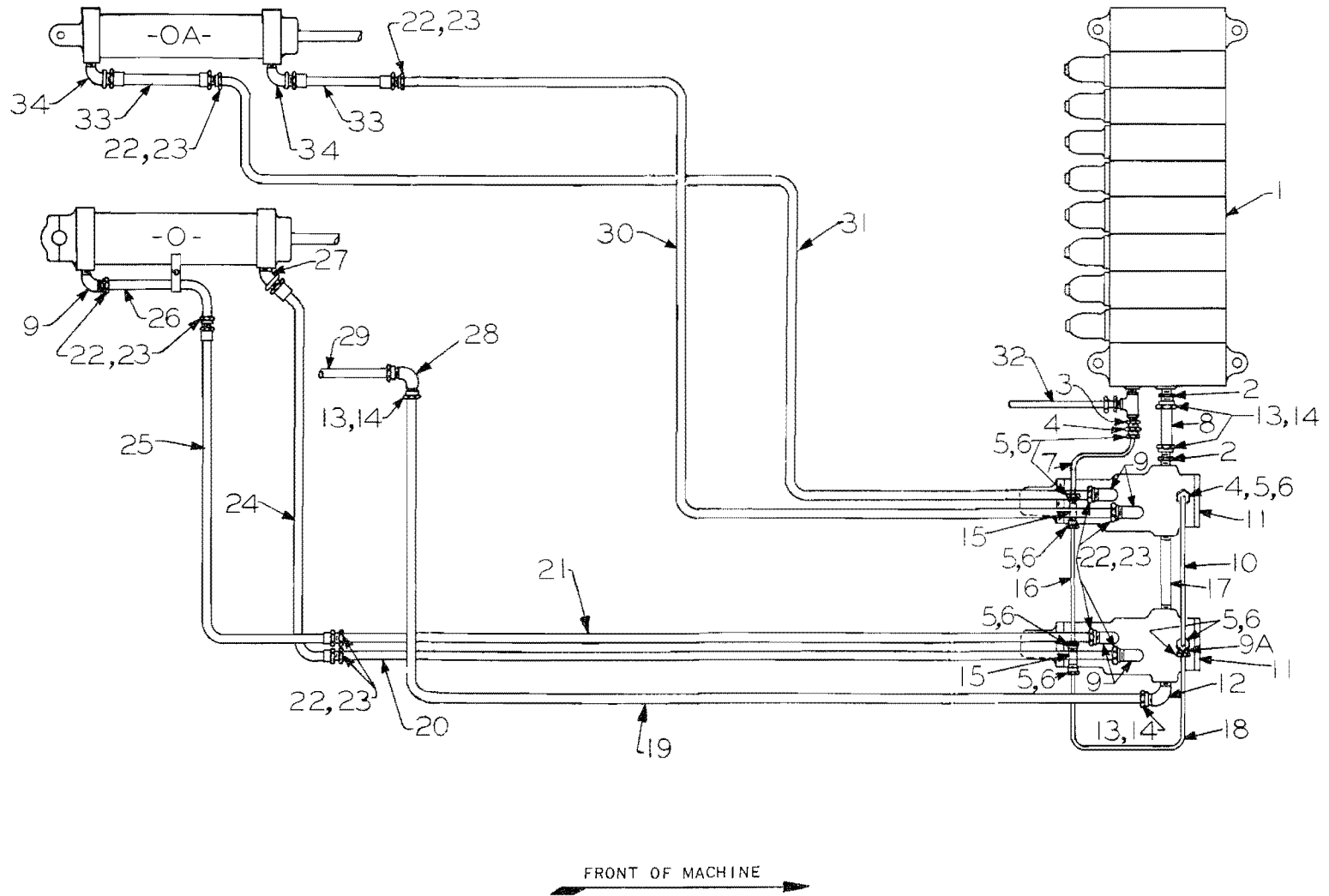
Figure 86. Snow Wing Hydraulic System (Piping Diagram)
