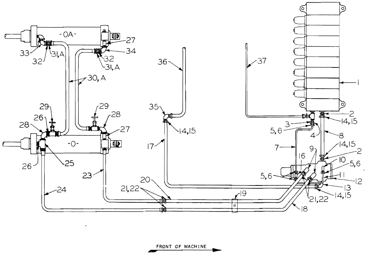
Figure 74. Conveyor Loader Hydraulic System (Piping Diagram)
