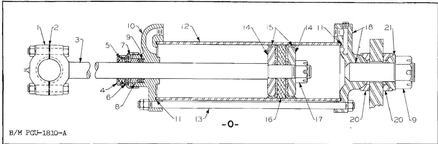
Figure 56. Scarifier Ram (2nd type) (Also used with Bulldozer and front Snow Plows)
