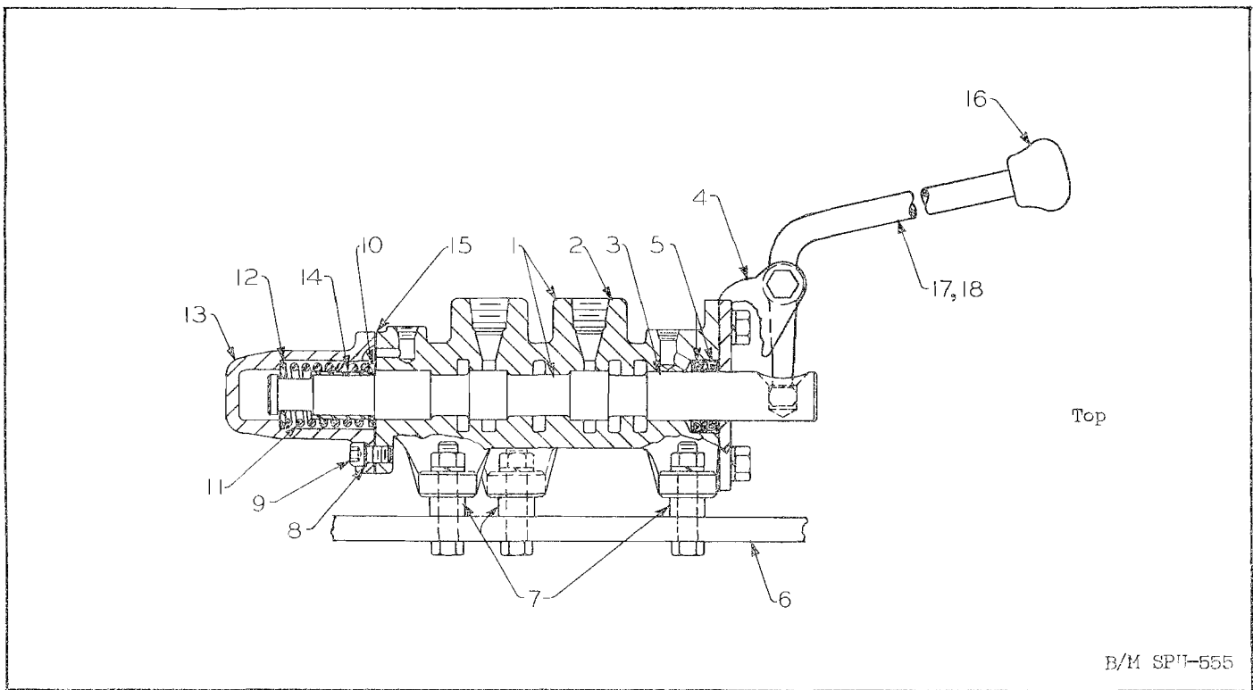
Figure 89. Snow Wing Hydraulic Control Valve
