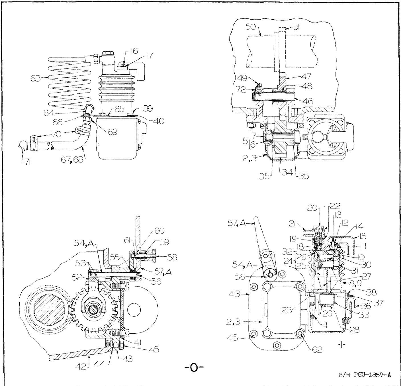
Figure 23. Tire Pump
