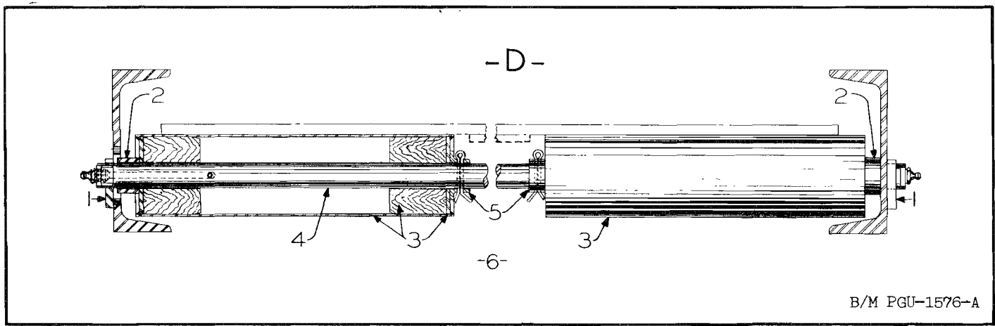
Figure 69. Conveyor Loader Return Roller
