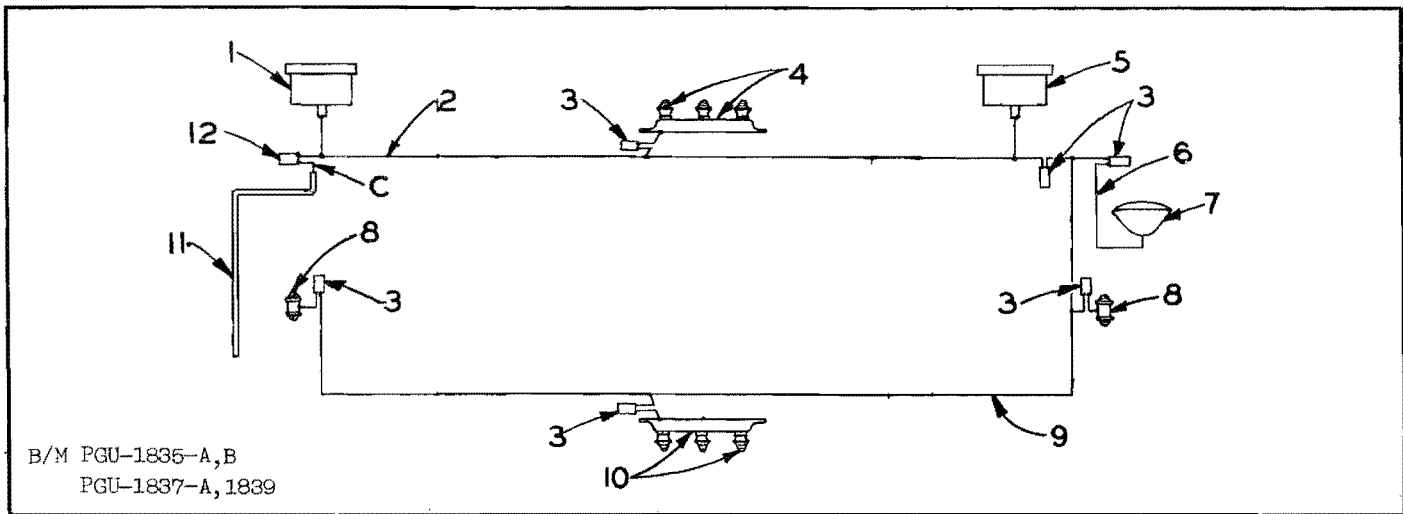
Figure 82. Wiring Diagram for Snow Removal Lights
