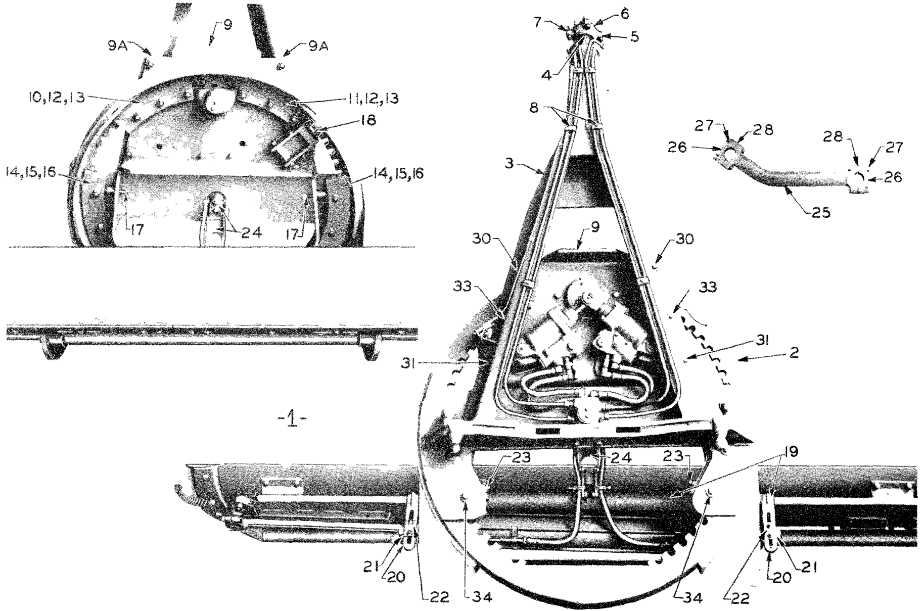
Figure 11A. Circle and Draw Bar (Machines H-904 and up)
