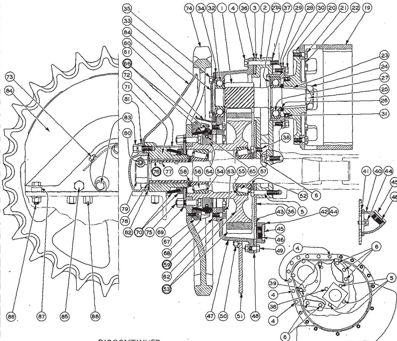
BOLT DIAGRAM FOR 52" TREAD MODEL
