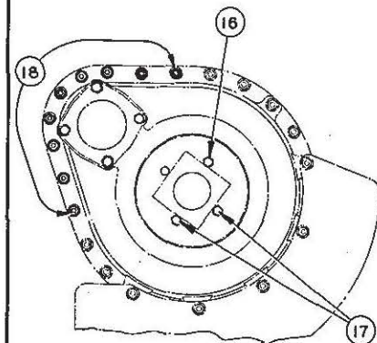
BOLT DIAGRAM FOR 63" TREAD MODEL
