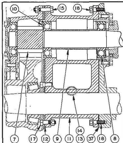
SPECIAL PARTS USED ON 63" TREAD MODEL
