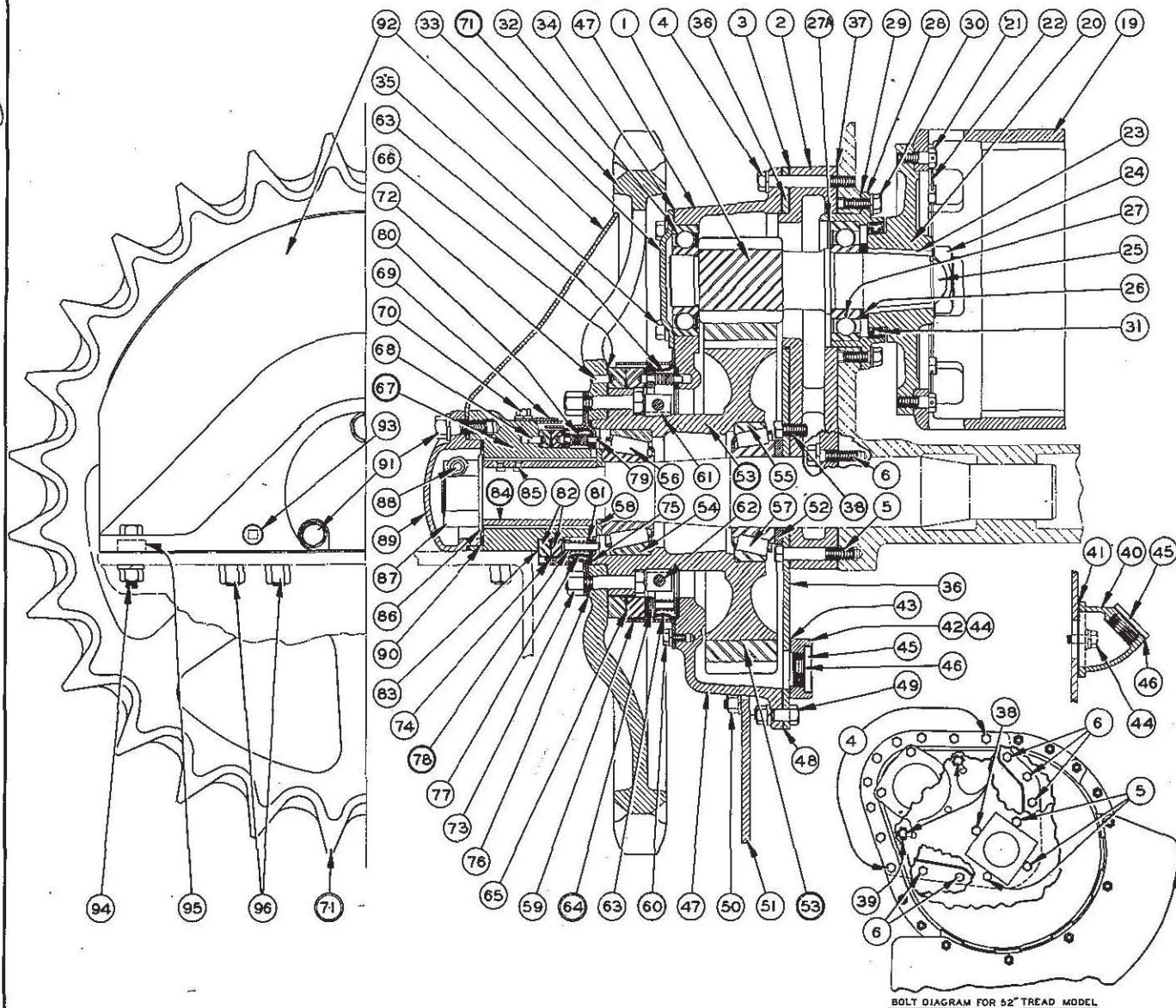
PLATE 1150 — FINAL DRIVE (SECOND TYPE)
