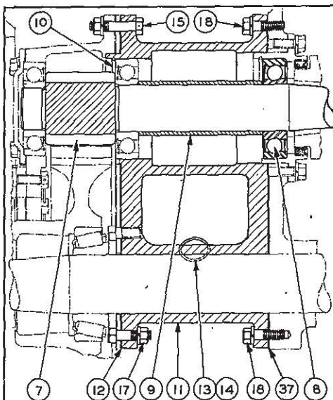
SPECIAL PARTS USED ON 63" TREAD MODEL
