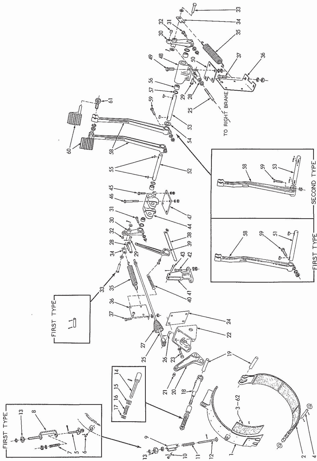
BRAKES (First type)
